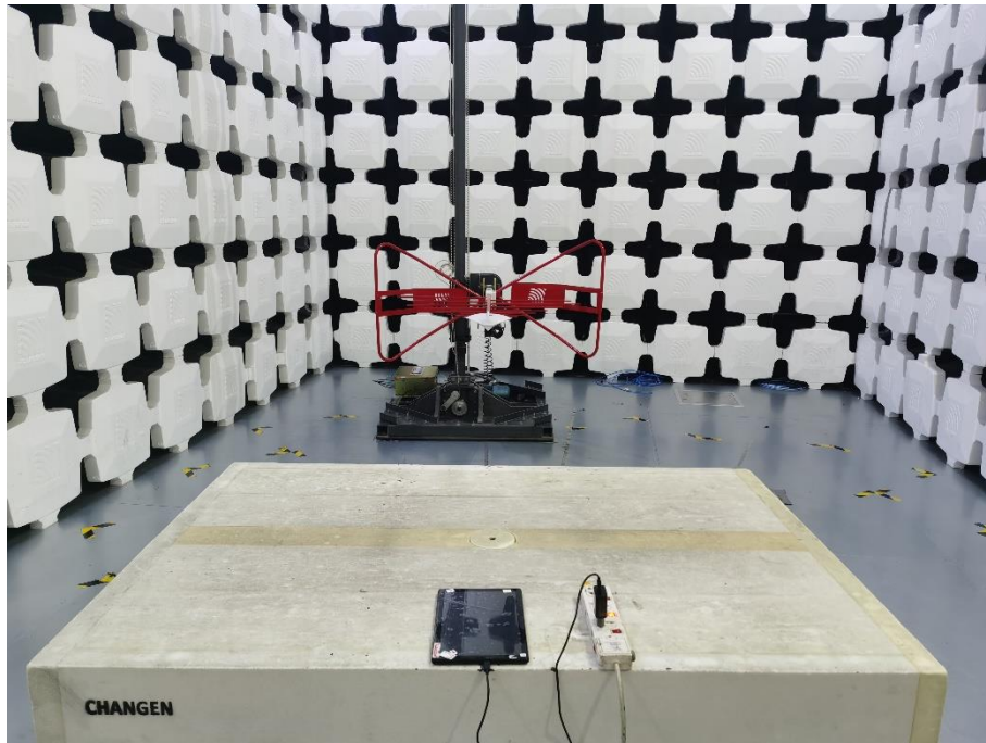
3. Radiated Emissions (Part 15B Charging Mode, 30MHz-1GHz)
