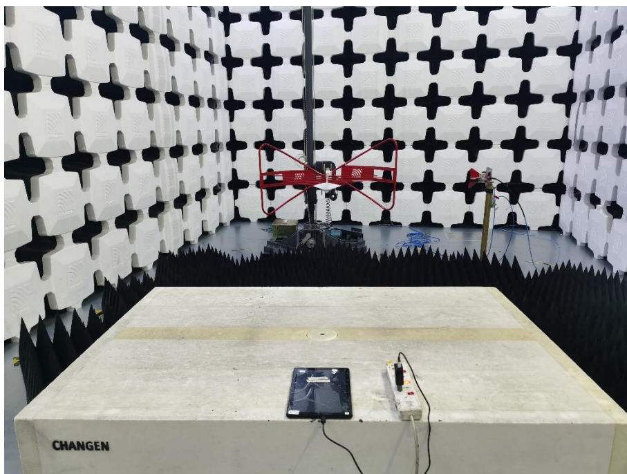
4. Radiated Emissions (Part 15B Charging Mode, 1GHz-18GHz)
