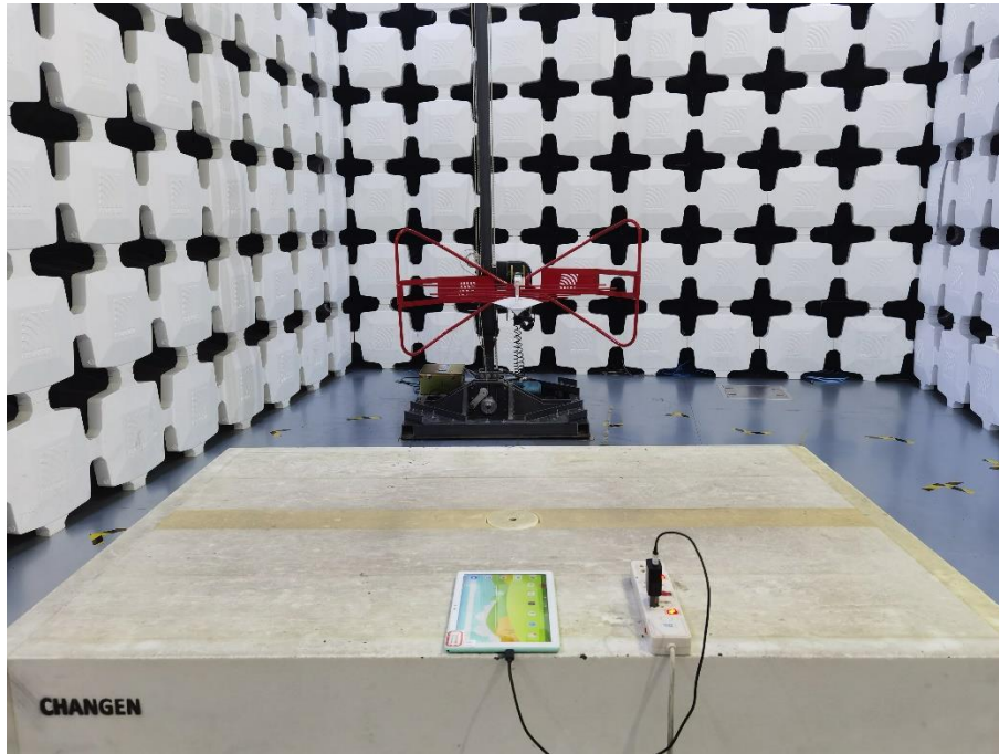
3. Radiated Emissions (Part 15B Camera/Video Player, 30MHz-1GHz)
