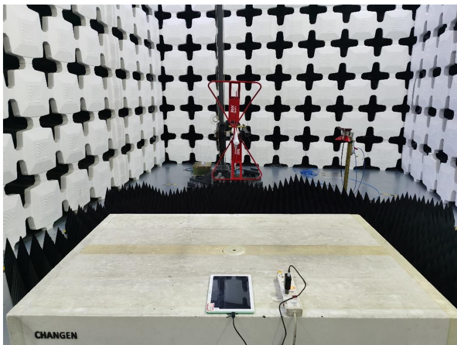
4. Radiated Emissions (Part 15B Camera/Video Player, 1GHz-18GHz)
