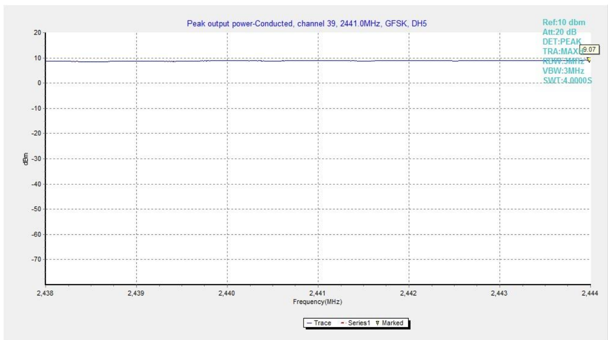
Fig. 2 RF output power (GFSK, Ch 39)
