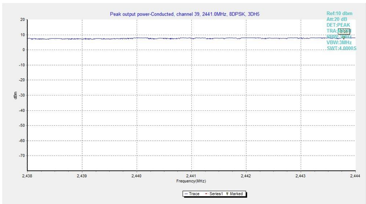
Fig. 8 RF output power (8DPSK, Ch 39)
