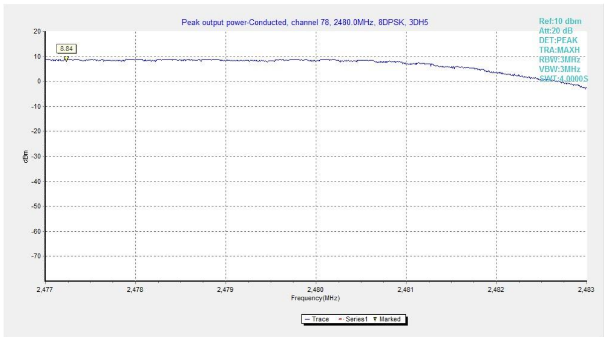
Fig. 9 RF output power (8DPSK, Ch 78)
