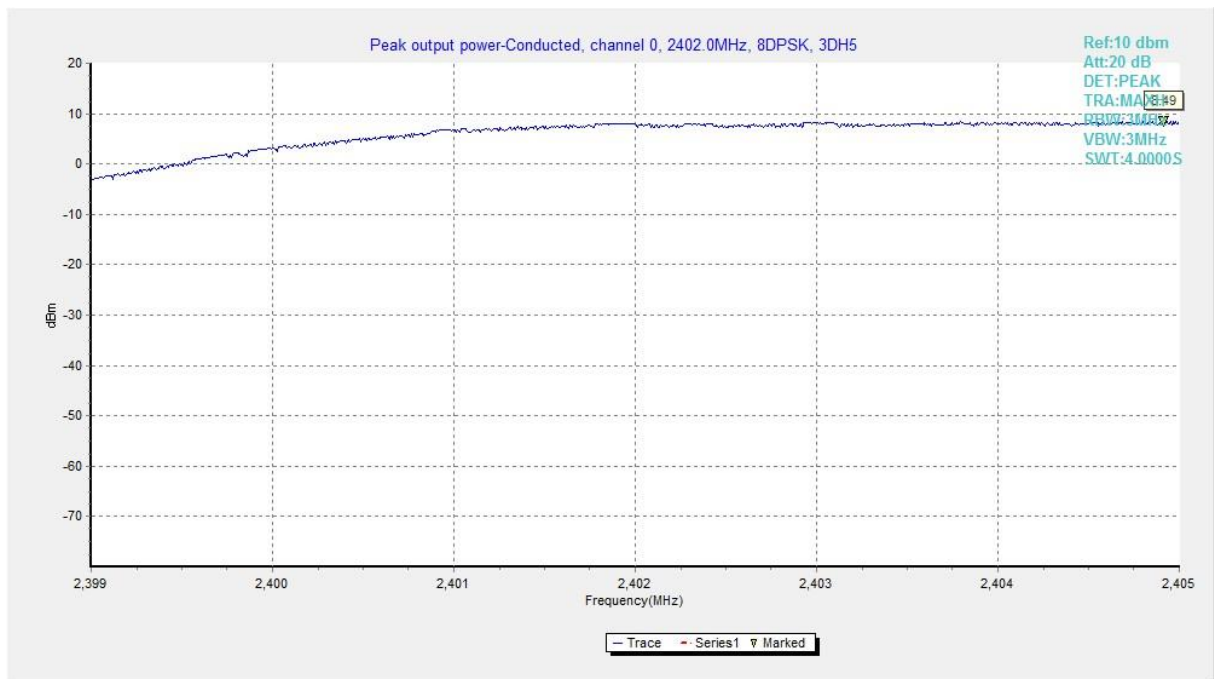
Fig. 7 RF output power (8DPSK, Ch 0)
