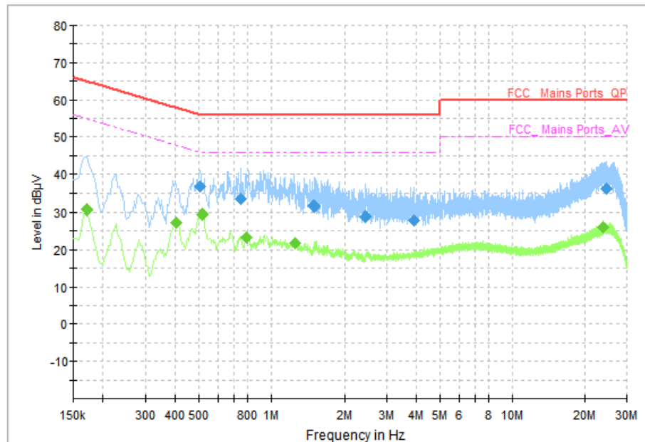
Fig.62 AC Power line Conducted Emission (Idle, LE 1M)
