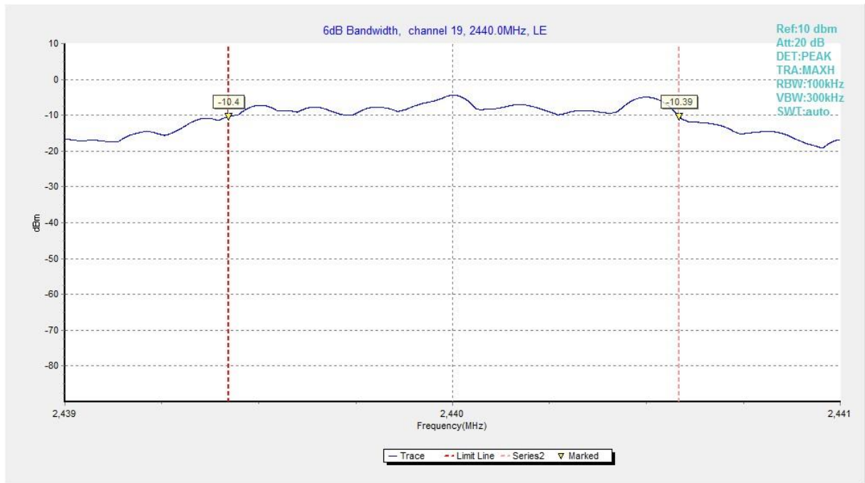
Fig.17 6dB Bandwidth (Ch 19), LE 2M
