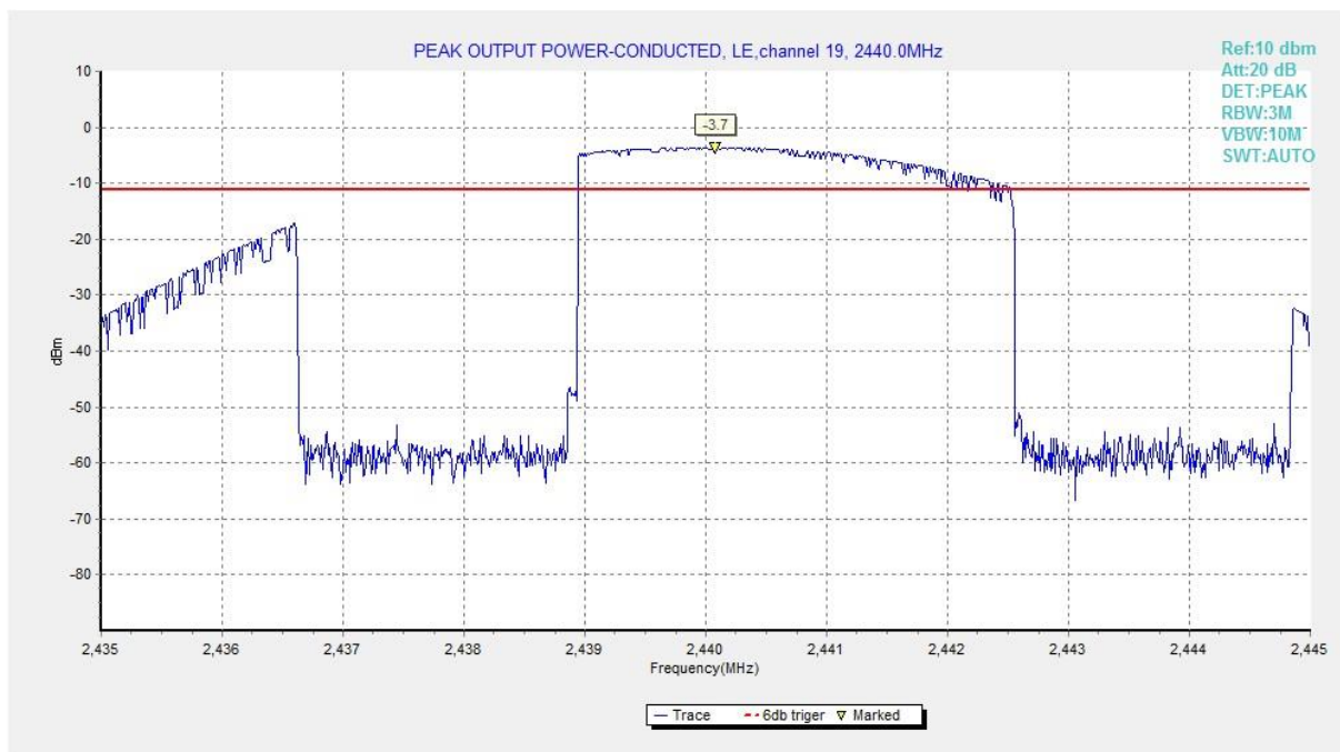
Fig.2 Peak Conducted Output Power (Ch 19), LE 1M
