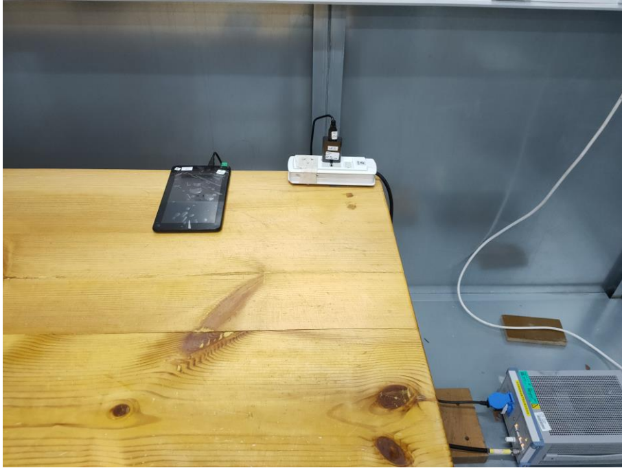
11. Conducted Emission (Part 15C, Bluetooth/Wi-Fi)
