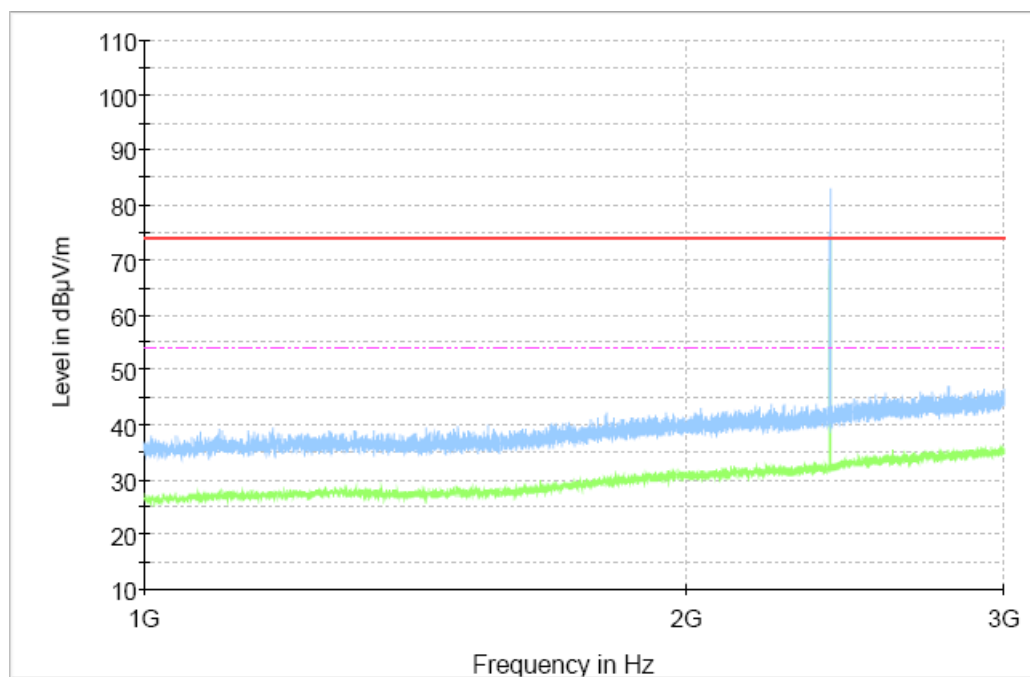
Fig.42 Radiated Spurious Emission (Ch19, 1 GHz - 3 GHz), 1M
