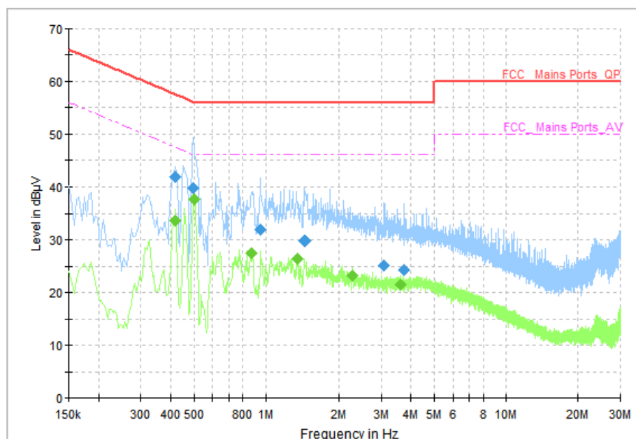
Fig.64 AC Power line Conducted Emission (Idle, AE3, 120V), 2M
