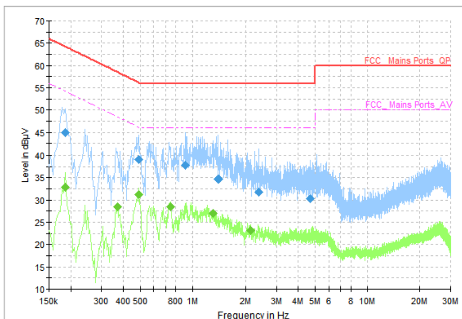
Fig.58 AC Power line Conducted Emission (Idle, AE2, 120V), 1M
