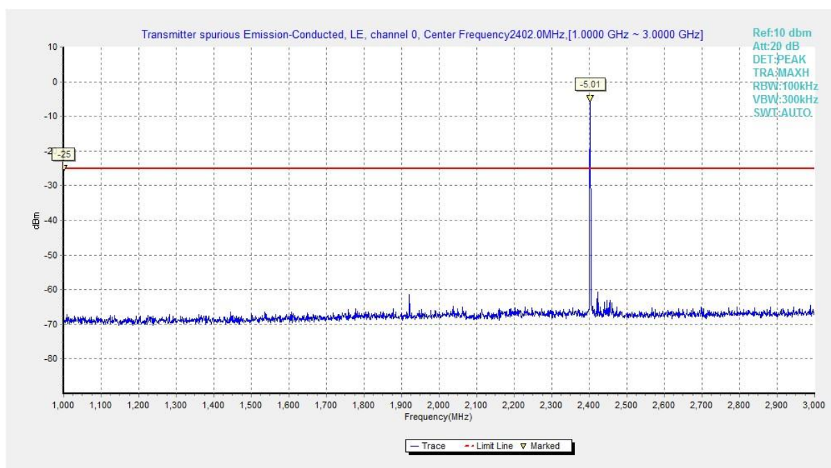
Fig.18 Conducted Spurious Emission (Ch0, 1 GHz-3 GHz), LE 1M
