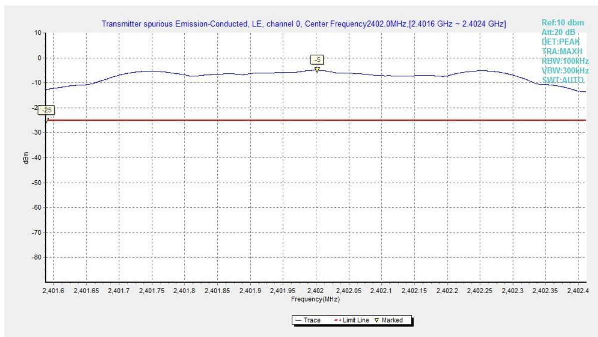
Fig.17 Conducted Spurious Emission (Ch0, Center Frequency), LE 1M
