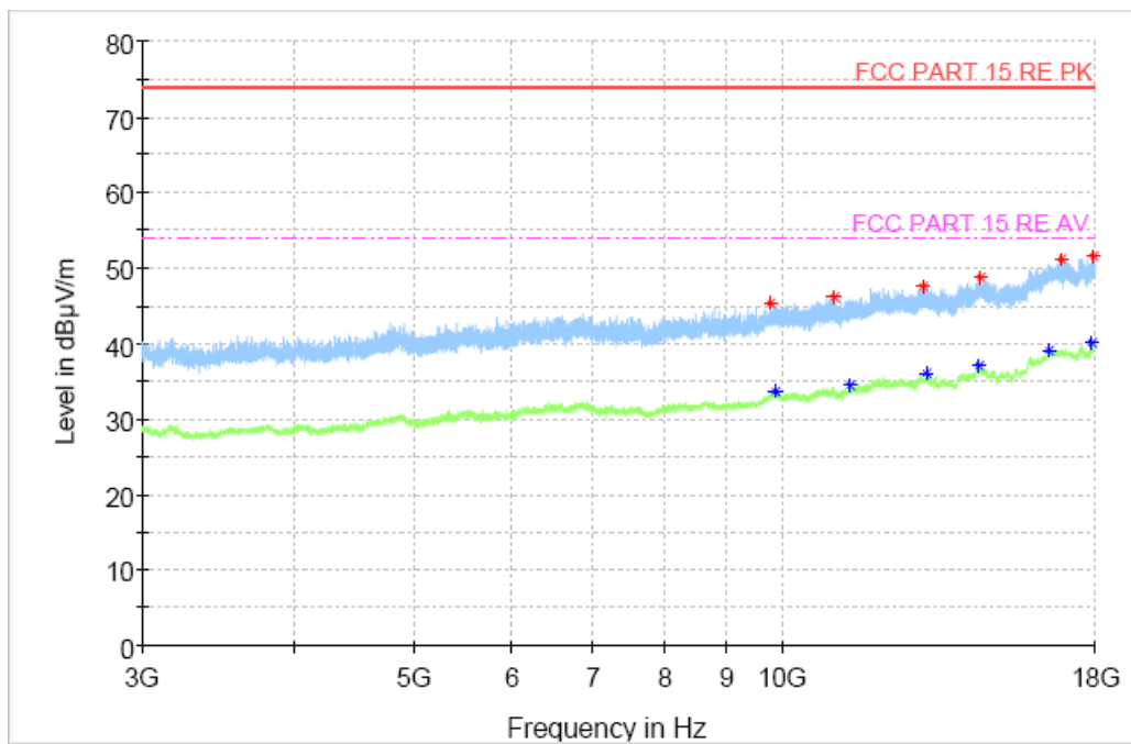
Fig.54 Radiated Spurious Emission (Ch39, 3 GHz - 18 GHz), 2M
