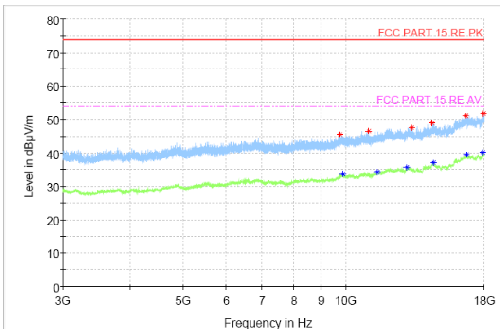
Fig.52 Radiated Spurious Emission (Ch19, 3 GHz - 18 GHz), 2M
