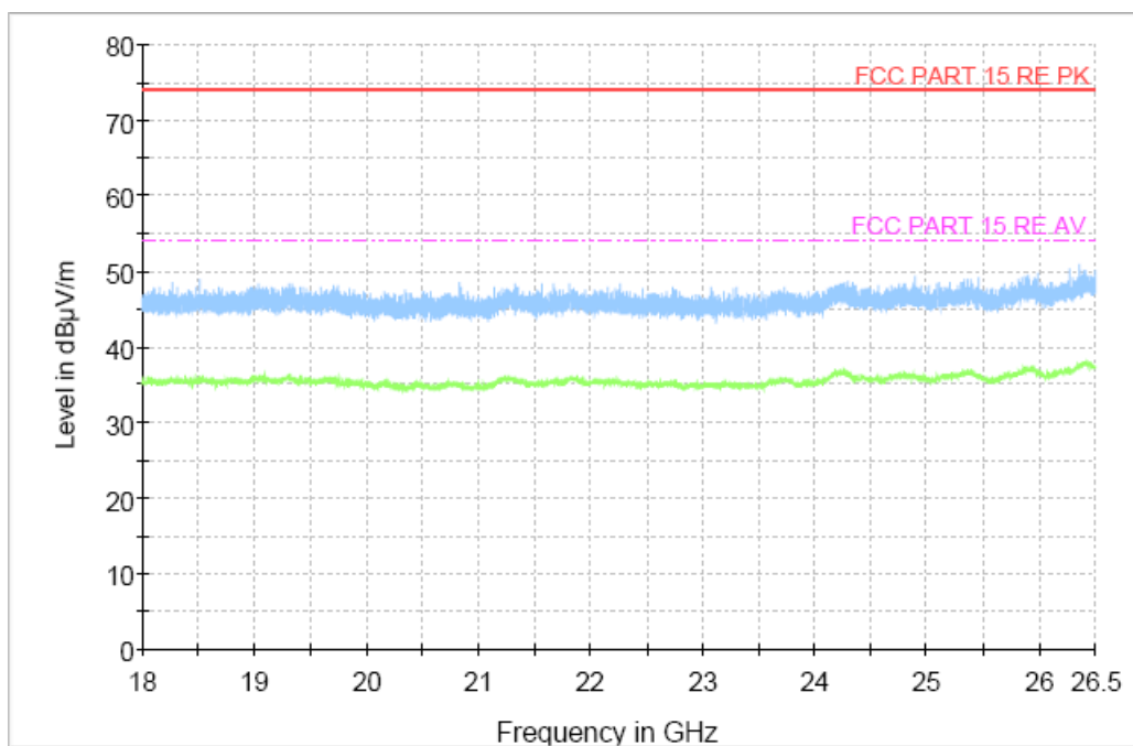
Fig.44 Radiated Spurious Emission (Ch19, 18 GHz - 26.5 GHz), 1M
