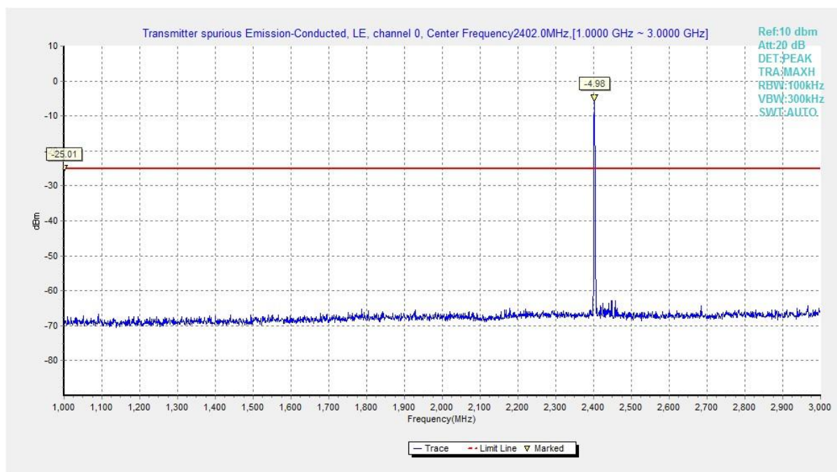
Fig.29 Conducted Spurious Emission (Ch0, 1 GHz-3 GHz), LE 2M
