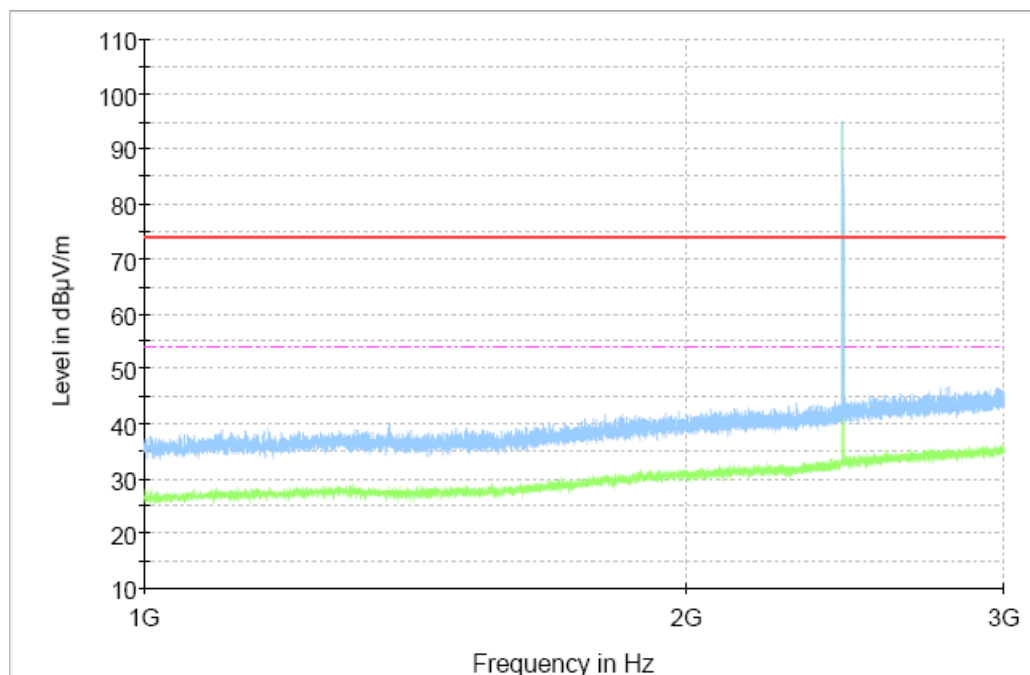
Fig. 59 Radiated Spurious Emission (All Channels, 1GHz ~ 3GHz)
