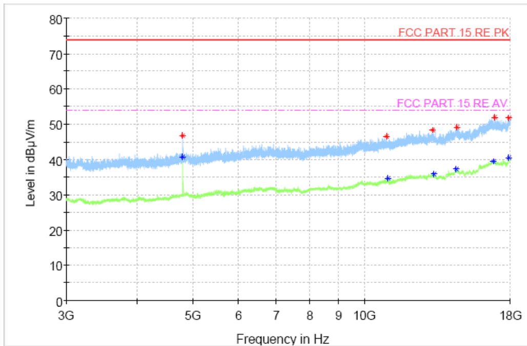
Fig. 52 Radiated Spurious Emission (8DPSK, Ch0, 3GHz ~ 18GHz)
