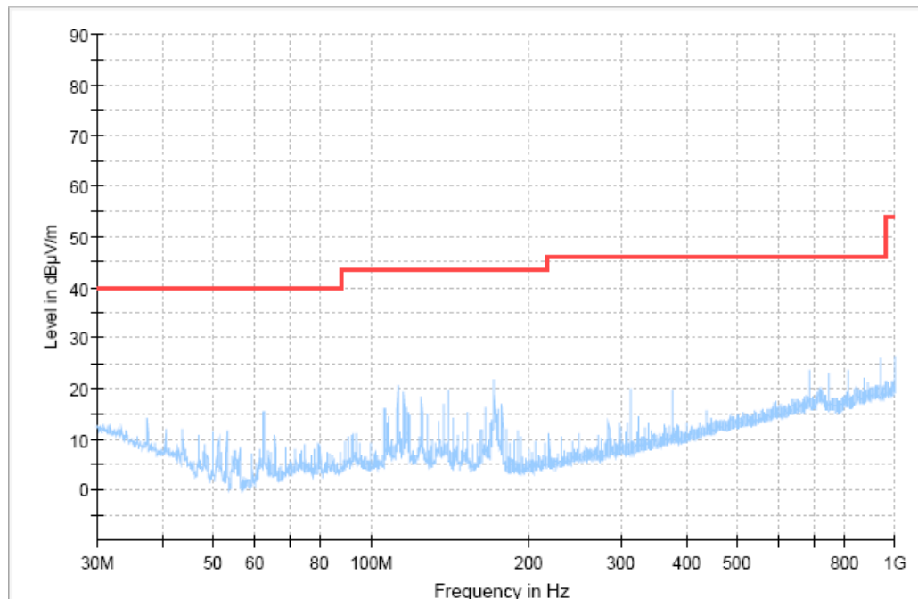
Fig. 58 Radiated Spurious Emission (All Channels, 30MHz ~ 1GHz)
