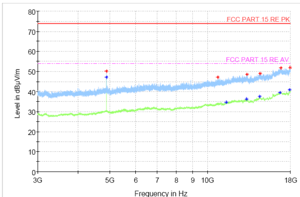
Fig. 43 Radiated Spurious Emission (GFSK, Ch39, 3GHz ~ 18GHz)
