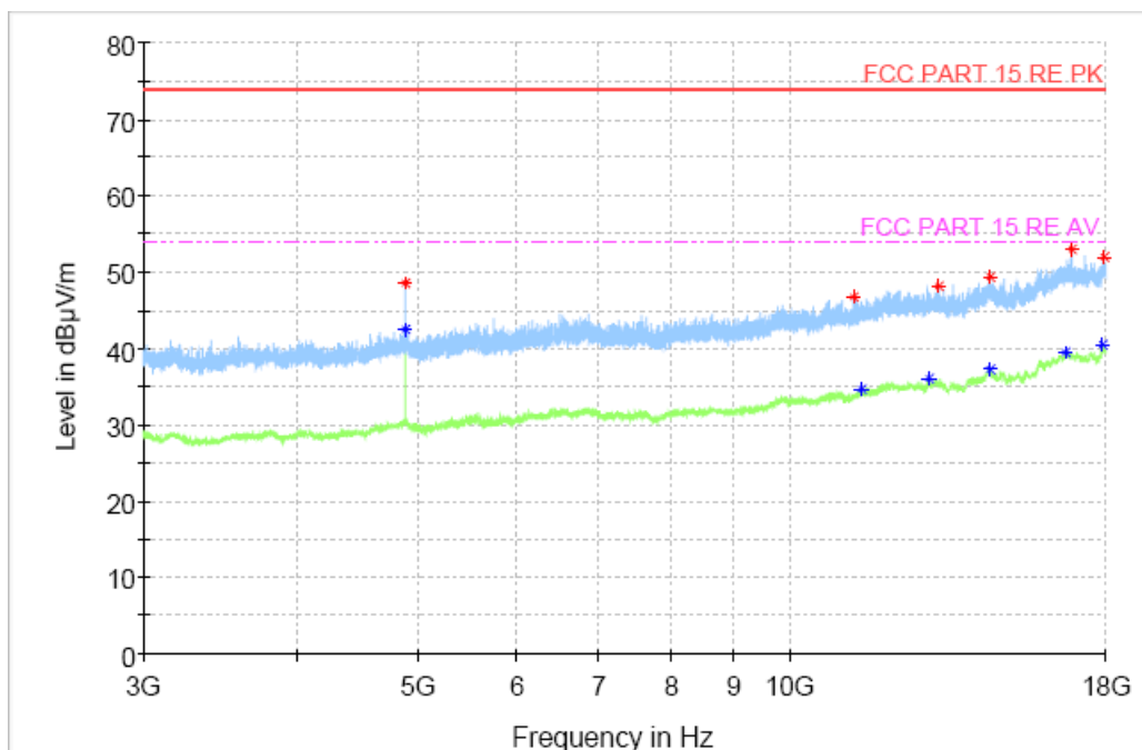
Fig. 53 Radiated Spurious Emission (8DPSK, Ch39, 3GHz ~ 18GHz)
