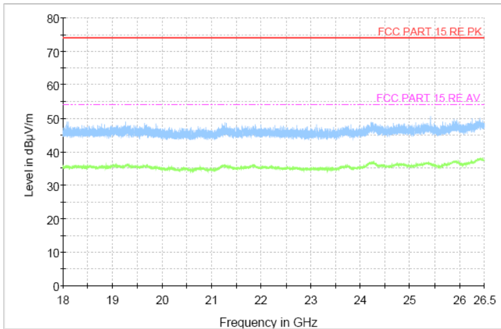
Fig. 60 Radiated Spurious Emission (All Channels, 18GHz ~ 26.5GHz)
