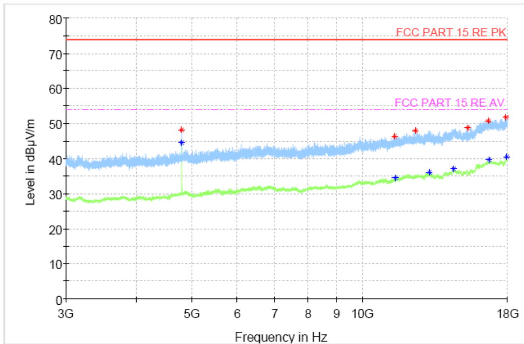
Fig. 42 Radiated Spurious Emission (GFSK, Ch0, 3GHz ~ 18GHz)
