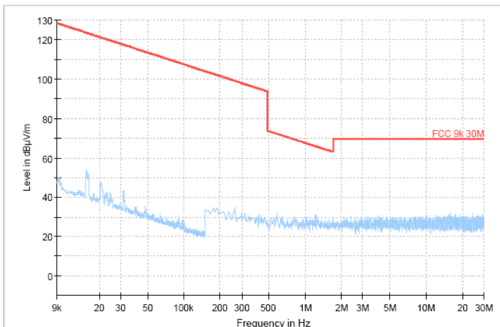
Fig. 57 Radiated Spurious Emission (All Channels, 9kHz ~ 30MHz)
