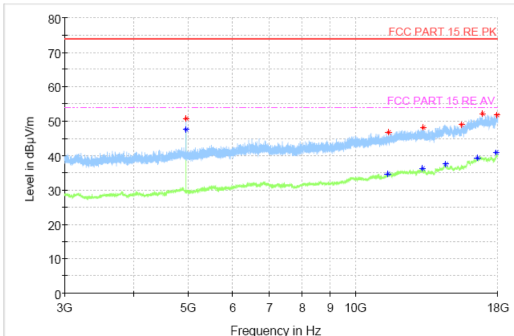
Fig. 44 Radiated Spurious Emission (GFSK, Ch78, 3GHz ~ 18GHz)
