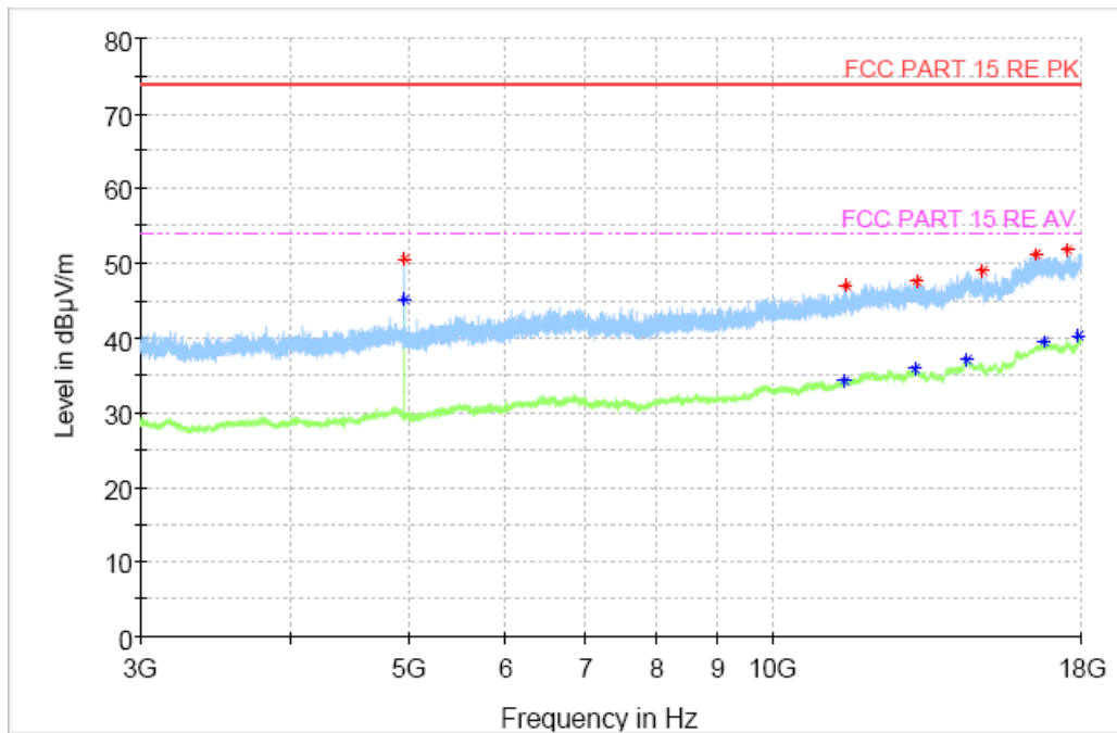
Fig. 54 Radiated Spurious Emission (8DPSK, Ch78, 3GHz ~ 18GHz)
