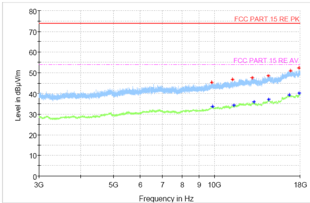
Fig.57 Radiated Spurious Emission (802.11n HT20, CH11, 3GHz-18GHz)
