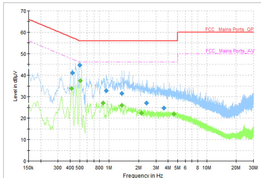
Fig.72 AC Power line Conducted Emission (Idle, AE3, 120V)
