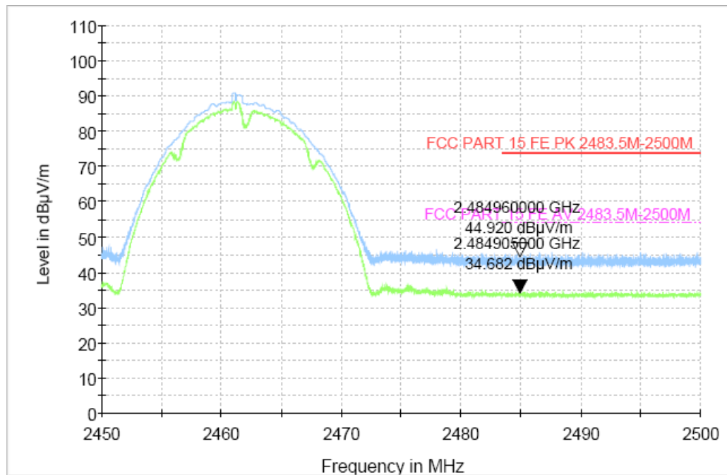
Fig.49 Radiated Restricted Band (802.11b, CH11, 2.45GHz~2.5GHz)
