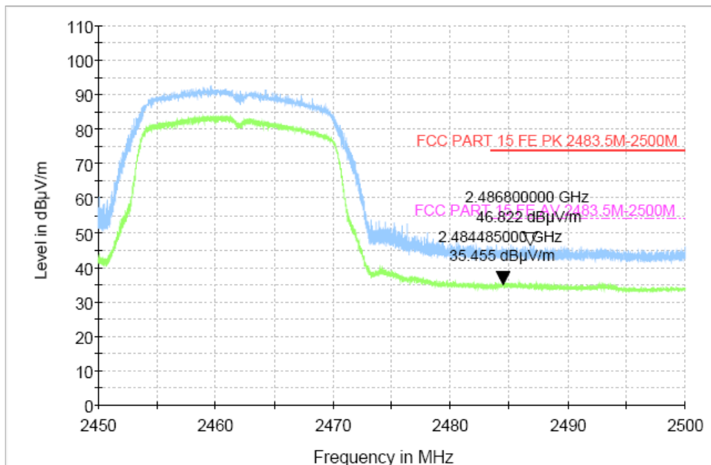
Fig.54 Radiated Restricted Band (802.11g, CH11, 2.45GHz~2.5GHz)
