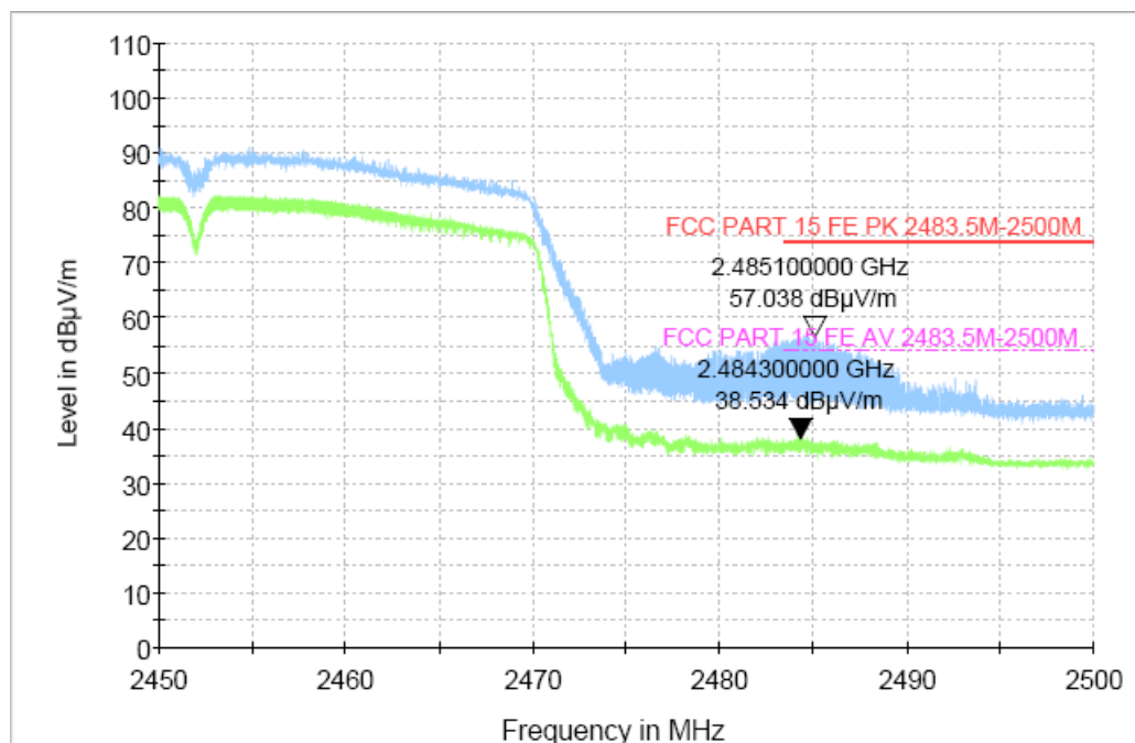
Fig.64 Radiated Restricted Band (802.11n HT40, CH9, 2.45GHz~2.5GHz)
