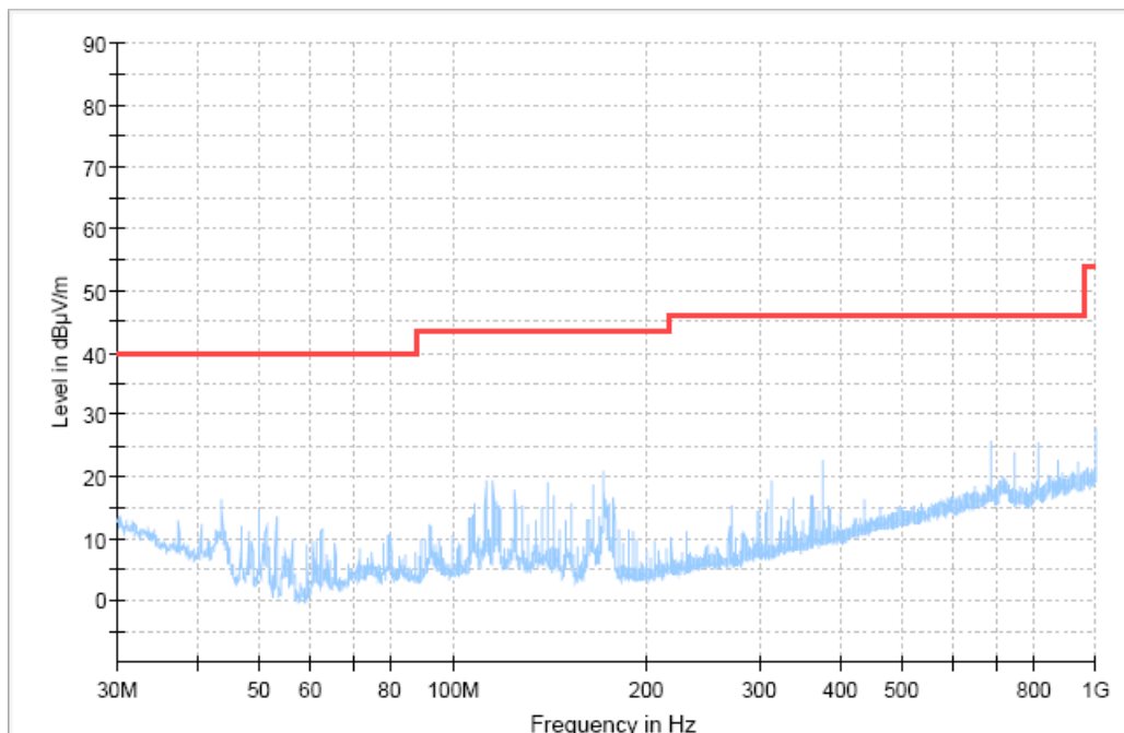
Fig.66 Radiated Spurious Emission (All Channels, 30MHz-1GHz)
