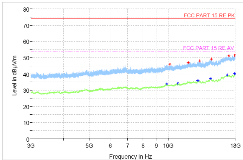
Fig.55 Radiated Spurious Emission (802.11n HT20, CH1, 3GHz-18GHz)
