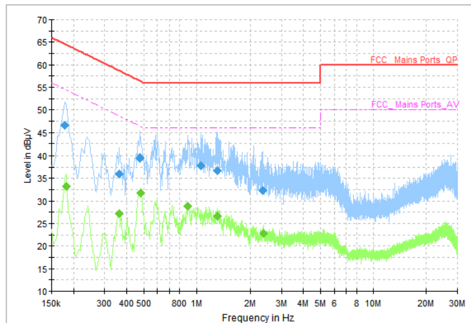
Fig.70 AC Power line Conducted Emission (Idle, AE2, 120V)
