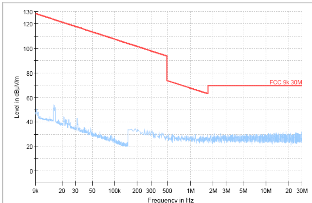
Fig.65 Radiated Spurious Emission (All Channels, 9KHz-30MHz)
