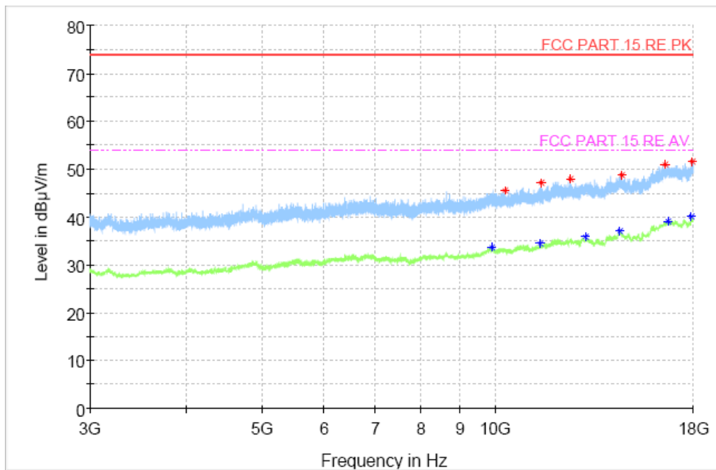
Fig.52 Radiated Spurious Emission (802.11g, CH11, 3GHz-18GHz)
