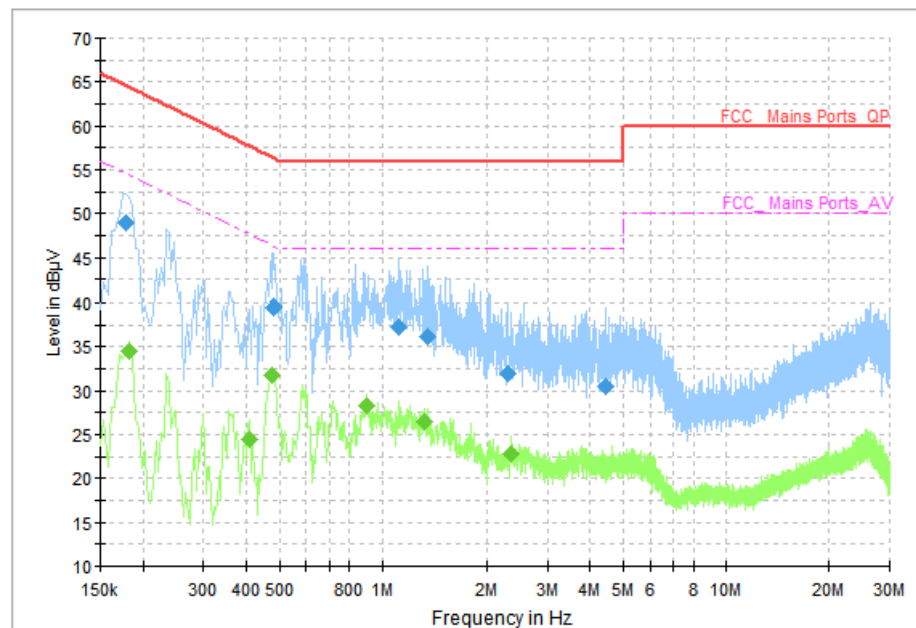
Fig.69 AC Power line Conducted Emission (Traffic, AE2, 120V)
