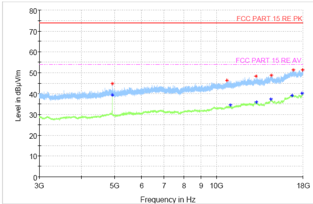
Fig.47 Radiated Spurious Emission (802.11b, CH11, 3GHz-18GHz)
