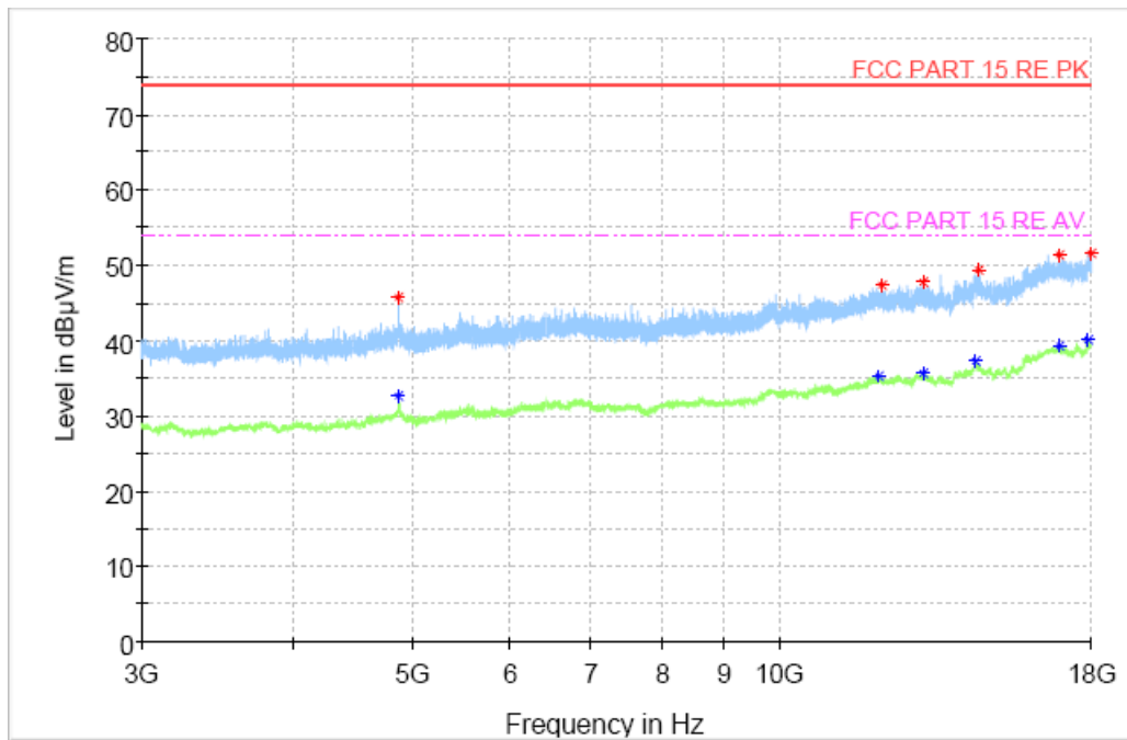
Fig.51 Radiated Spurious Emission (802.11g, CH6, 3GHz-18GHz)
