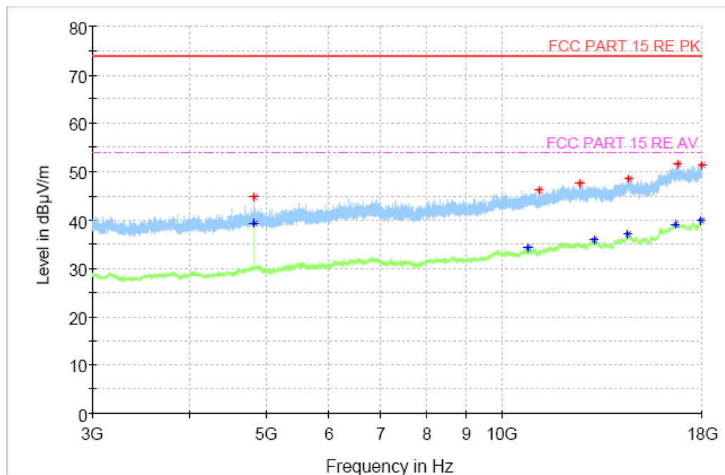
Fig.45 Radiated Spurious Emission (802.11b, CH1, 3GHz-18GHz)
