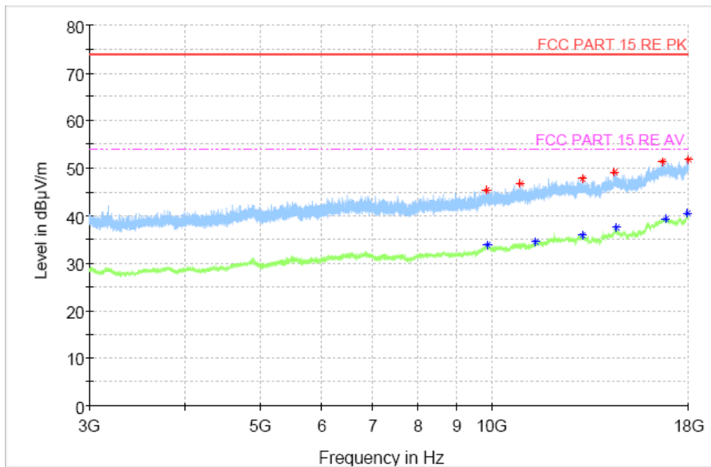
Fig.62 Radiated Spurious Emission (802.11n HT40, CH9, 3GHz-18GHz)
