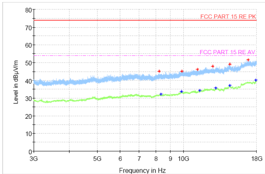
Fig.50 Radiated Spurious Emission (802.11g, CH1, 3GHz-18GHz)
