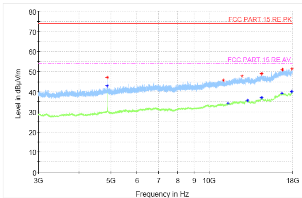
Fig.46 Radiated Spurious Emission (802.11b, CH6, 3GHz-18GHz)
