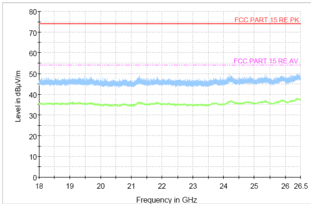
Fig.68 Radiated Spurious Emission (All Channels, 18GHz-26.5GHz)
