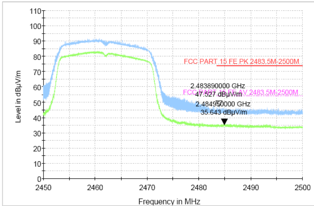
Fig.59 Radiated Restricted Band (802.11n HT20, CH11, 2.45GHz~2.5GHz)
