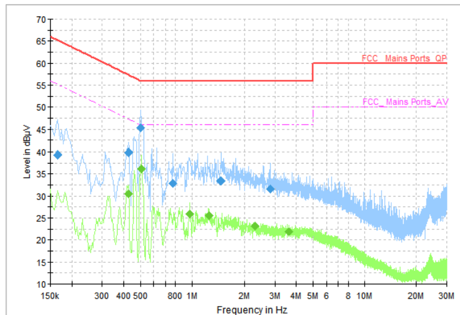
Fig.71 AC Power line Conducted Emission (Traffic, AE3, 120V)
