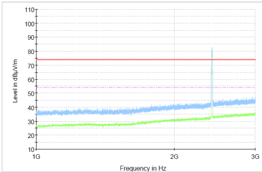
Fig.67 Radiated Spurious Emission (All Channels, 1GHz-3GHz)
