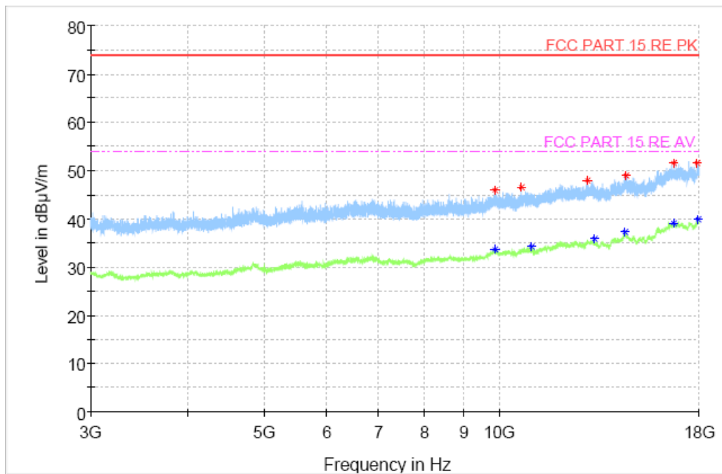
Fig.60 Radiated Spurious Emission (802.11n HT40, CH3, 3GHz-18GHz)
