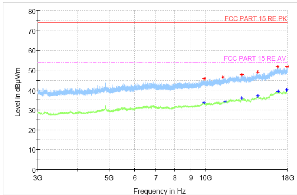
Fig.56 Radiated Spurious Emission (802.11n HT20, CH6, 3GHz-18GHz)
