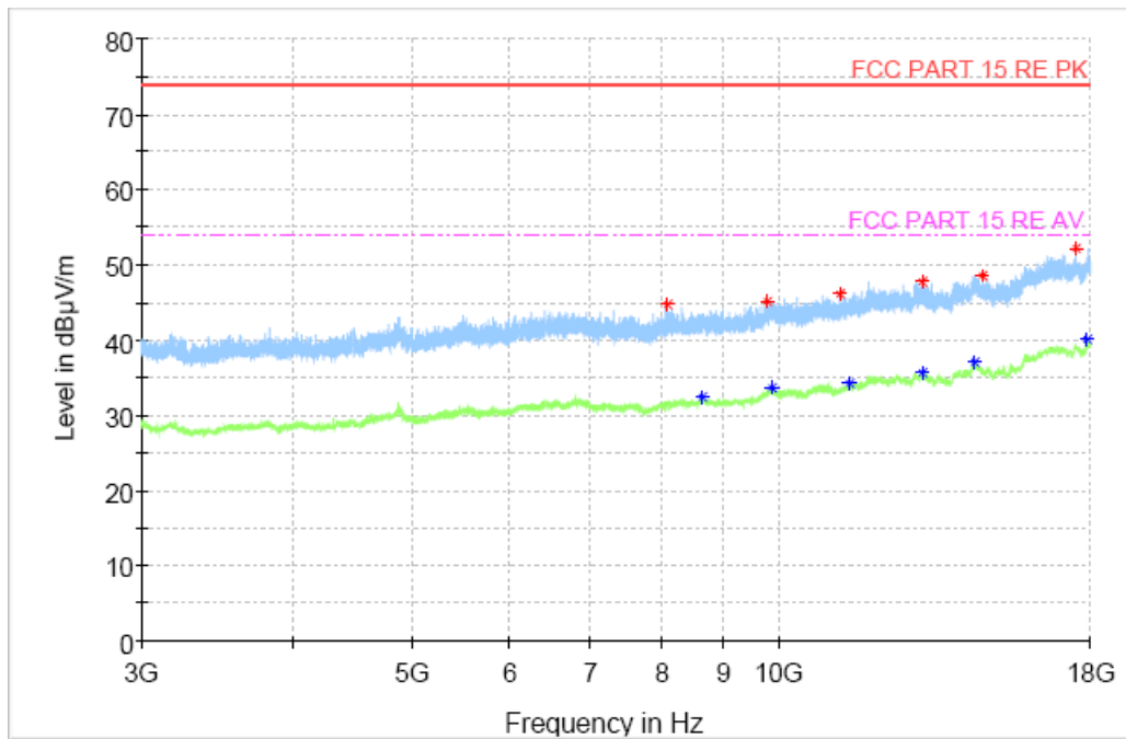
Fig.61 Radiated Spurious Emission (802.11n HT40, CH6, 3GHz-18GHz)
