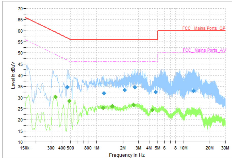
Fig. 84 AC Power line Conducted Emission (Traffic, AE3, 120V)
