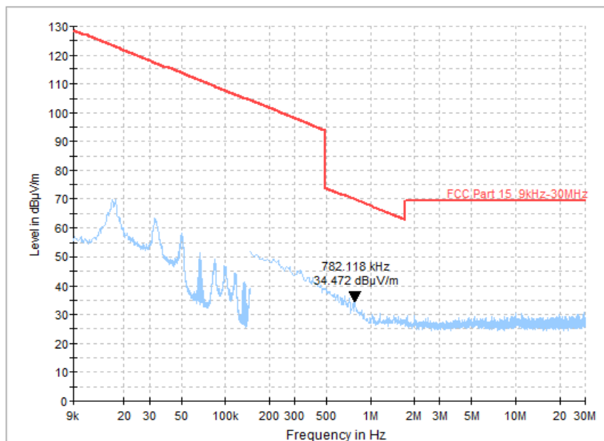
Fig. 57 Radiated Spurious Emission (All Channels, 9kHz ~ 30MHz)
