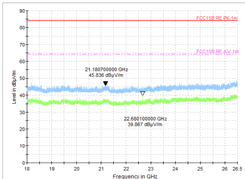
Fig. 59 Radiated Spurious Emission (All Channels, 18GHz ~ 26.5GHz)
