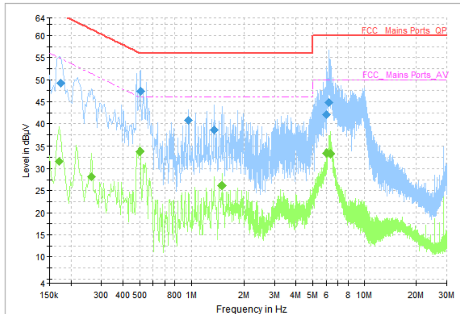
Fig. 86 AC Power line Conducted Emission (Traffic, AE4, 120V)
