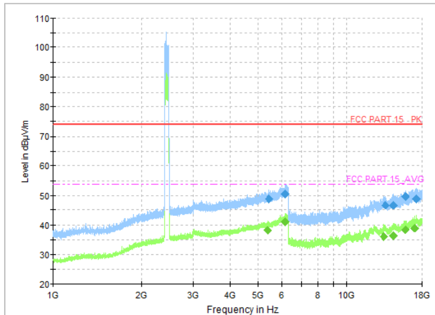
Fig.45 Radiated Spurious Emission (Ch0, 1 GHz - 18 GHz), 2M
