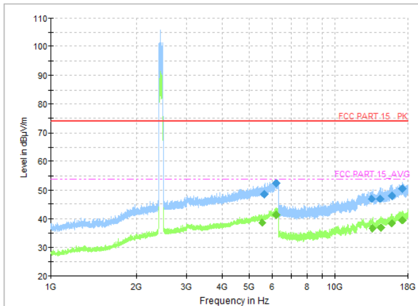
Fig.50 Radiated Spurious Emission (Ch39, 1 GHz - 18 GHz), 2M
