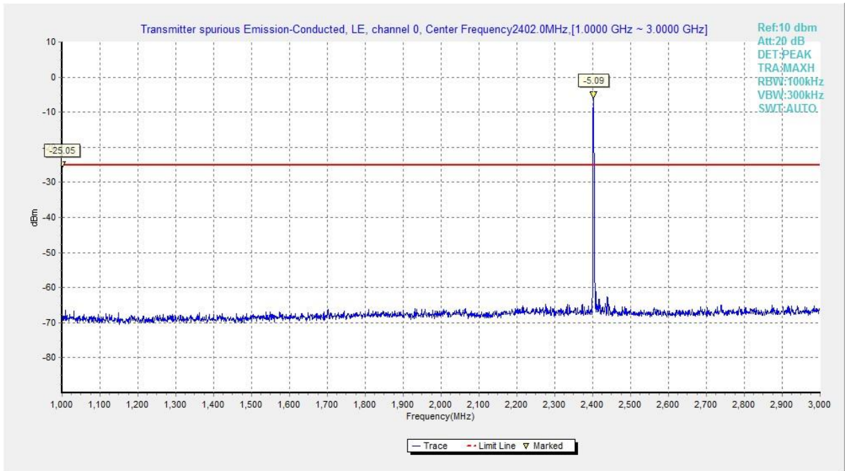
Fig.27 Conducted Spurious Emission (Ch0, 1 GHz-3 GHz), LE 2M
