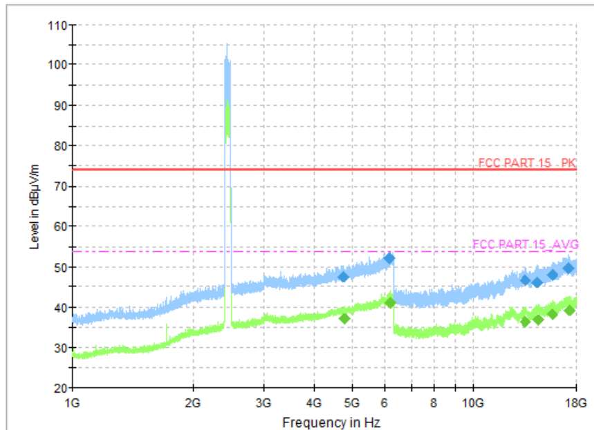
Fig.37 Radiated Spurious Emission (Ch0, 1 GHz - 18 GHz), 1M
