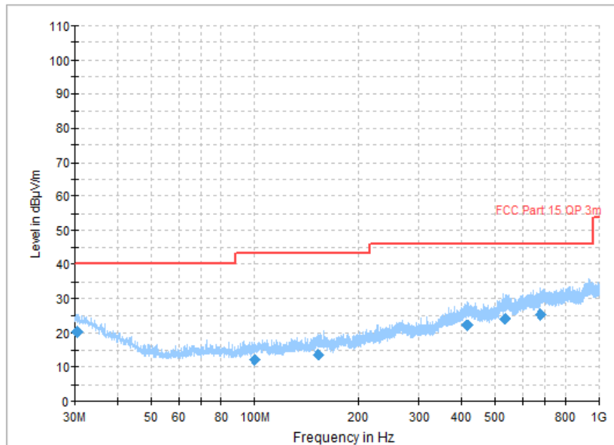
Fig.47 Radiated Spurious Emission (Ch19, 30 MHz - 1 GHz), 2M
