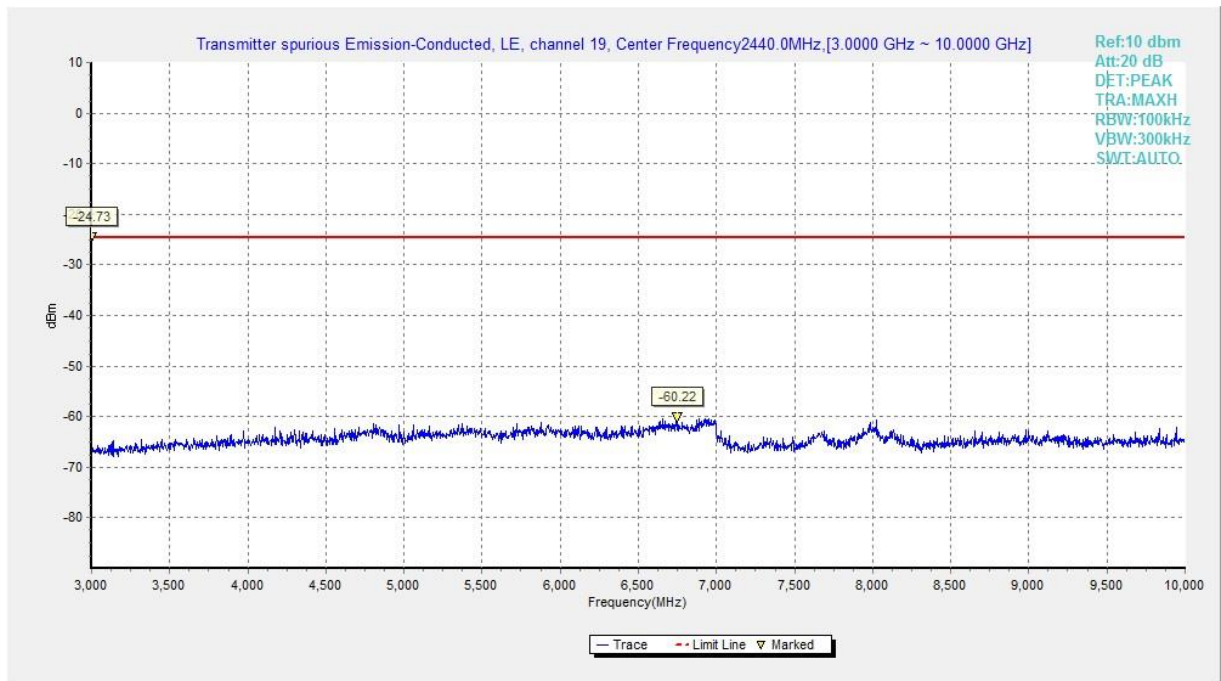
Fig.31 Conducted Spurious Emission (Ch19, 3 GHz-10 GHz), LE 2M
