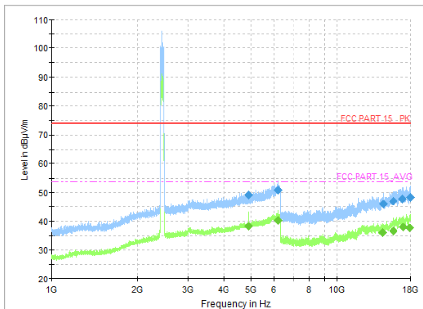
Fig.48 Radiated Spurious Emission (Ch19, 1 GHz - 18 GHz), 2M
