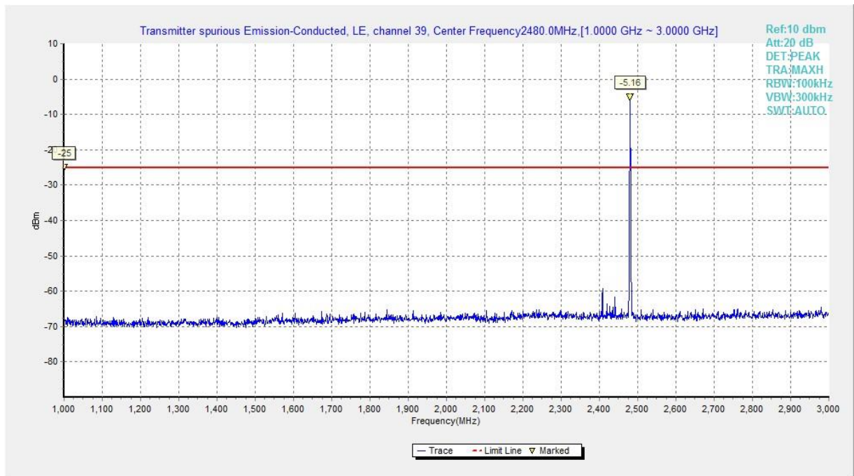
Fig.33 Conducted Spurious Emission (Ch39, 1 GHz-3 GHz), LE 2M
