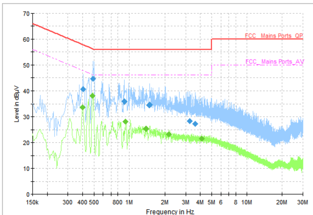
Fig.54 AC Power line Conducted Emission (Idle, AE2, 120V), 1M
