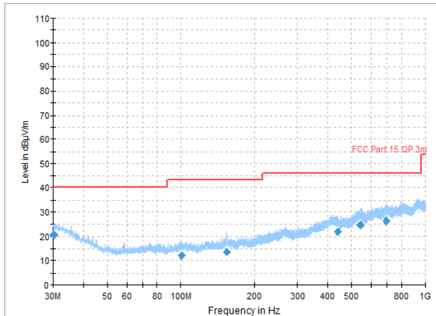
Fig.39 Radiated Spurious Emission (Ch19, 30 MHz - 1 GHz), 1M
