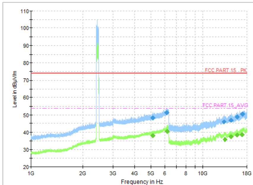
Fig.42 Radiated Spurious Emission (Ch39, 1 GHz - 18 GHz), 1M
