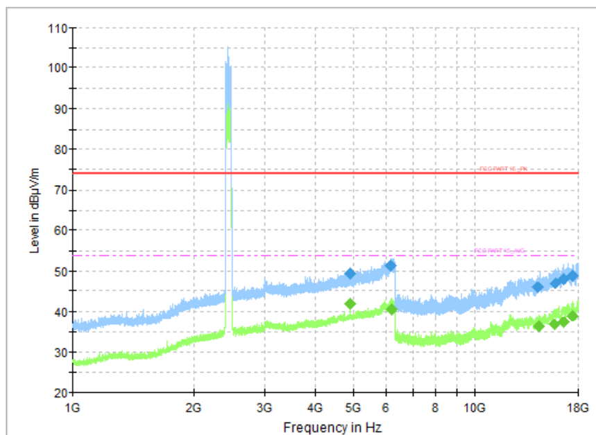
Fig.40 Radiated Spurious Emission (Ch19, 1 GHz - 18 GHz), 1M
