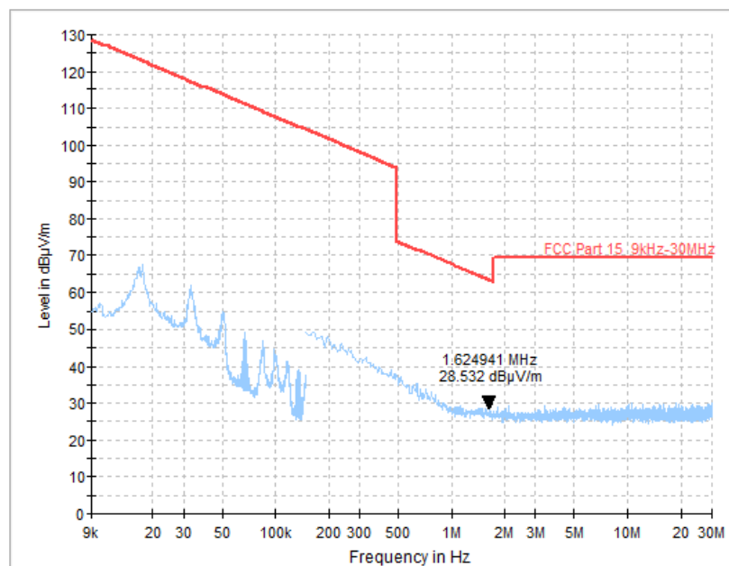
Fig.46 Radiated Spurious Emission (Ch19, 9 kHz - 30 MHz), 2M
