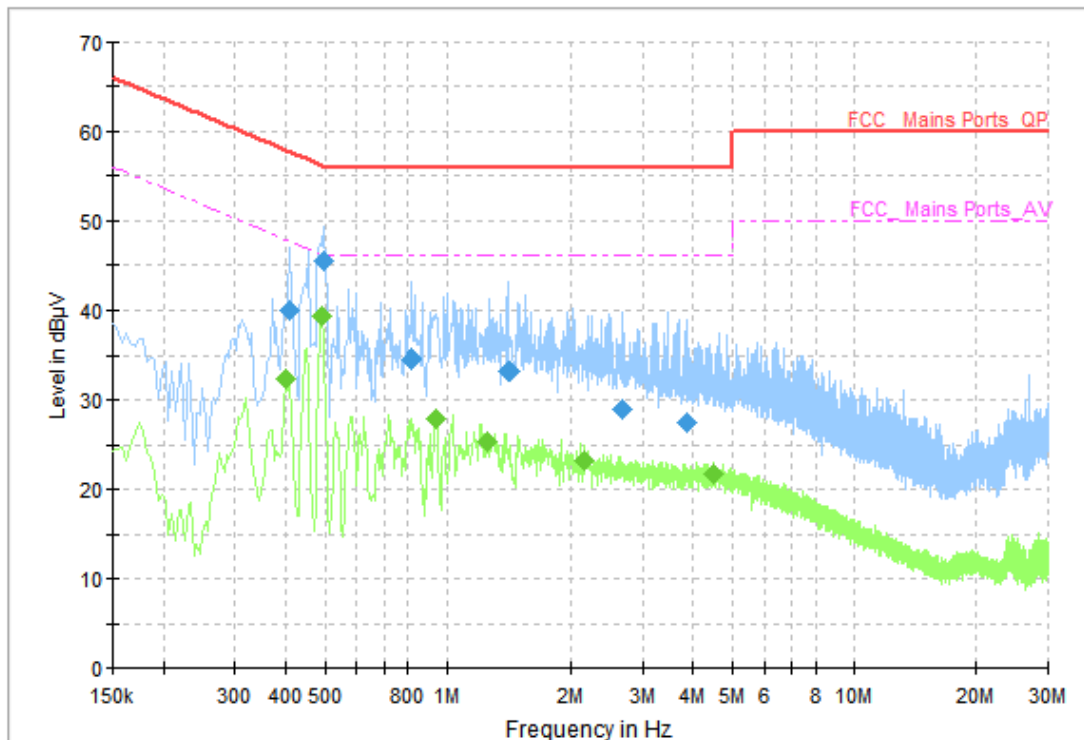
Fig.53 AC Power line Conducted Emission (Traffic, AE2, 120V), 1M
