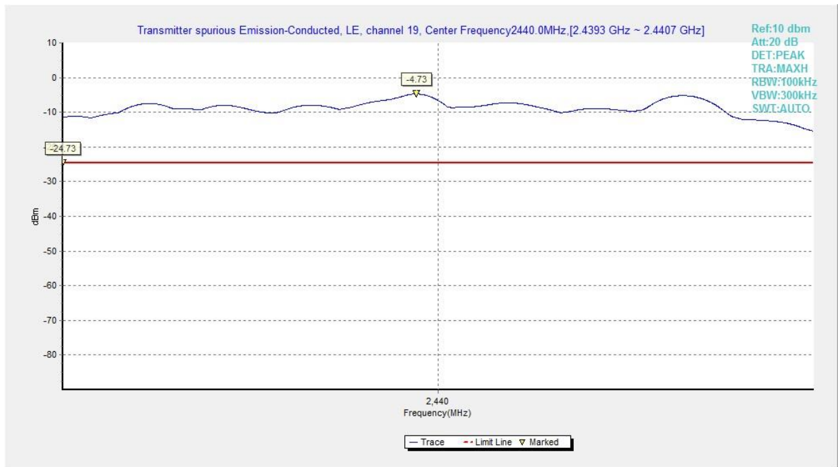
Fig.29 Conducted Spurious Emission (Ch19, Center Frequency), LE 2M
