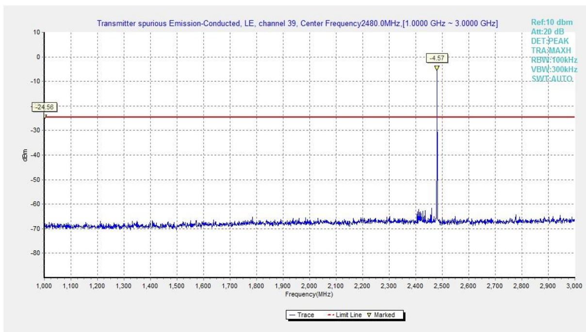
Fig.24 Conducted Spurious Emission (Ch39, 1 GHz-3 GHz), LE 1M
