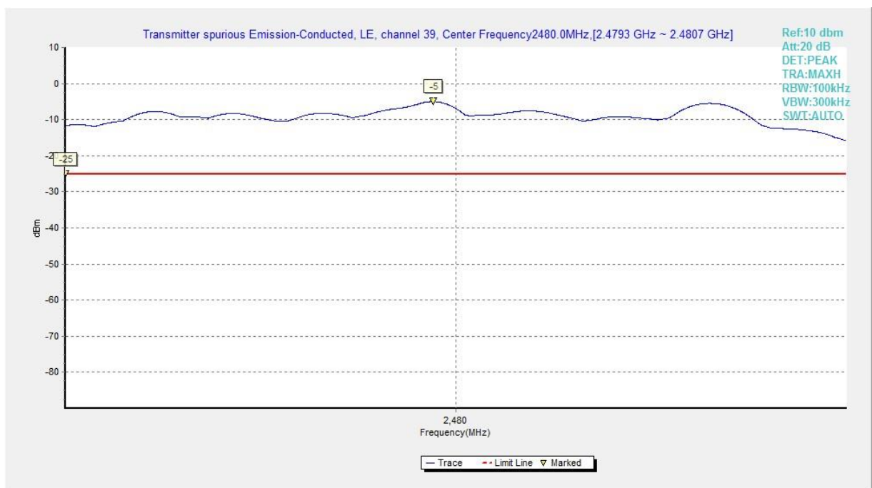
Fig.32 Conducted Spurious Emission (Ch39, Center Frequency), LE 2M
