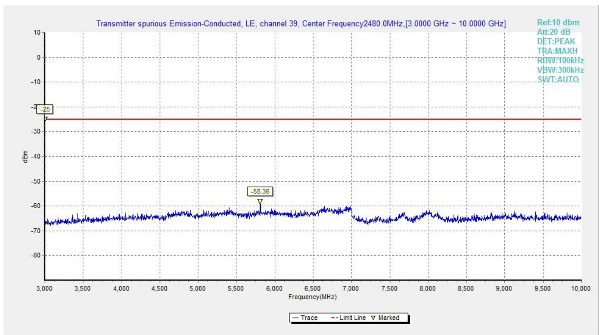
Fig.34 Conducted Spurious Emission (Ch39, 3 GHz-10 GHz), LE 2M
