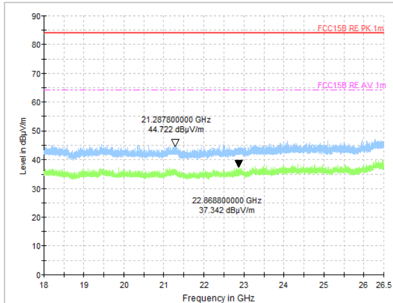
Fig.49 Radiated Spurious Emission (Ch19, 18 GHz - 26.5 GHz), 2M
