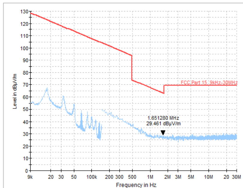
Fig.38 Radiated Spurious Emission (Ch19, 9 kHz - 30 MHz), 1M
