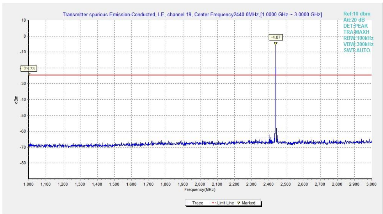
Fig.30 Conducted Spurious Emission (Ch19, 1 GHz-3 GHz), LE 2M
