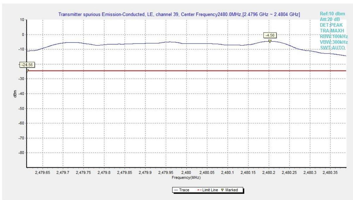
Fig.23 Conducted Spurious Emission (Ch39, Center Frequency), LE 1M
