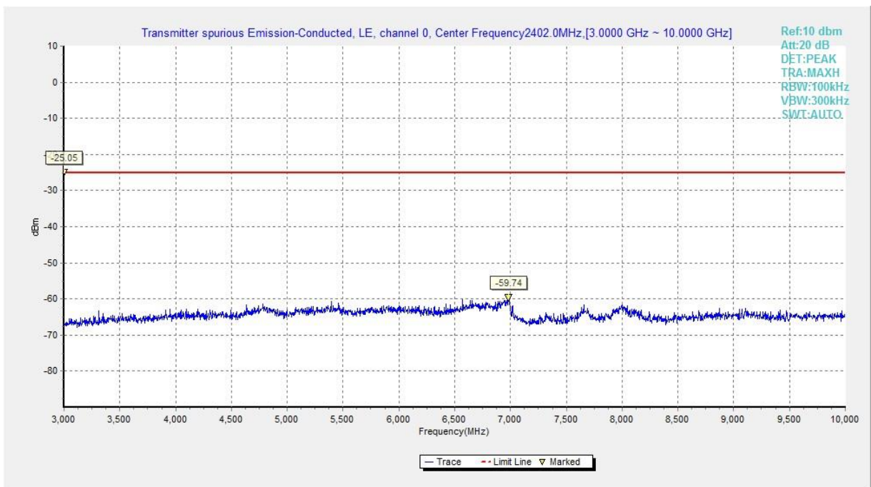
Fig.28 Conducted Spurious Emission (Ch0, 3 GHz-10 GHz), LE 2M
