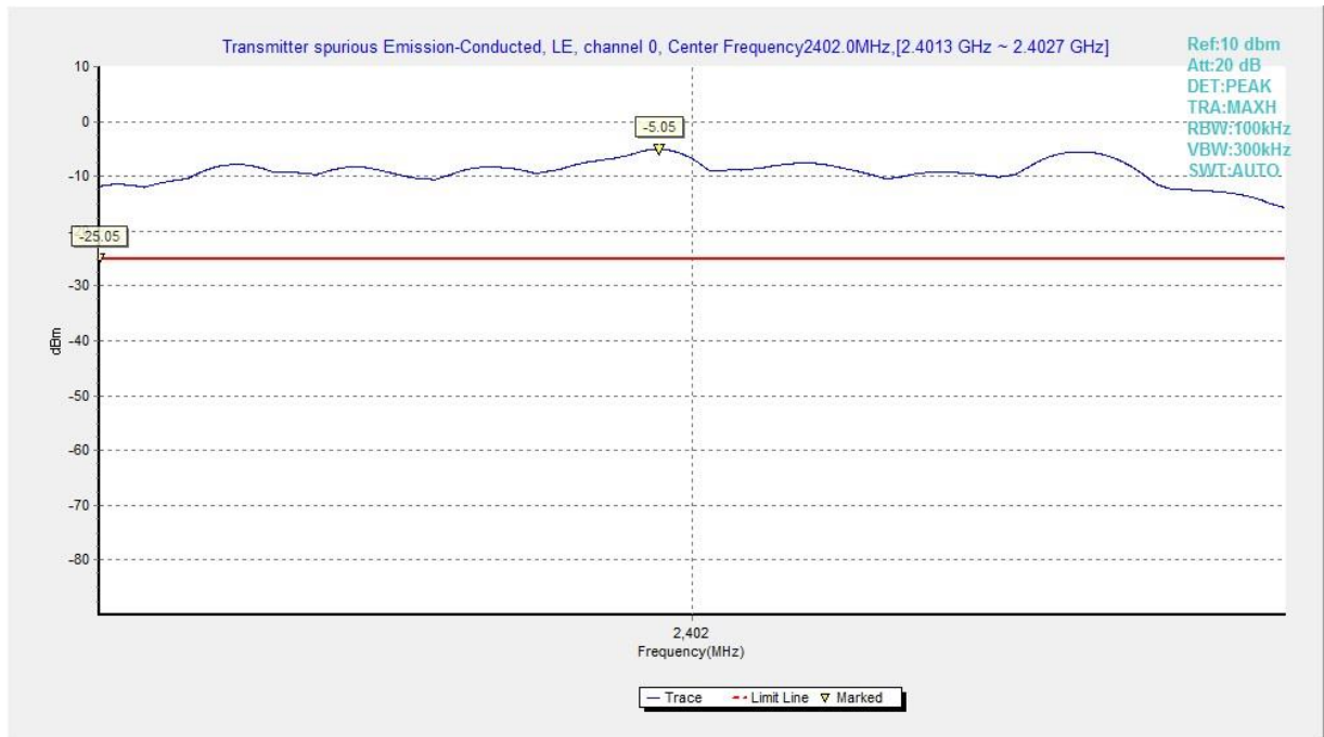
Fig.26 Conducted Spurious Emission (Ch0, Center Frequency), LE 2M
