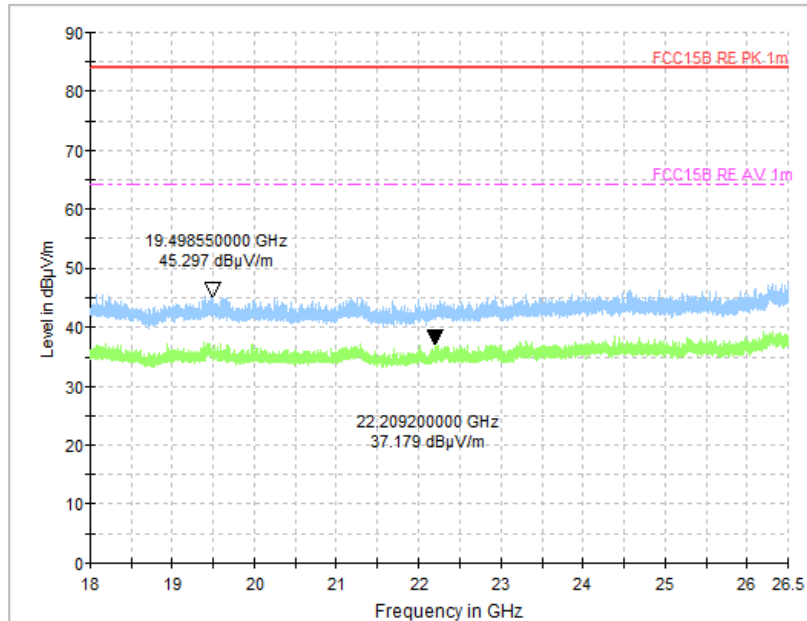
Fig.41 Radiated Spurious Emission (Ch19, 18 GHz - 26.5 GHz), 1M
