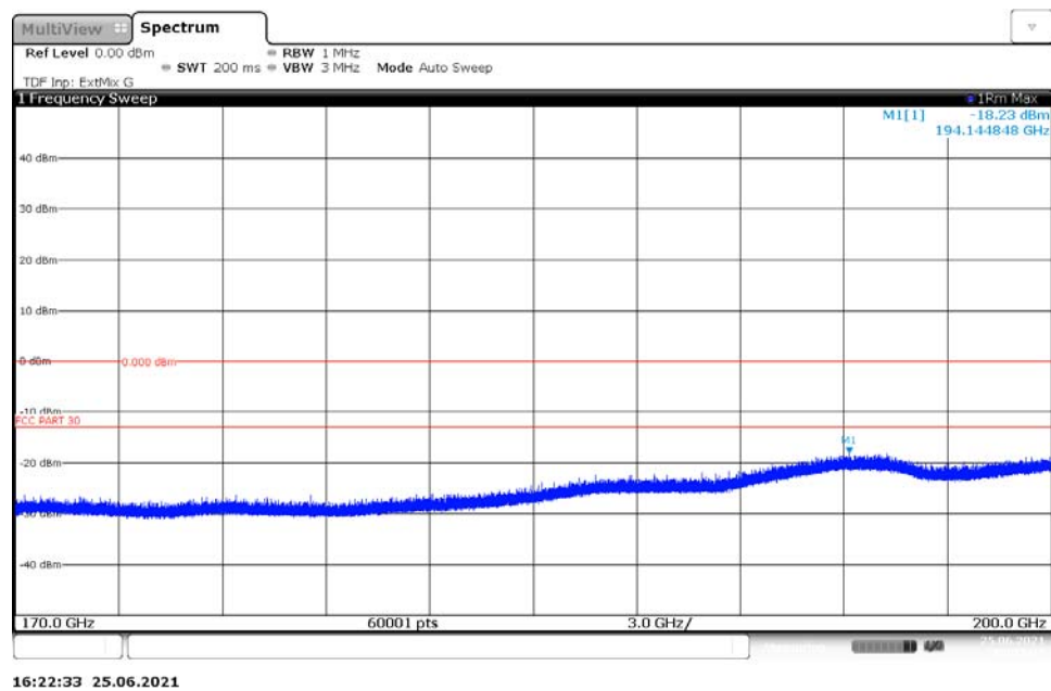
n260, Mid Channel, 170GHz-200GHz
