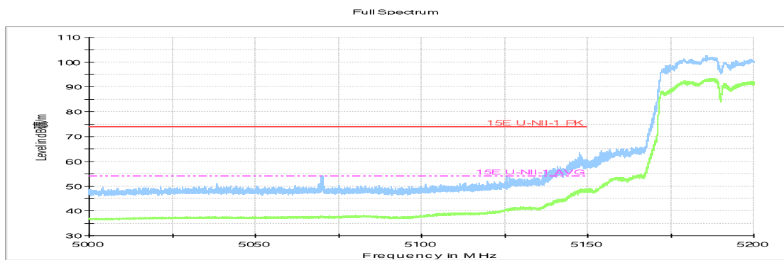
Fig.36 Band Edges (802.11n-HT40 Ch38, 5190MHz)
