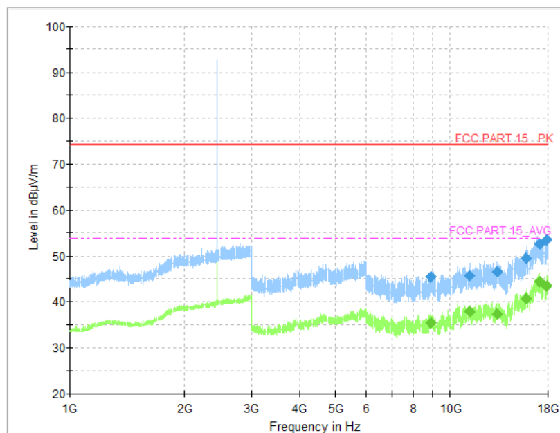
Fig.19 Radiated Spurious Emission (CH19, 1 GHz ~18 GHz), LE 1M
