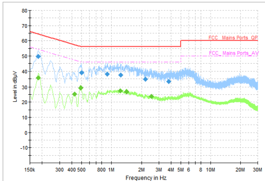
Fig.26 AC Power line Conducted Emission (Traffic), LE 1M
