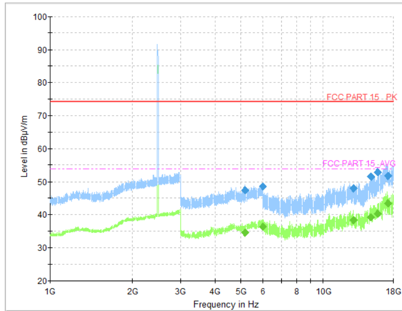
Fig.20 Radiated Spurious Emission (CH39, 1 GHz ~18 GHz), LE 1M
