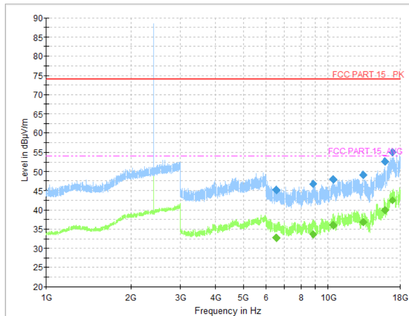
Fig.18 Radiated Spurious Emission (CH0, 1 GHz ~18 GHz), LE 1M
