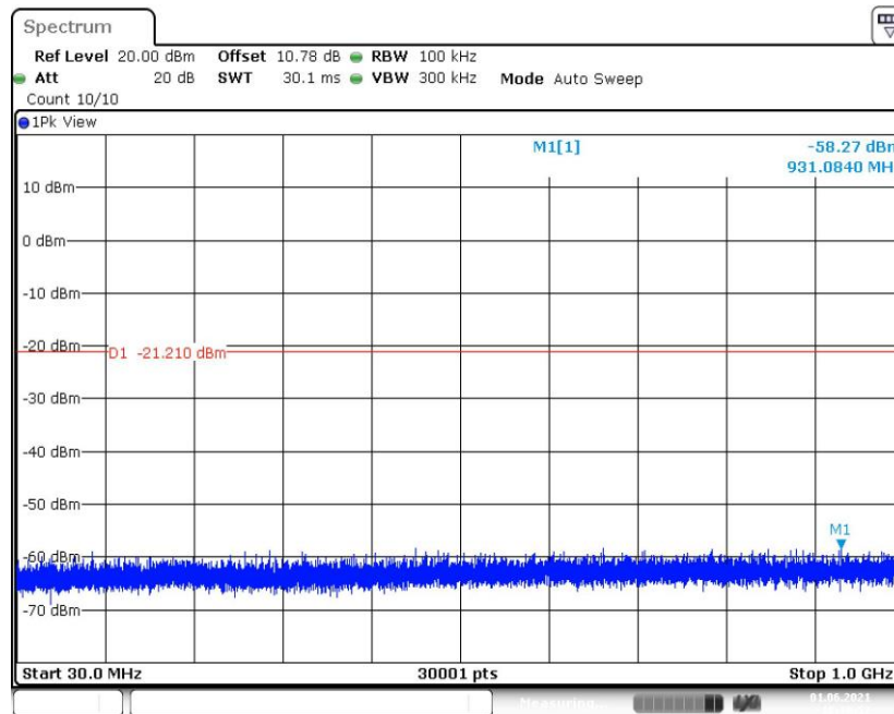
Fig.16 Conducted Spurious Emission (CH39, 30MHz -1GHz), LE 1M
