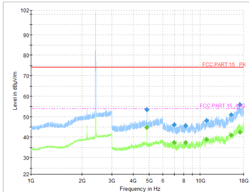
Fig.52 Radiated Spurious Emission (802.11b, CH1, 1 GHz-18GHz)
