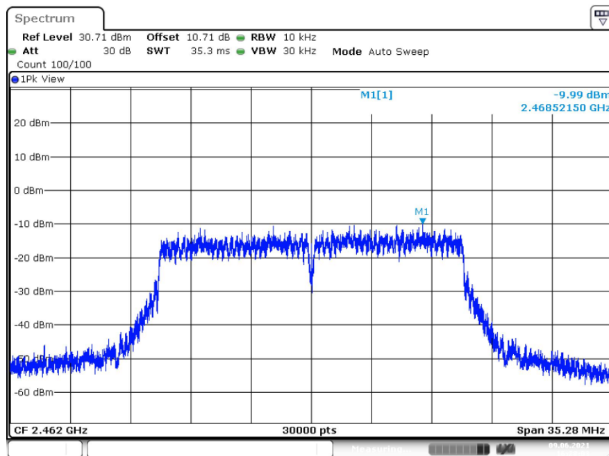
Fig.9 Power Spectral Density (802.11n-HT20, CH 11)
