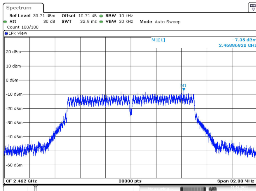
Fig.6 Power Spectral Density (802.11g, CH 11)
