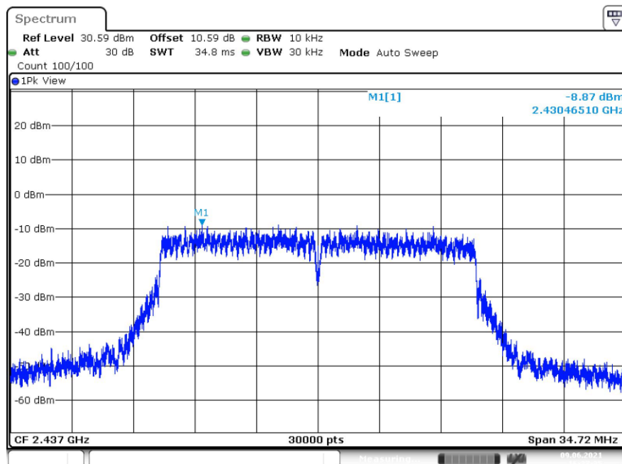
Fig.8 Power Spectral Density (802.11n-HT20, CH 6)
