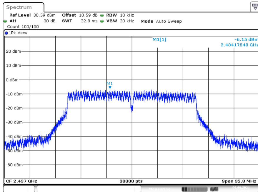
Fig.5 Power Spectral Density (802.11g, CH 6)
