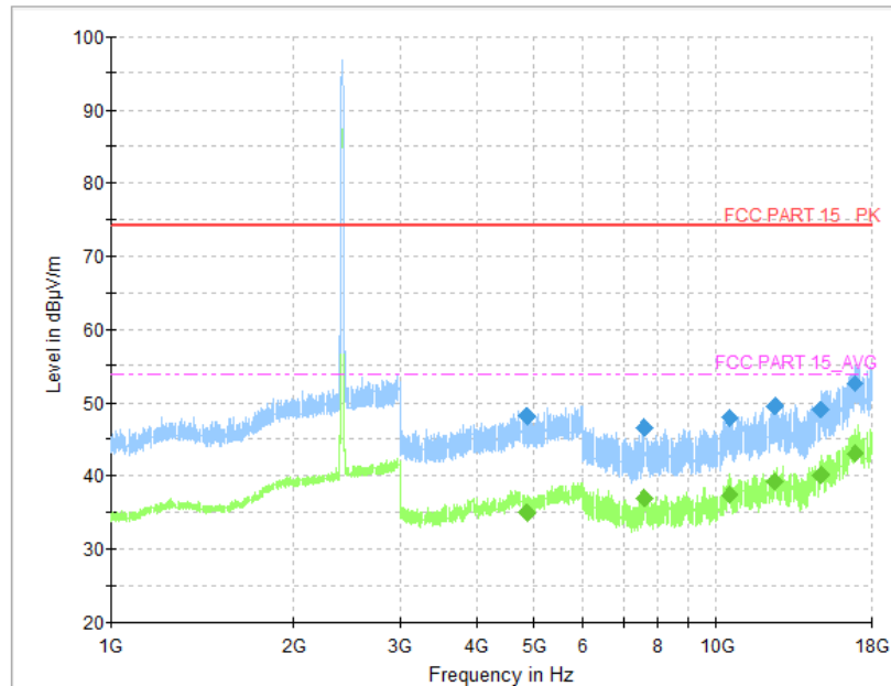
Fig.62 Radiated Spurious Emission (802.11n-HT20, CH1, 1 GHz-18 GHz)
