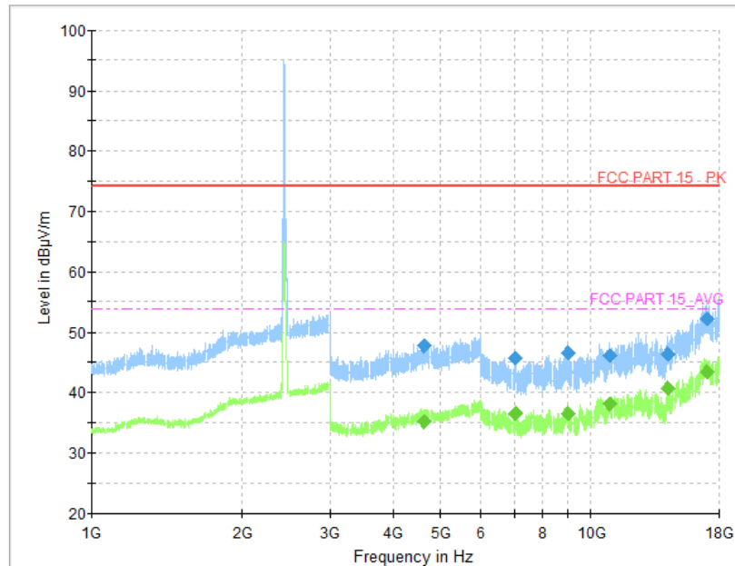
Fig.58 Radiated Spurious Emission (802.11g, CH6, 1 GHz-18 GHz)
