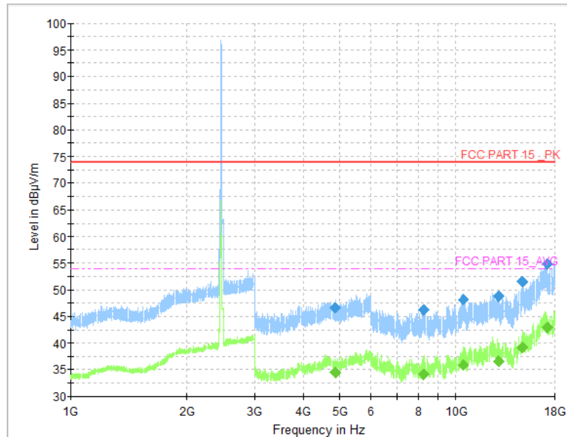
Fig.64 Radiated Spurious Emission (802.11n-HT20, CH11, 1 GHz-18 GHz)
