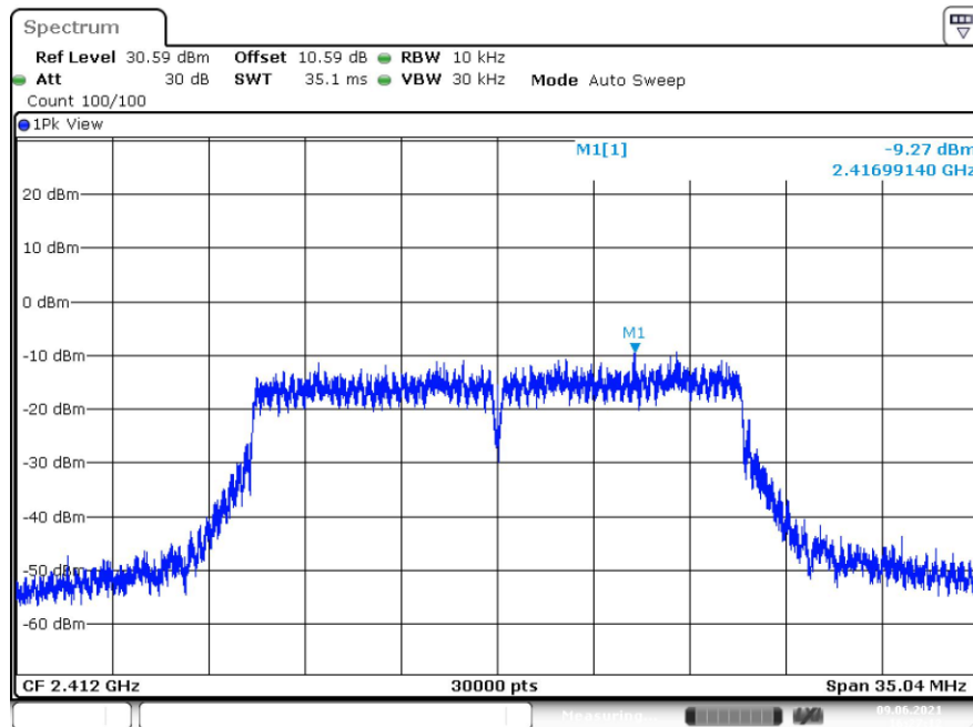
Fig.7 Power Spectral Density (802.11n-HT20, CH 1)
