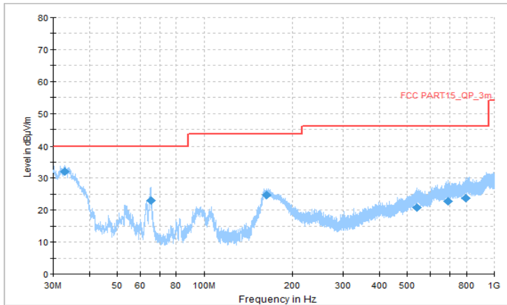
Figure A.1.1. Radiated Emission (GSM Receiver 850MHz, 30MHz to 1GHz) Final Result
