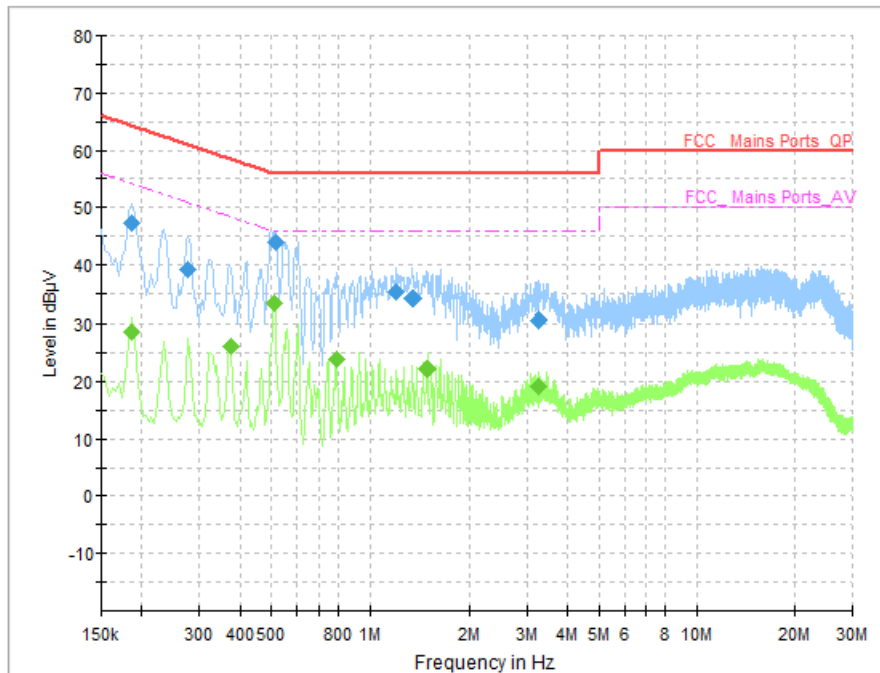
Fig. 73 AC Power line Conducted Emission (Idle)
