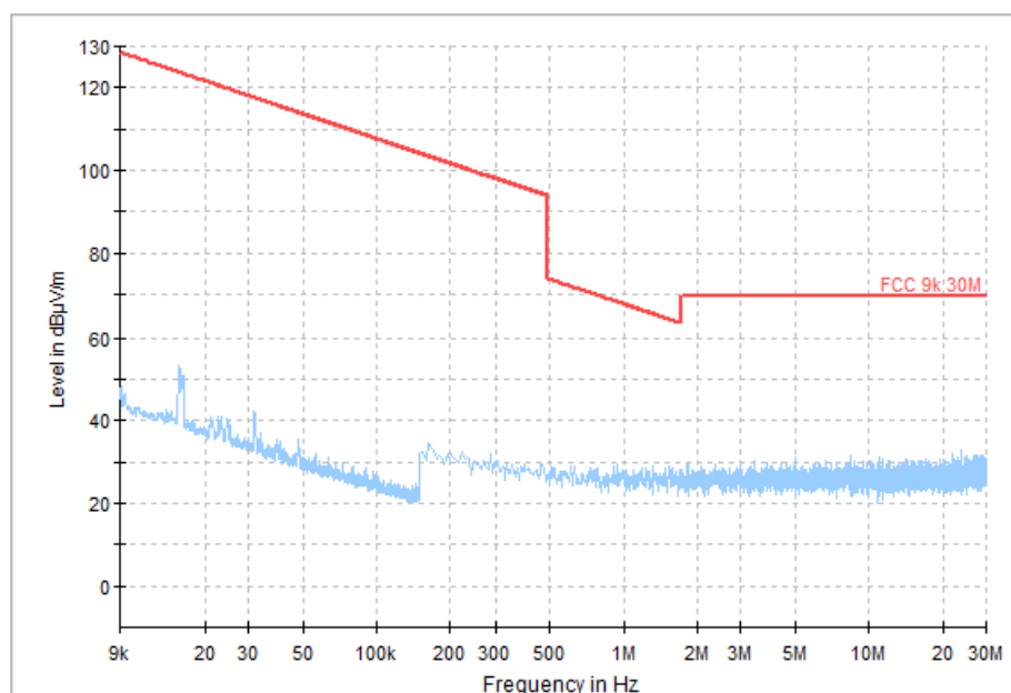
Fig. 71 Radiated Spurious Emission (All Channel, 9 kHz ~ 30 MHz)
