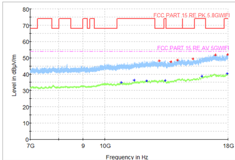
Fig. 54 Transmitter Spurious Emission (802. 11a, CH149 5745MHz)
