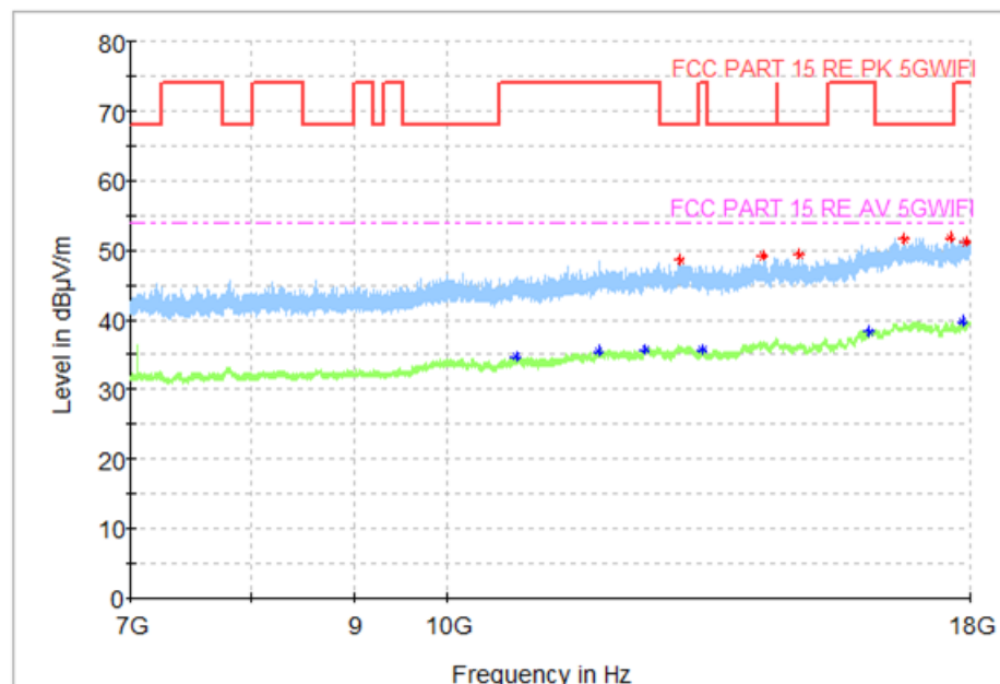
Fig. 64 Transmitter Spurious Emission (802. 11ac-VHT80, CH58 5290MHz)
