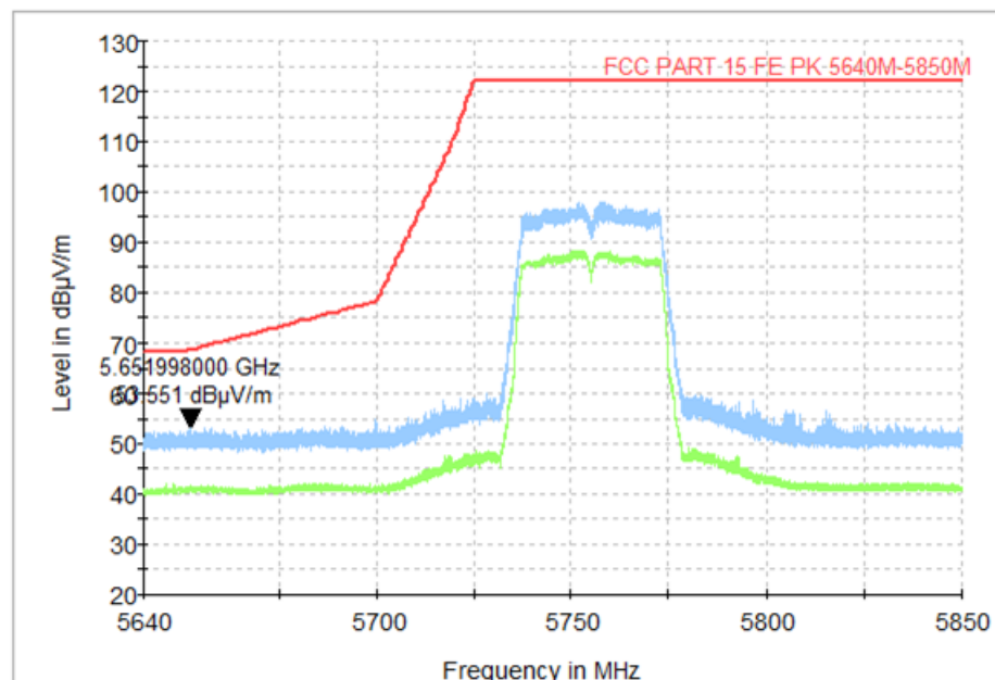
Fig. 43 Band Edges (802.11n-HT40, CH151 5755MHz)
