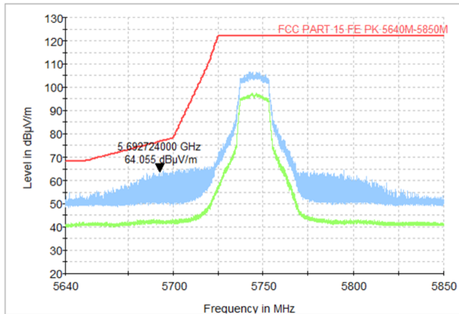
Fig. 39 Band Edges (802.11a, CH149 5745MHz)
