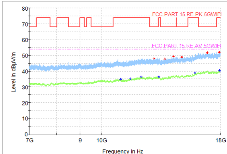
Fig. 50 Transmitter Spurious Emission (802.11a, CH48 5240MHz)
