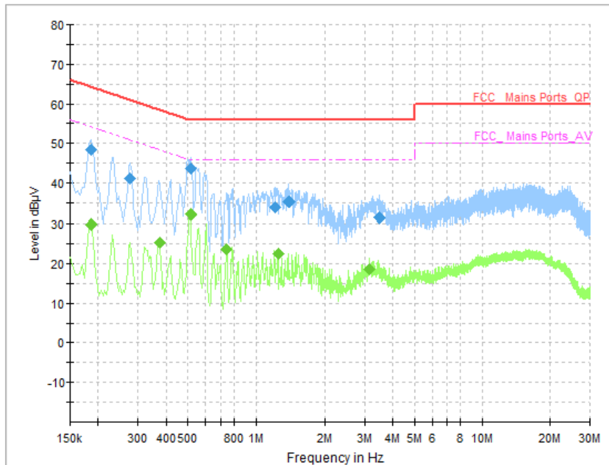
Fig. 72 AC Power line Conducted Emission (Traffic)
