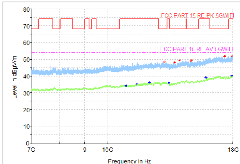
Fig. 58 Transmitter Spurious Emission (802.11n-HT40, CH46 5230MHz)
