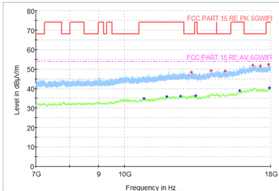
Fig. 48 Transmitter Spurious Emission (802.11a, CH36 5180MHz)
