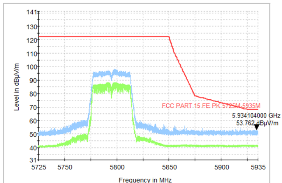
Fig. 44 Band Edges (802.11n-HT40, CH159 5795MHz)
