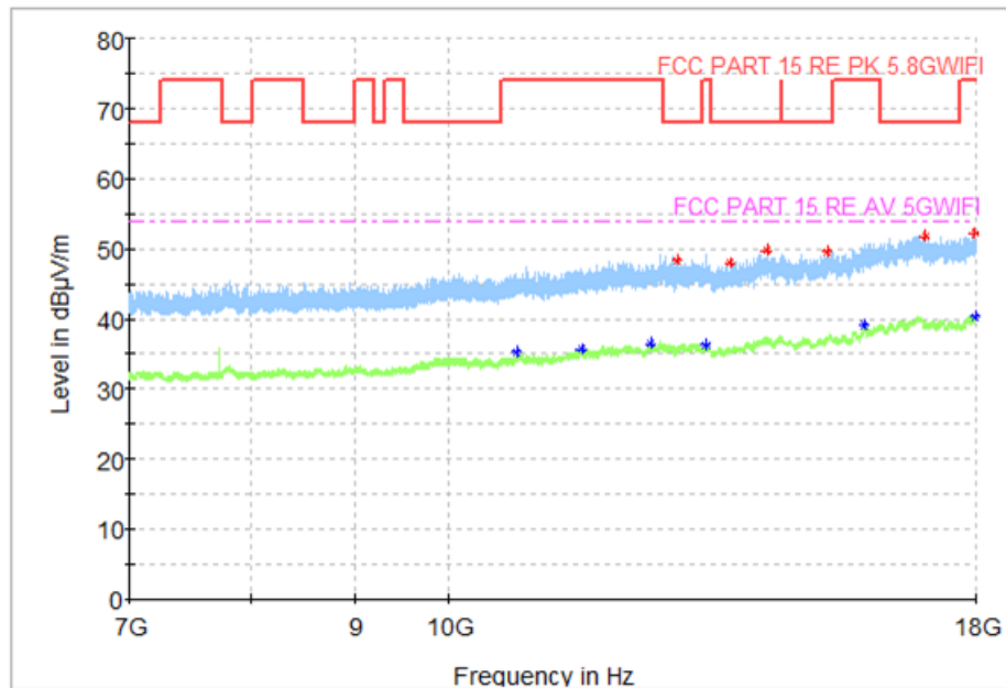
Fig. 62 Transmitter Spurious Emission (802. 11n-HT40, CH159 5795MHz)
