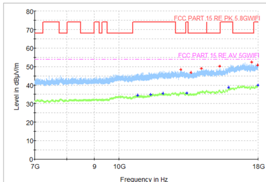
Fig. 56 Transmitter Spurious Emission (802. 11a, CH165 5825MHz)
