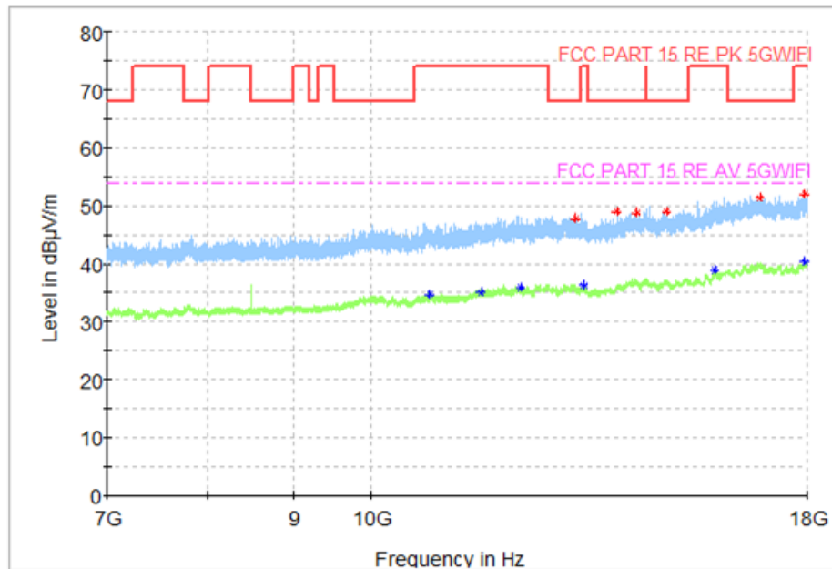
Fig. 60 Transmitter Spurious Emission (802.11n-HT40, CH62 5310MHz)
