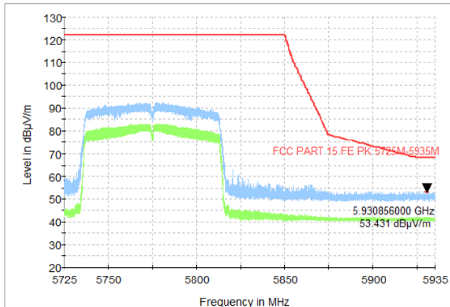
Fig. 47 Band Edges (802.11ac-VHT80, CH155 5775MHz)
