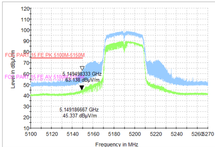
Fig. 41 Band Edges (802.11n-HT40, CH38 5190MHz)
