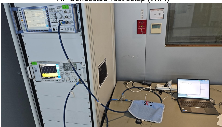
RF Conducted Test setup (WCDMA/LTE)
