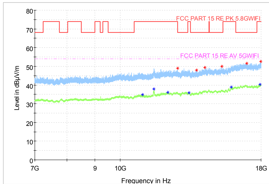
Fig. 61 Transmitter Spurious Emission (802. 11ac-VHT40, CH151 5755MHz)
