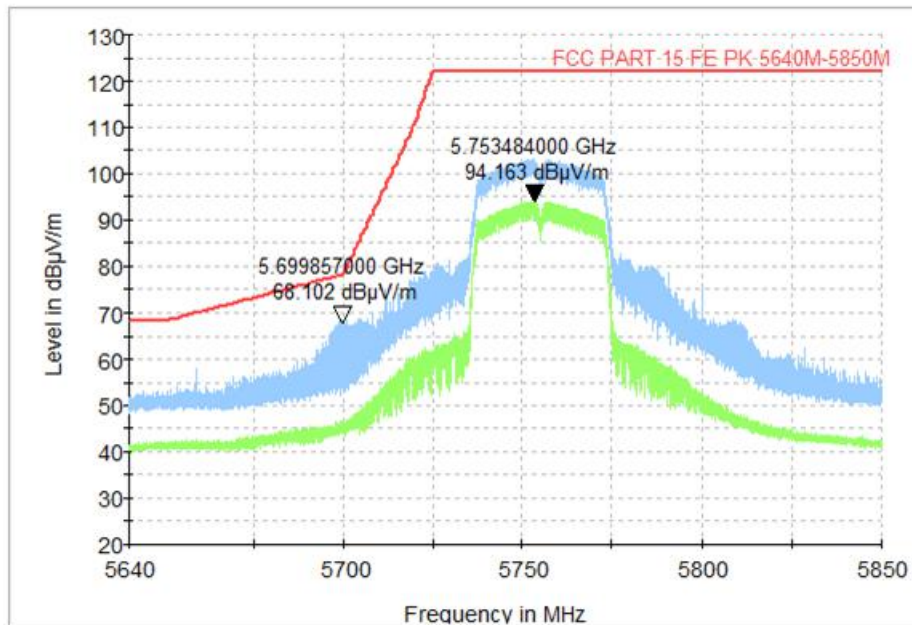
Fig. 43 Band Edges (802.11ac-VHT40, CH151 5755MHz)
