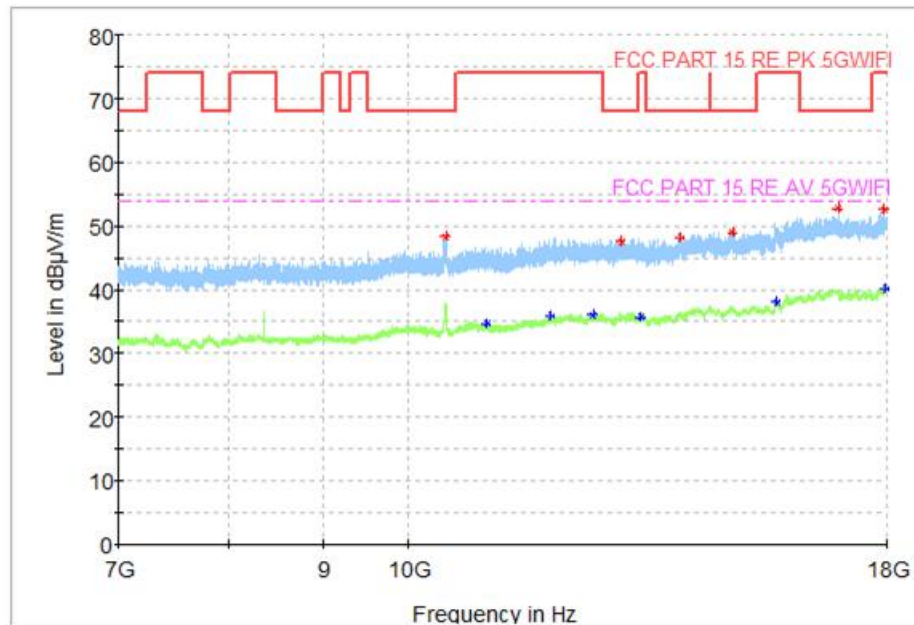
Fig. 58 Transmitter Spurious Emission (802.11ac-VHT40, CH46 5230MHz)
