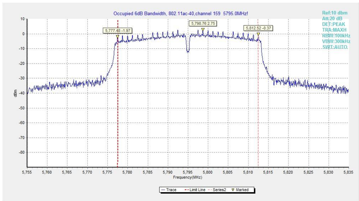
Fig. 17 Occupied 6dB Bandwidth (802.11ac-VHT40, 5795MHz)
