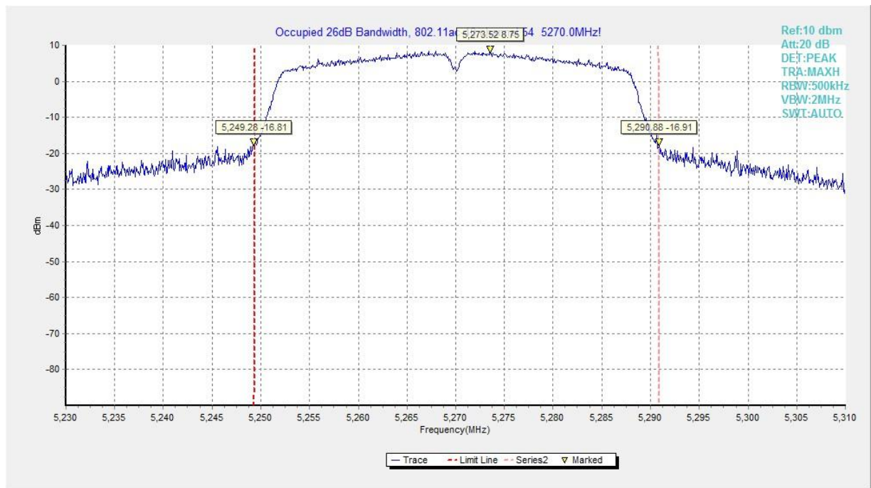
Fig. 9 Occupied 26dB Bandwidth (802. 11ac-VHT40, 5270MHz)
