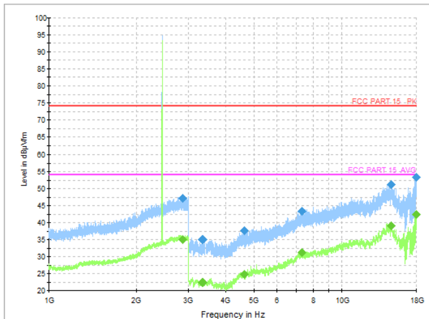
Fig. 39 Radiated Spurious Emission ( \pi/4 DQPSK, Ch39, 1GHz ~ 18GHz)
