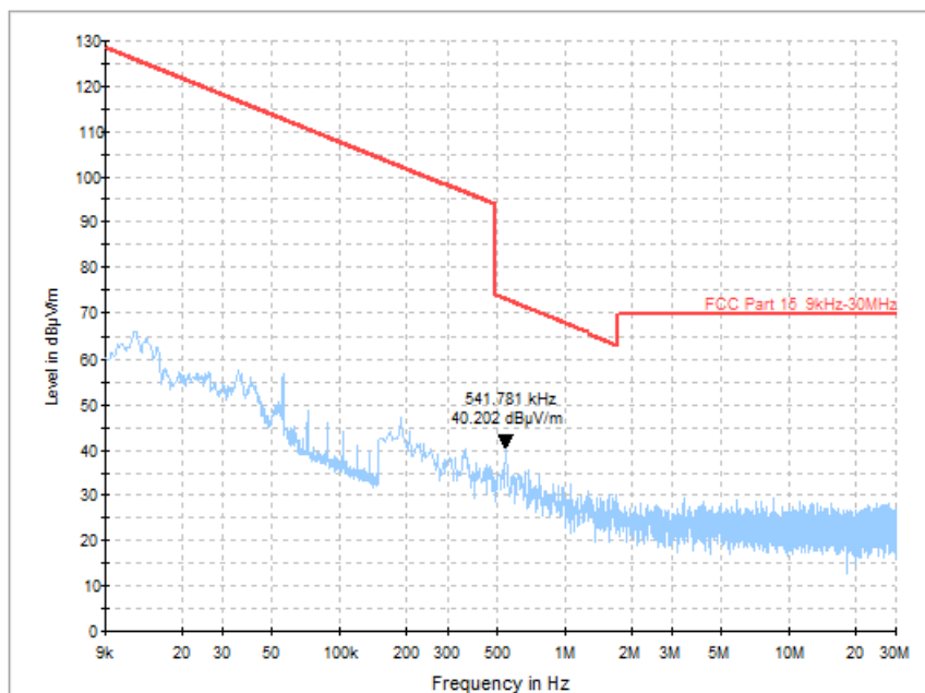
Fig. 48 Radiated Spurious Emission (All Channels, 9kHz ~ 30MHz)
