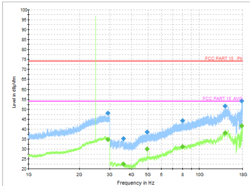
Fig. 35 Radiated Spurious Emission (GFSK, Ch78, 1GHz ~ 18GHz)
