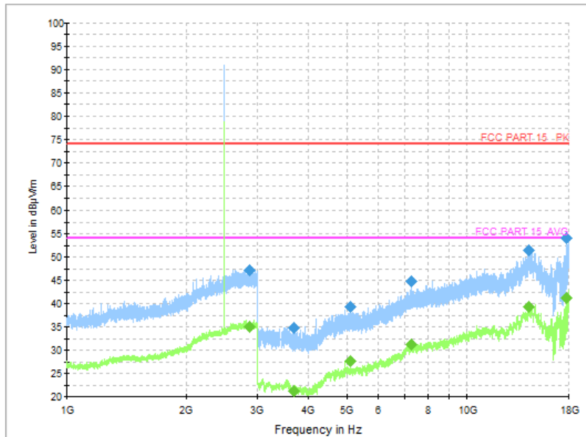
Fig. 45 Radiated Spurious Emission (8DPSK, Ch78, 1GHz ~ 18GHz)
