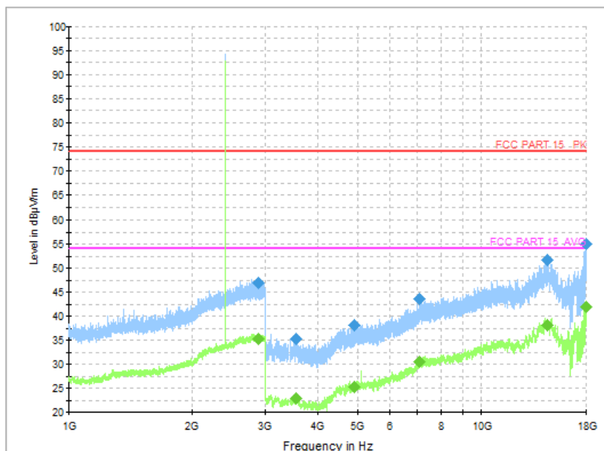
Fig. 38 Radiated Spurious Emission ( \pi/4 DQPSK, Ch0, 1GHz ~ 18GHz)
