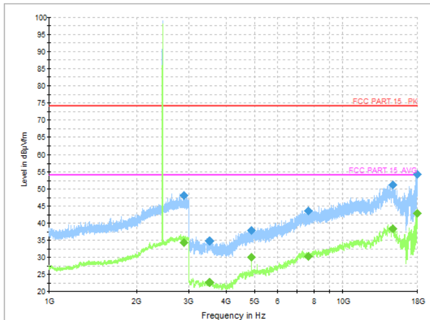
Fig. 34 Radiated Spurious Emission (GFSK, Ch39, 1GHz ~ 18GHz)
