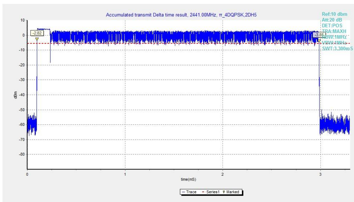
Fig. 62 Time of Occupancy (Dwell Time) ( \pi /4 DQPSK, Ch39)
