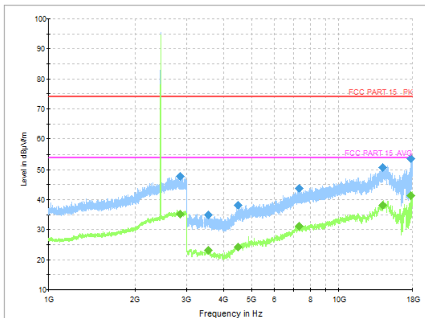
Fig. 44 Radiated Spurious Emission (8DPSK, Ch39, 1GHz ~ 18GHz)
