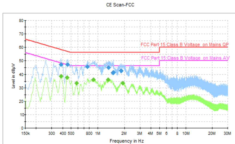
Fig. 75 AC Powerline Conducted Emission (Traffic, AE2, 120V)
