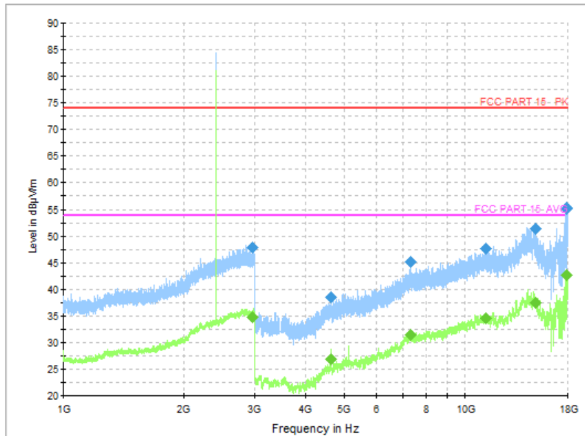
Fig. 33 Radiated Spurious Emission (GFSK, Ch0, 1GHz ~ 18GHz)
