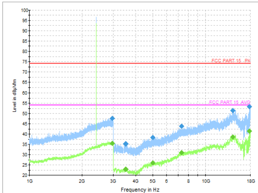
Fig. 43 Radiated Spurious Emission (8DPSK, Ch0, 1GHz ~ 18GHz)
