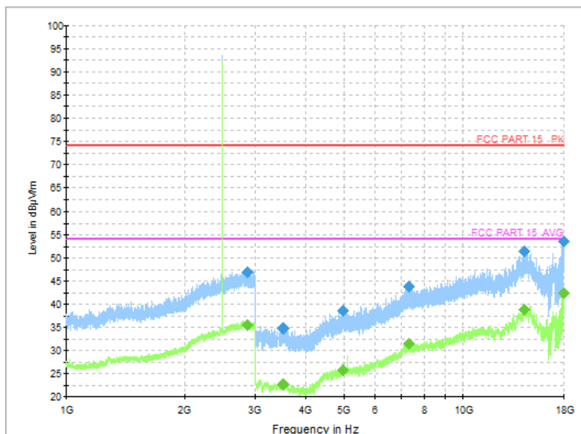
Fig. 40 Radiated Spurious Emission ( \pi/4 DQPSK, Ch78, 1GHz ~ 18GHz)
