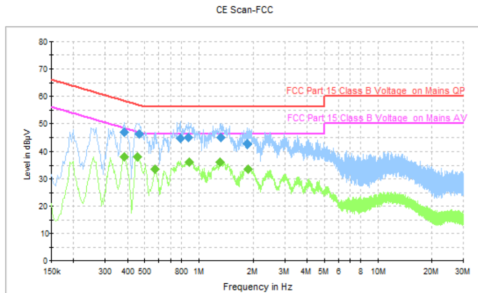
Fig. 76 AC Power line Conducted Emission (Idle, AE2, 120V)
