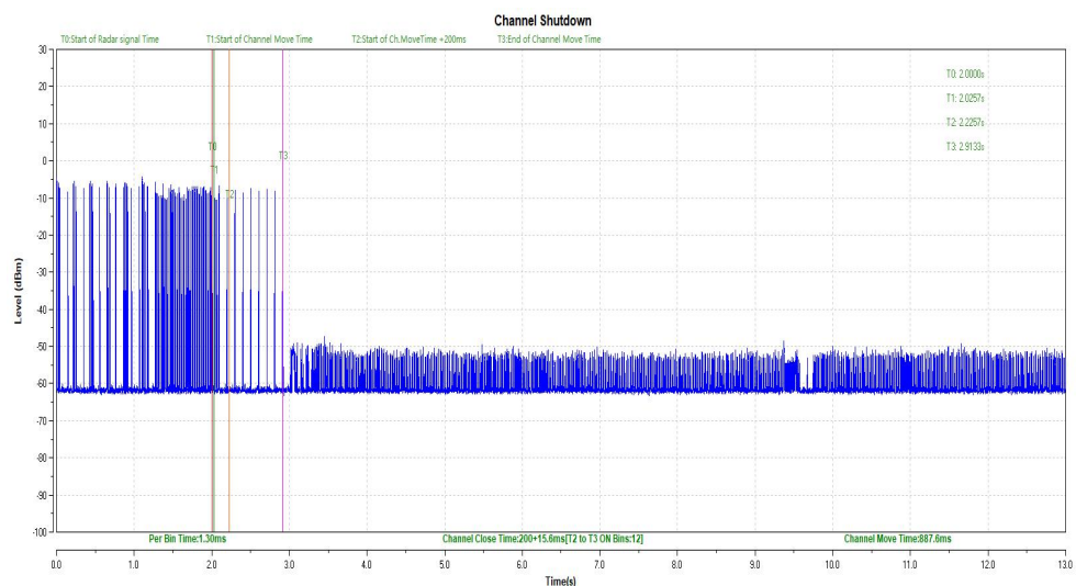
Fig.2 Channel Move Time & Channel Closing Transmission Time (HT80 Frequency Band: 5250MHz ~ 5350MHz)
