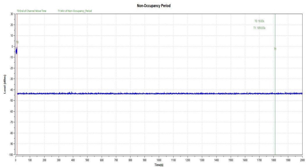
Fig.4 Non-Occupancy Period (HT80 Frequency Band: 5250MHz ~ 5350MHz)
