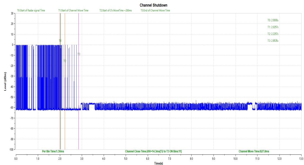
Fig.1 Channel Move Time & Channel Closing Transmission Time (HT20 Frequency Band: 5250MHz ~ 5350MHz)
