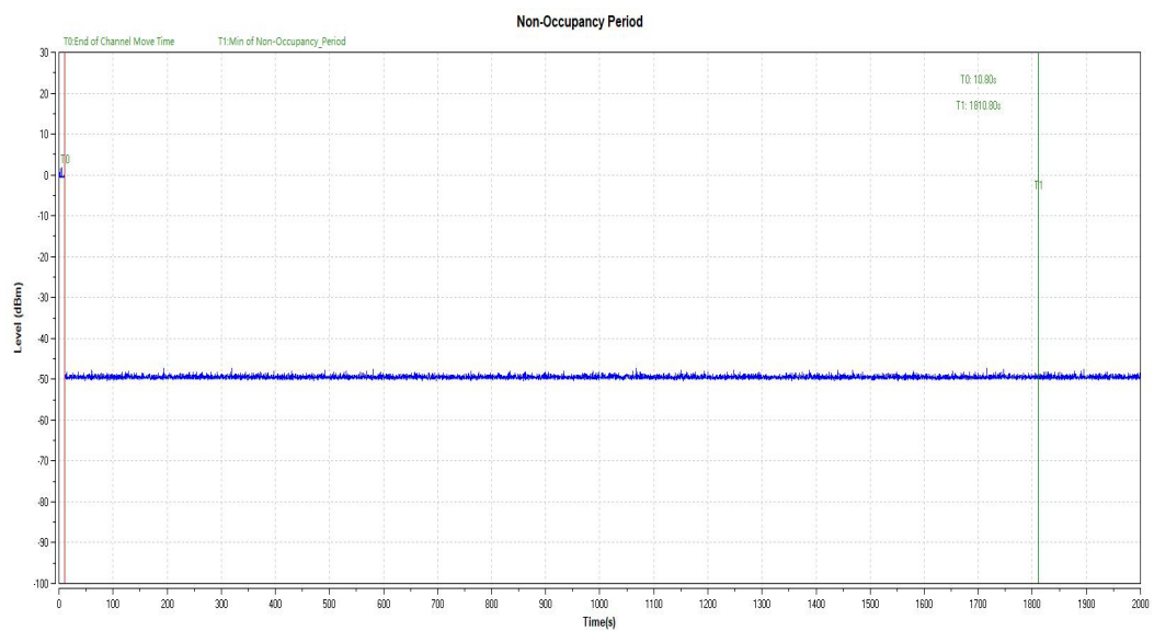
Fig.3 Non-Occupancy Period (HT20 Frequency Band: 5250MHz ~ 5350MHz)
