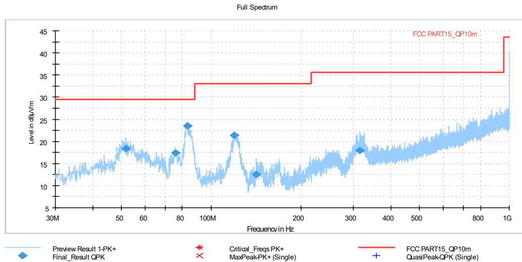
Figure A.1 Radiated Emission from 30MHz to 1GHz
