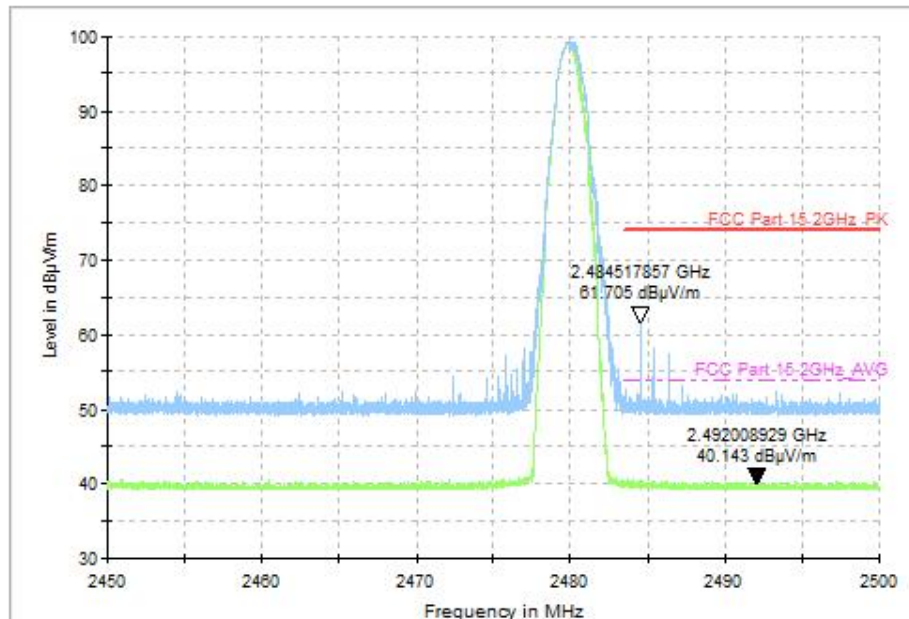
Fig. 37 Radiated Band Edges (GFSK, CH78, 2.45GHz~2.50GHz)
