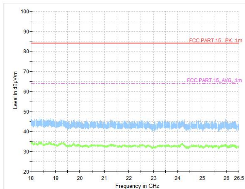
Fig. 50 Radiated Spurious Emission (All Channels, 18GHz ~26.5GHz)
