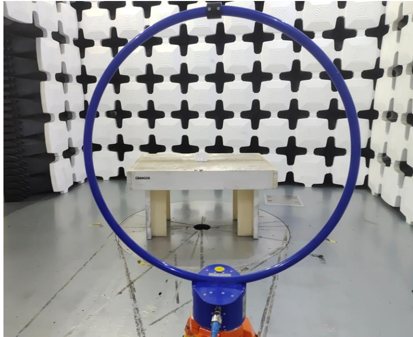
3. Radiated Emissions (Part 15C, 9kHz-30MHz)
