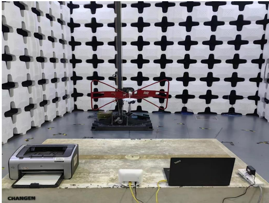
1. Radiated Emissions (Part 15B LTE receiver, 30MHz-1GHz)
