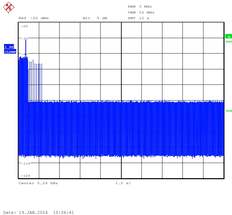
Fig.A.2 Channel move time
