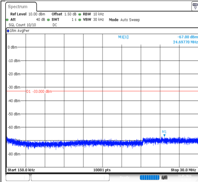
EGPRS1900-661-2-0.15~30MHz-PASS
