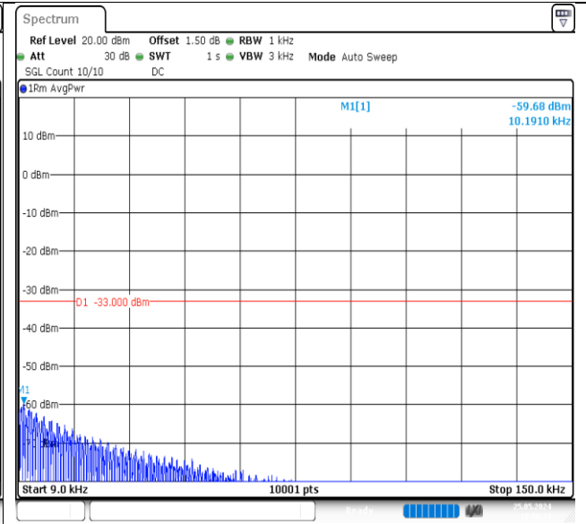
GPRS850-190-5-0.009~0.15MHz-PASS
