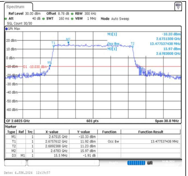
Band41-15MHz-16QAM-41515-75RB#0-PASS
