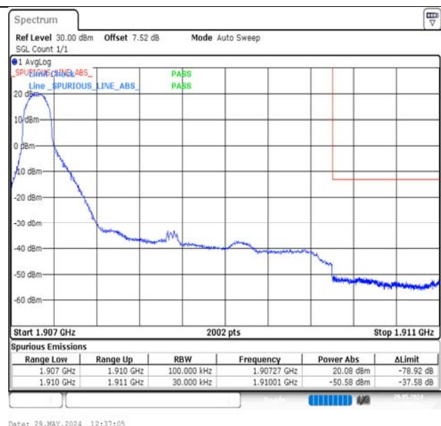
Band2-3MHz-16QAM-19185-1RB#0-PASS
