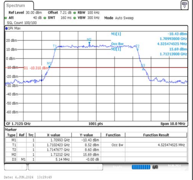
Band66-5MHz-16QAM-131997-25RB#0-PASS
