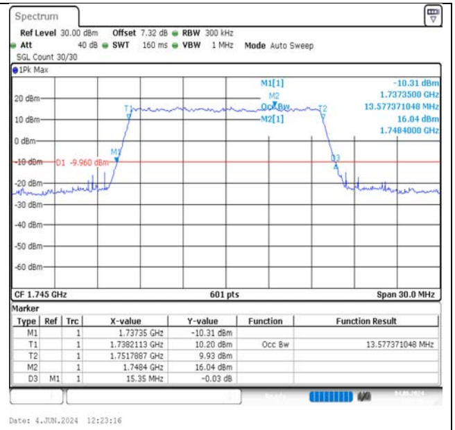
Band66-15MHz-QPSK-132322-75RB#0-PASS
