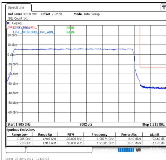
Band2-5MHz-QPSK-19175-25RB#0-PASS
