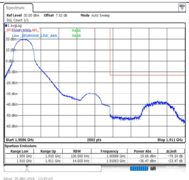
Band2-1.4MHz-16QAM-19193-1RB#0-PASS
