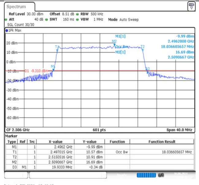
Band41-20MHz-16QAM-39750-100RB#0-PASS
