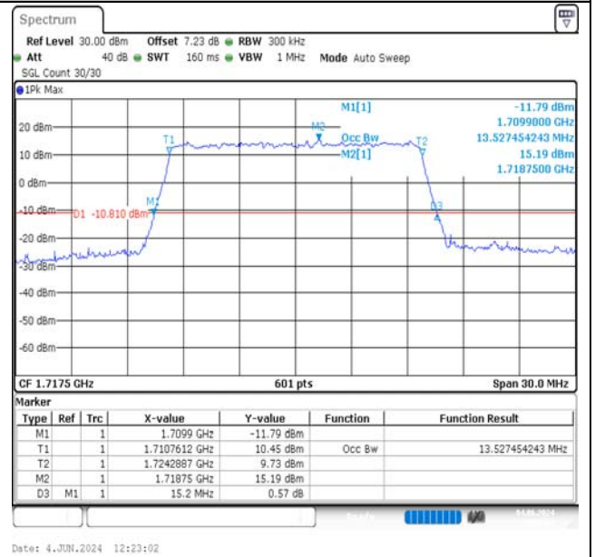
Band66-15MHz-16QAM-132047-75RB#0-PASS
