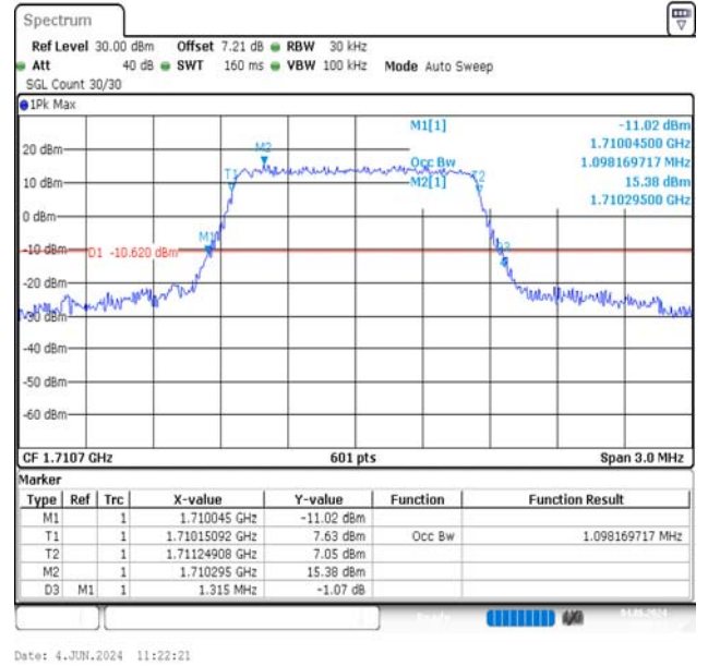
Band66-1.4MHz-16QAM-131979-6RB#0-PASS
