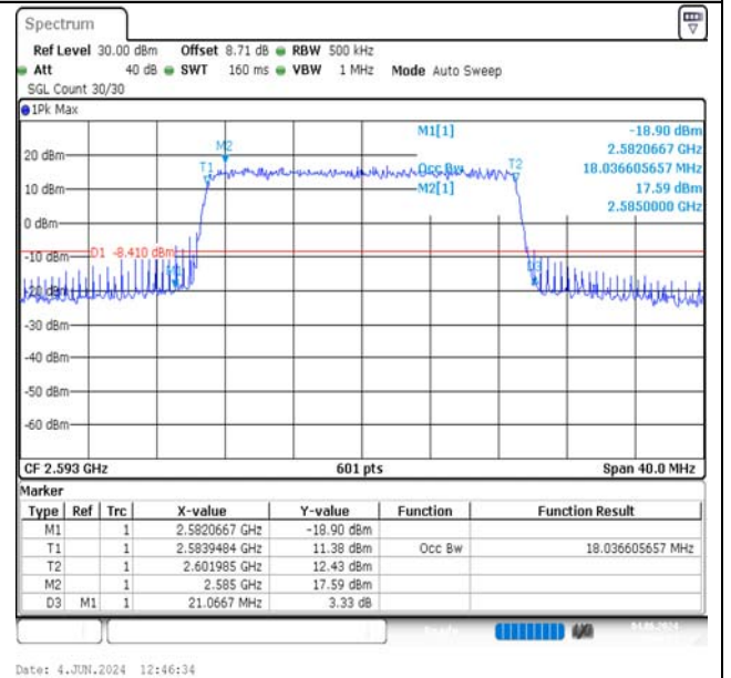
Band41-20MHz-QPSK-40620-100RB#0-PASS
