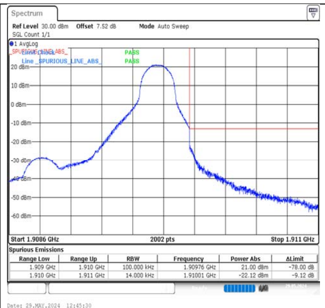
Band2-1.4MHz-QPSK-19193-1RB#5-PASS
