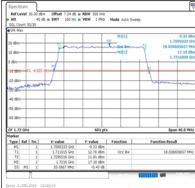
Band66-20MHz-QPSK-132072-100RB#0-PASS
