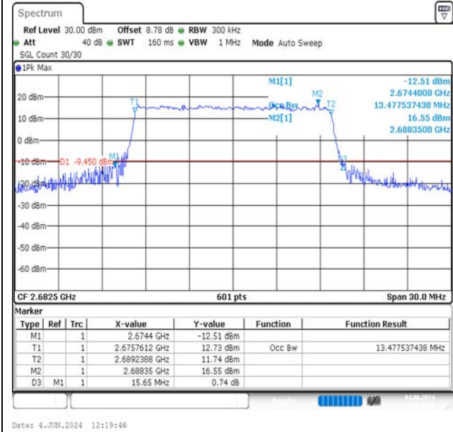
Band41-15MHz-QPSK-41515-75RB#0-PASS
