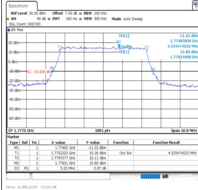
Band66-5MHz-QPSK-132647-25RB#0-PASS
