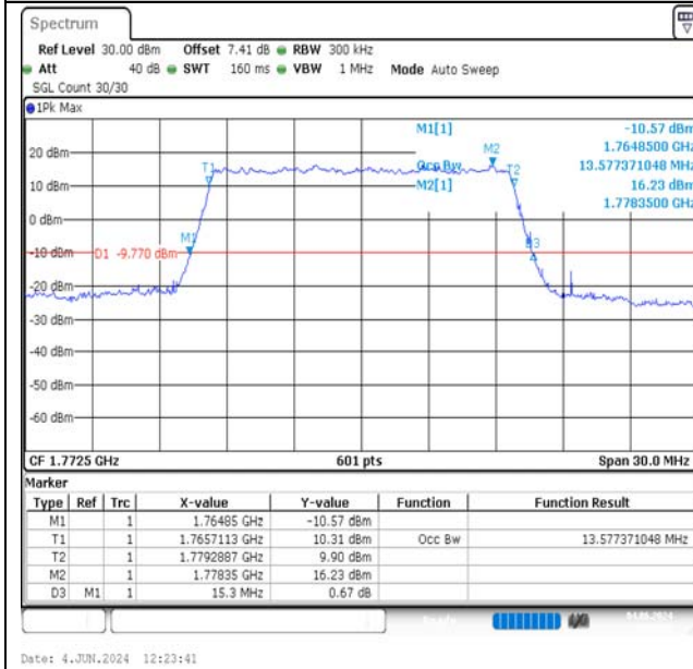
Band66-15MHz-QPSK-132597-75RB#0-PASS
