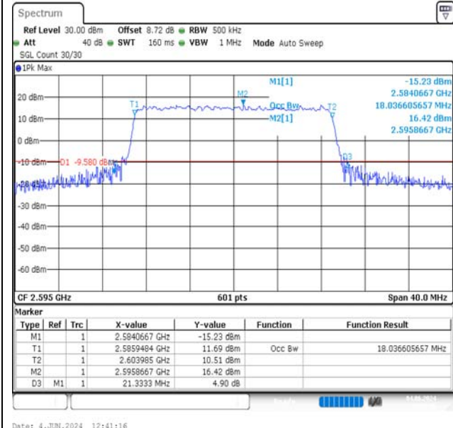
Band38-20MHz-16QAM-38000-100RB#0-PASS
