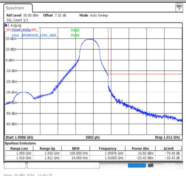
Band2-1.4MHz-16QAM-19193-1RB#5-PASS
