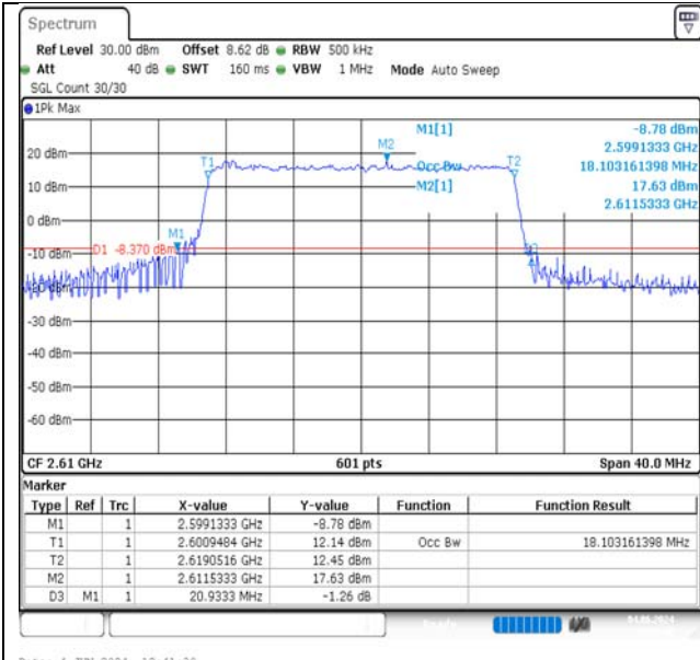
Band38-20MHz-QPSK-38150-100RB#0-PASS
