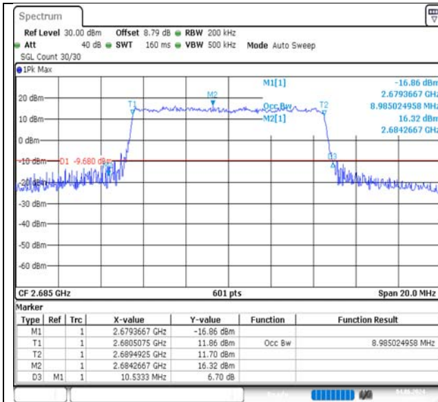
Band41-10MHz-QPSK-41540-50RB#0-PASS
