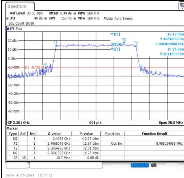
Band41-10MHz-QPSK-39700-50RB#0-PASS
