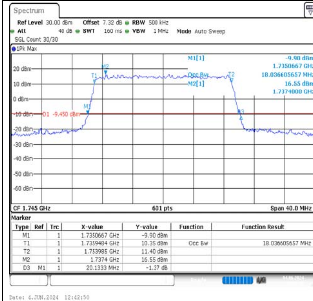
Band66-20MHz-16QAM-132322-100RB#0-PASS
