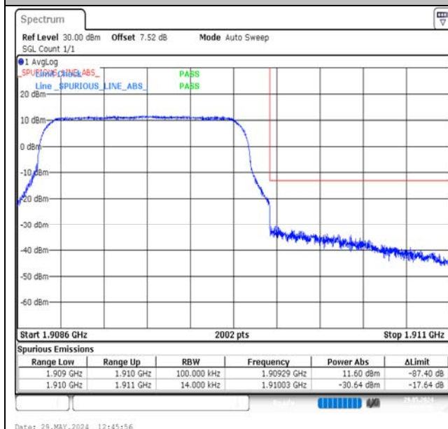
Band2-1.4MHz-16QAM-19193-6RB#0-PASS
