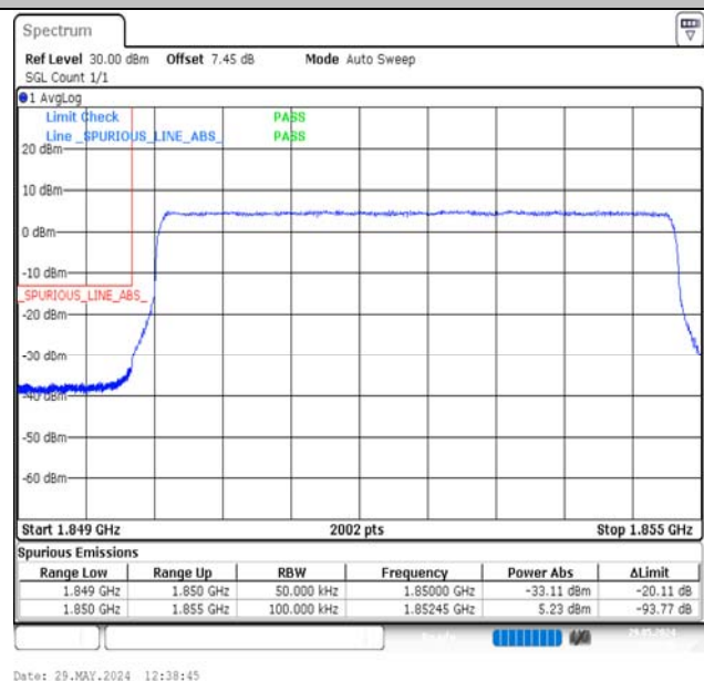
Band2-5MHz-16QAM-18625-25RB#0-PASS
