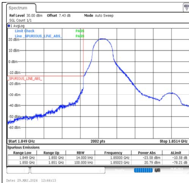
Band2-1.4MHz-QPSK-18607-1RB#0-PASS
