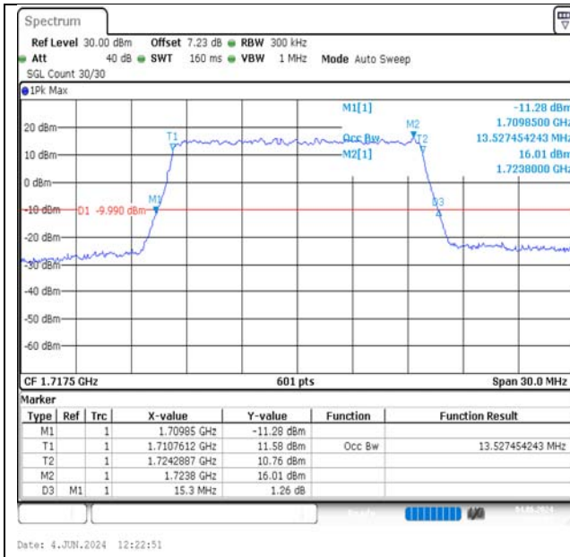
Band66-15MHz-QPSK-132047-75RB#0-PASS
