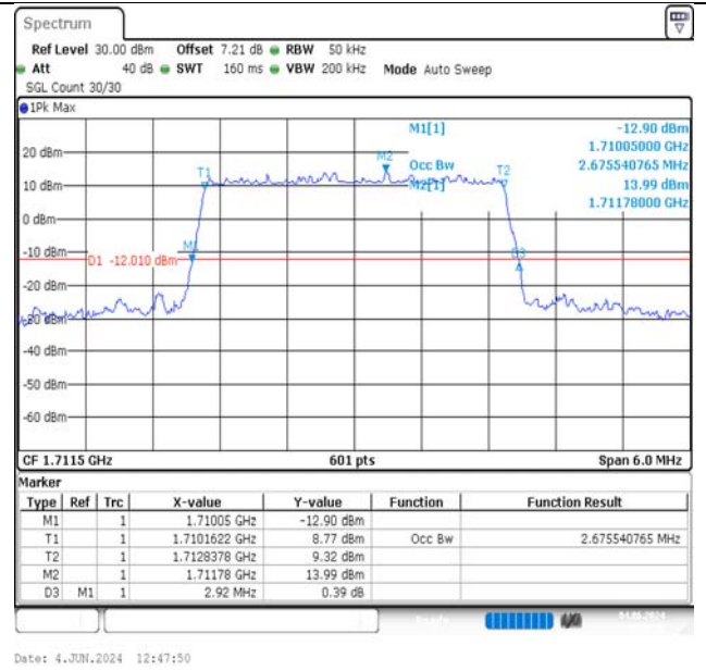
Band66-3MHz-16QAM-131987-15RB#0-PASS
