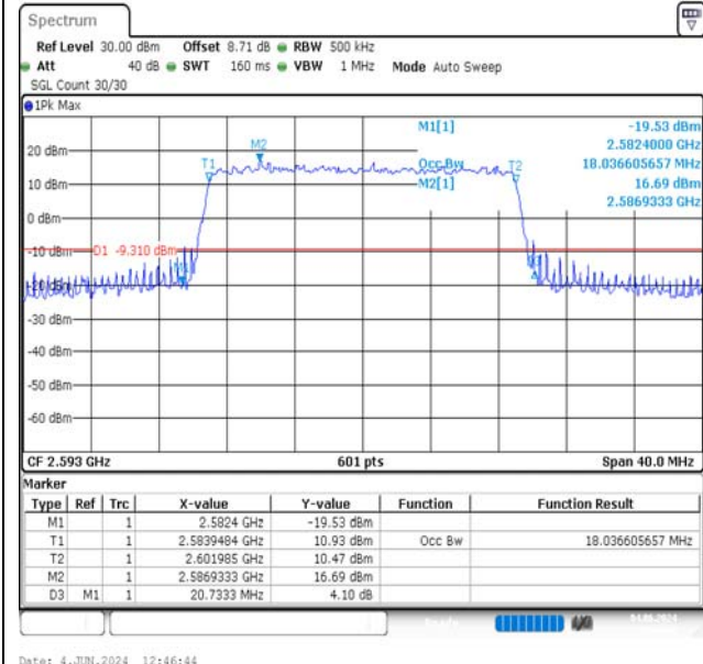
Band41-20MHz-16QAM-40620-100RB#0-PASS
