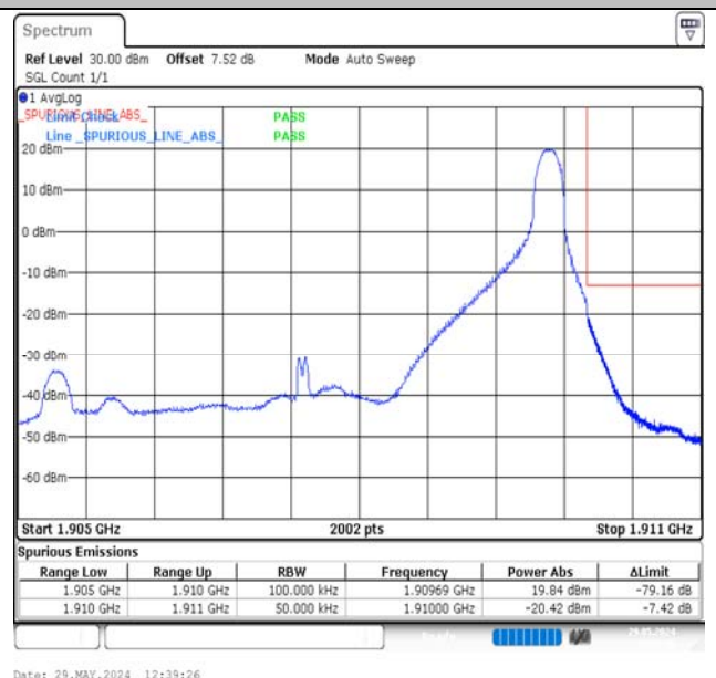
Band2-5MHz-16QAM-19175-1RB#24-PASS
