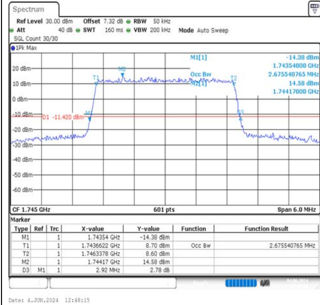
Band66-3MHz-16QAM-132322-15RB#0-PASS
