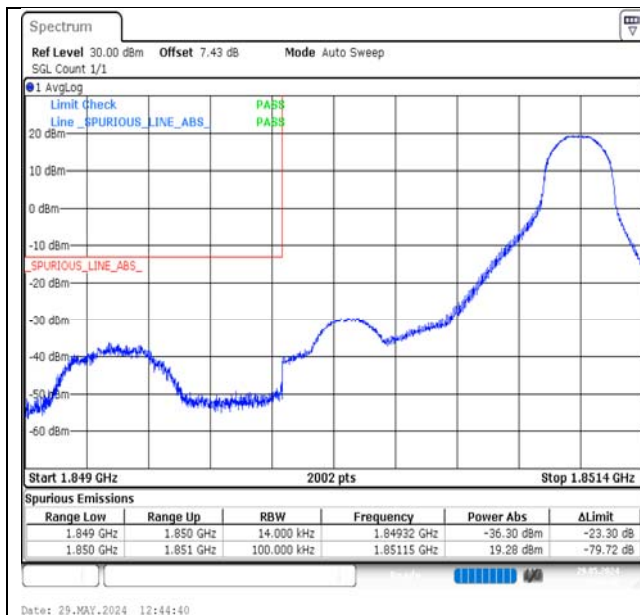
Band2-1.4MHz-16QAM-18607-1RB#5-PASS
