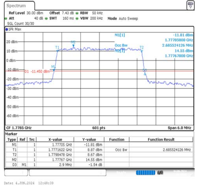
Band66-3MHz-16QAM-132657-15RB#0-PASS
