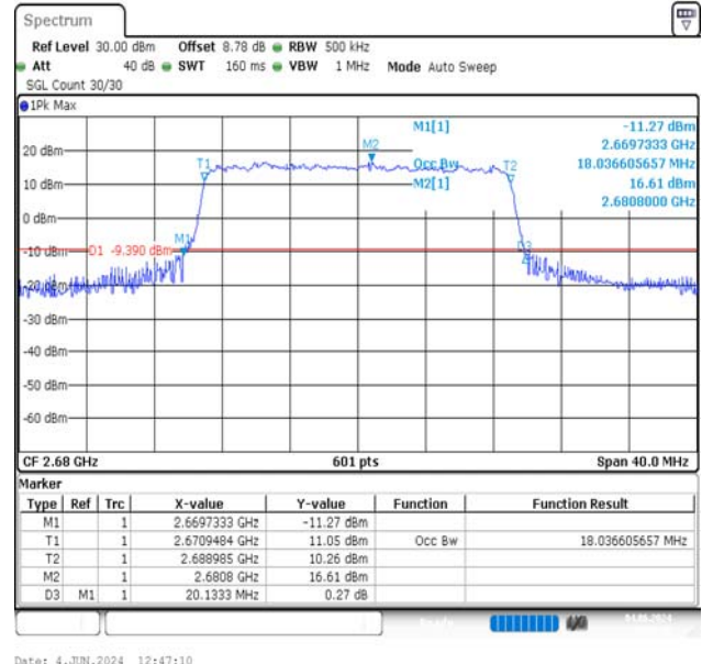
Band41-20MHz-16QAM-41490-100RB#0-PASS
