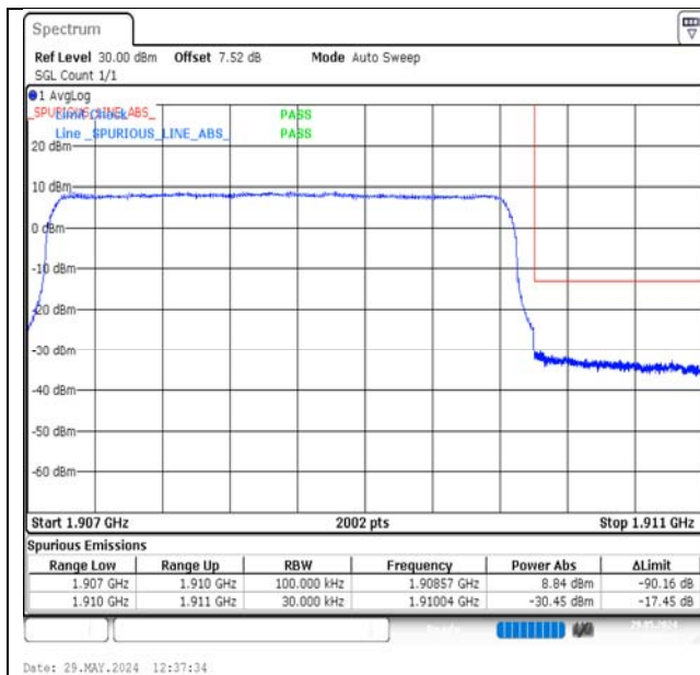
Band2-3MHz-QPSK-19185-15RB#0-PASS
