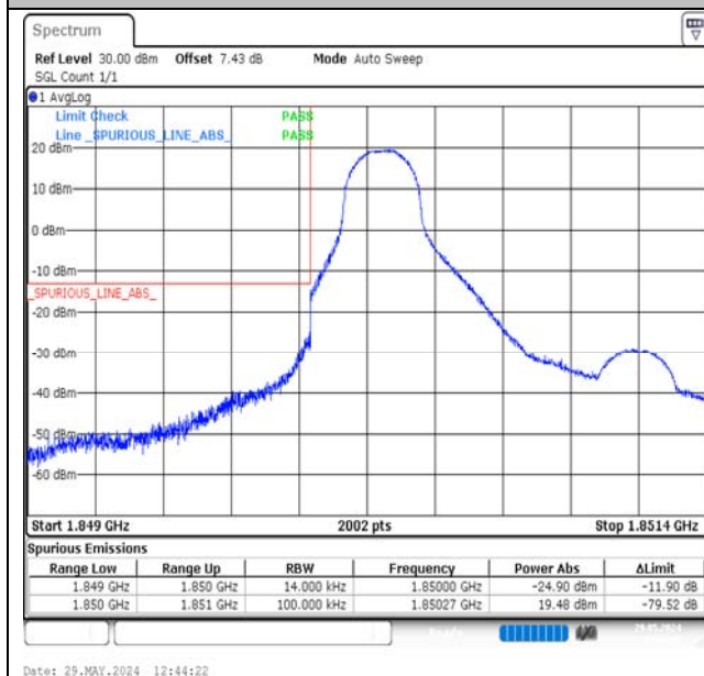
Band2-1.4MHz-16QAM-18607-1RB#0-PASS
