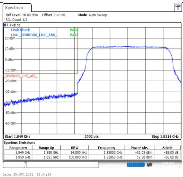
Band2-1.4MHz-QPSK-18607-6RB#0-PASS
