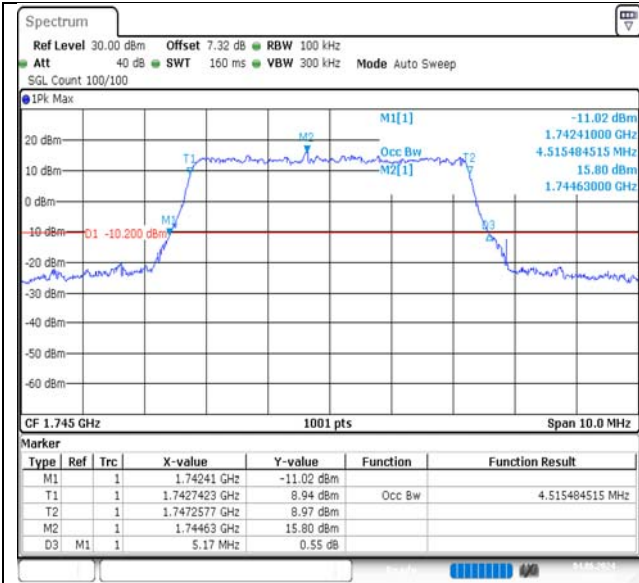
Band66-5MHz-16QAM-132322-25RB#0-PASS
