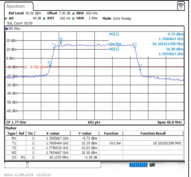
Band66-20MHz-16QAM-132572-100RB#0-PASS
