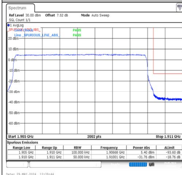
Band2-5MHz-16QAM-19175-25RB#0-PASS
