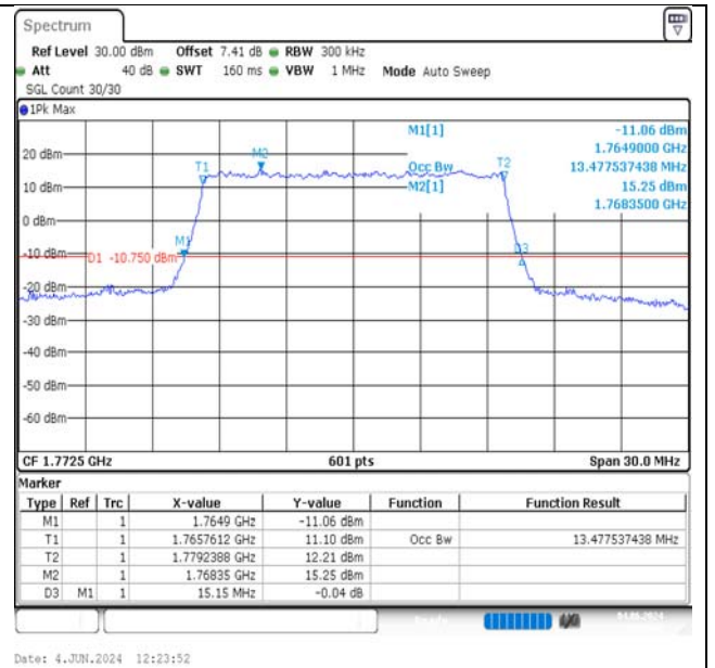
Band66-15MHz-16QAM-132597-75RB#0-PASS
