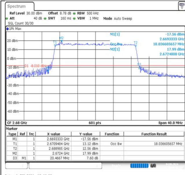
Band41-20MHz-QPSK-41490-100RB#0-PASS
