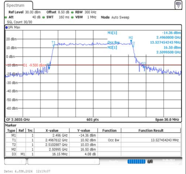
Band41-15MHz-16QAM-39725-75RB#0-PASS
