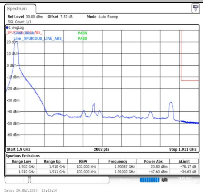
Band2-10MHz-QPSK-19150-1RB#0-PASS
