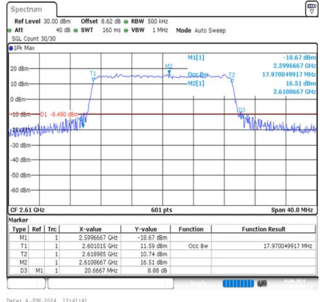
Band38-20MHz-16QAM-38150-100RB#0-PASS
