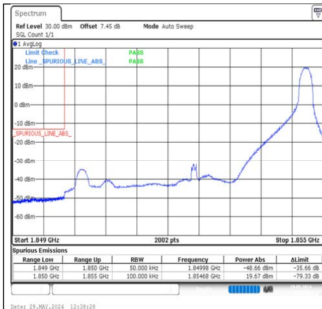
Band2-5MHz-16QAM-18625-1RB#24-PASS
