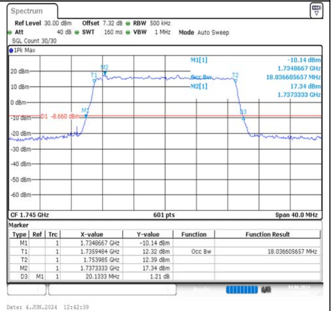
Band66-20MHz-QPSK-132322-100RB#0-PASS
