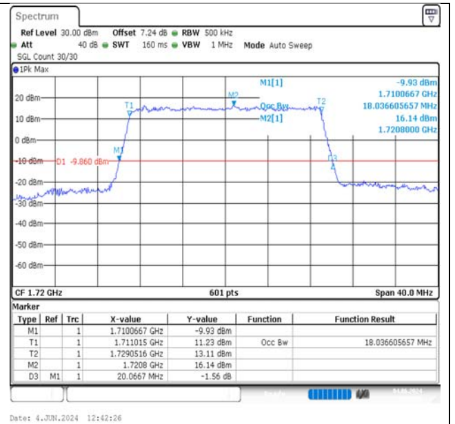
Band66-20MHz-16QAM-132072-100RB#0-PASS
