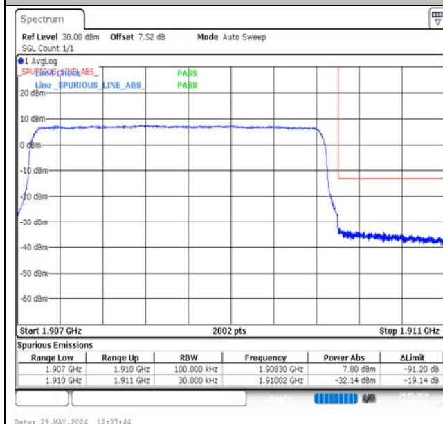
Band2-3MHz-16QAM-19185-15RB#0-PASS
