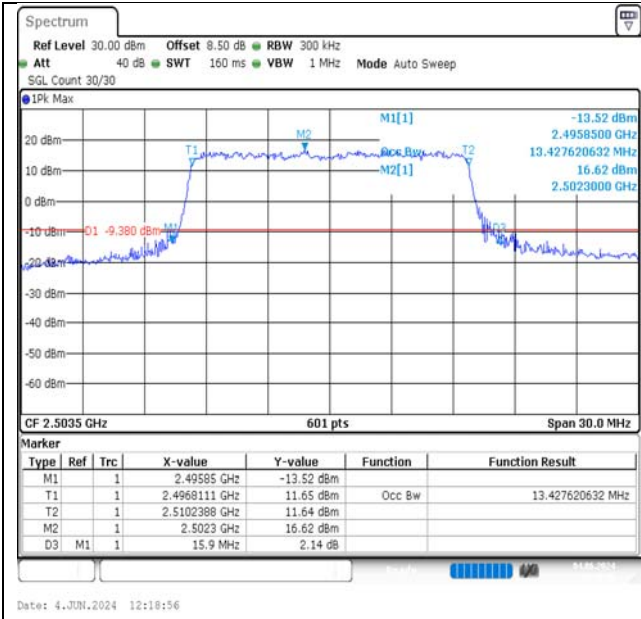
Band41-15MHz-QPSK-39725-75RB#0-PASS
