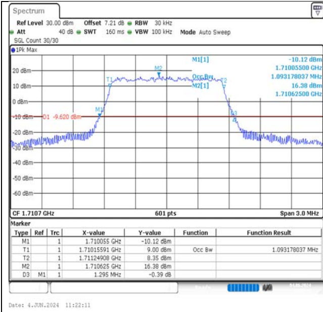
Band66-1.4MHz-QPSK-131979-6RB#0-PASS
