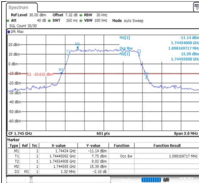
Band66-1.4MHz-16QAM-132322-6RB#0-PASS
