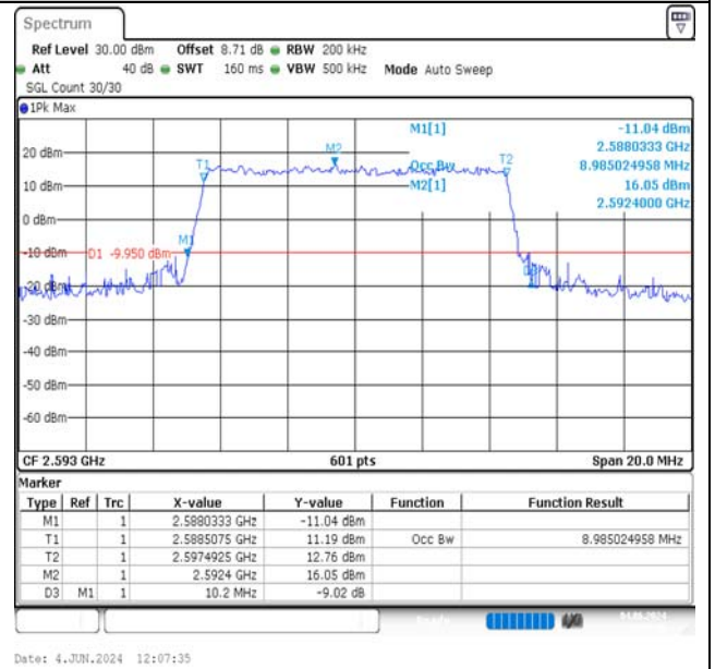
Band41-10MHz-QPSK-40620-50RB#0-PASS
