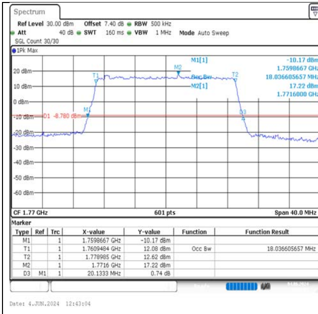
Band66-20MHz-QPSK-132572-100RB#0-PASS
