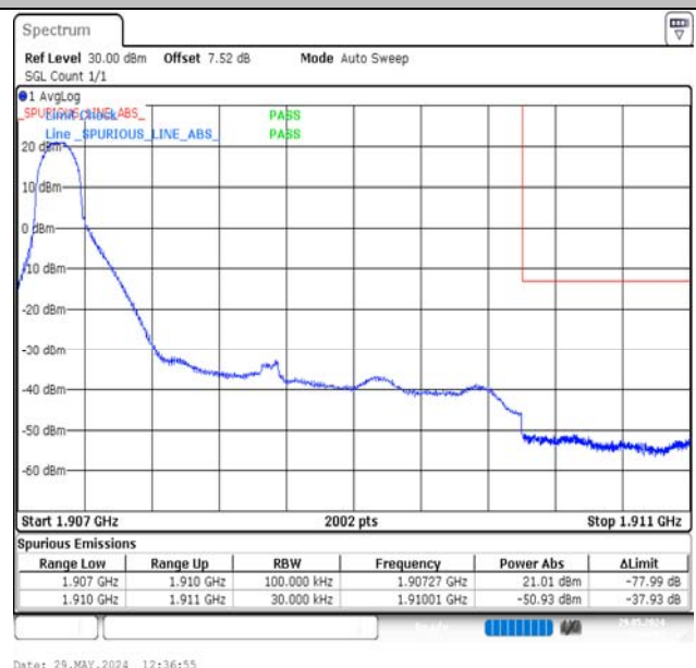
Band2-3MHz-QPSK-19185-1RB#0-PASS
