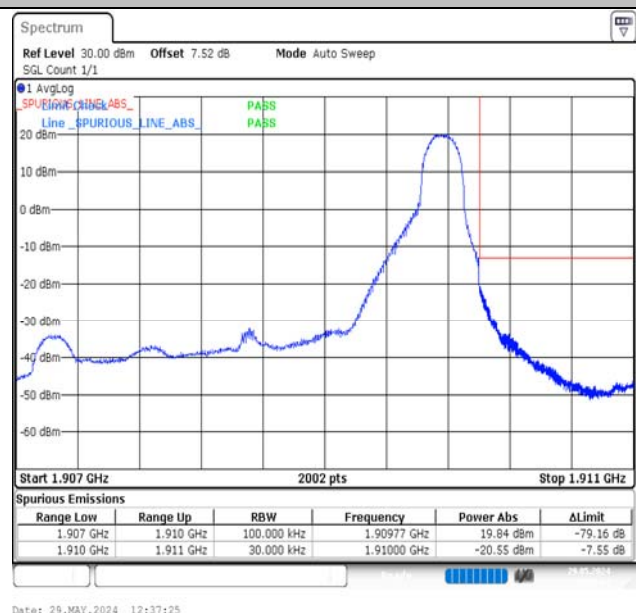
Band2-3MHz-16QAM-19185-1RB#14-PASS
