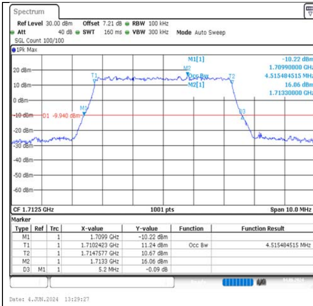
Band66-5MHz-QPSK-131997-25RB#0-PASS
