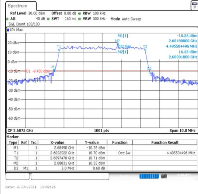
Band41-5MHz-QPSK-41565-25RB#0-PASS
