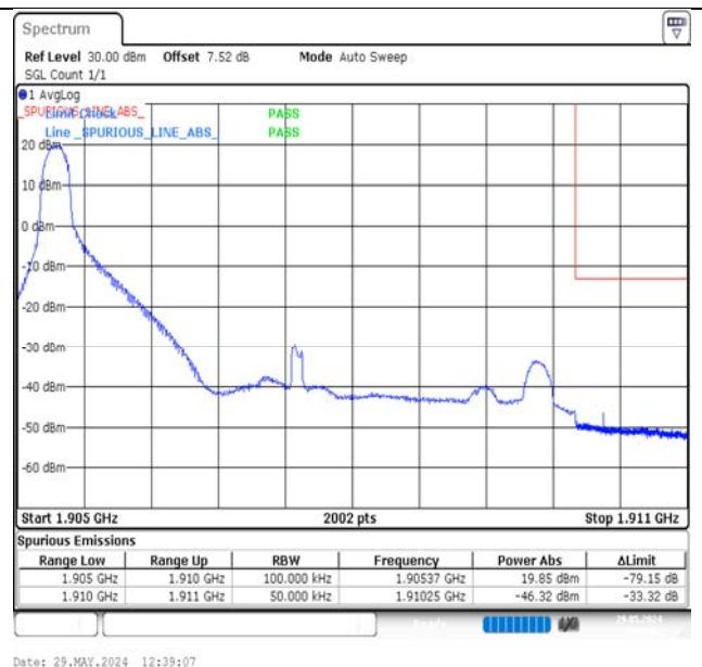
Band2-5MHz-16QAM-19175-1RB#0-PASS
