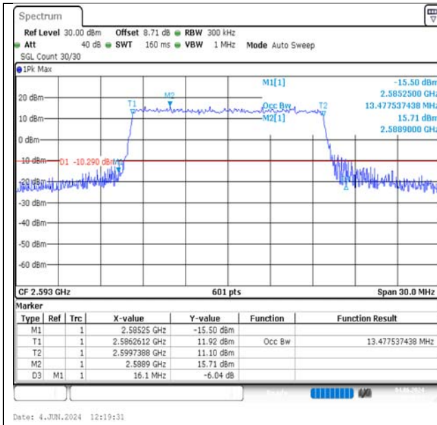
Band41-15MHz-16QAM-40620-75RB#0-PASS
