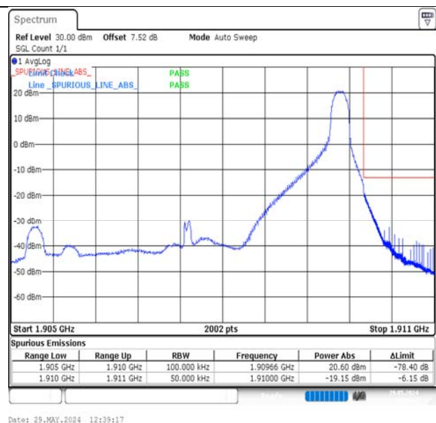
Band2-5MHz-QPSK-19175-1RB#24-PASS
