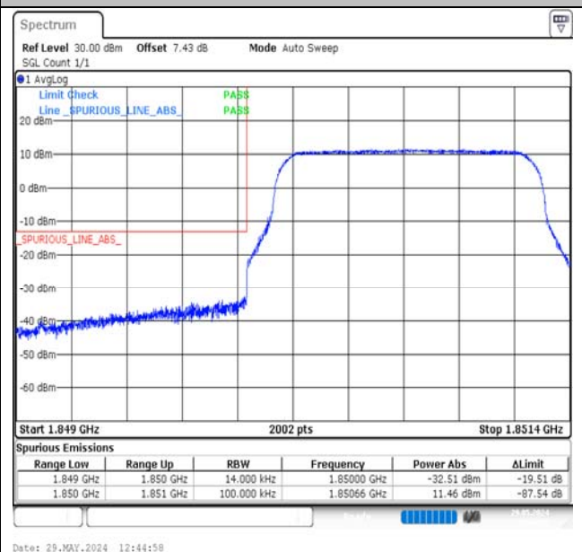
Band2-1.4MHz-16QAM-18607-6RB#0-PASS
