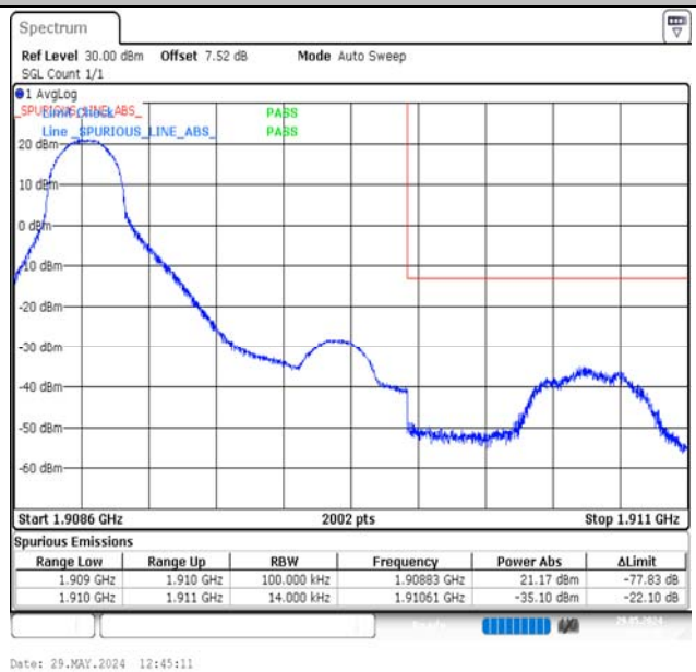
Band2-1.4MHz-QPSK-19193-1RB#0-PASS
