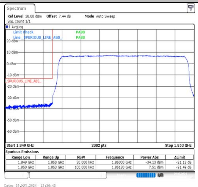
Band2-3MHz-16QAM-18615-15RB#0-PASS
