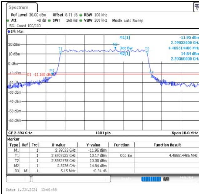
Band41-5MHz-16QAM-40620-25RB#0-PASS
