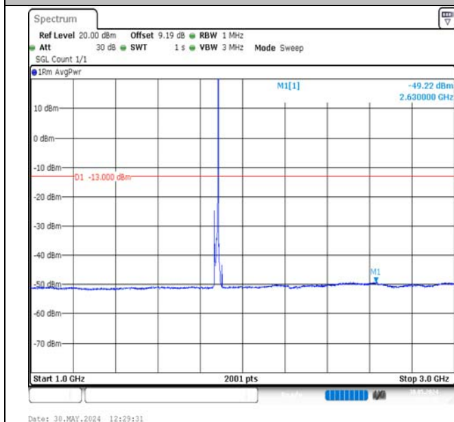
Band2-10MHz-QPSK-18900-1RB#49-1000~3000-PASS
