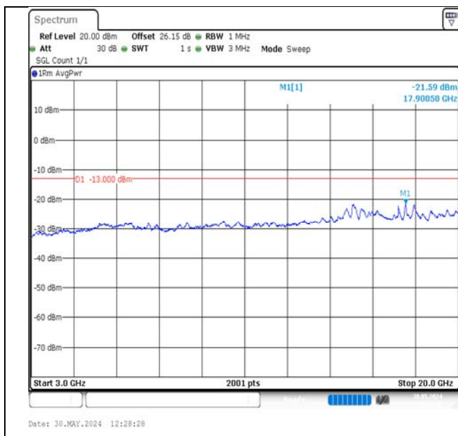
Band2-10MHz-16QAM-18650-50RB#0-3000~20000-PASS
