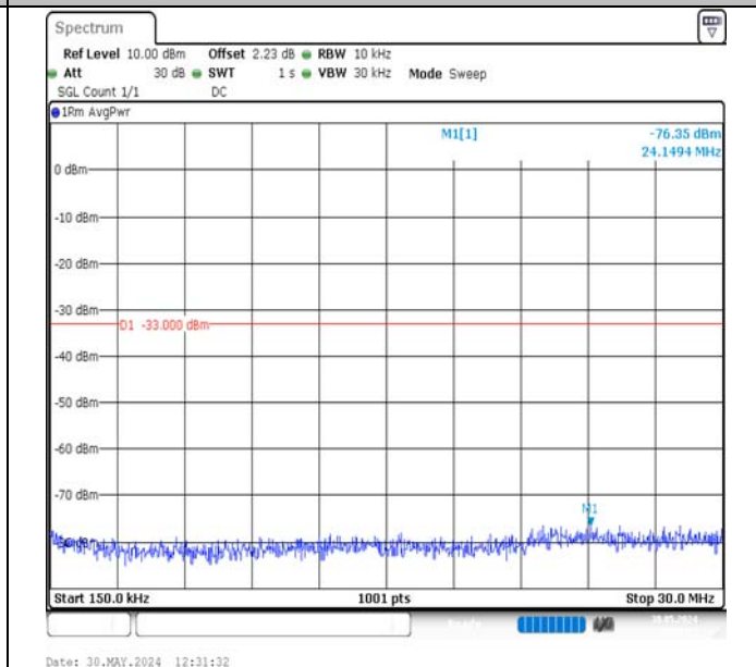
Band2-10MHz-QPSK-19150-1RB#49-0.15~30-PASS
