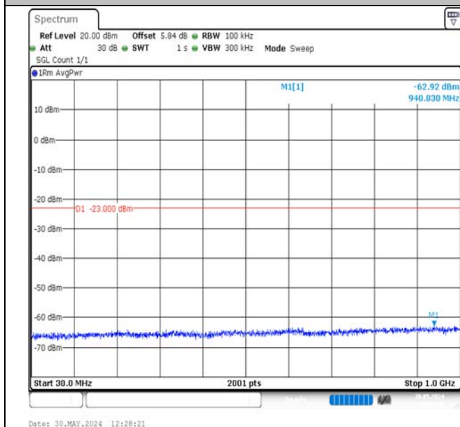
Band2-10MHz-16QAM-18650-50RB#0-30~1000-PASS
