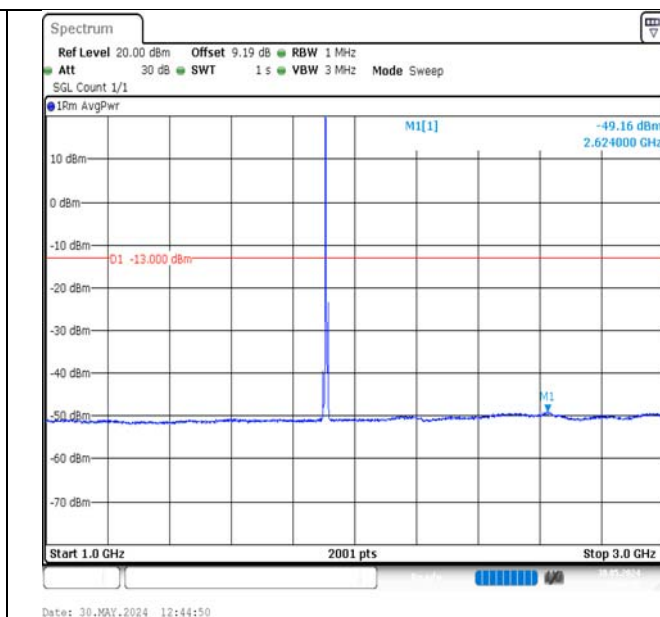
Band2-5MHz-QPSK-19175-1RB#0-1000~3000-PASS
