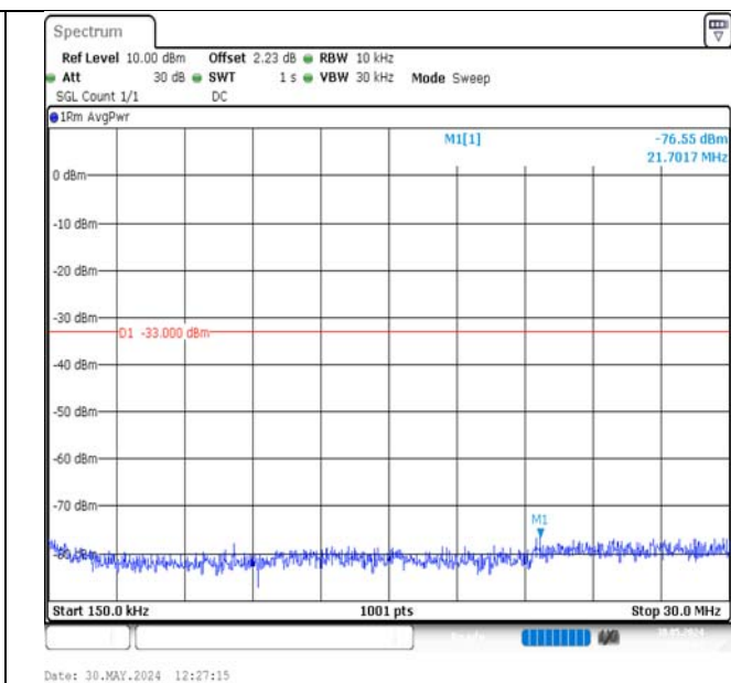
Band2-10MHz-QPSK-18650-1RB#49-0.15~30-PASS
