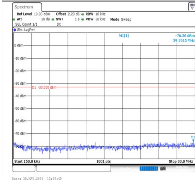
Band2-5MHz-16QAM-19175-1RB#24-0.15~30-PASS
