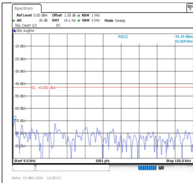
Band2-10MHz-16QAM-18650-50RB#0-0.009~0.15-PASS
