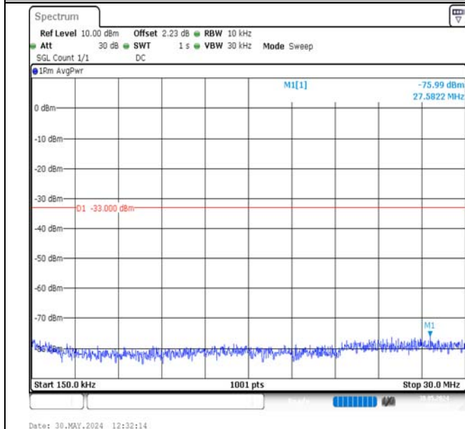
Band2-10MHz-QPSK-19150-50RB#0-0.15~30-PASS
