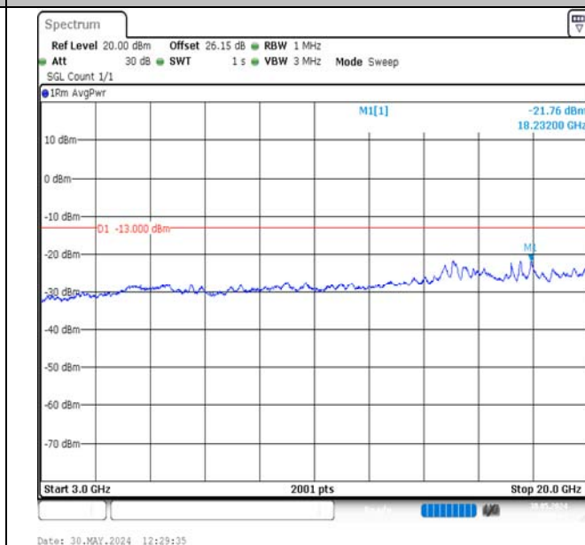
Band2-10MHz-QPSK-18900-1RB#49-3000~20000-PASS
