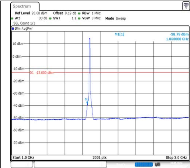
Band2-10MHz-QPSK-18900-50RB#0-1000~3000-PASS
