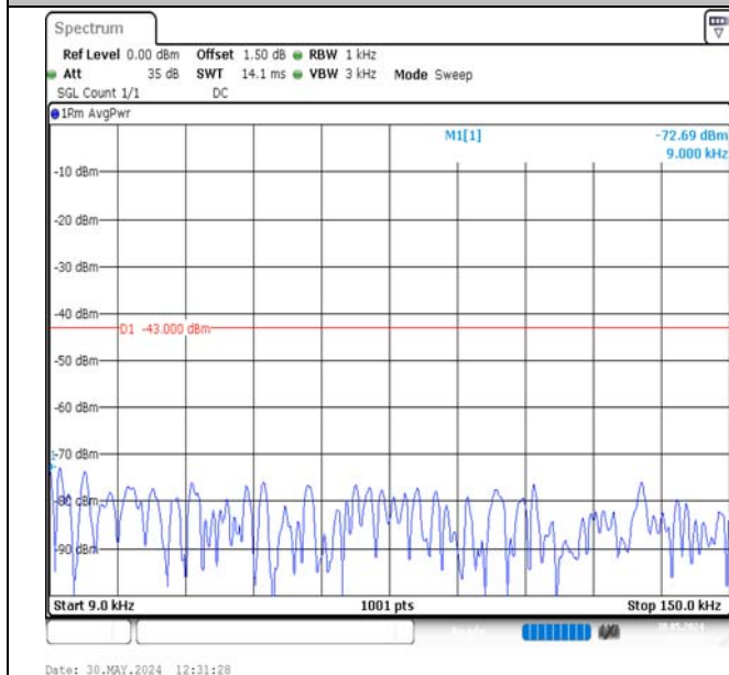
Band2-10MHz-QPSK-19150-1RB#49-0.009~0.15-PASS
