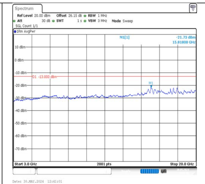
Band2-5MHz-16QAM-18625-1RB#0-3000~20000-PASS
