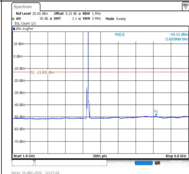
Band2-10MHz-QPSK-18650-1RB#49-1000~3000-PASS
