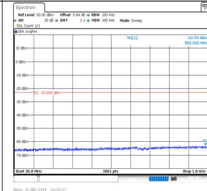
Band2-10MHz-QPSK-19150-50RB#0-30~1000-PASS
