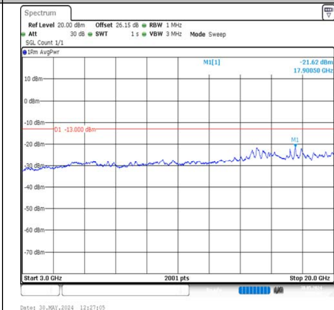
Band2-10MHz-16QAM-18650-1RB#0-3000~20000-PASS
