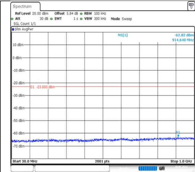
Band2-10MHz-QPSK-18900-50RB#0-30~1000-PASS
