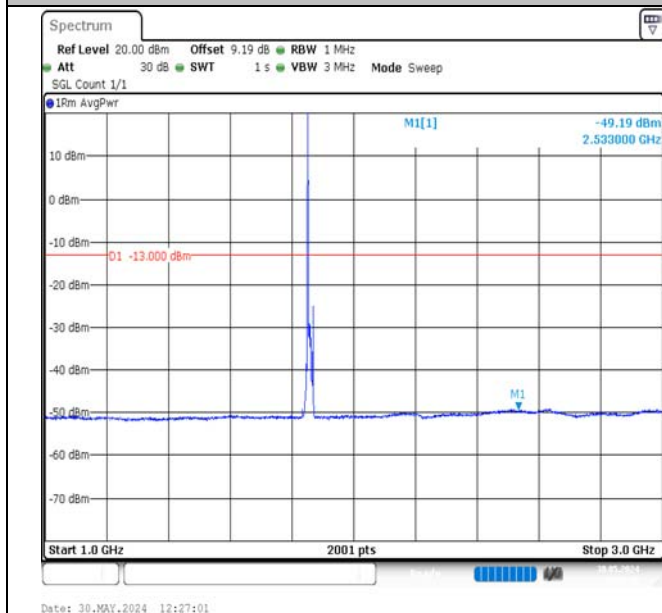
Band2-10MHz-16QAM-18650-1RB#0-1000~3000-PASS
