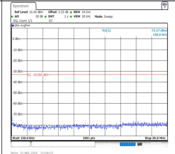
Band2-10MHz-QPSK-18650-1RB#0-0.15~30-PASS
