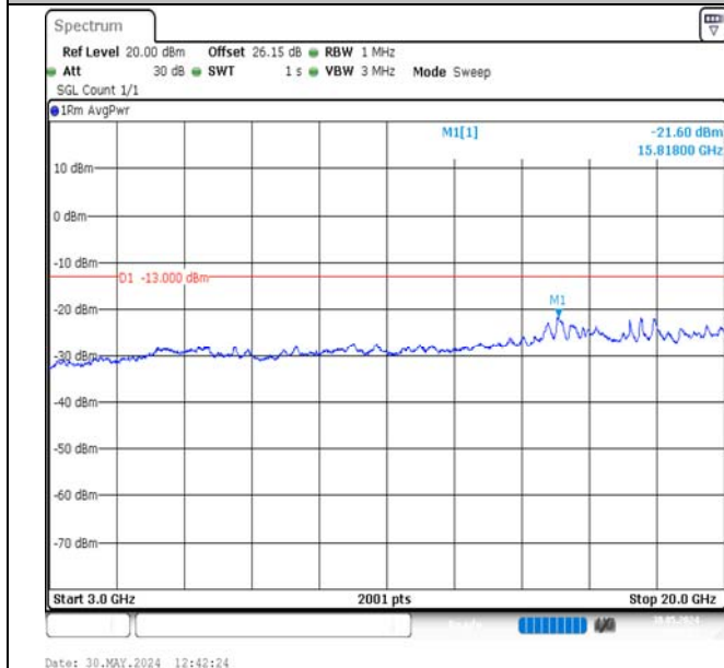
Band2-5MHz-16QAM-18625-25RB#0-3000~20000-PASS
