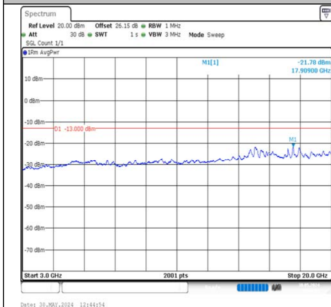
Band2-5MHz-QPSK-19175-1RB#0-3000~20000-PASS
