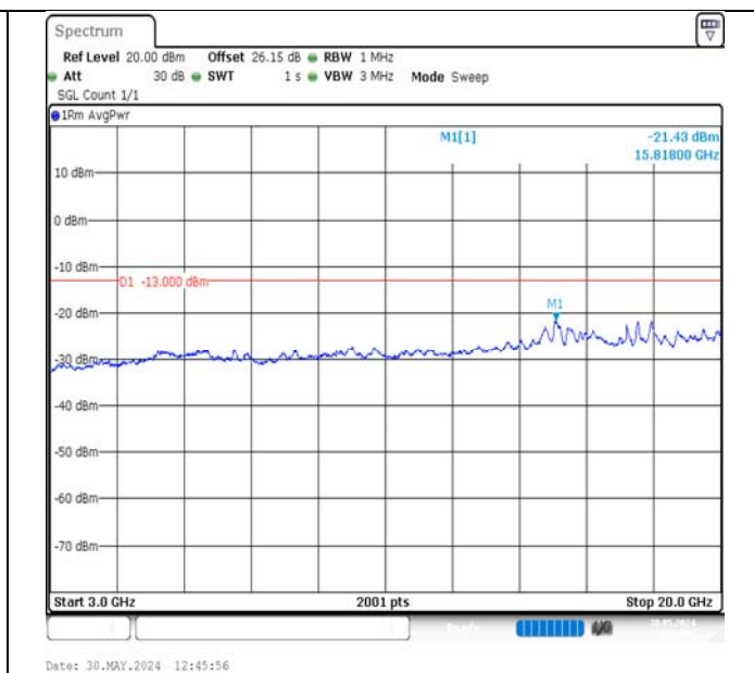
Band2-5MHz-16QAM-19175-1RB#24-3000~20000-PASS
