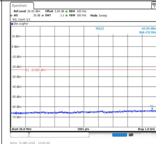
Band2-5MHz-16QAM-19175-1RB#24-30~1000-PASS
