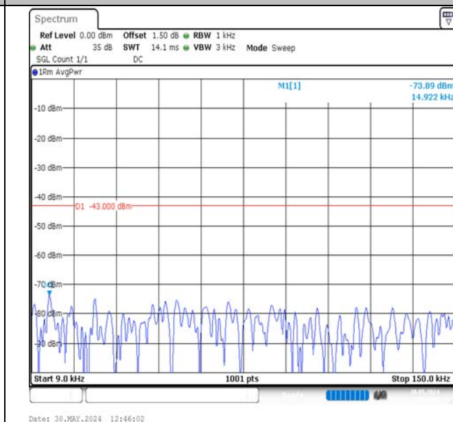
Band2-5MHz-QPSK-19175-25RB#0-0.009~0.15-PASS
