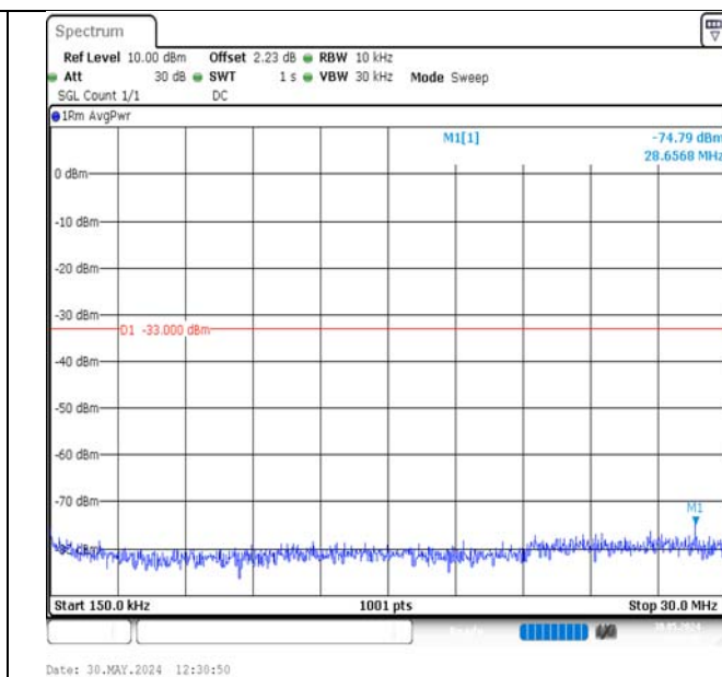
Band2-10MHz-QPSK-19150-1RB#0-0.15~30-PASS
