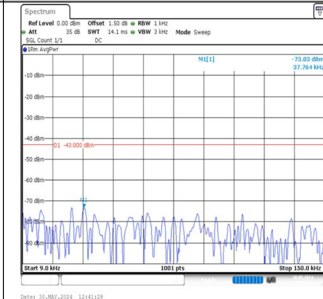
Band2-5MHz-16QAM-18625-1RB#24-0.009~0.15-PASS
