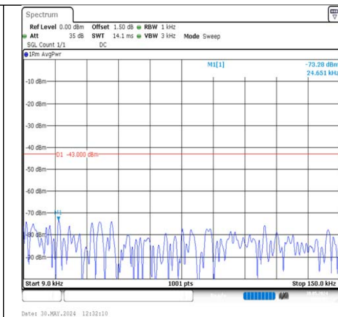
Band2-10MHz-QPSK-19150-50RB#0-0.009~0.15-PASS
