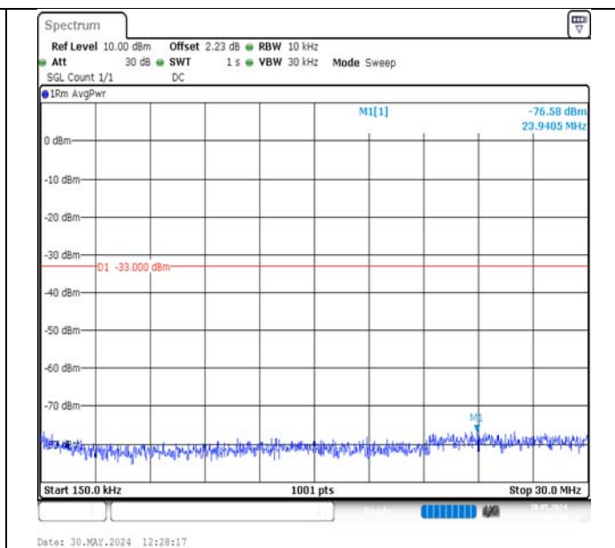
Band2-10MHz-16QAM-18650-50RB#0-0.15~30-PASS
