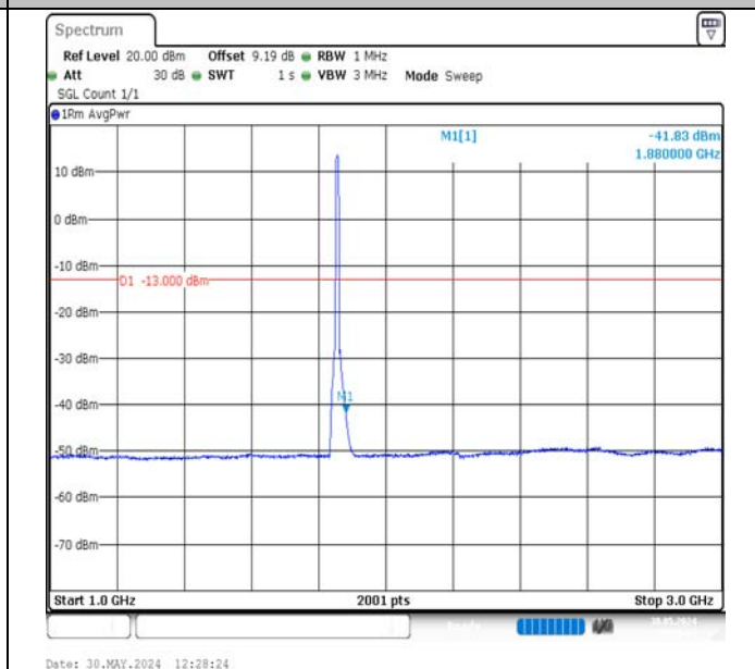
Band2-10MHz-16QAM-18650-50RB#0-1000~3000-PASS
