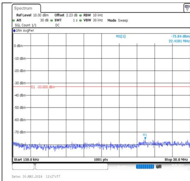
Band2-10MHz-QPSK-18650-50RB#0-0.15~30-PASS
