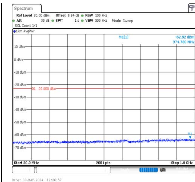
Band2-10MHz-16QAM-18650-1RB#0-30~1000-PASS
