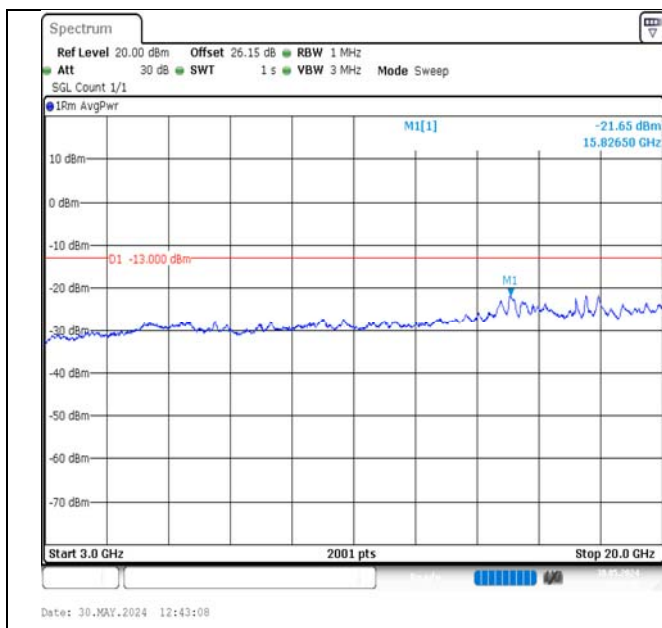
Band2-5MHz-16QAM-18900-1RB#0-3000~20000-PASS
