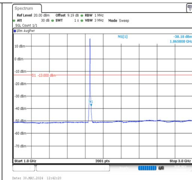
Band2-5MHz-16QAM-18625-25RB#0-1000~3000-PASS
