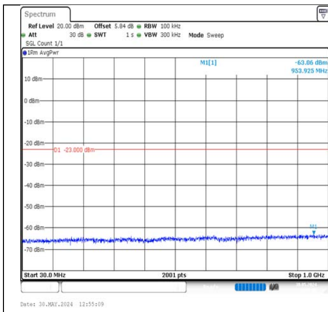
Band2-15MHz-16QAM-18675-75RB#0-30~1000-PASS
