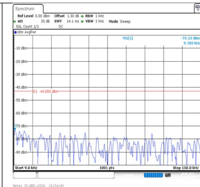
Band2-15MHz-QPSK-18675-75RB#0-0.009~0.15-PASS
