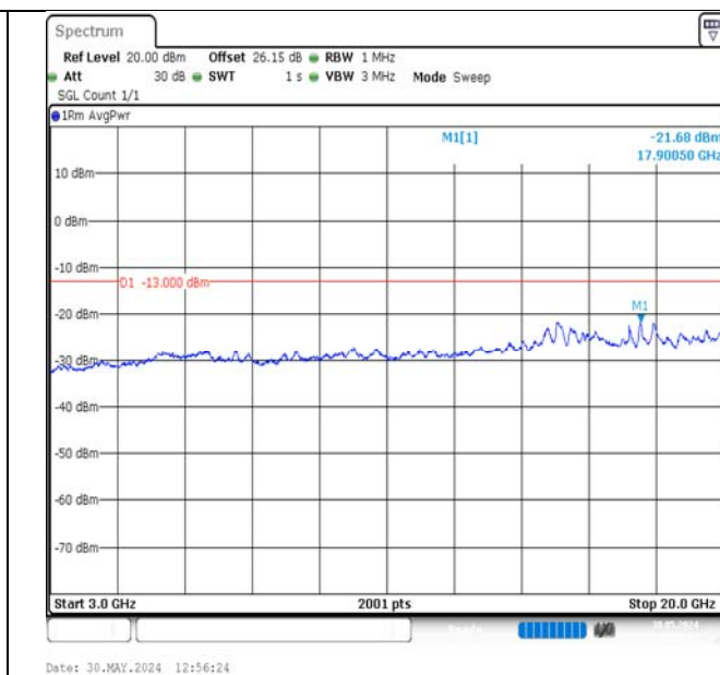
Band2-15MHz-QPSK-18900-1RB#74-3000~20000-PASS
