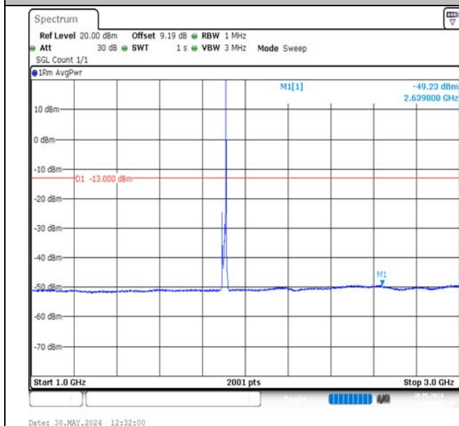
Band2-10MHz-16QAM-19150-1RB#49-1000~3000-PASS
