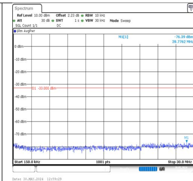
Band2-15MHz-16QAM-19125-75RB#0-0.15~30-PASS
