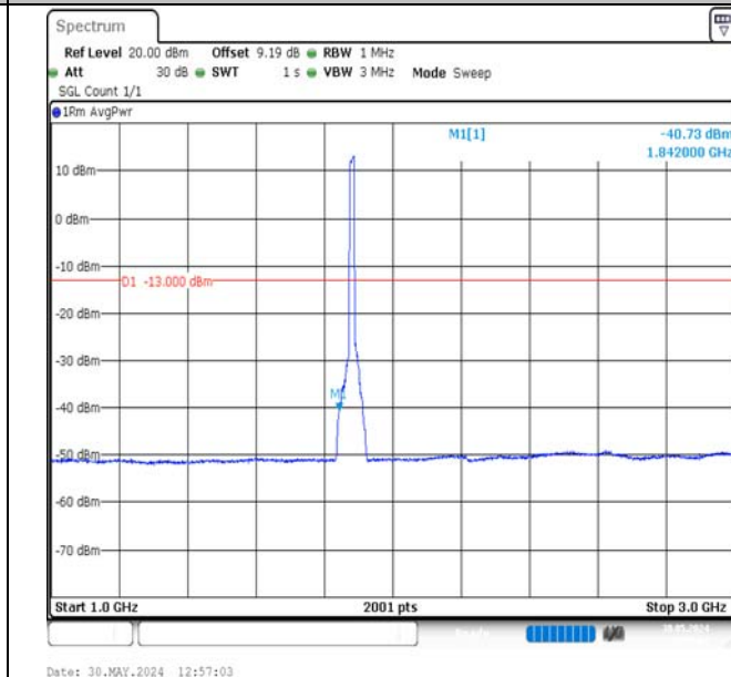
Band2-15MHz-QPSK-18900-75RB#0-1000~3000-PASS
