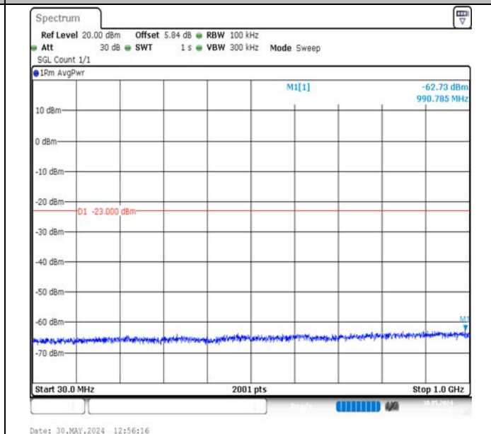
Band2-15MHz-QPSK-18900-1RB#74-30~1000-PASS
