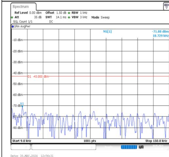
Band2-15MHz-16QAM-18900-1RB#74-0.009~0.15-PASS
