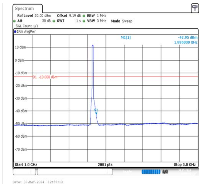
Band2-15MHz-16QAM-18675-75RB#0-1000~3000-PASS
