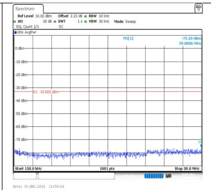
Band2-15MHz-QPSK-19125-1RB#74-0.15~30-PASS
