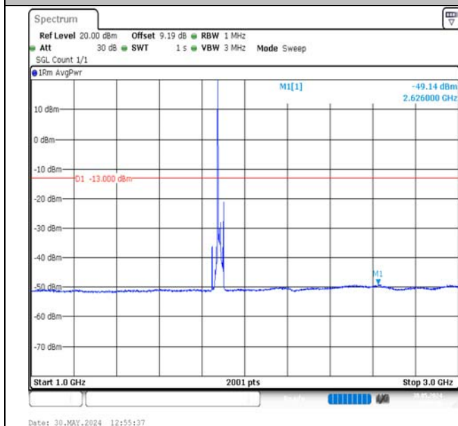
Band2-15MHz-QPSK-18900-1RB#0-1000~3000-PASS
