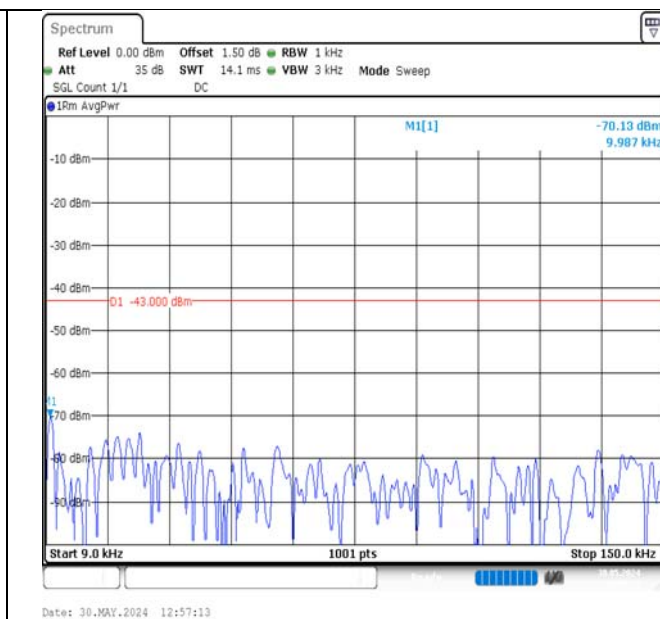
Band2-15MHz-16QAM-18900-75RB#0-0.009~0.15-PASS
