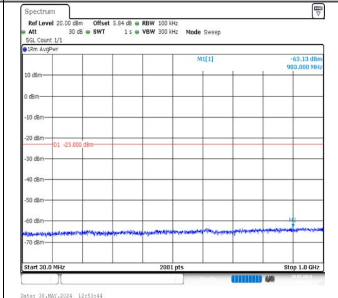
Band2-15MHz-16QAM-18675-1RB#0-30~1000-PASS
