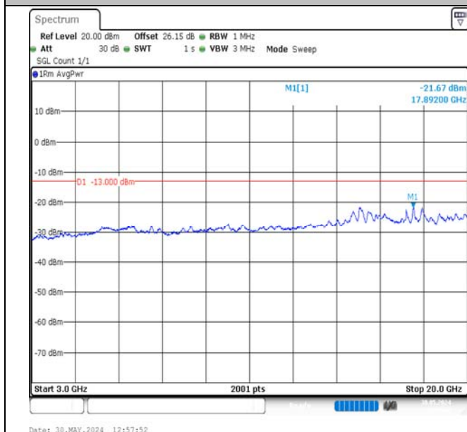
Band2-15MHz-QPSK-19125-1RB#0-3000~20000-PASS
