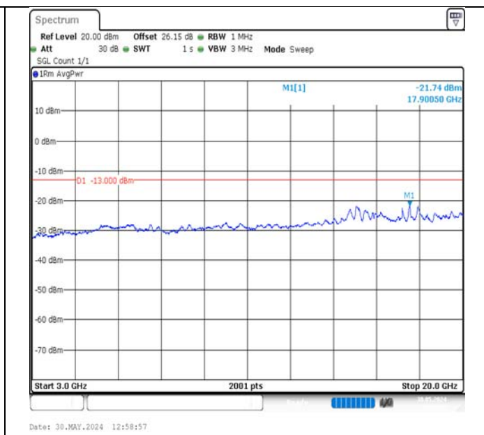
Band2-15MHz-16QAM-19125-1RB#74-3000~20000-PASS
