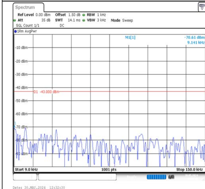
Band2-10MHz-16QAM-19150-50RB#0-0.009~0.15-PASS
