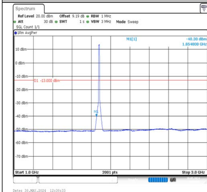
Band2-10MHz-16QAM-18900-50RB#0-1000~3000-PASS
