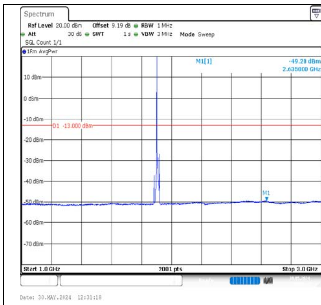
Band2-10MHz-16QAM-19150-1RB#0-1000~3000-PASS
