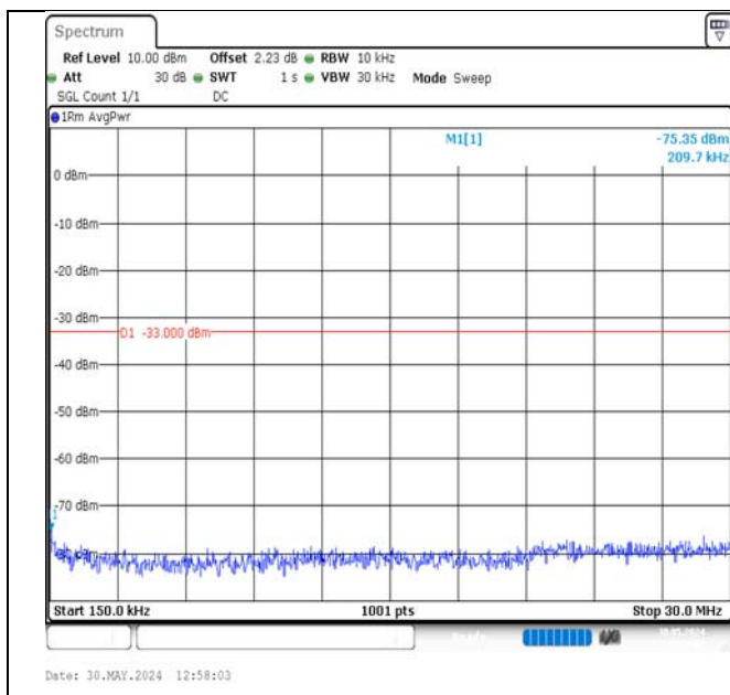
Band2-15MHz-16QAM-19125-1RB#0-0.15~30-PASS
