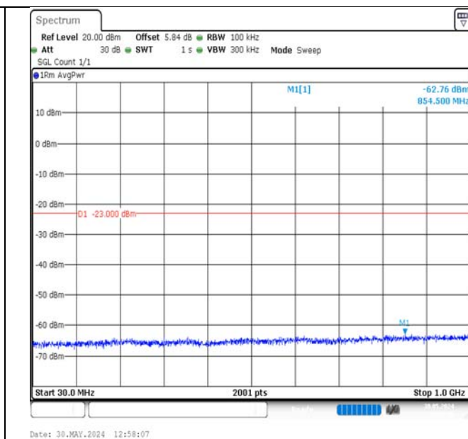
Band2-15MHz-16QAM-19125-1RB#0-30~1000-PASS
