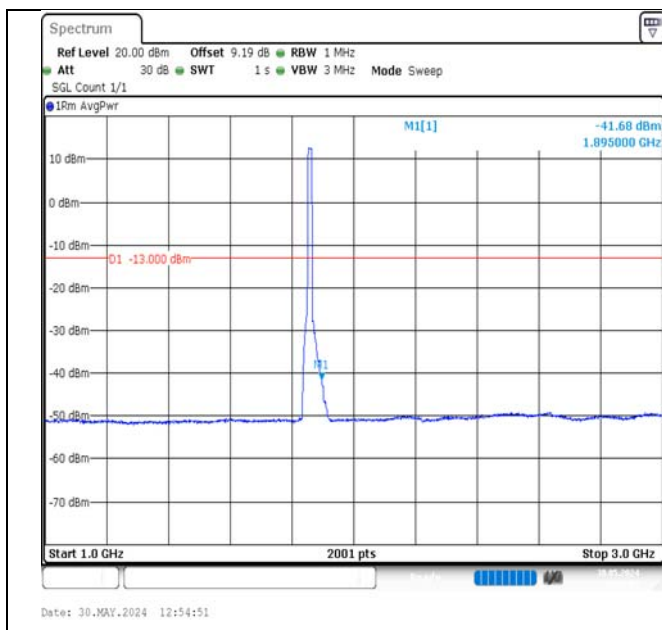
Band2-15MHz-QPSK-18675-75RB#0-1000~3000-PASS
