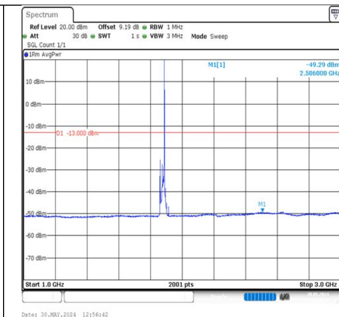
Band2-15MHz-16QAM-18900-1RB#74-1000~3000-PASS
