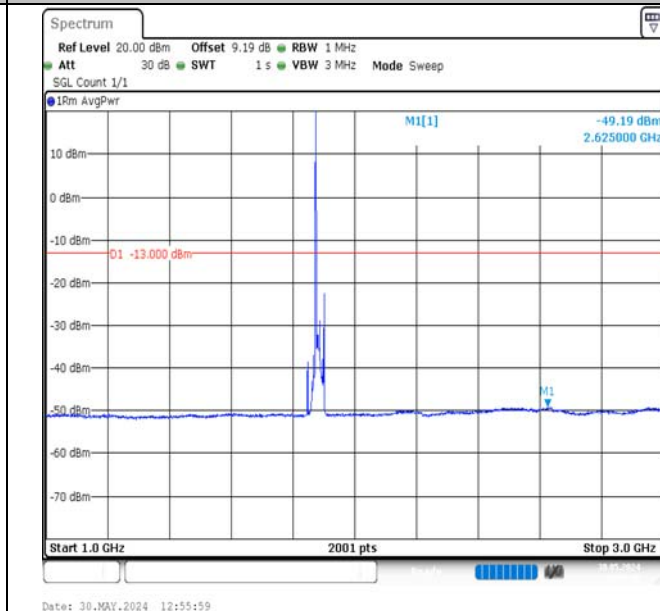
Band2-15MHz-16QAM-18900-1RB#0-1000~3000-PASS
