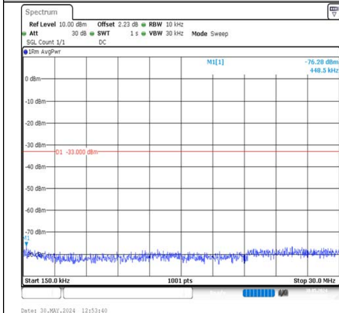
Band2-15MHz-16QAM-18675-1RB#0-0.15~30-PASS
