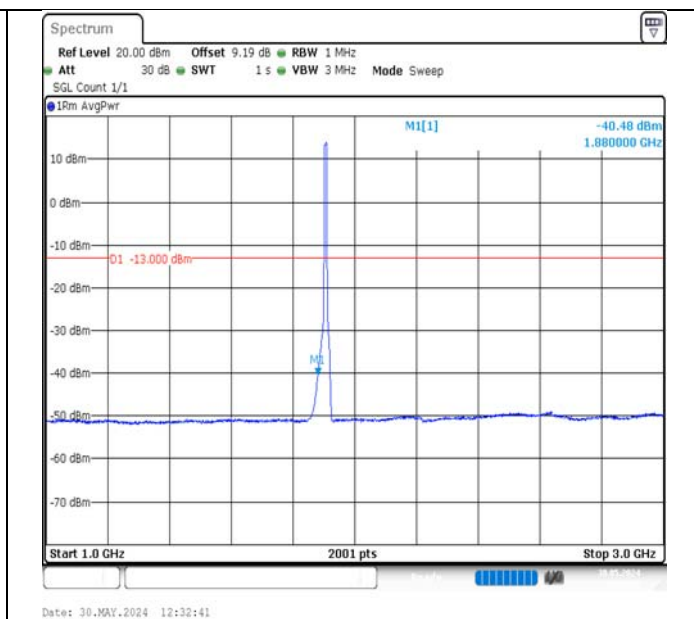
Band2-10MHz-16QAM-19150-50RB#0-1000~3000-PASS
