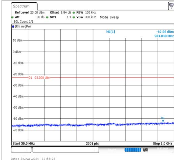
Band2-15MHz-QPSK-19125-1RB#74-30~1000-PASS
