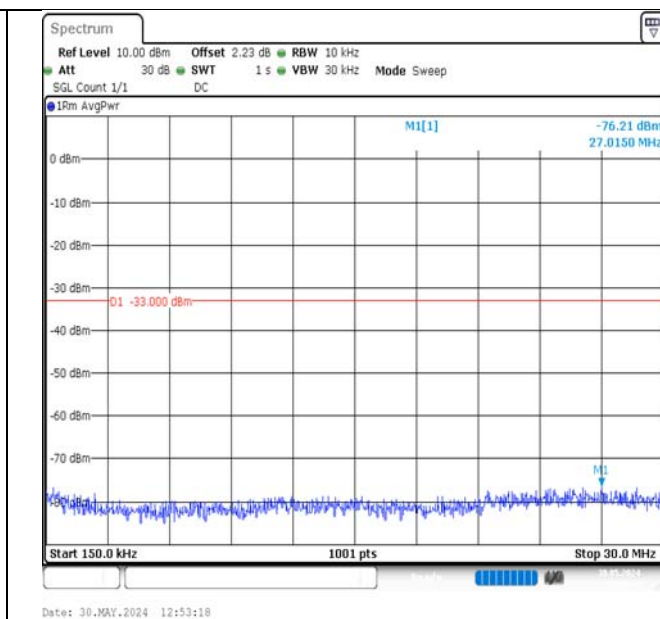
Band2-15MHz-QPSK-18675-1RB#0-0.15~30-PASS
