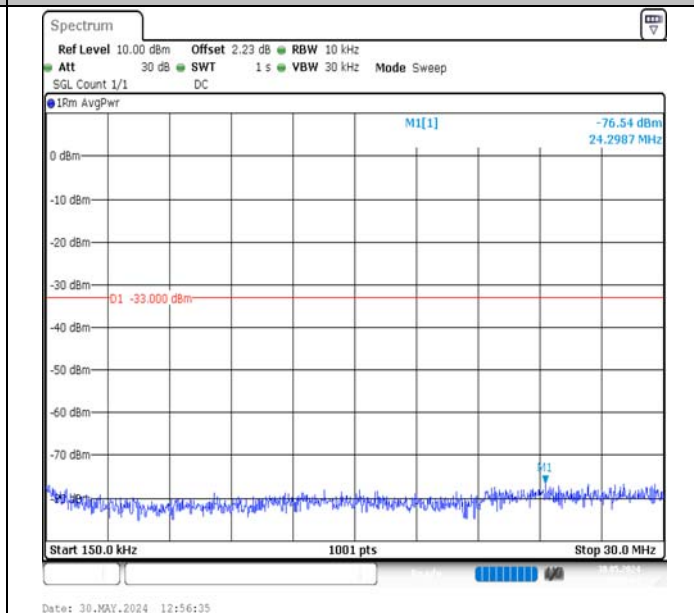
Band2-15MHz-16QAM-18900-1RB#74-0.15~30-PASS
