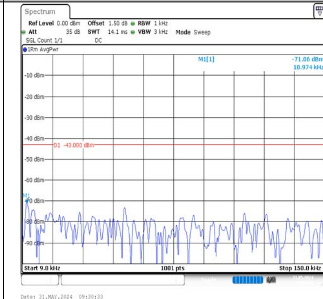
Band2-20MHz-QPSK-18700-100RB#0-0.009~0.15-PASS
