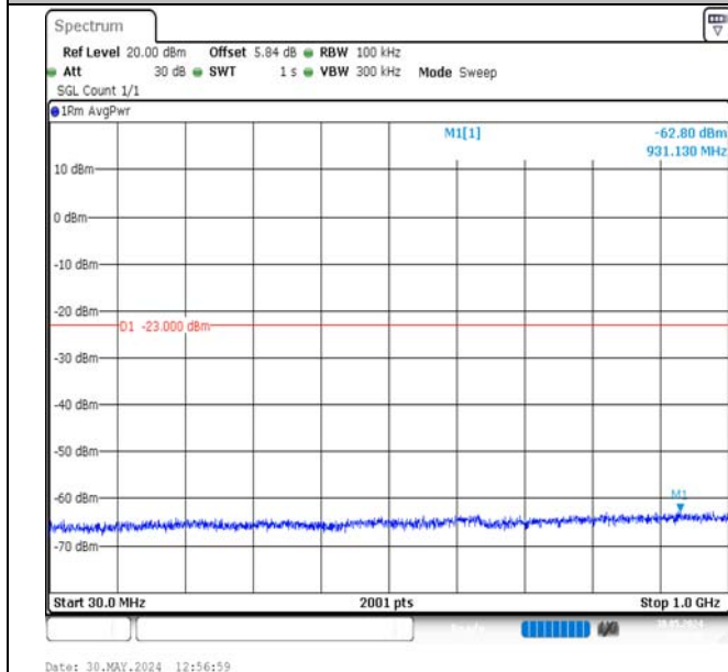
Band2-15MHz-QPSK-18900-75RB#0-30~1000-PASS
