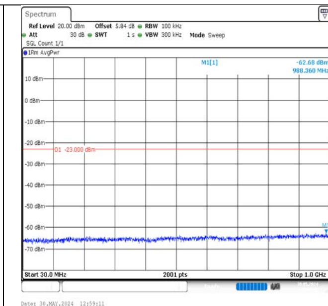
Band2-15MHz-QPSK-19125-75RB#0-30~1000-PASS
