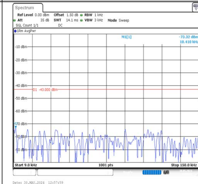
Band2-15MHz-16QAM-19125-1RB#0-0.009~0.15-PASS
