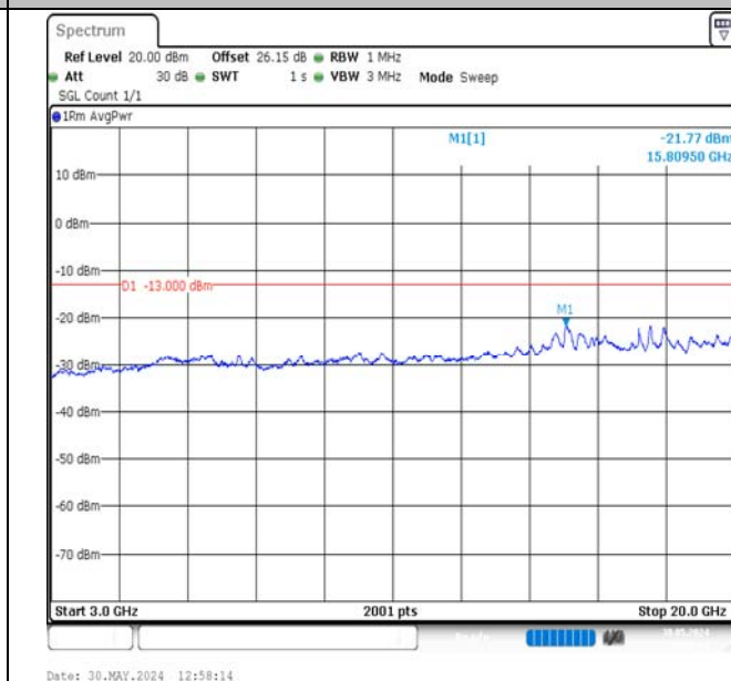
Band2-15MHz-16QAM-19125-1RB#0-3000~20000-PASS
