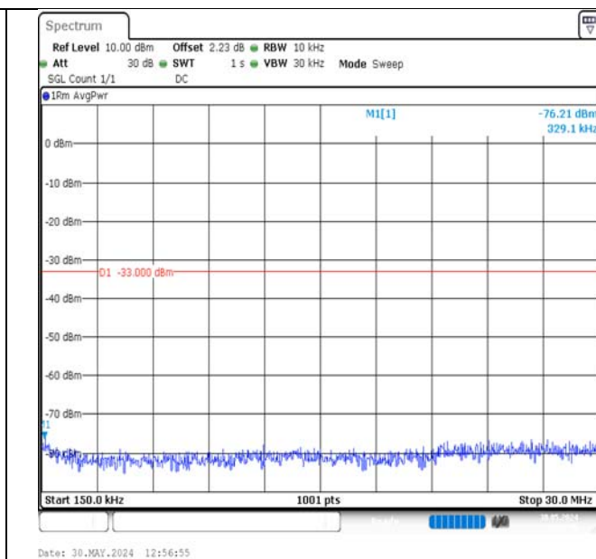
Band2-15MHz-QPSK-18900-75RB#0-0.15~30-PASS
