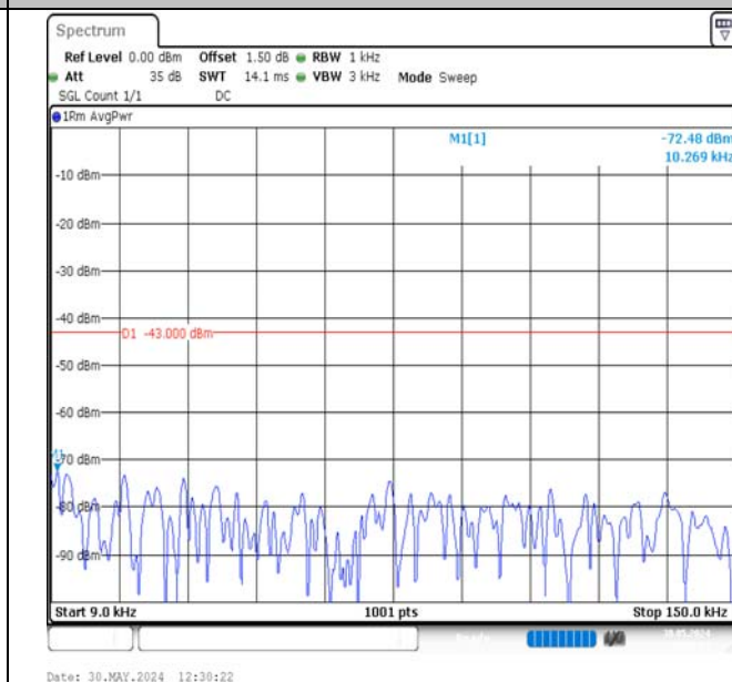
Band2-10MHz-16QAM-18900-50RB#0-0.009~0.15-PASS
