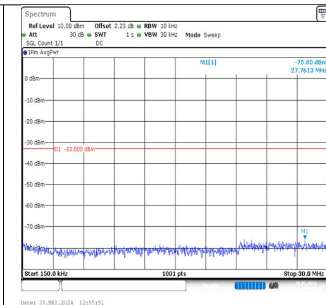
Band2-15MHz-16QAM-18900-1RB#0-0.15~30-PASS
