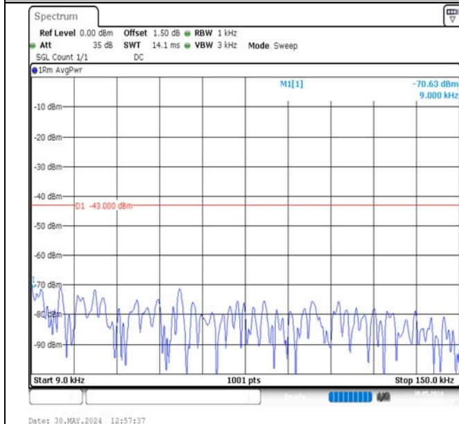
Band2-15MHz-QPSK-19125-1RB#0-0.009~0.15-PASS
