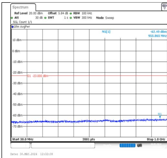
Band2-10MHz-16QAM-19150-50RB#0-30~1000-PASS
