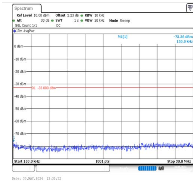
Band2-10MHz-16QAM-19150-1RB#49-0.15~30-PASS
