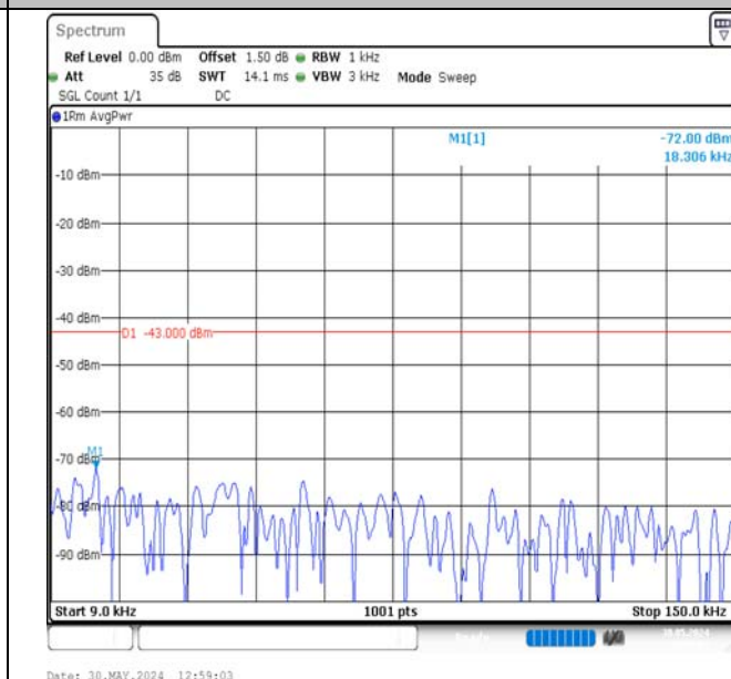
Band2-15MHz-QPSK-19125-75RB#0-0.009~0.15-PASS
