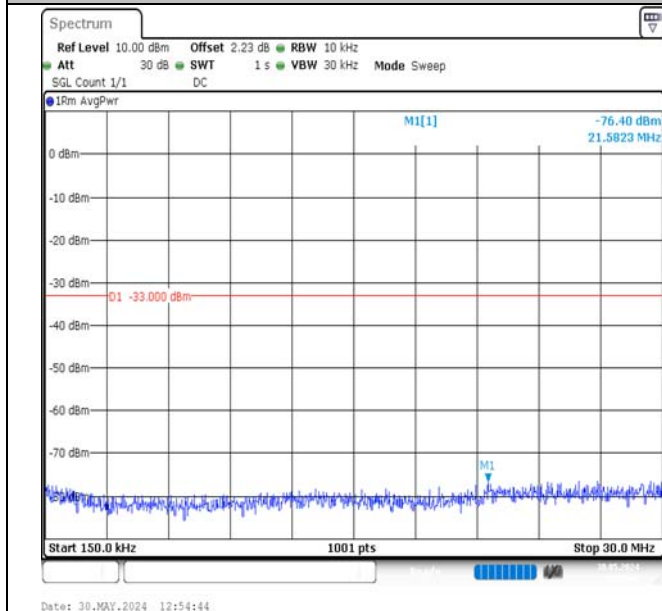
Band2-15MHz-QPSK-18675-75RB#0-0.15~30-PASS
