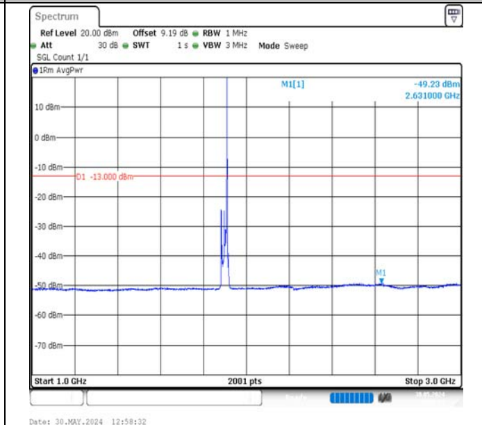
Band2-15MHz-QPSK-19125-1RB#74-1000~3000-PASS
