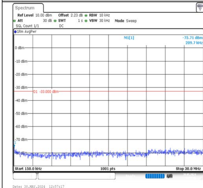
Band2-15MHz-16QAM-18900-75RB#0-0.15~30-PASS
