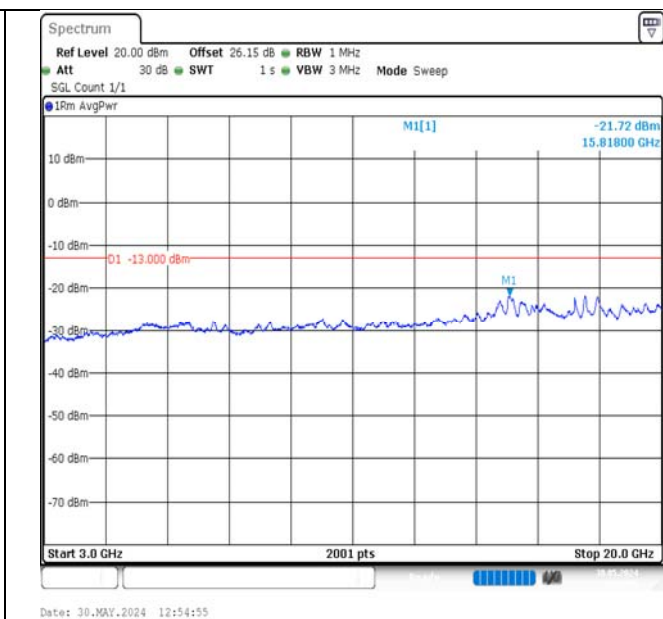
Band2-15MHz-QPSK-18675-75RB#0-3000~20000-PASS
