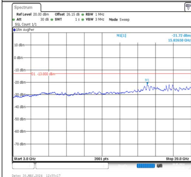
Band2-15MHz-16QAM-18675-75RB#0-3000~20000-PASS
