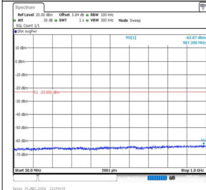
Band2-15MHz-16QAM-19125-75RB#0-30~1000-PASS
