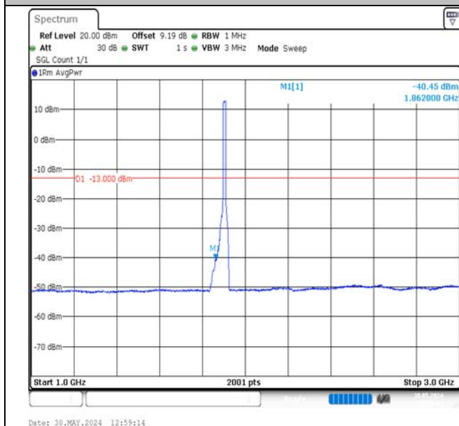
Band2-15MHz-QPSK-19125-75RB#0-1000~3000-PASS
