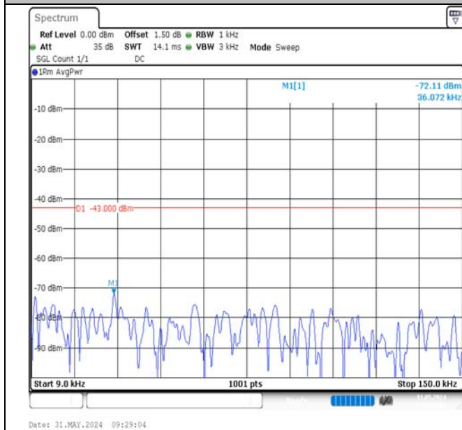
Band2-20MHz-QPSK-18700-1RB#0-0.009~0.15-PASS
