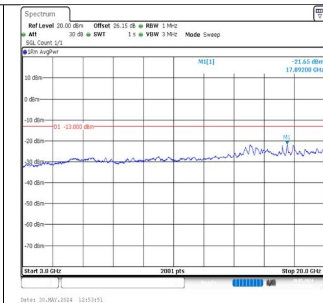
Band2-15MHz-16QAM-18675-1RB#0-3000~20000-PASS
