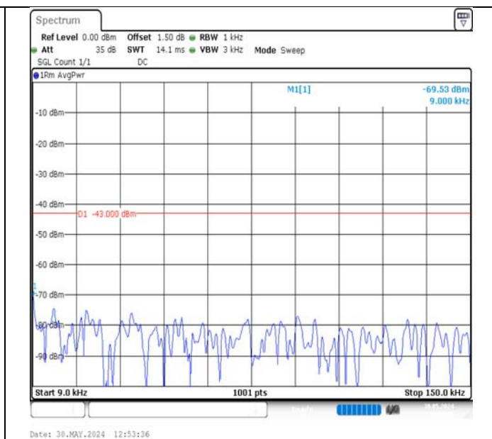
Band2-15MHz-16QAM-18675-1RB#0-0.009~0.15-PASS
