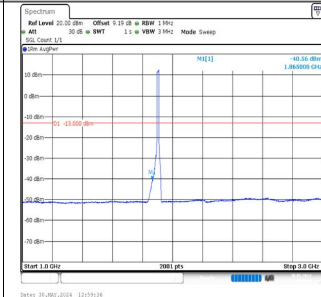
Band2-15MHz-16QAM-19125-75RB#0-1000~3000-PASS
