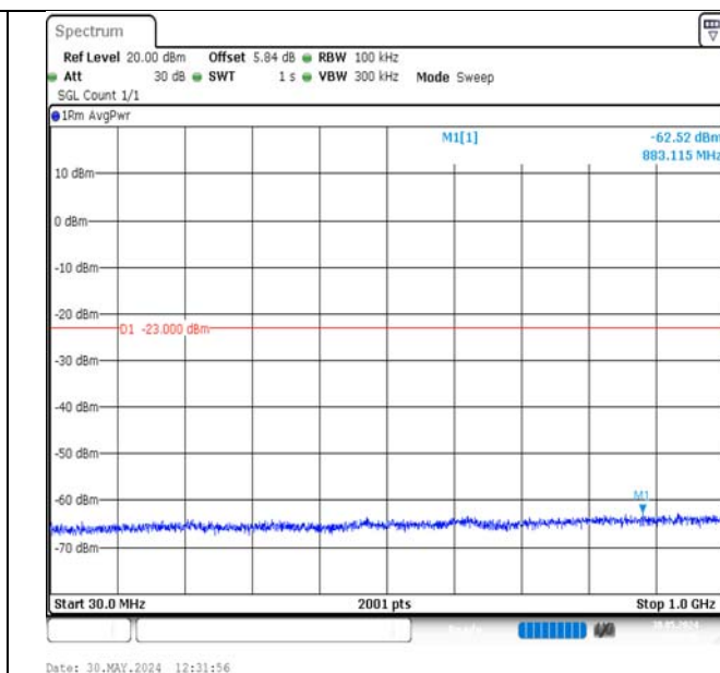
Band2-10MHz-16QAM-19150-1RB#49-30~1000-PASS
