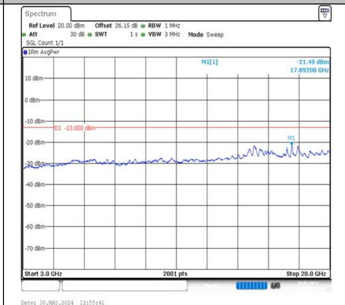
Band2-15MHz-QPSK-18900-1RB#0-3000~20000-PASS
