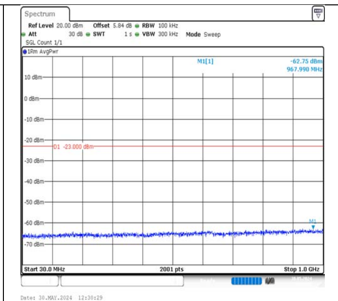
Band2-10MHz-16QAM-18900-50RB#0-30~1000-PASS
