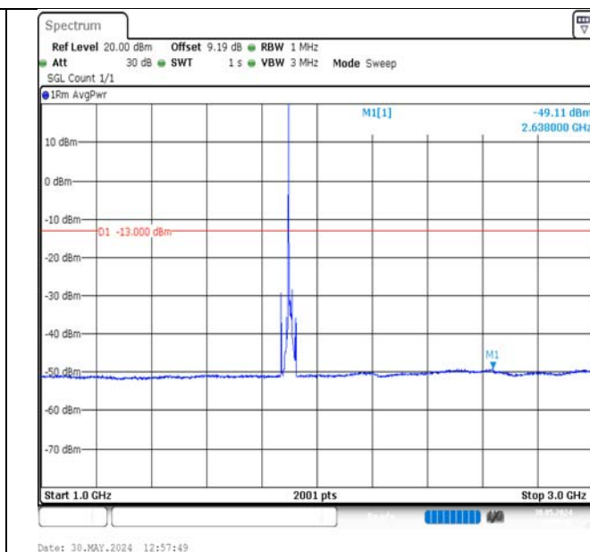
Band2-15MHz-QPSK-19125-1RB#0-1000~3000-PASS
