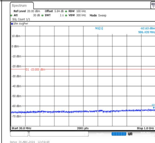
Band2-15MHz-QPSK-18675-75RB#0-30~1000-PASS
