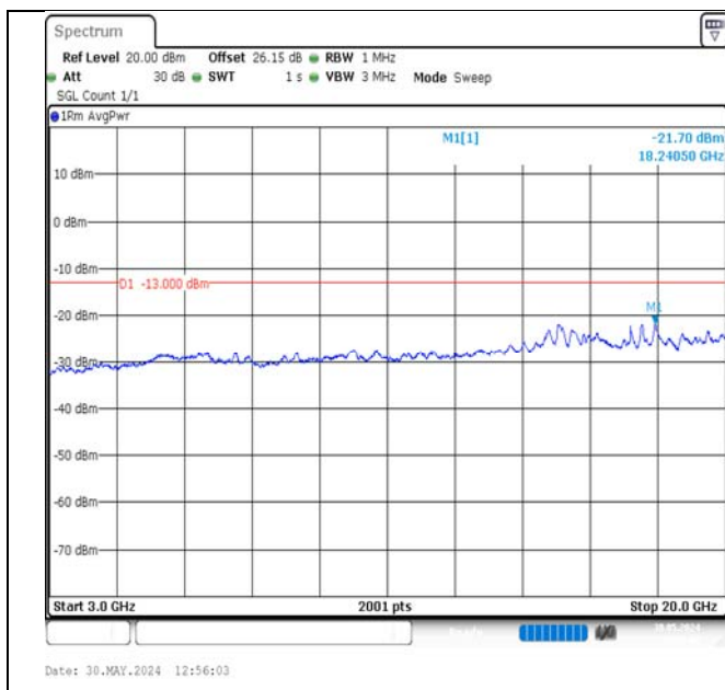
Band2-15MHz-16QAM-18900-1RB#0-3000~20000-PASS
