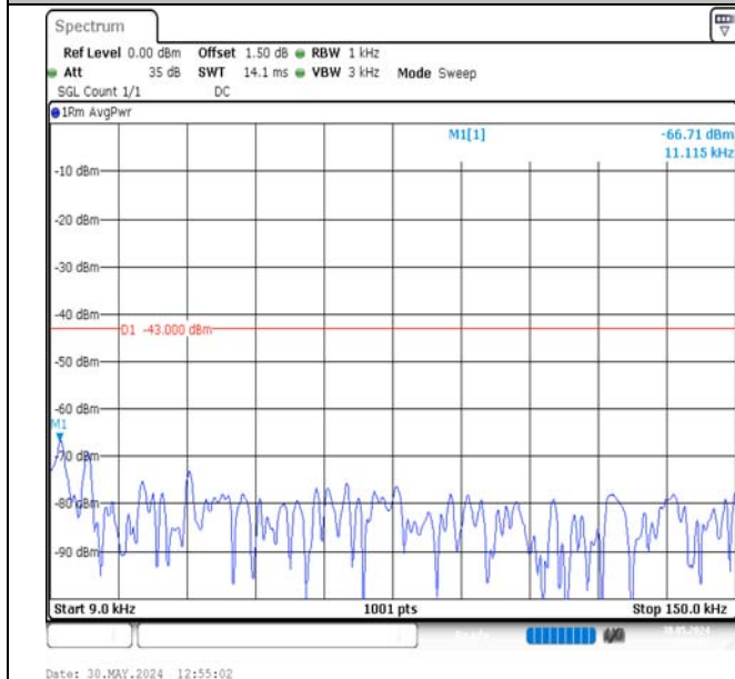
Band2-15MHz-16QAM-18675-75RB#0-0.009~0.15-PASS
