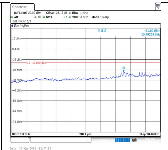
Band2-15MHz-16QAM-18900-75RB#0-3000~20000-PASS
