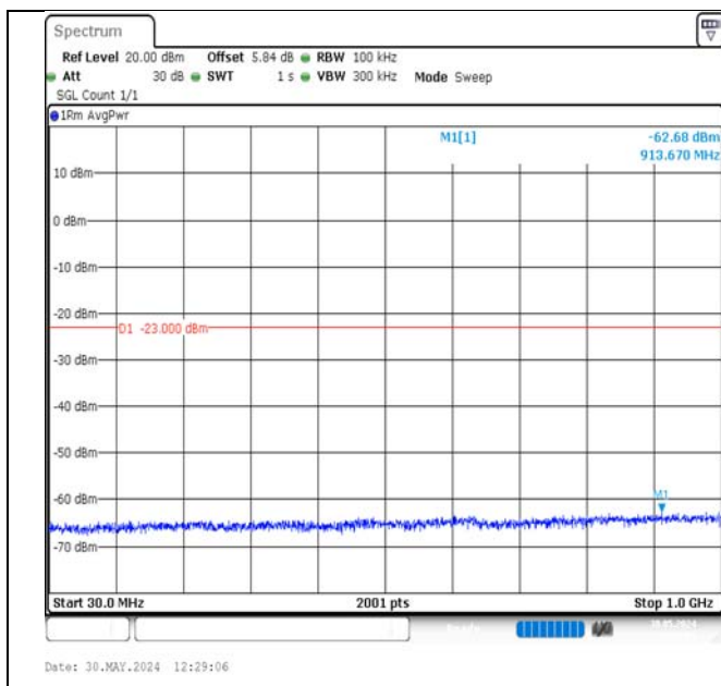
Band2-10MHz-16QAM-18900-1RB#0-30~1000-PASS
