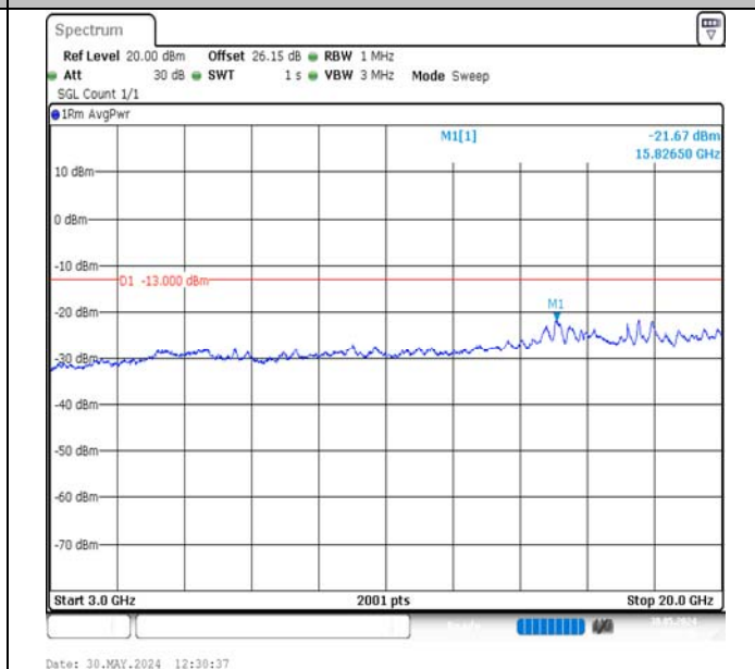
Band2-10MHz-16QAM-18900-50RB#0-3000~20000-PASS
