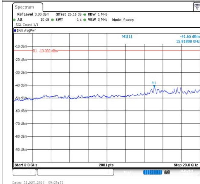
Band2-20MHz-QPSK-18700-1RB#0-3000~20000-PASS
