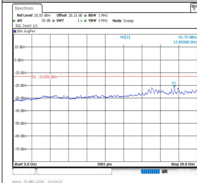
Band2-15MHz-QPSK-18675-1RB#74-3000~20000-PASS
