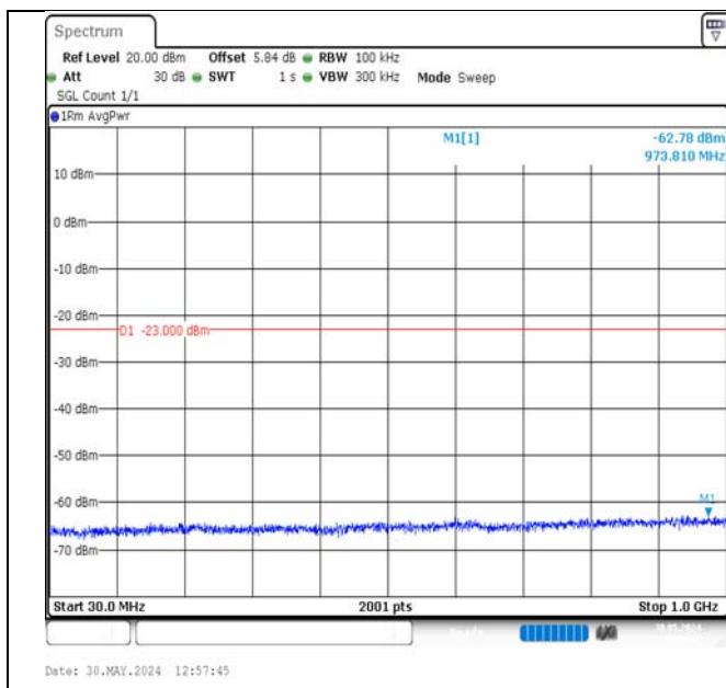
Band2-15MHz-QPSK-19125-1RB#0-30~1000-PASS
