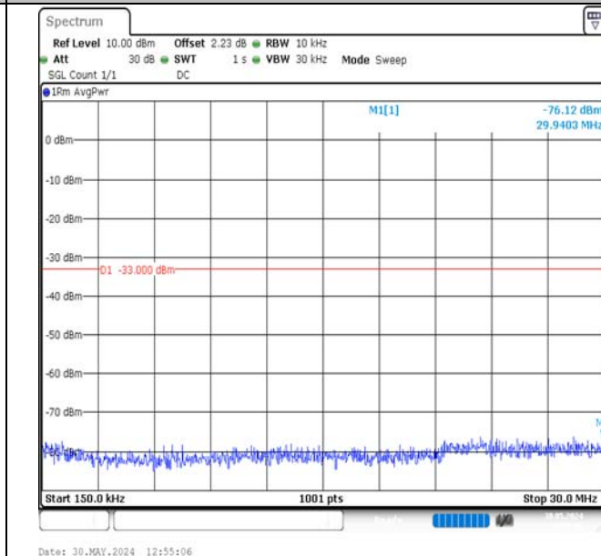
Band2-15MHz-16QAM-18675-75RB#0-0.15~30-PASS
