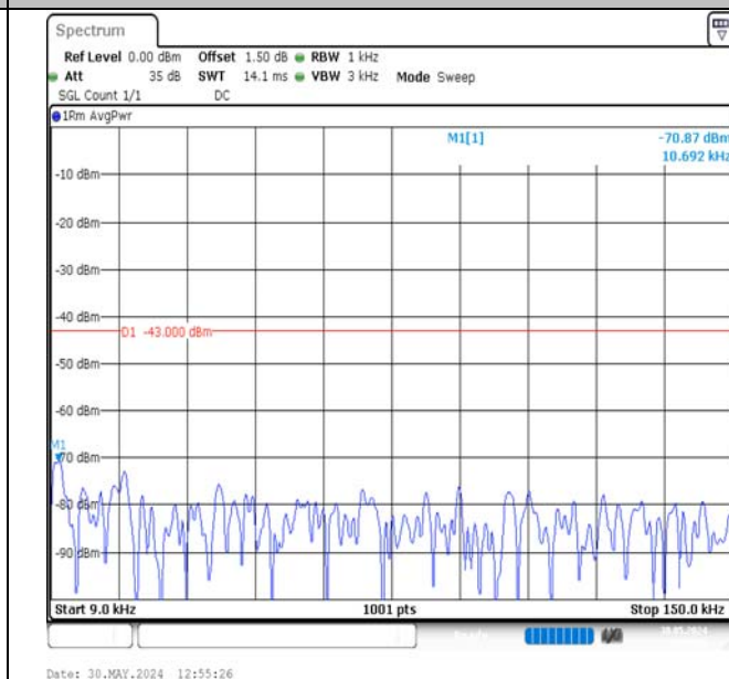
Band2-15MHz-QPSK-18900-1RB#0-0.009~0.15-PASS
