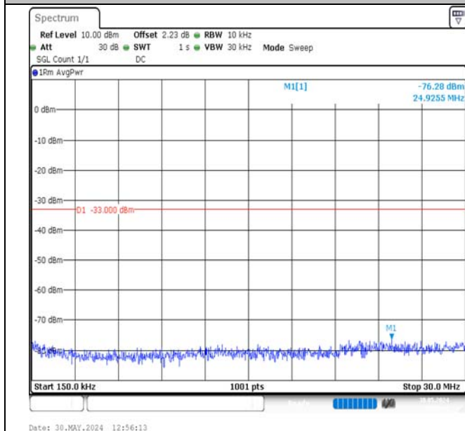
Band2-15MHz-QPSK-18900-1RB#74-0.15~30-PASS
