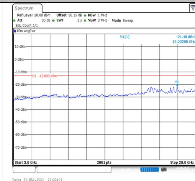
Band2-10MHz-16QAM-19150-1RB#49-3000~20000-PASS
