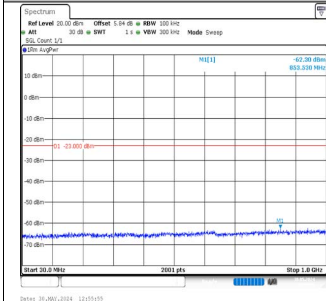
Band2-15MHz-16QAM-18900-1RB#0-30~1000-PASS
