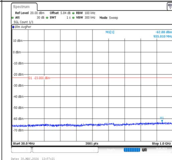
Band2-15MHz-16QAM-18900-75RB#0-30~1000-PASS
