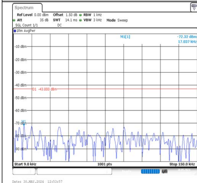
Band2-15MHz-QPSK-18675-1RB#74-0.009~0.15-PASS
