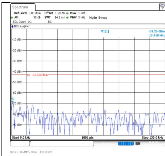
Band2-15MHz-16QAM-19125-75RB#0-0.009~0.15-PASS
