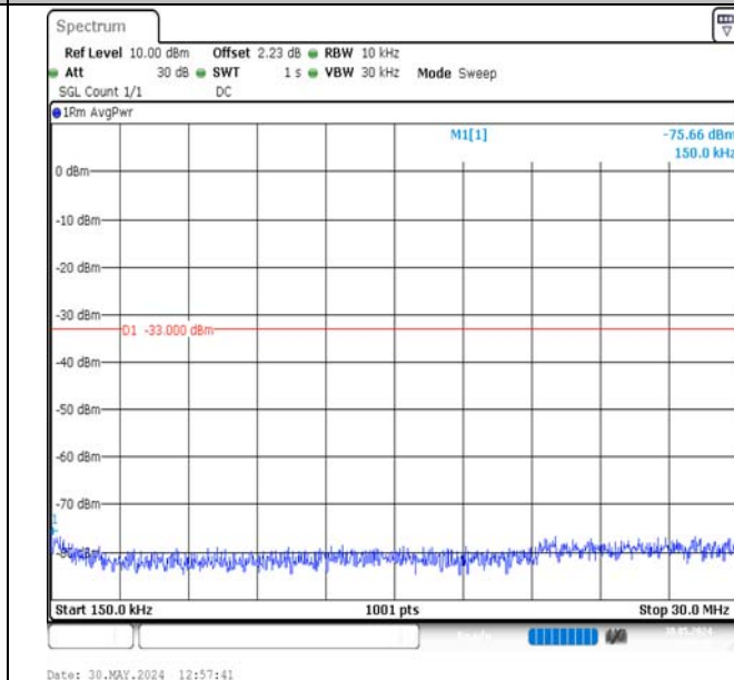
Band2-15MHz-QPSK-19125-1RB#0-0.15~30-PASS
