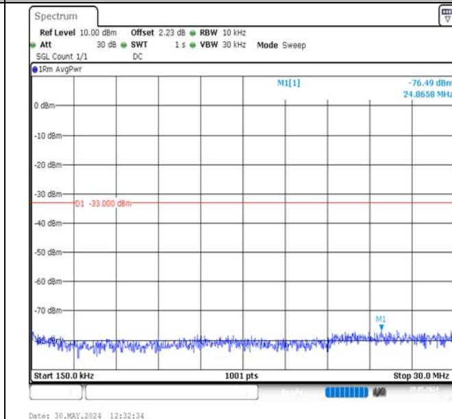
Band2-10MHz-16QAM-19150-50RB#0-0.15~30-PASS
