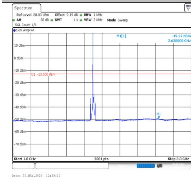
Band2-15MHz-16QAM-19125-1RB#0-1000~3000-PASS
