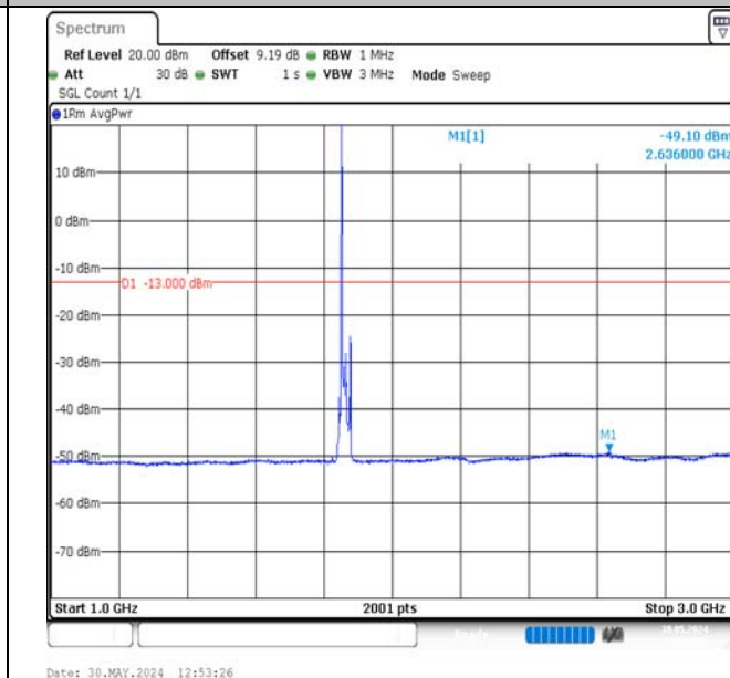
Band2-15MHz-QPSK-18675-1RB#0-1000~3000-PASS
