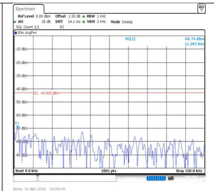
Band2-15MHz-QPSK-18900-1RB#74-0.009~0.15-PASS
