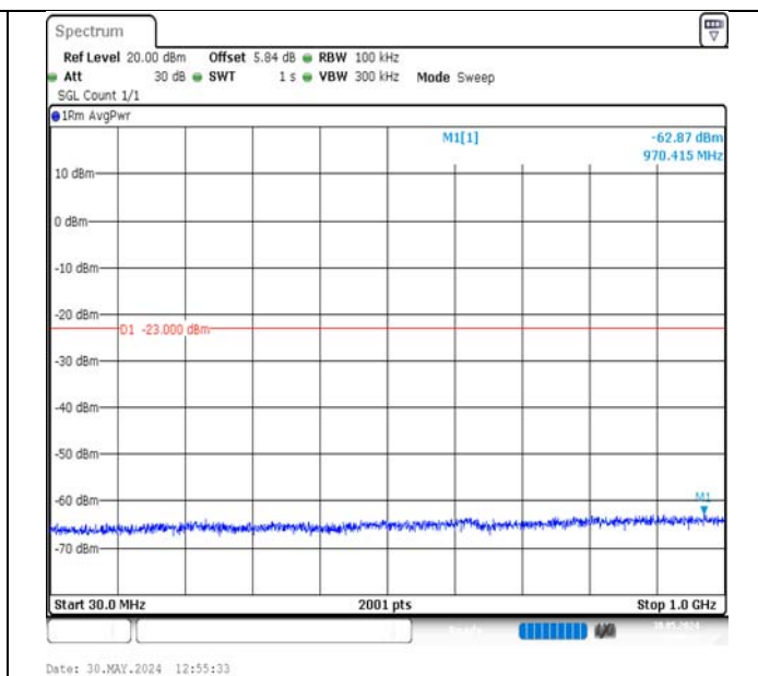
Band2-15MHz-QPSK-18900-1RB#0-30~1000-PASS
