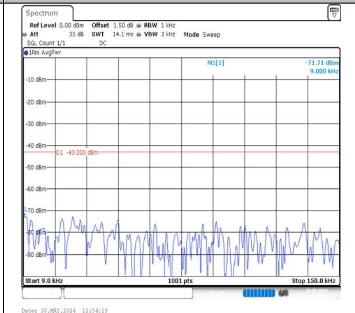
Band2-15MHz-16QAM-18675-1RB#74-0.009~0.15-PASS
