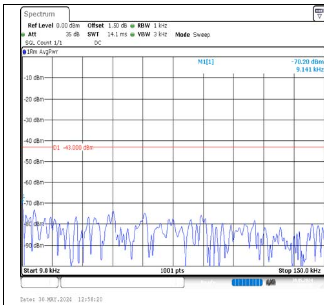
Band2-15MHz-QPSK-19125-1RB#74-0.009~0.15-PASS
