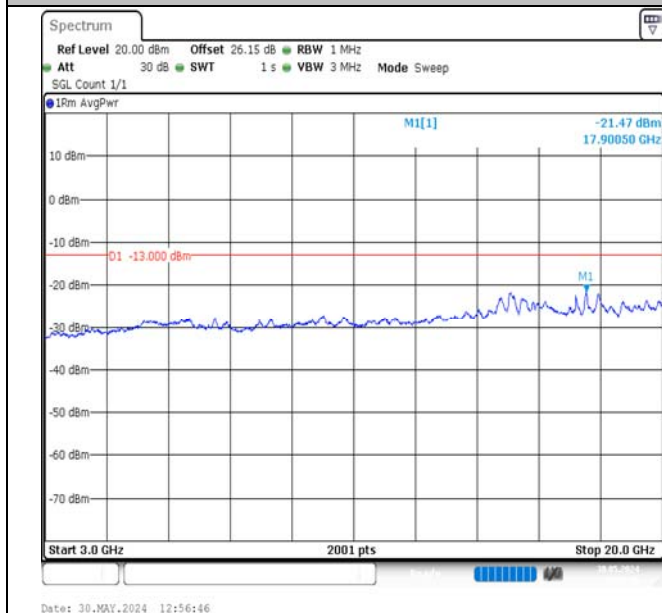
Band2-15MHz-16QAM-18900-1RB#74-3000~20000-PASS
