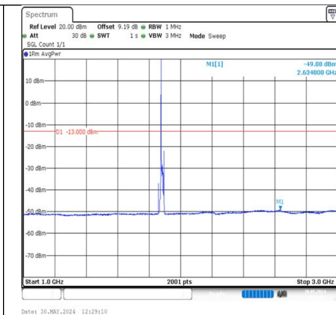
Band2-10MHz-16QAM-18900-1RB#0-1000~3000-PASS
