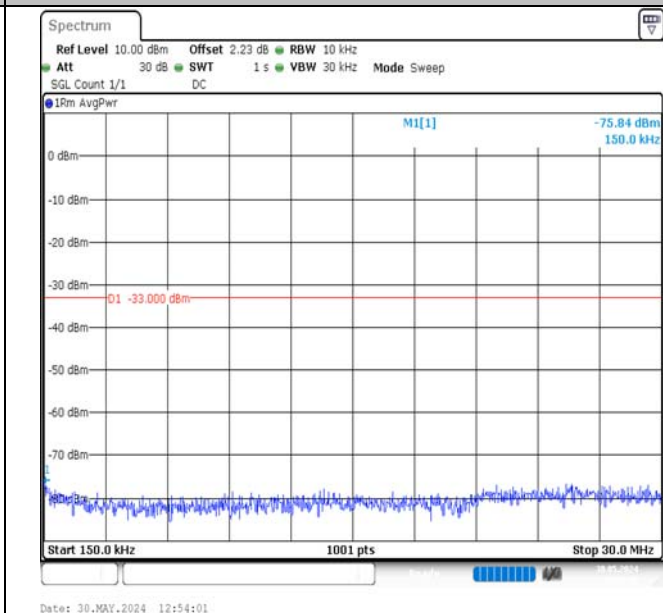
Band2-15MHz-QPSK-18675-1RB#74-0.15~30-PASS
