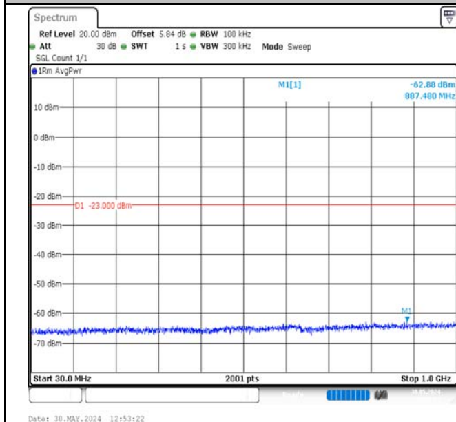
Band2-15MHz-QPSK-18675-1RB#0-30~1000-PASS
