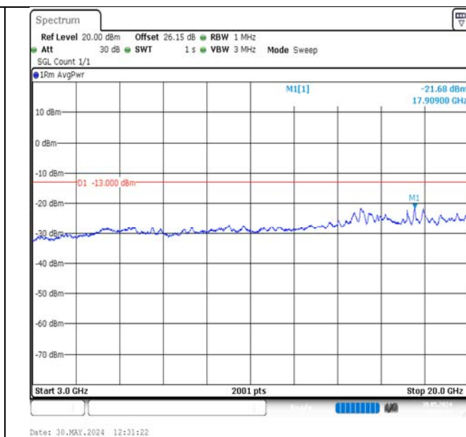
Band2-10MHz-16QAM-19150-1RB#0-3000~20000-PASS
