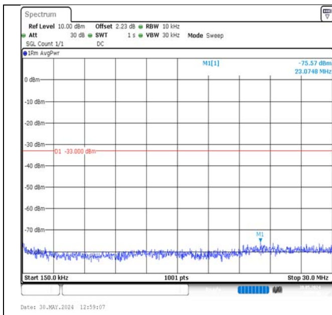
Band2-15MHz-QPSK-19125-75RB#0-0.15~30-PASS
