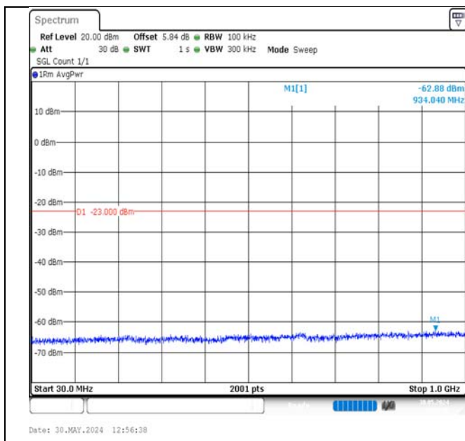
Band2-15MHz-16QAM-18900-1RB#74-30~1000-PASS
