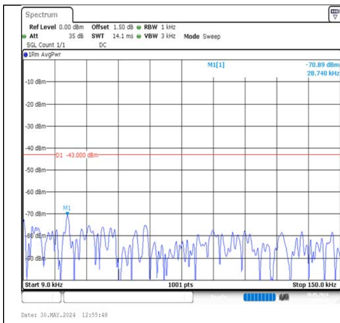
Band2-15MHz-16QAM-18900-1RB#0-0.009~0.15-PASS
