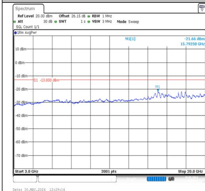
Band2-10MHz-16QAM-18900-1RB#0-3000~20000-PASS
