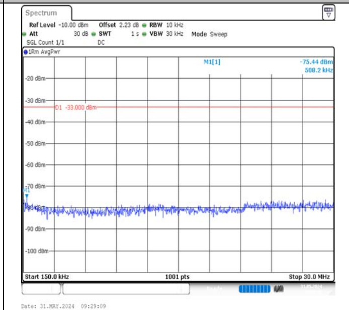
Band2-20MHz-QPSK-18700-1RB#0-0.15~30-PASS
