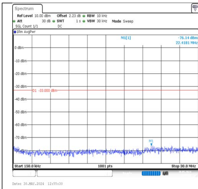
Band2-15MHz-QPSK-18900-1RB#0-0.15~30-PASS
