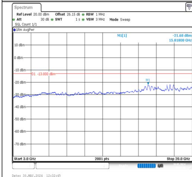
Band2-10MHz-16QAM-19150-50RB#0-3000~20000-PASS
