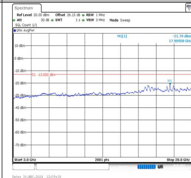
Band2-15MHz-QPSK-19125-75RB#0-3000~20000-PASS
