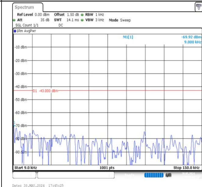
Band4-15MHz-QPSK-20325-75RB#0-0.009~0.15-PASS
