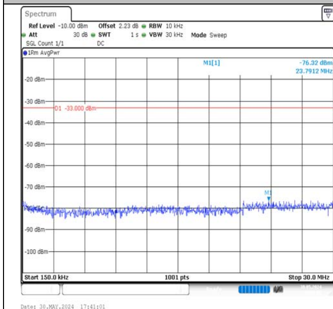
Band4-15MHz-QPSK-20025-75RB#0-0.15~30-PASS
