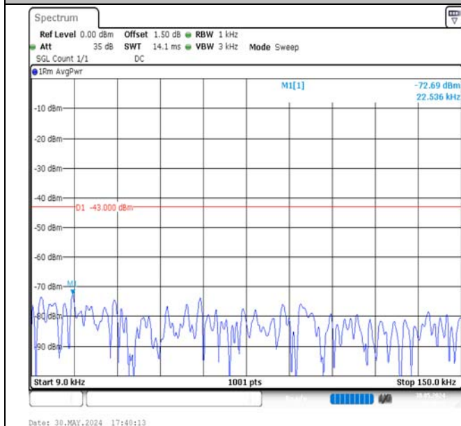
Band4-15MHz-QPSK-20025-1RB#74-0.009~0.15-PASS
