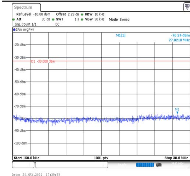
Band4-15MHz-16QAM-20025-1RB#0-0.15~30-PASS
