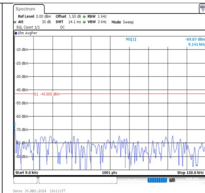
Band4-10MHz-QPSK-20350-50RB#0-0.009~0.15-PASS
