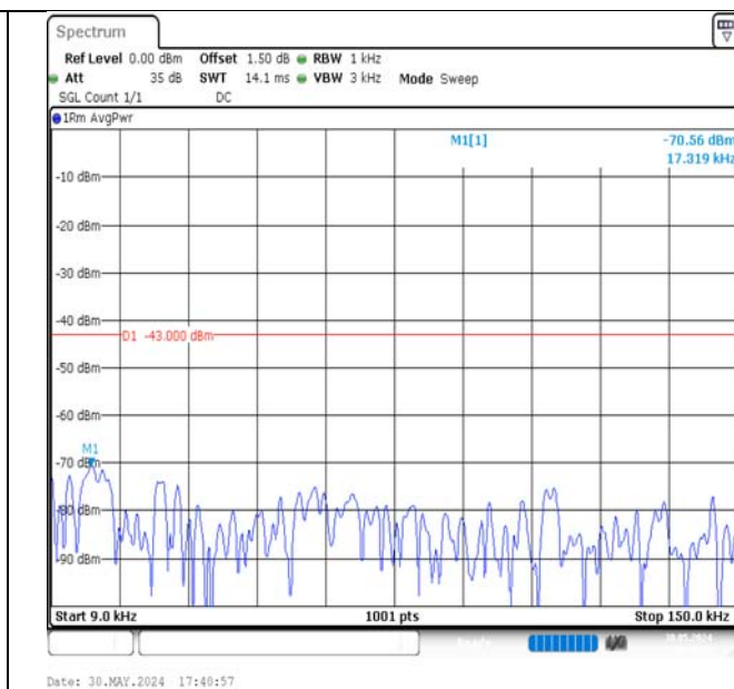
Band4-15MHz-QPSK-20025-75RB#0-0.009~0.15-PASS
