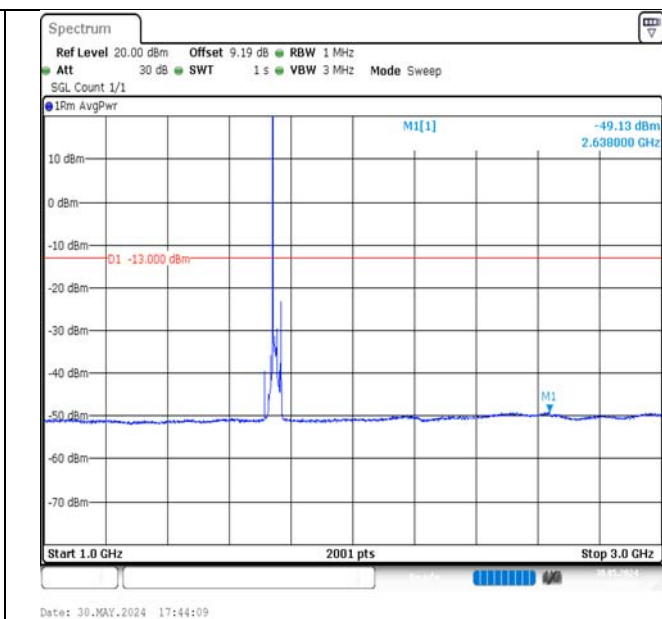
Band4-15MHz-QPSK-20325-1RB#0-1000~3000-PASS
