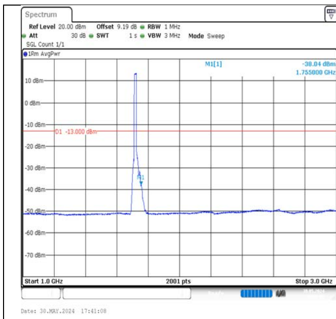
Band4-15MHz-QPSK-20025-75RB#0-1000~3000-PASS
