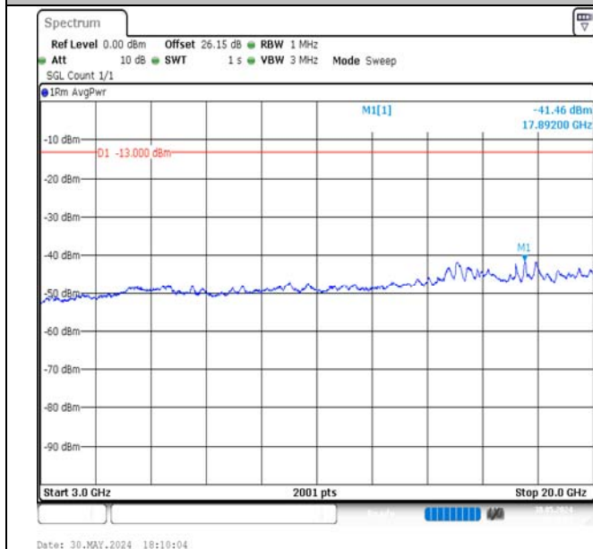
Band4-10MHz-QPSK-20175-50RB#0-3000~20000-PASS
