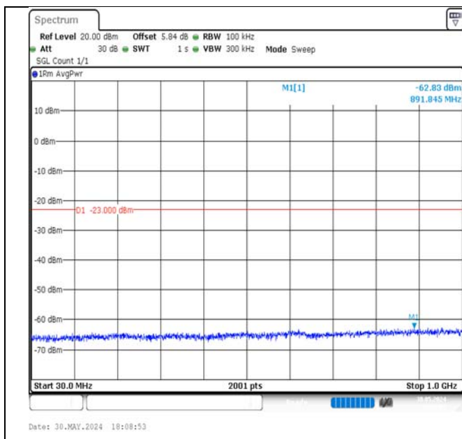
Band4-10MHz-16QAM-20175-1RB#0-30~1000-PASS
