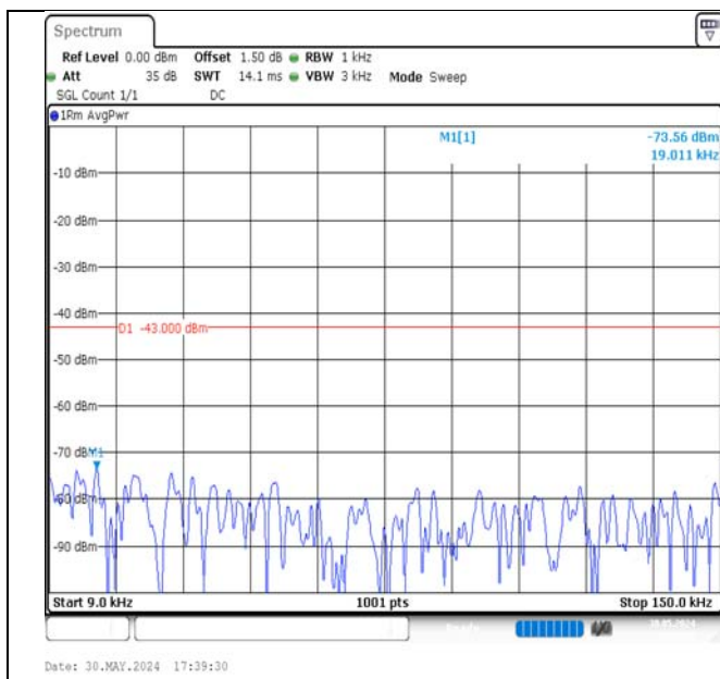
Band4-15MHz-QPSK-20025-1RB#0-0.009~0.15-PASS
