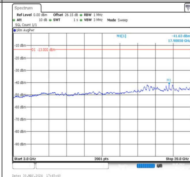
Band4-15MHz-QPSK-20325-75RB#0-3000~20000-PASS
