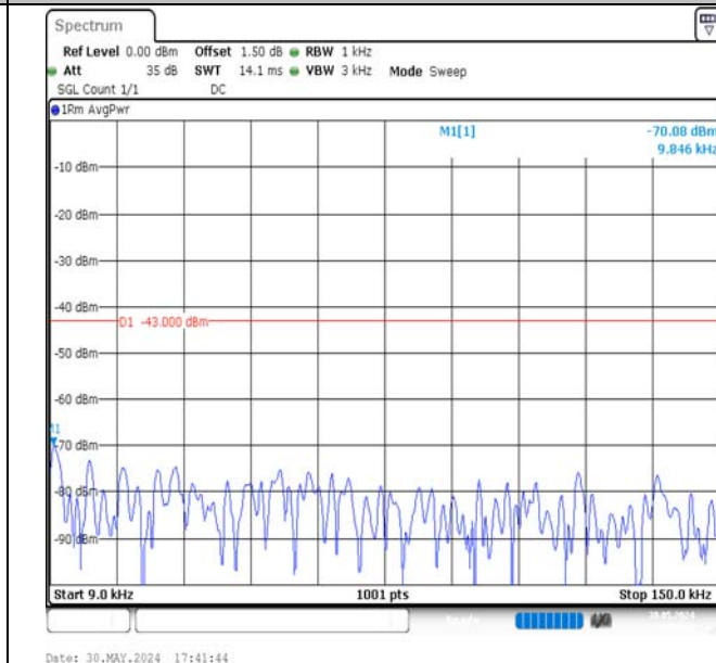
Band4-15MHz-QPSK-20175-1RB#0-0.009~0.15-PASS
