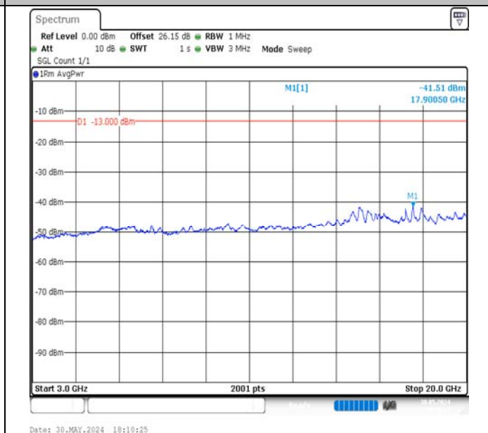
Band4-10MHz-16QAM-20175-50RB#0-3000~20000-PASS
