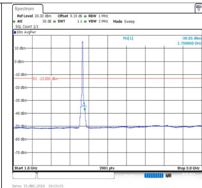
Band4-10MHz-QPSK-20175-50RB#0-1000~3000-PASS
