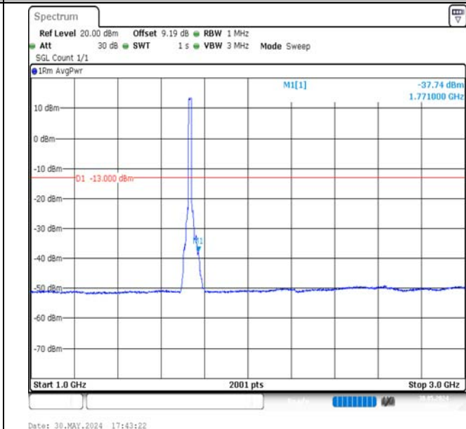
Band4-15MHz-QPSK-20175-75RB#0-1000~3000-PASS
