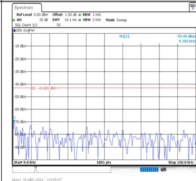
Band4-10MHz-QPSK-20175-1RB#49-0.009~0.15-PASS
