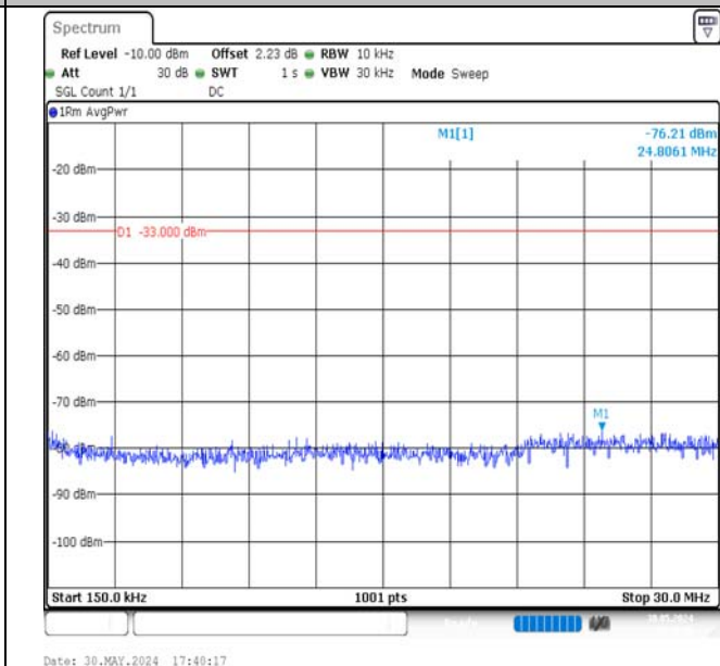
Band4-15MHz-QPSK-20025-1RB#74-0.15~30-PASS
