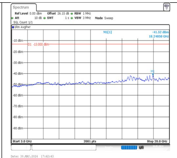
Band4-15MHz-QPSK-20175-1RB#74-3000~20000-PASS
