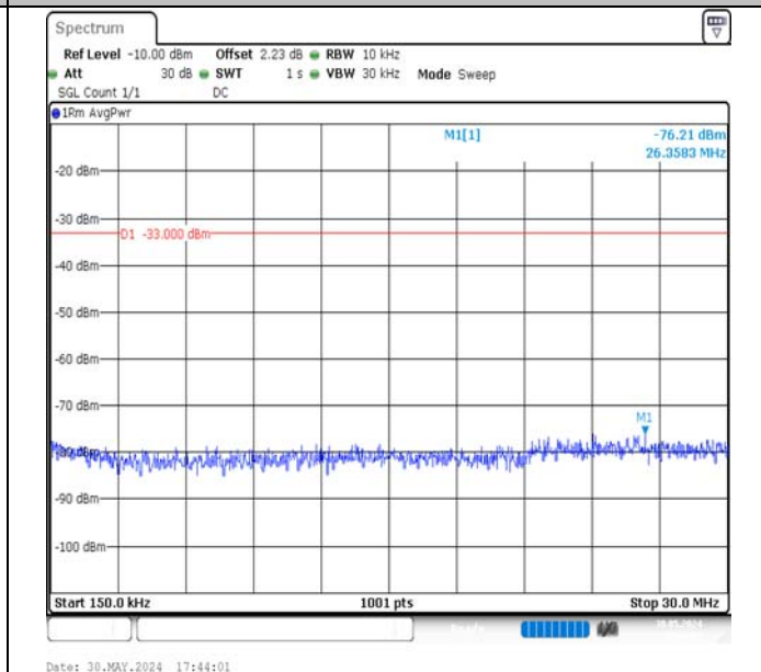
Band4-15MHz-QPSK-20325-1RB#0-0.15~30-PASS
