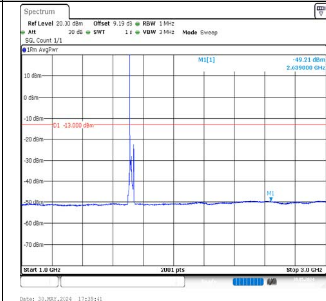
Band4-15MHz-QPSK-20025-1RB#0-1000~3000-PASS
