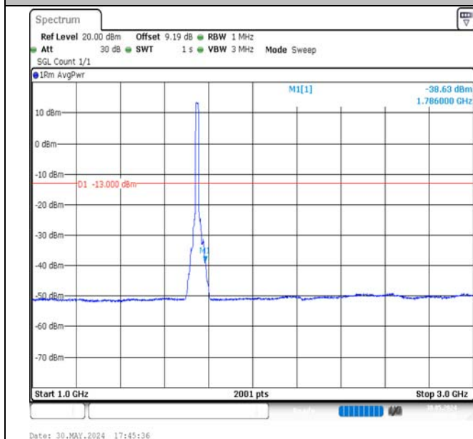
Band4-15MHz-QPSK-20325-75RB#0-1000~3000-PASS
