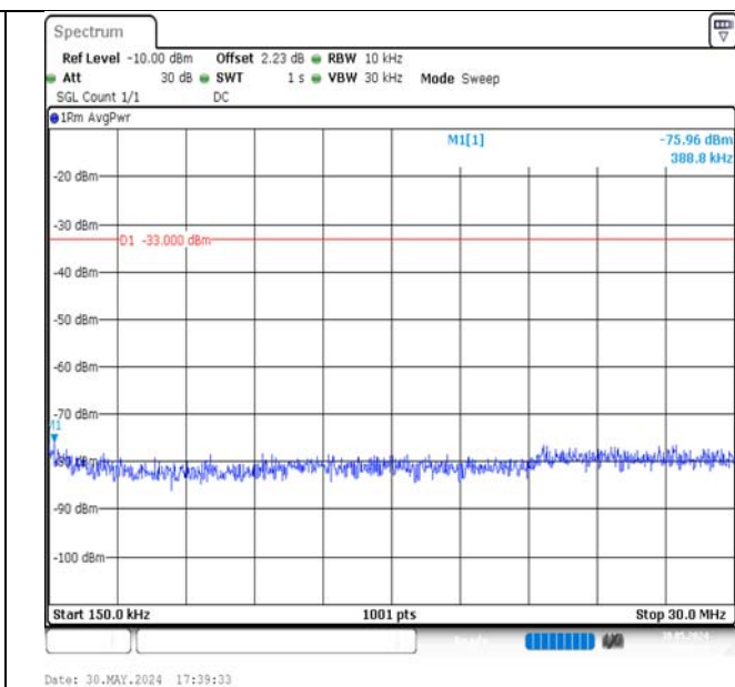
Band4-15MHz-QPSK-20025-1RB#0-0.15~30-PASS
