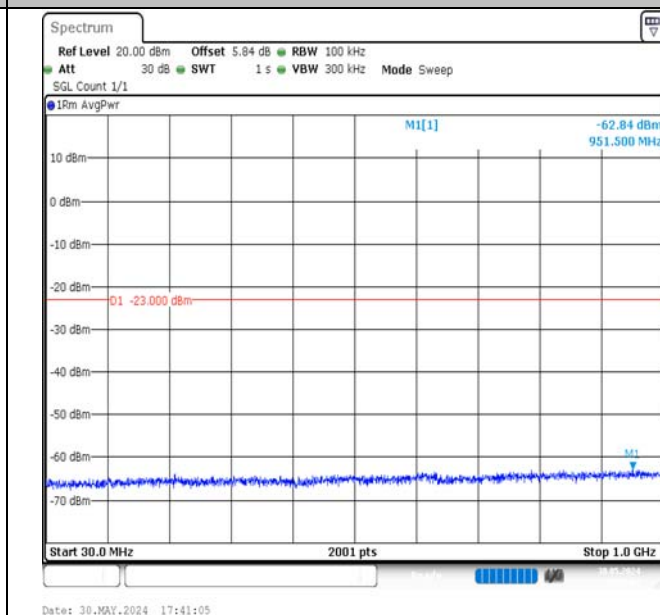
Band4-15MHz-QPSK-20025-75RB#0-30~1000-PASS
