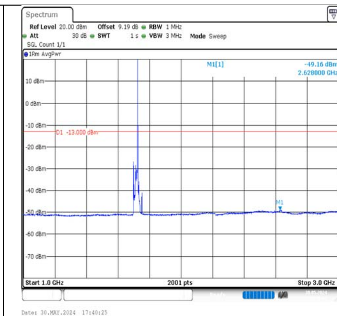
Band4-15MHz-QPSK-20025-1RB#74-1000~3000-PASS
