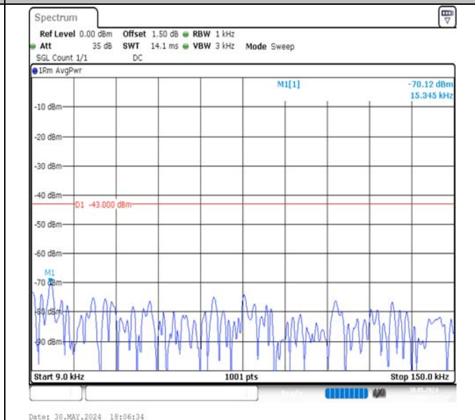
Band4-10MHz-16QAM-20000-1RB#0-0.009~0.15-PASS
