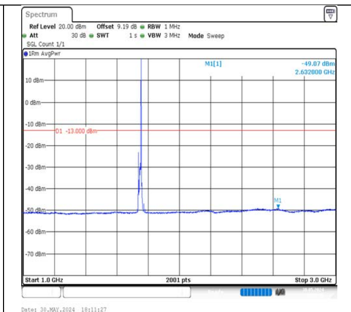
Band4-10MHz-QPSK-20350-1RB#49-1000~3000-PASS
