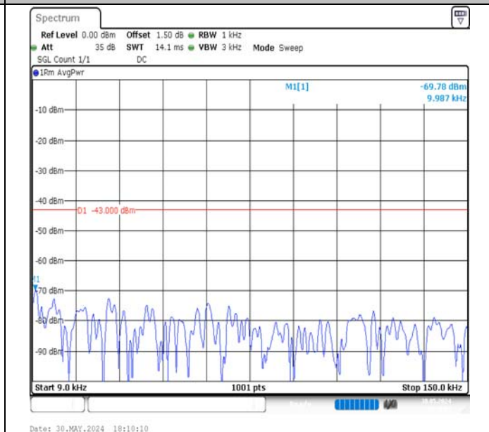
Band4-10MHz-16QAM-20175-50RB#0-0.009~0.15-PASS
