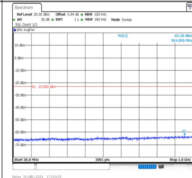
Band4-15MHz-16QAM-20025-1RB#0-30~1000-PASS
