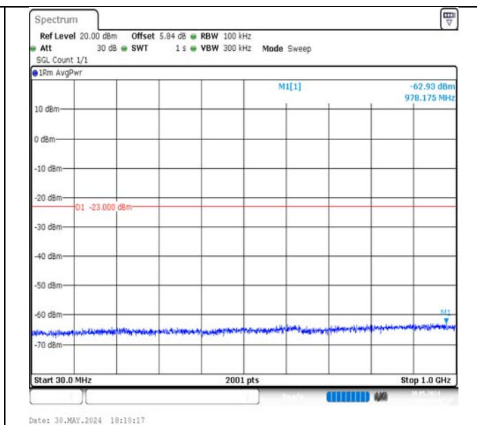
Band4-10MHz-16QAM-20175-50RB#0-30~1000-PASS
