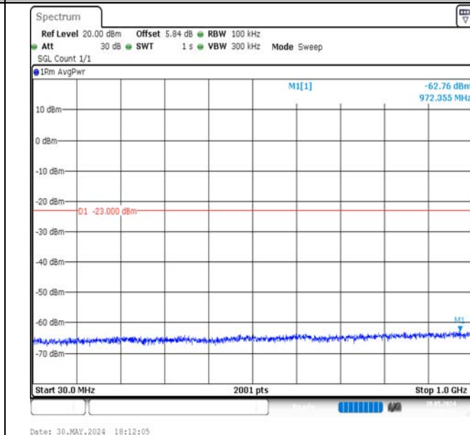
Band4-10MHz-QPSK-20350-50RB#0-30~1000-PASS
