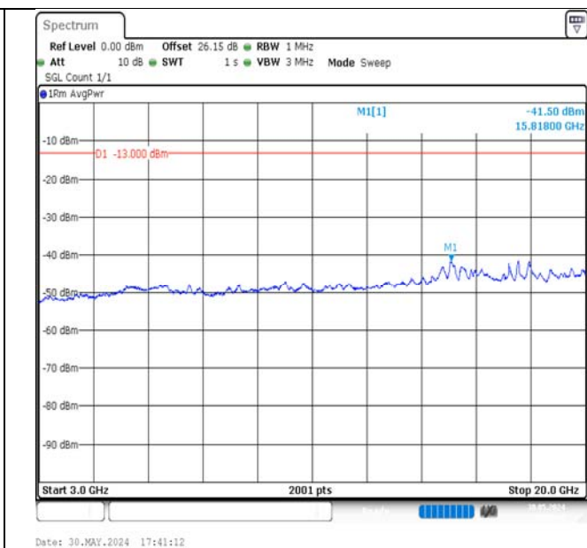
Band4-15MHz-QPSK-20025-75RB#0-3000~20000-PASS
