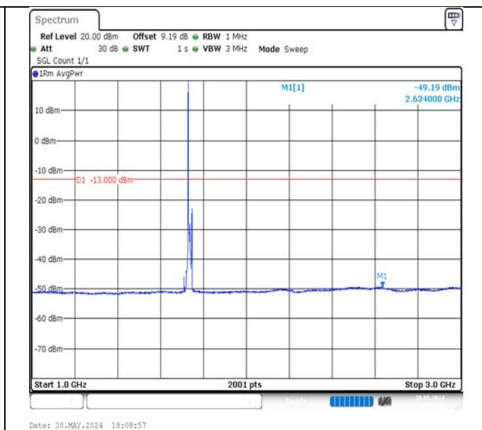
Band4-10MHz-16QAM-20175-1RB#0-1000~3000-PASS
