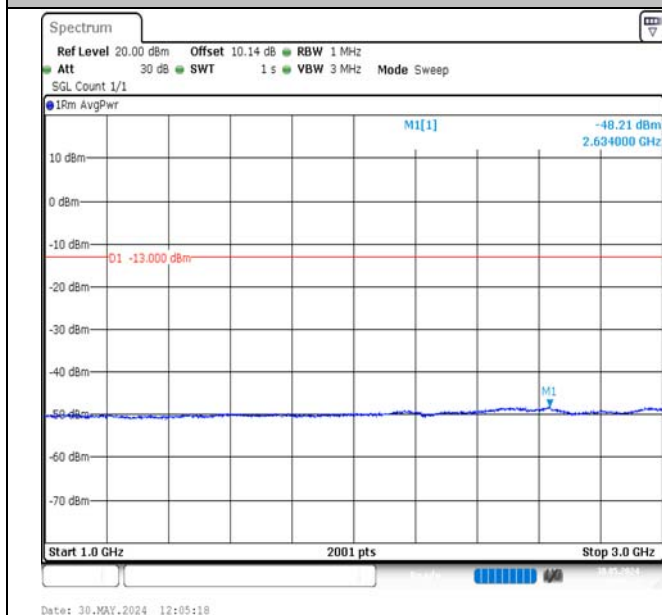
Band13-5MHz-QPSK-23255-25RB#0-1000~3000-PASS
