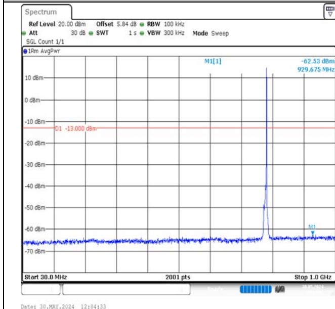
Band13-5MHz-QPSK-23255-1RB#24-30~1000-PASS
