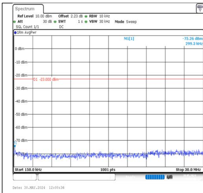
Band13-5MHz-16QAM-23205-1RB#24-0.15~30-PASS
