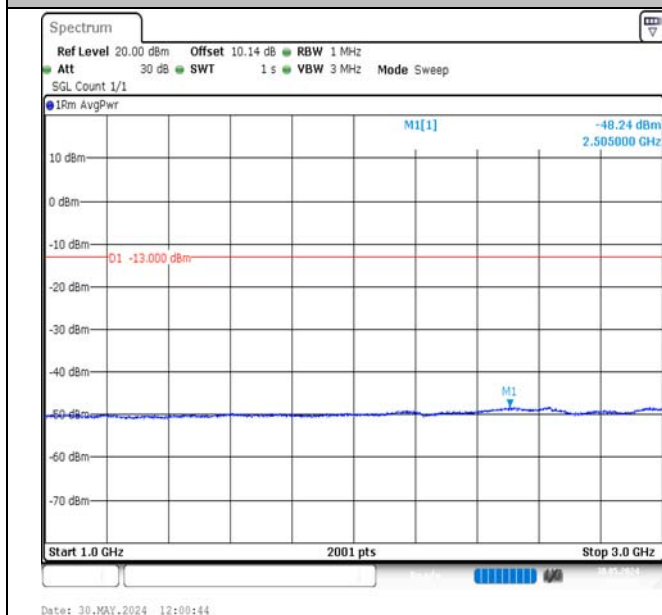
Band13-5MHz-16QAM-23205-1RB#24-1000~3000-PASS
