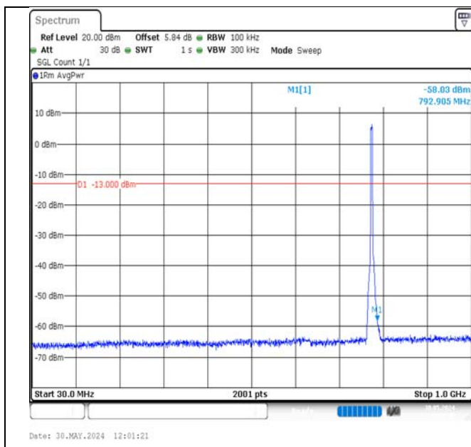
Band13-5MHz-16QAM-23205-25RB#0-30~1000-PASS
