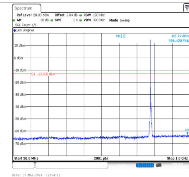
Band13-5MHz-16QAM-23255-1RB#0-30~1000-PASS
