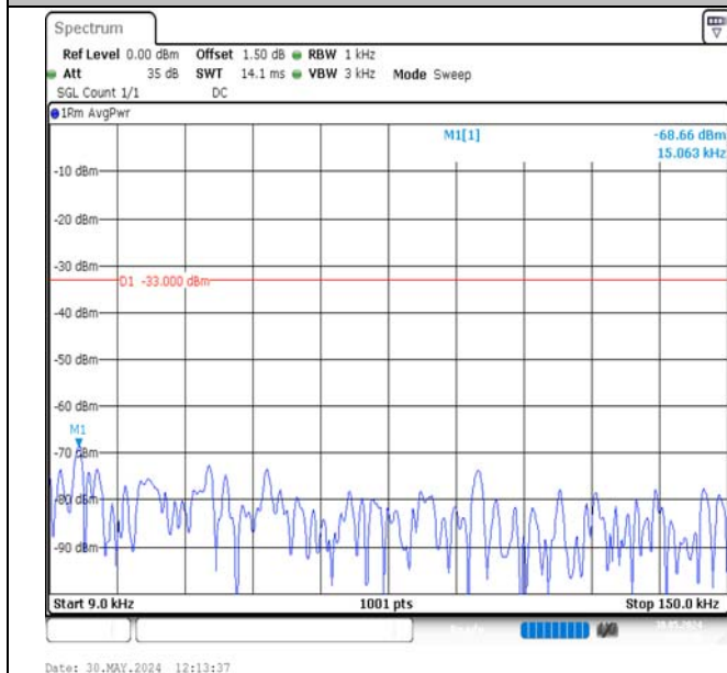
Band17-5MHz-QPSK-23755-1RB#24-0.009~0.15-PASS
