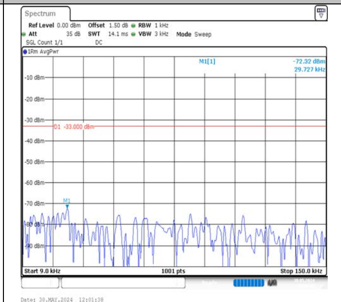
Band13-5MHz-QPSK-23230-1RB#0-0.009~0.15-PASS
