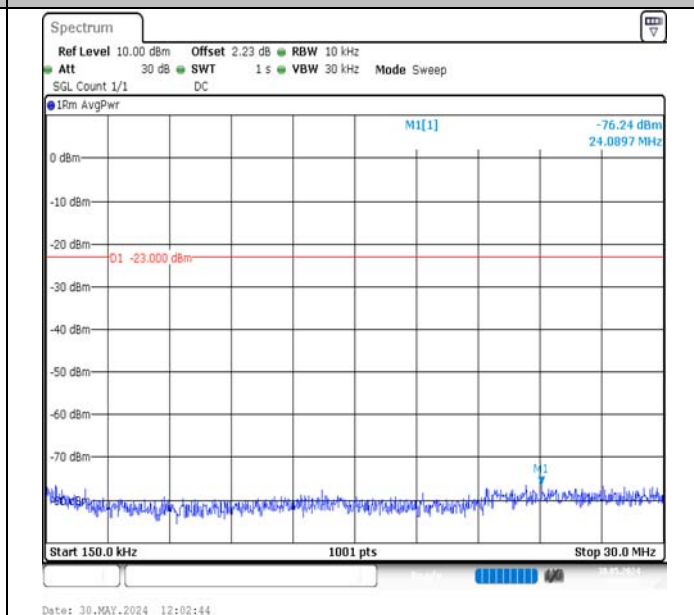
Band13-5MHz-16QAM-23230-1RB#24-0.15~30-PASS
