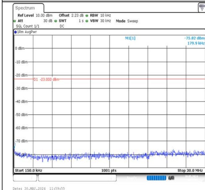
Band13-5MHz-16QAM-23205-1RB#0-0.15~30-PASS
