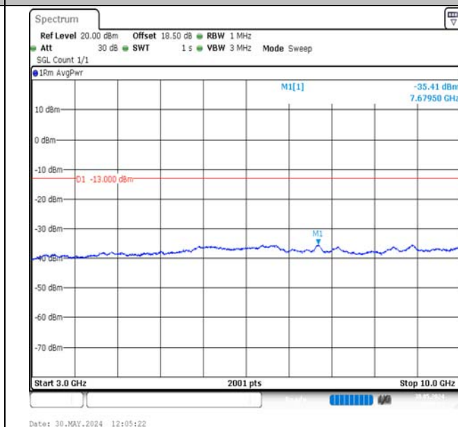
Band13-5MHz-QPSK-23255-25RB#0-3000~10000-PASS
