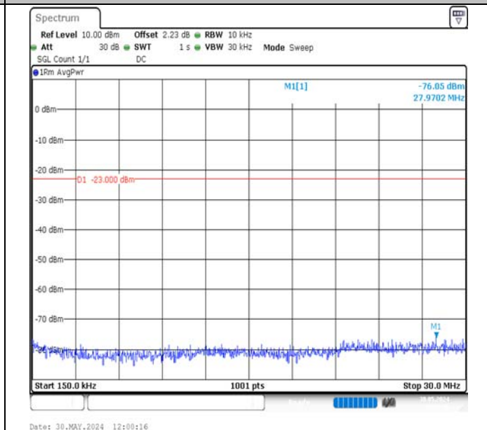
Band13-5MHz-QPSK-23205-1RB#24-0.15~30-PASS
