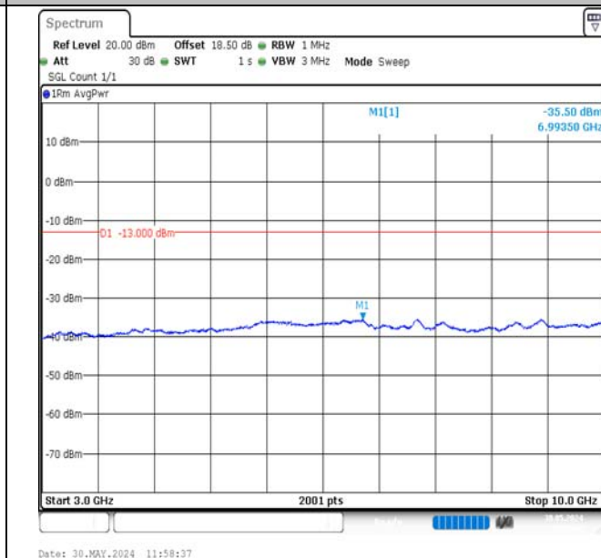
Band13-10MHz-16QAM-23230-1RB#49-3000~10000-PASS
