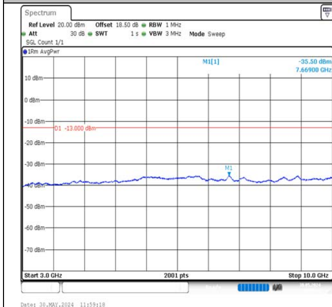
Band13-10MHz-16QAM-23230-50RB#0-3000~10000-PASS
