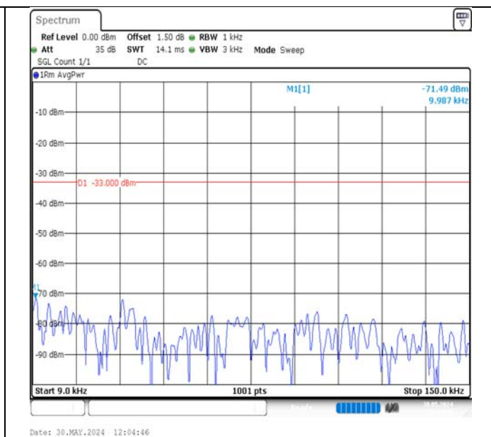
Band13-5MHz-16QAM-23255-1RB#24-0.009~0.15-PASS
