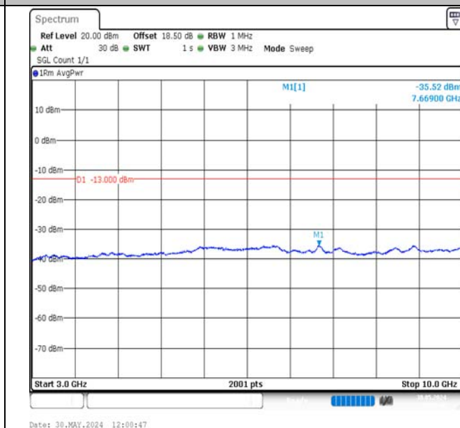
Band13-5MHz-16QAM-23205-1RB#24-3000~10000-PASS
