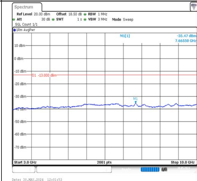
Band13-5MHz-QPSK-23230-1RB#0-3000~10000-PASS
