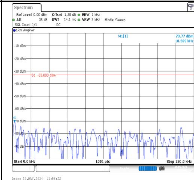
Band13-10MHz-16QAM-23230-1RB#49-0.009~0.15-PASS
