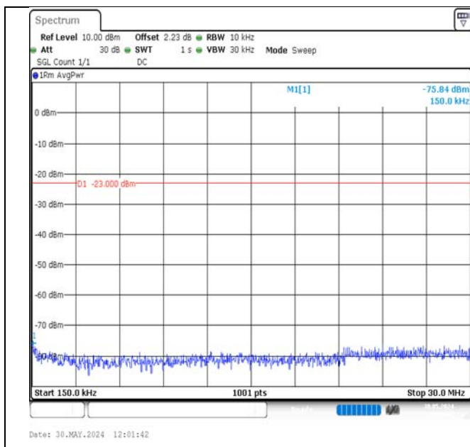
Band13-5MHz-QPSK-23230-1RB#0-0.15~30-PASS
