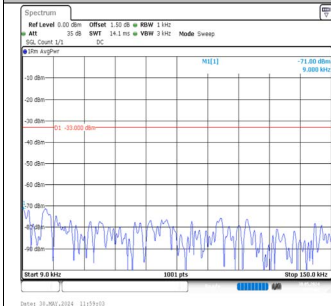
Band13-10MHz-16QAM-23230-50RB#0-0.009~0.15-PASS
