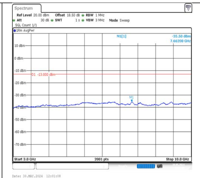
Band13-5MHz-QPSK-23205-25RB#0-3000~10000-PASS
