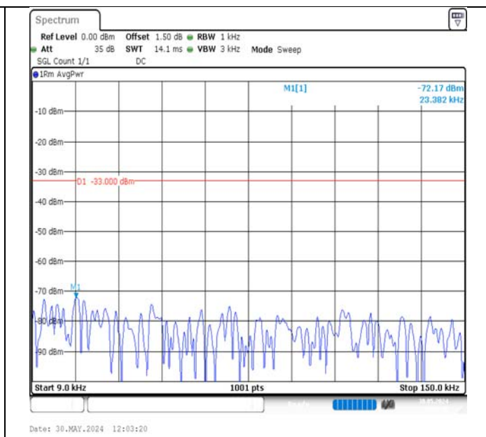
Band13-5MHz-16QAM-23230-25RB#0-0.009~0.15-PASS
