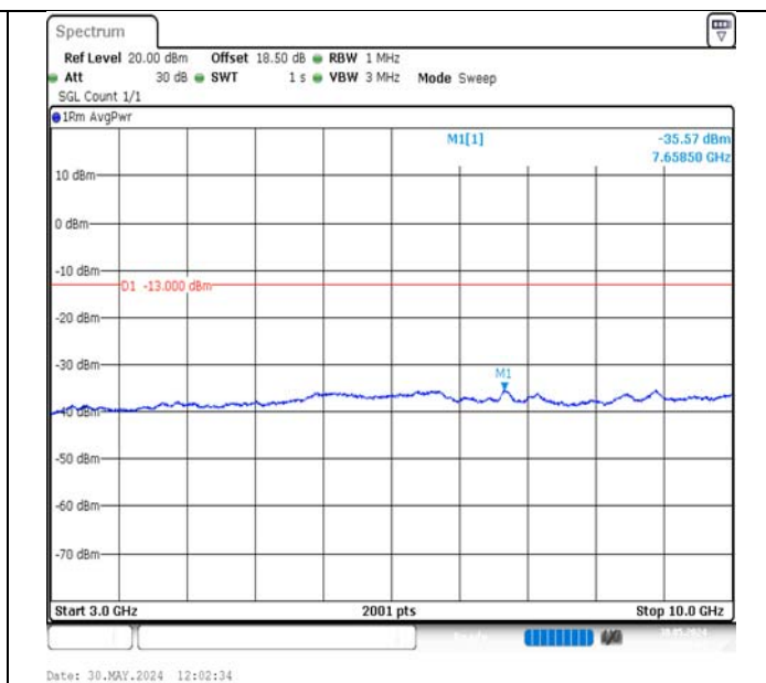
Band13-5MHz-QPSK-23230-1RB#24-3000~10000-PASS
