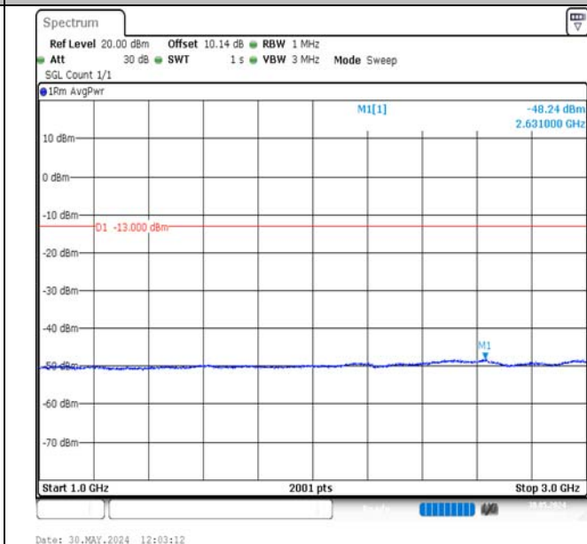
Band13-5MHz-QPSK-23230-25RB#0-1000~3000-PASS
