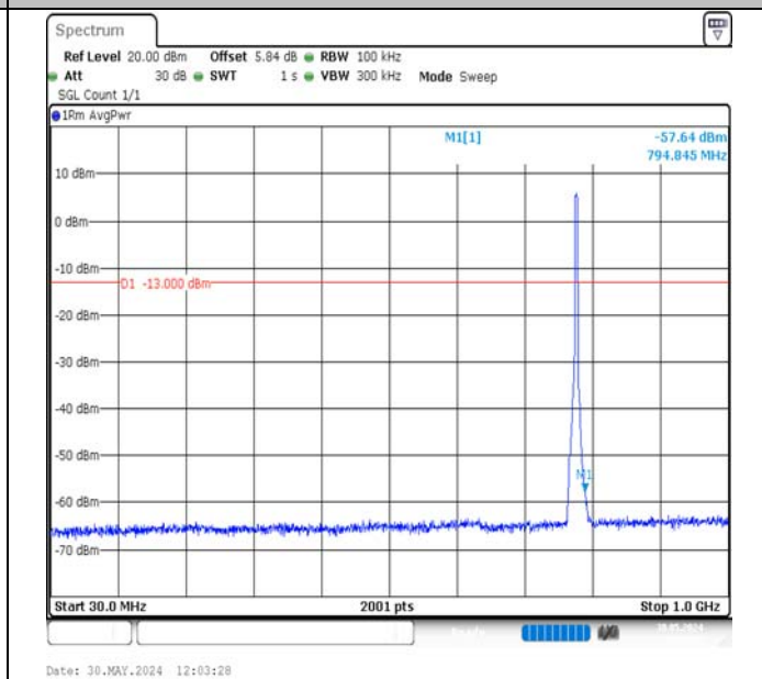
Band13-5MHz-16QAM-23230-25RB#0-30~1000-PASS
