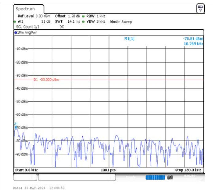
Band13-5MHz-QPSK-23205-25RB#0-0.009~0.15-PASS
