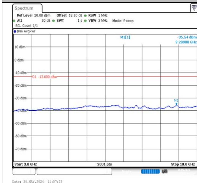
Band13-10MHz-QPSK-23230-1RB#0-3000~10000-PASS
