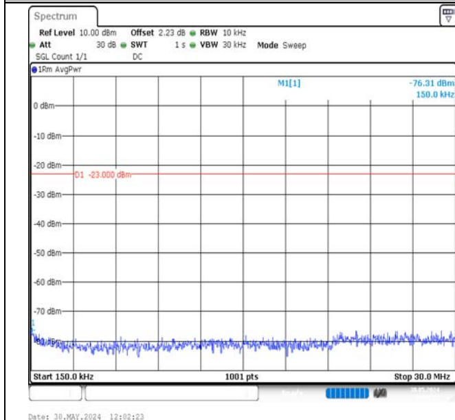
Band13-5MHz-QPSK-23230-1RB#24-0.15~30-PASS
