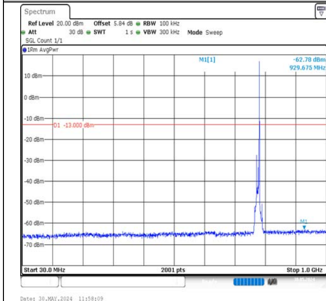
Band13-10MHz-QPSK-23230-1RB#49-30~1000-PASS
