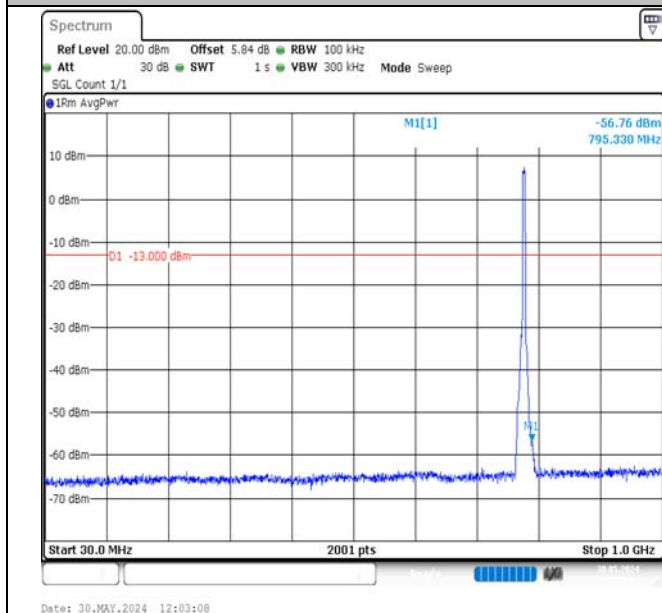
Band13-5MHz-QPSK-23230-25RB#0-30~1000-PASS
