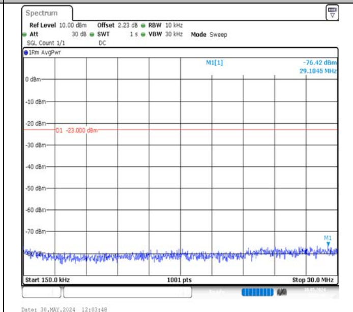
Band13-5MHz-QPSK-23255-1RB#0-0.15~30-PASS
