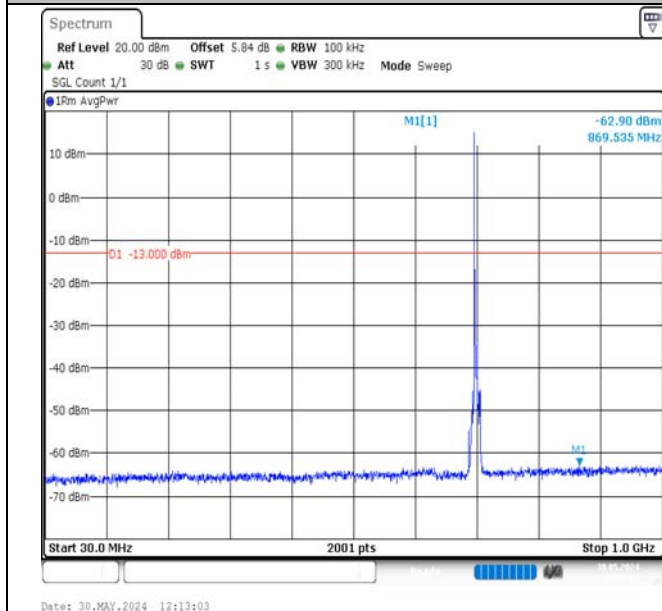
Band17-5MHz-QPSK-23755-1RB#0-30~1000-PASS
