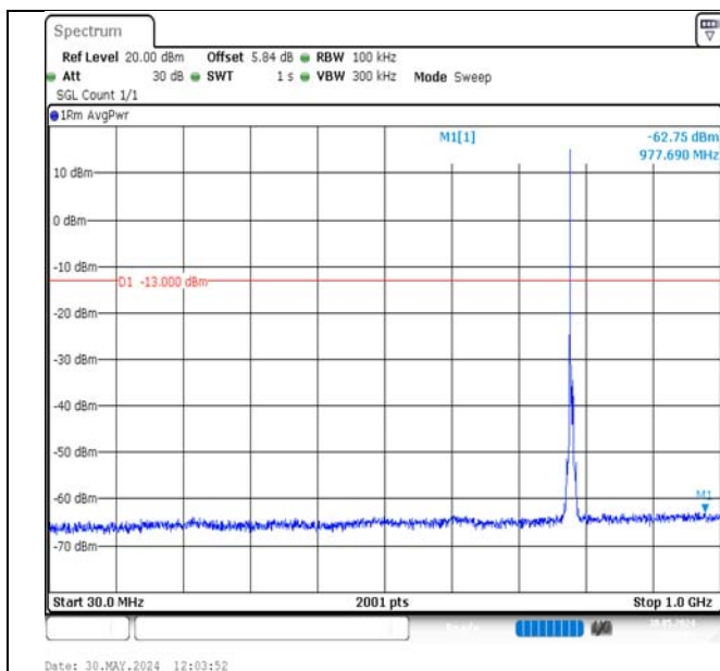
Band13-5MHz-QPSK-23255-1RB#0-30~1000-PASS
