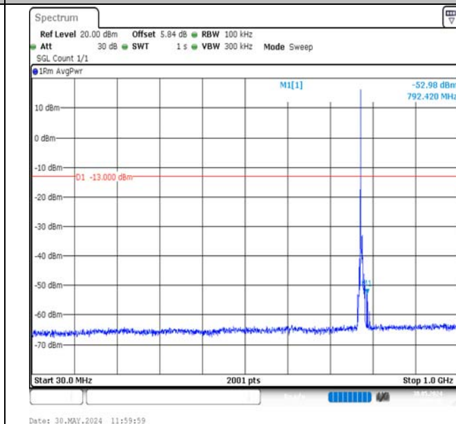
Band13-5MHz-16QAM-23205-1RB#0-30~1000-PASS
