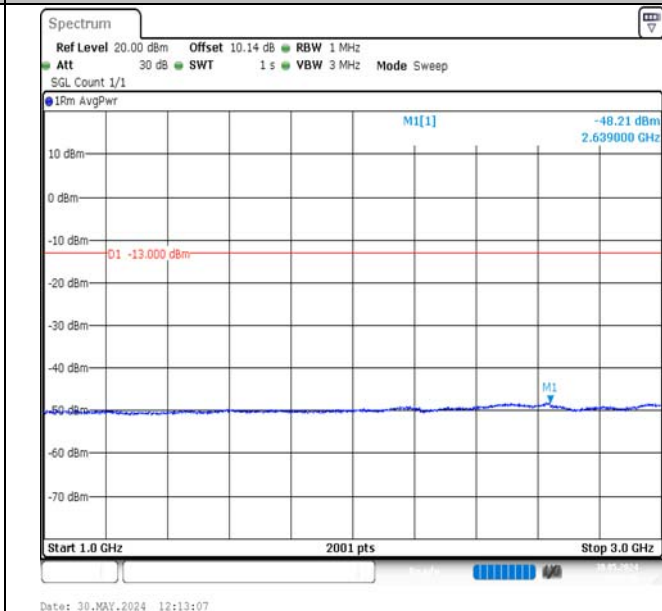
Band17-5MHz-QPSK-23755-1RB#0-1000~3000-PASS
