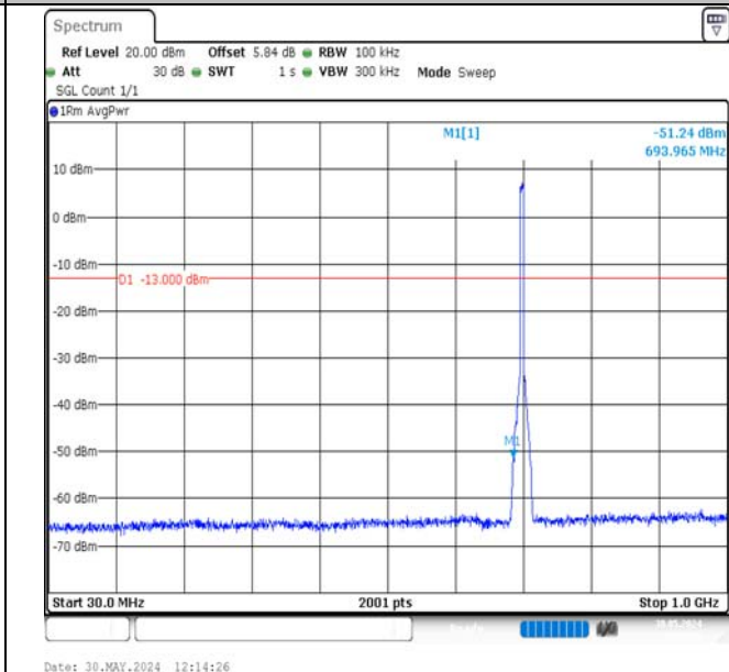
Band17-5MHz-QPSK-23755-25RB#0-30~1000-PASS
