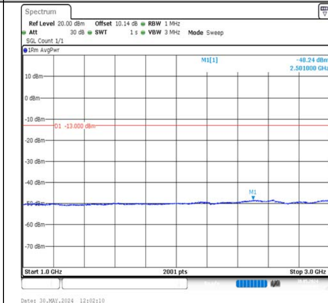
Band13-5MHz-16QAM-23230-1RB#0-1000~3000-PASS
