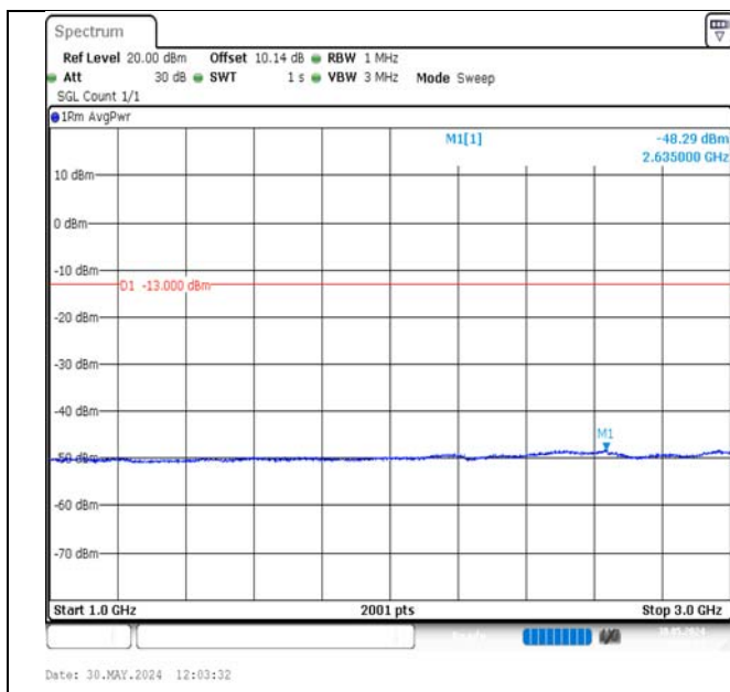
Band13-5MHz-16QAM-23230-25RB#0-1000~3000-PASS
