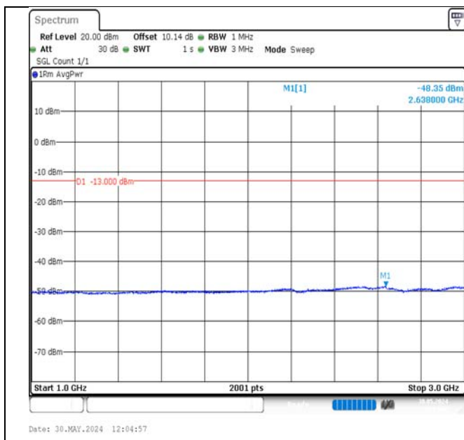
Band13-5MHz-16QAM-23255-1RB#24-1000~3000-PASS
