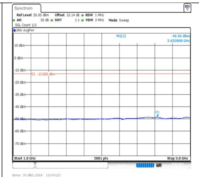
Band13-5MHz-QPSK-23205-1RB#24-1000~3000-PASS
