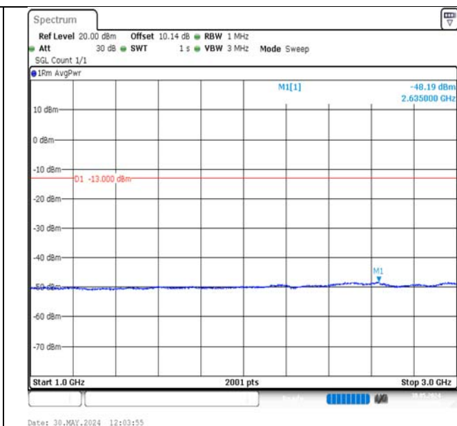
Band13-5MHz-QPSK-23255-1RB#0-1000~3000-PASS
