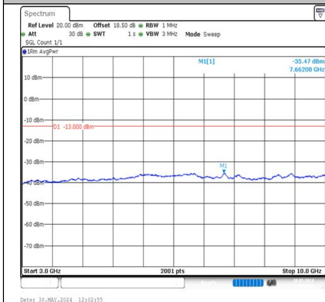
Band13-5MHz-16QAM-23230-1RB#24-3000~10000-PASS
