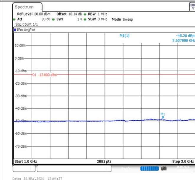
Band13-5MHz-QPSK-23255-1RB#24-1000~3000-PASS
