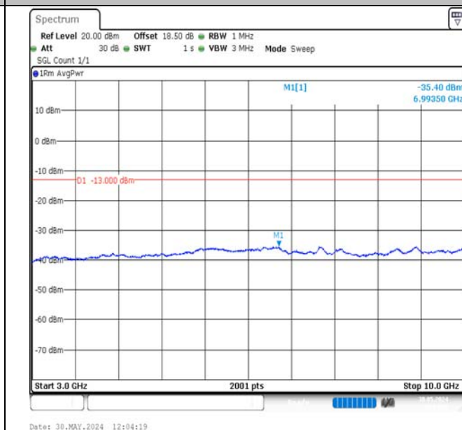
Band13-5MHz-16QAM-23255-1RB#0-3000~10000-PASS
