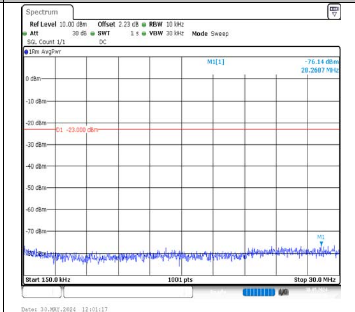
Band13-5MHz-16QAM-23205-25RB#0-0.15~30-PASS
