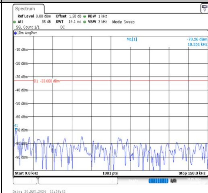
Band13-10MHz-QPSK-23230-50RB#0-0.009~0.15-PASS
