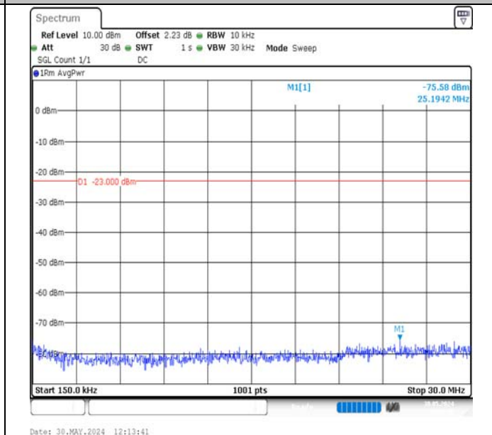
Band17-5MHz-QPSK-23755-1RB#24-0.15~30-PASS
