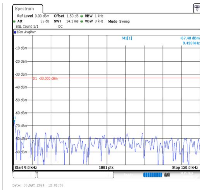
Band13-5MHz-16QAM-23230-1RB#0-0.009~0.15-PASS
