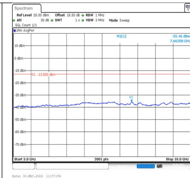
Band13-10MHz-16QAM-23230-1RB#0-3000~10000-PASS
