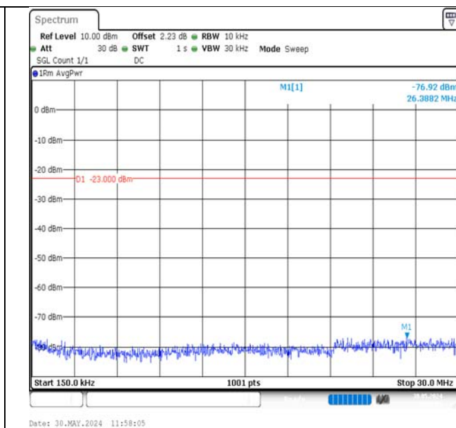
Band13-10MHz-QPSK-23230-1RB#49-0.15~30-PASS
