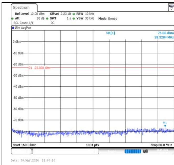
Band13-5MHz-QPSK-23255-25RB#0-0.15~30-PASS
