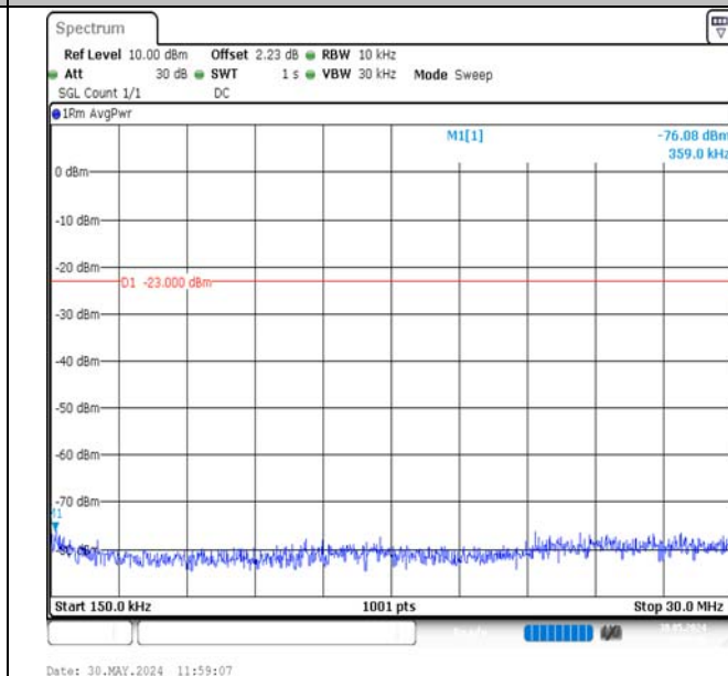
Band13-10MHz-16QAM-23230-50RB#0-0.15~30-PASS
