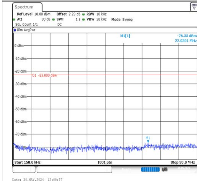
Band13-5MHz-QPSK-23205-25RB#0-0.15~30-PASS
