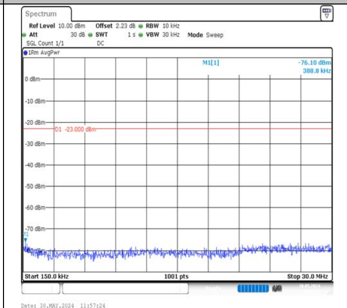
Band13-10MHz-QPSK-23230-1RB#0-0.15~30-PASS
