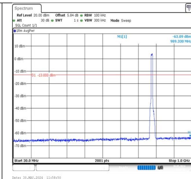
Band13-10MHz-QPSK-23230-50RB#0-30~1000-PASS
