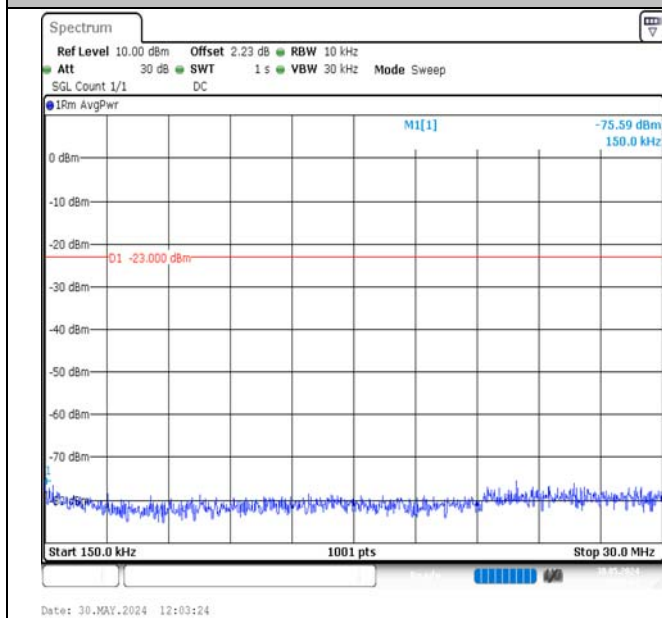
Band13-5MHz-16QAM-23230-25RB#0-0.15~30-PASS
