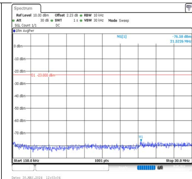
Band13-5MHz-QPSK-23230-25RB#0-0.15~30-PASS
