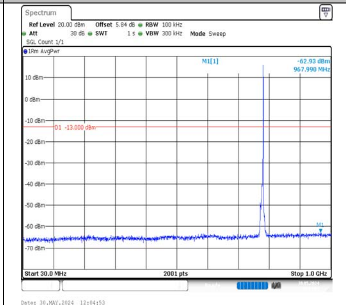
Band13-5MHz-16QAM-23255-1RB#24-30~1000-PASS
