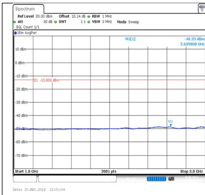
Band13-5MHz-QPSK-23205-25RB#0-1000~3000-PASS
