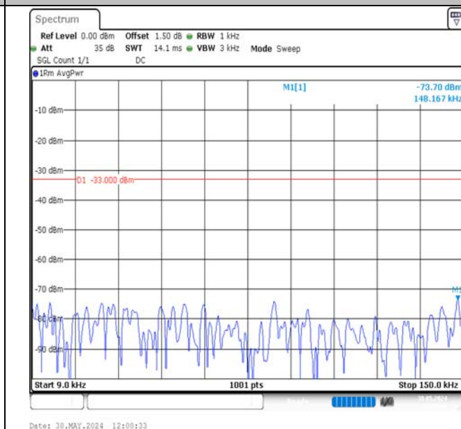
Band13-5MHz-16QAM-23205-1RB#24-0.009~0.15-PASS
