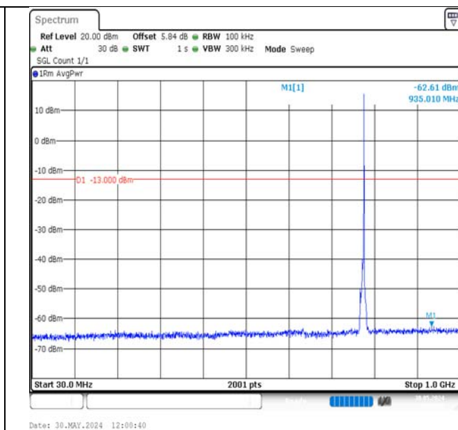
Band13-5MHz-16QAM-23205-1RB#24-30~1000-PASS
