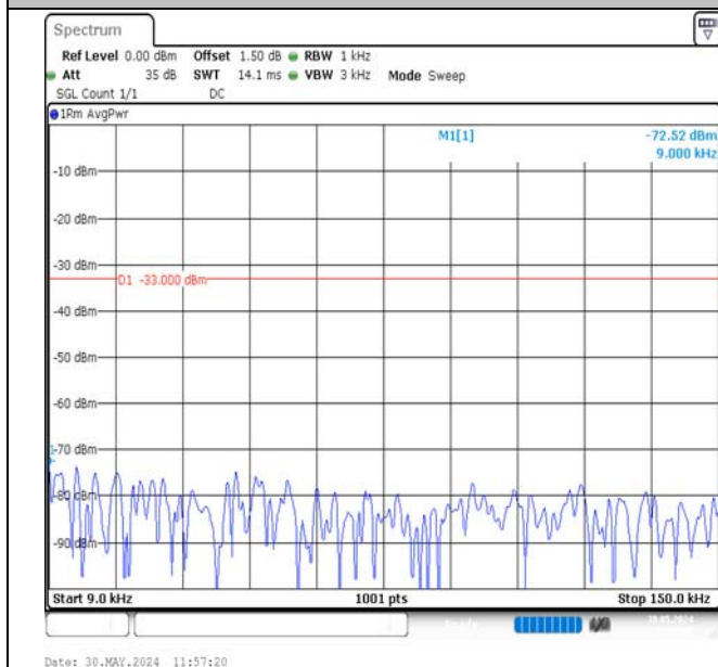
Band13-10MHz-QPSK-23230-1RB#0-0.009~0.15-PASS
