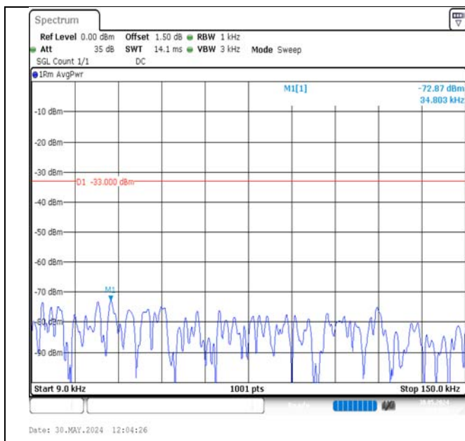
Band13-5MHz-QPSK-23255-1RB#24-0.009~0.15-PASS
