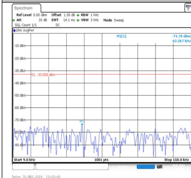
Band13-5MHz-16QAM-23230-1RB#24-0.009~0.15-PASS
