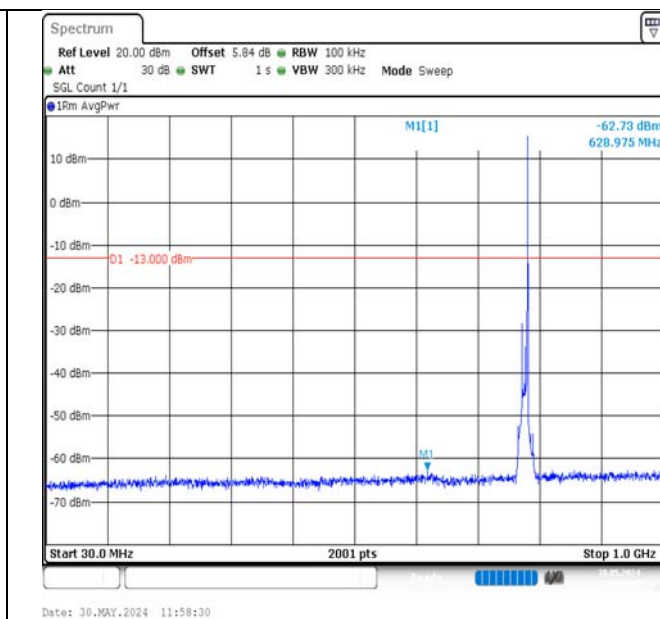
Band13-10MHz-16QAM-23230-1RB#49-30~1000-PASS
