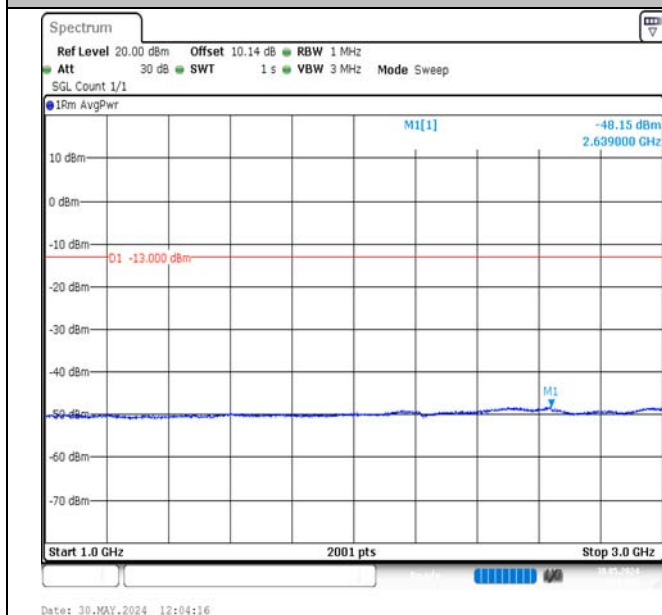
Band13-5MHz-16QAM-23255-1RB#0-1000~3000-PASS
