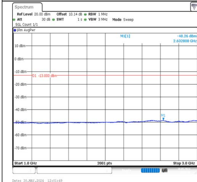
Band13-5MHz-QPSK-23230-1RB#0-1000~3000-PASS
