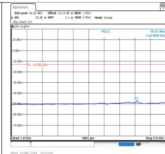
Band13-5MHz-16QAM-23205-25RB#0-1000~3000-PASS
