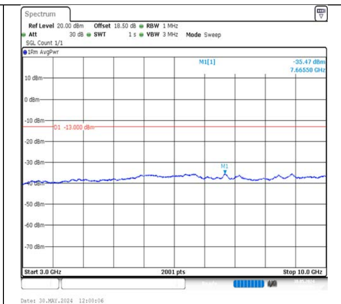
Band13-5MHz-16QAM-23205-1RB#0-3000~10000-PASS
