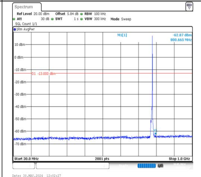
Band13-5MHz-QPSK-23230-1RB#24-30~1000-PASS
