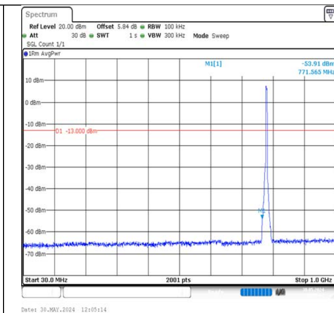
Band13-5MHz-QPSK-23255-25RB#0-30~1000-PASS
