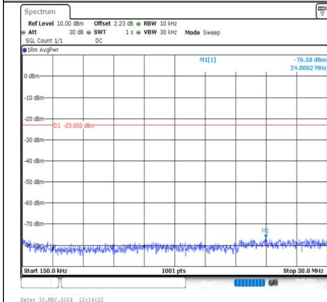
Band17-5MHz-QPSK-23755-25RB#0-0.15~30-PASS
