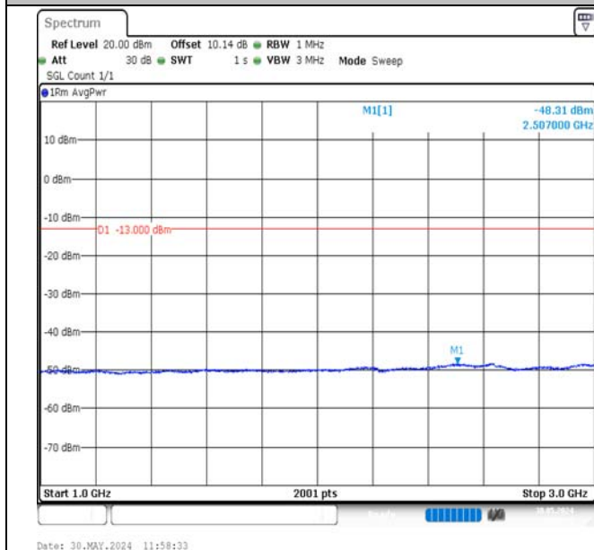
Band13-10MHz-16QAM-23230-1RB#49-1000~3000-PASS
