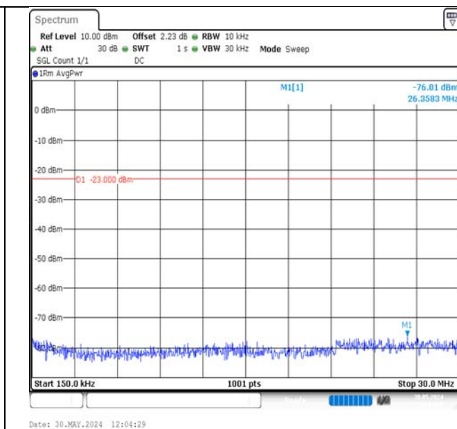
Band13-5MHz-QPSK-23255-1RB#24-0.15~30-PASS
