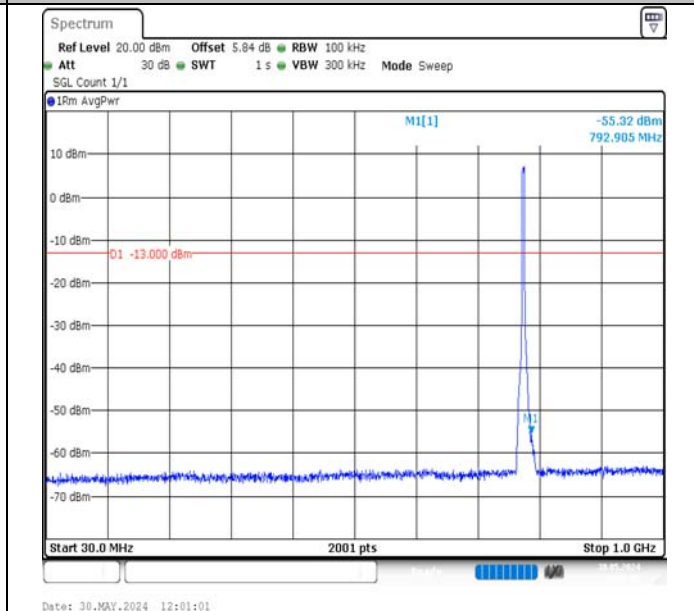
Band13-5MHz-QPSK-23205-25RB#0-30~1000-PASS
