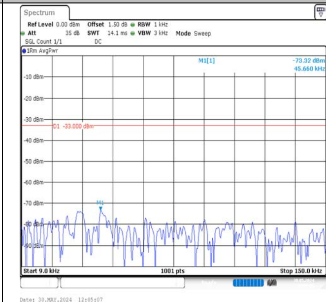
Band13-5MHz-QPSK-23255-25RB#0-0.009~0.15-PASS
