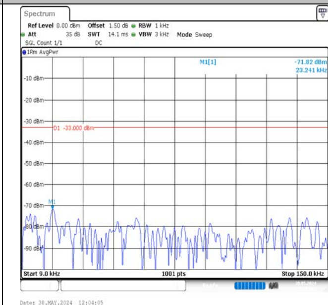
Band13-5MHz-16QAM-23255-1RB#0-0.009~0.15-PASS
