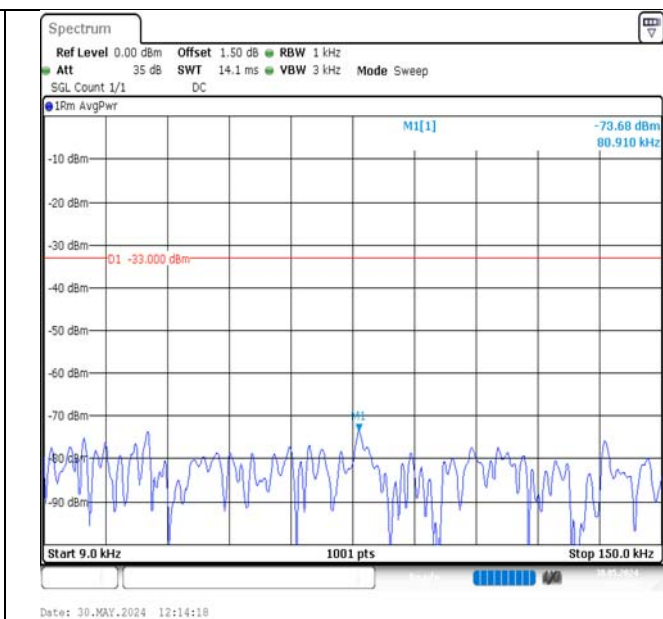
Band17-5MHz-QPSK-23755-25RB#0-0.009~0.15-PASS
