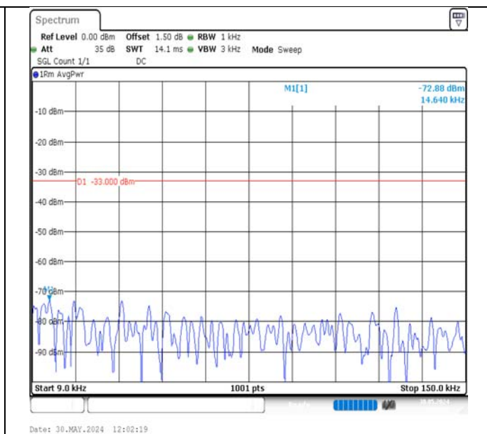
Band13-5MHz-QPSK-23230-1RB#24-0.009~0.15-PASS
