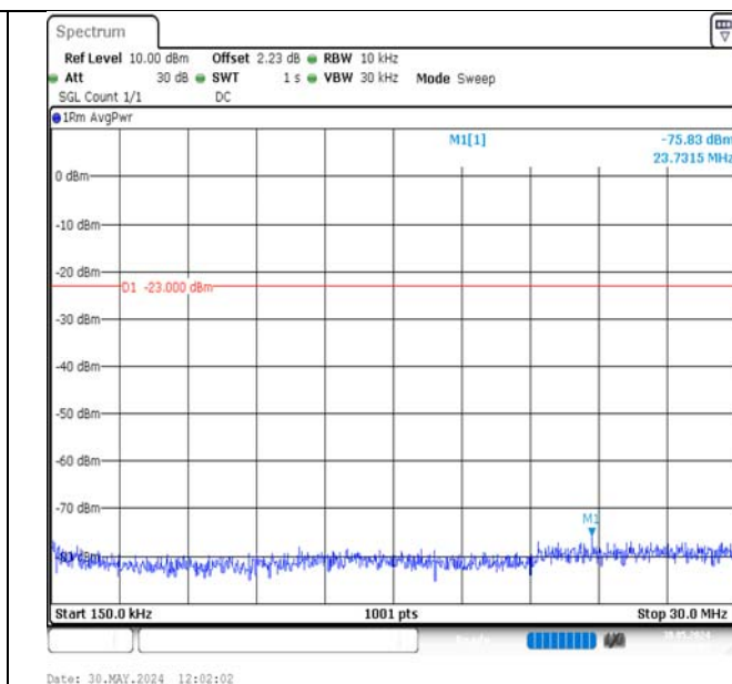
Band13-5MHz-16QAM-23230-1RB#0-0.15~30-PASS
