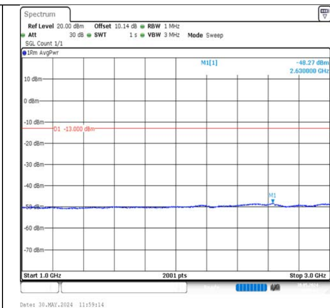
Band13-10MHz-16QAM-23230-50RB#0-1000~3000-PASS
