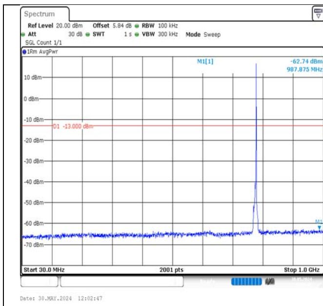
Band13-5MHz-16QAM-23230-1RB#24-30~1000-PASS
