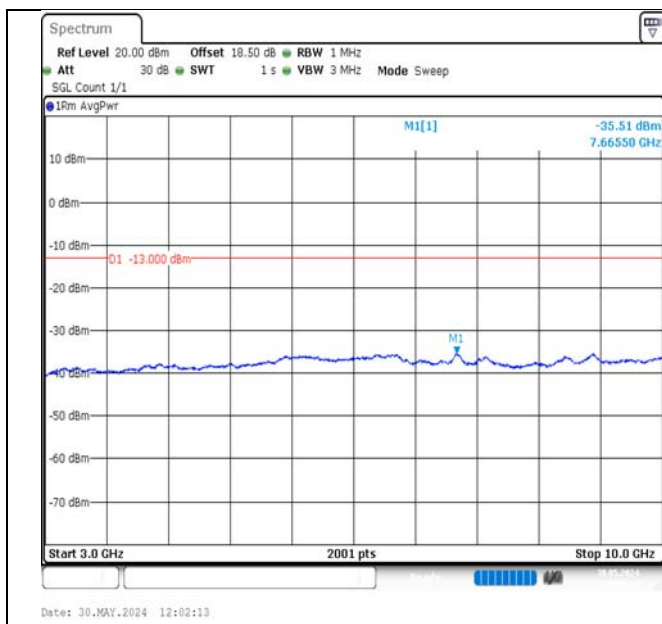
Band13-5MHz-16QAM-23230-1RB#0-3000~10000-PASS
