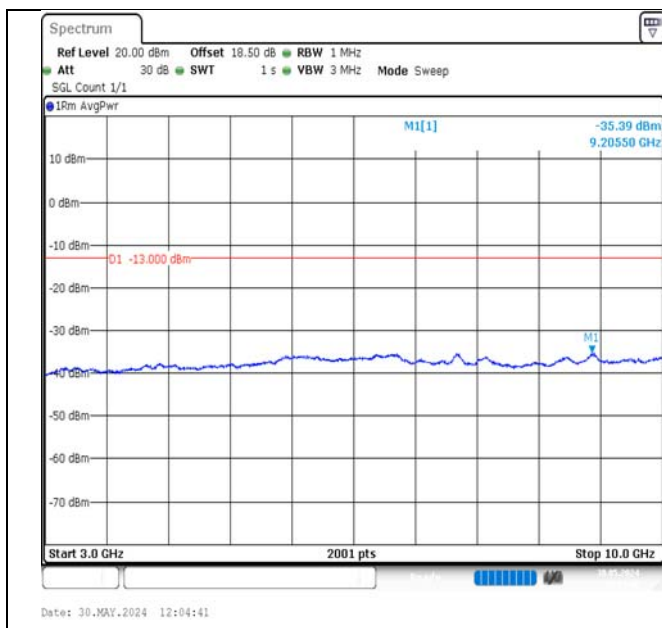
Band13-5MHz-QPSK-23255-1RB#24-3000~10000-PASS
