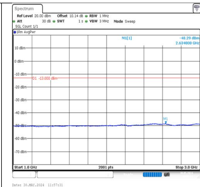
Band13-10MHz-QPSK-23230-1RB#0-1000~3000-PASS
