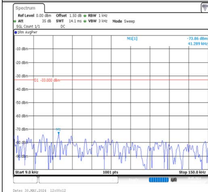
Band13-5MHz-QPSK-23205-1RB#24-0.009~0.15-PASS
