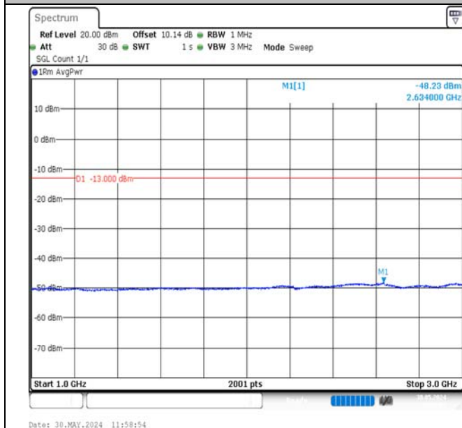
Band13-10MHz-QPSK-23230-50RB#0-1000~3000-PASS
