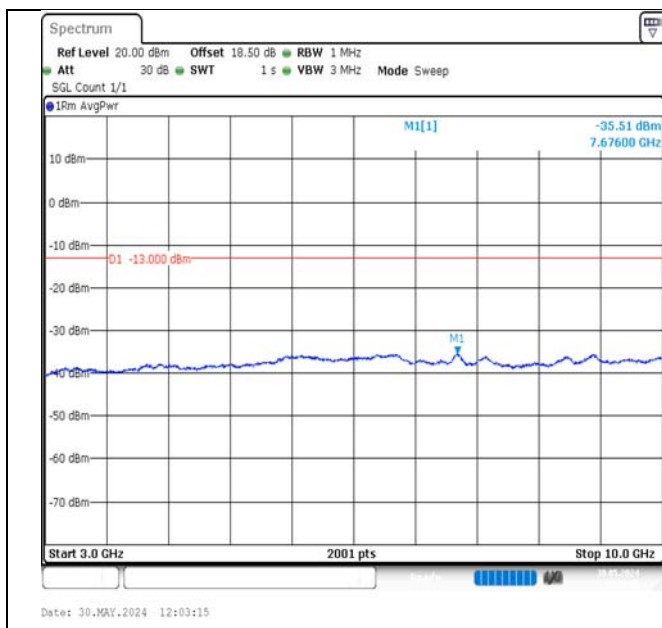
Band13-5MHz-QPSK-23230-25RB#0-3000~10000-PASS
