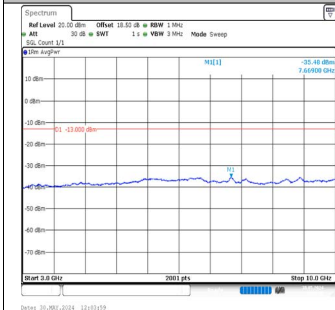
Band13-5MHz-QPSK-23255-1RB#0-3000~10000-PASS
