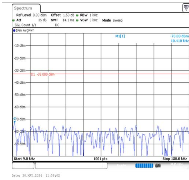
Band13-10MHz-QPSK-23230-1RB#49-0.009~0.15-PASS
