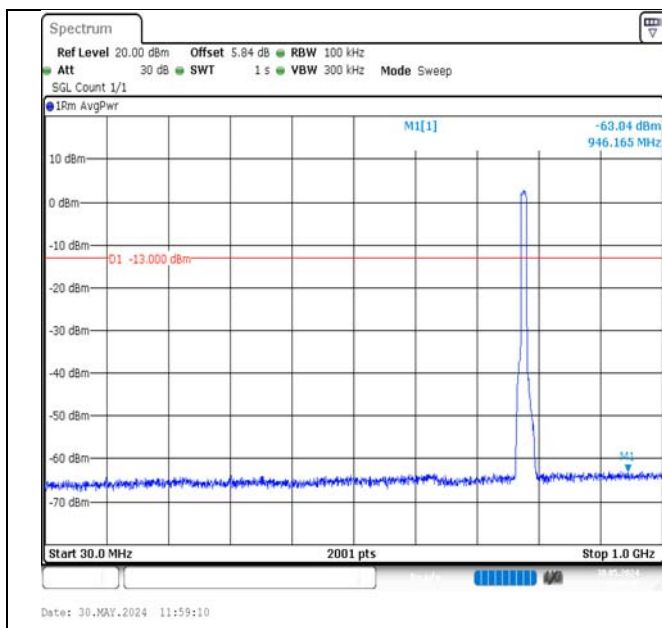
Band13-10MHz-16QAM-23230-50RB#0-30~1000-PASS
