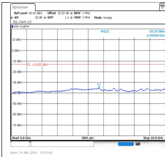
Band13-5MHz-16QAM-23255-25RB#0-3000~10000-PASS
