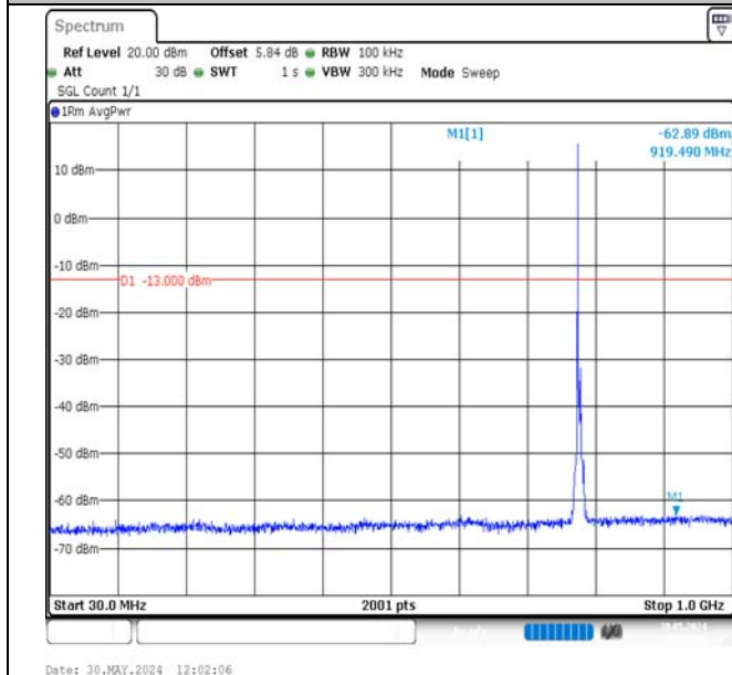
Band13-5MHz-16QAM-23230-1RB#0-30~1000-PASS
