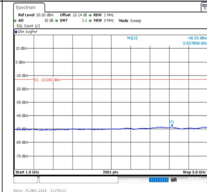
Band13-10MHz-QPSK-23230-1RB#49-1000~3000-PASS
