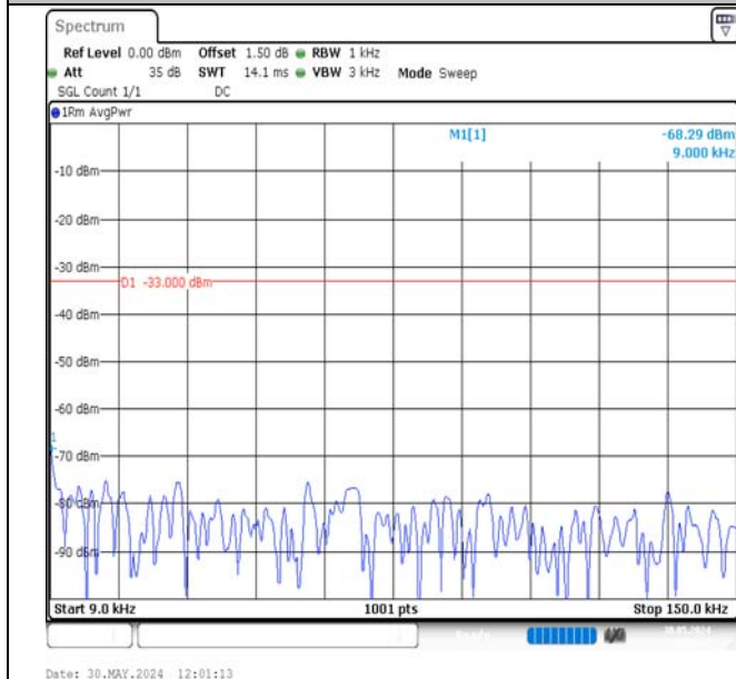
Band13-5MHz-16QAM-23205-25RB#0-0.009~0.15-PASS
