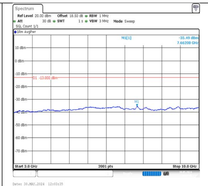
Band13-5MHz-16QAM-23230-25RB#0-3000~10000-PASS
