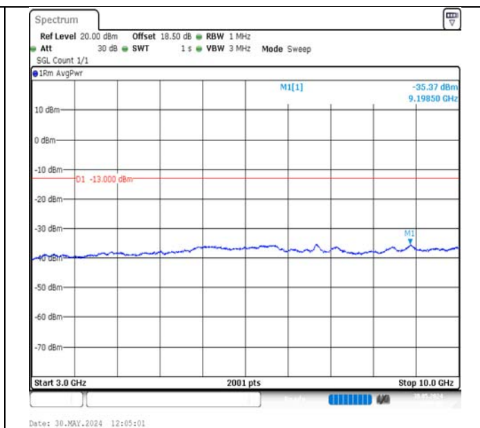
Band13-5MHz-16QAM-23255-1RB#24-3000~10000-PASS
