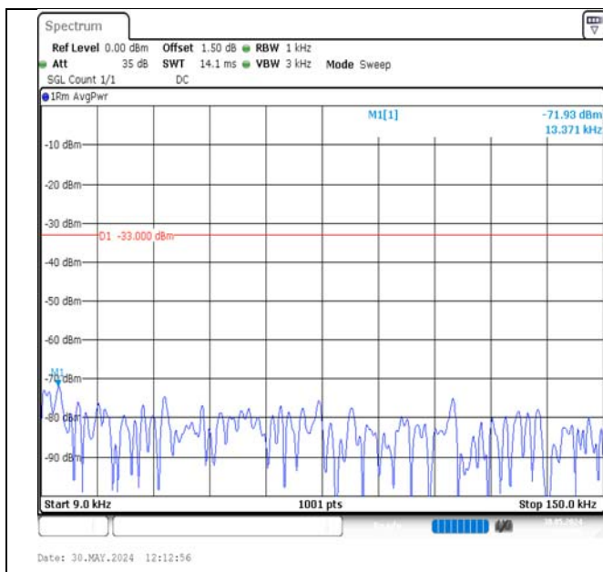
Band17-5MHz-QPSK-23755-1RB#0-0.009~0.15-PASS
