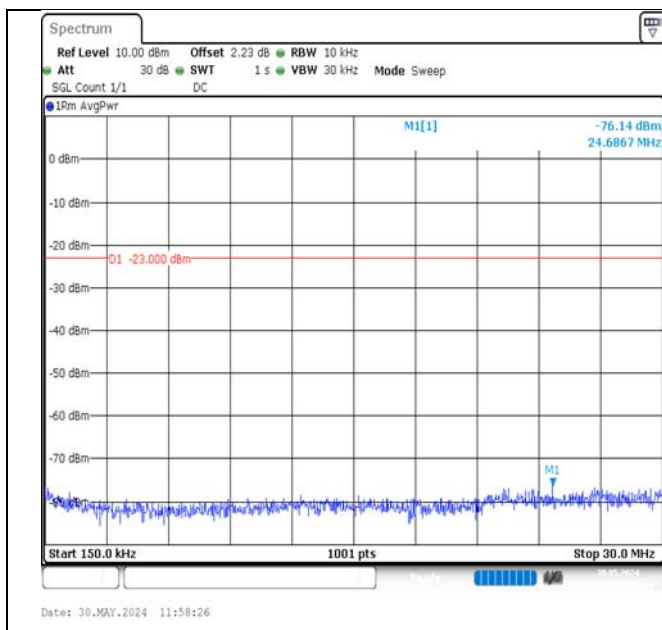
Band13-10MHz-16QAM-23230-1RB#49-0.15~30-PASS
