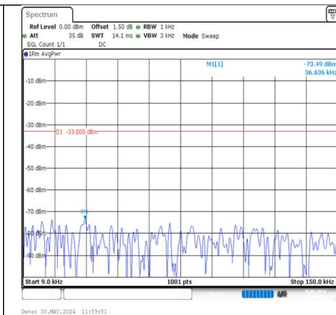
Band13-5MHz-16QAM-23205-1RB#0-0.009~0.15-PASS
