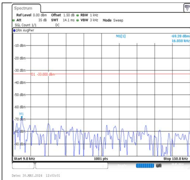
Band13-5MHz-QPSK-23230-25RB#0-0.009~0.15-PASS
