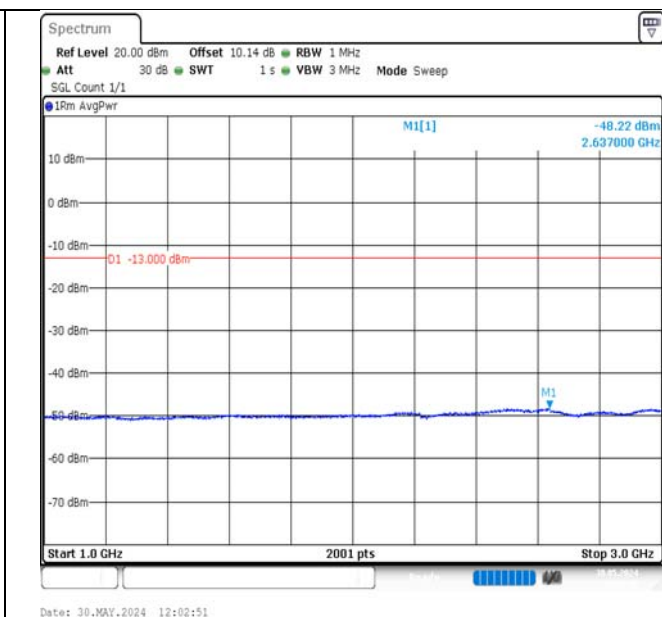
Band13-5MHz-16QAM-23230-1RB#24-1000~3000-PASS
