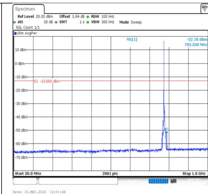
Band13-5MHz-QPSK-23230-1RB#0-30~1000-PASS
