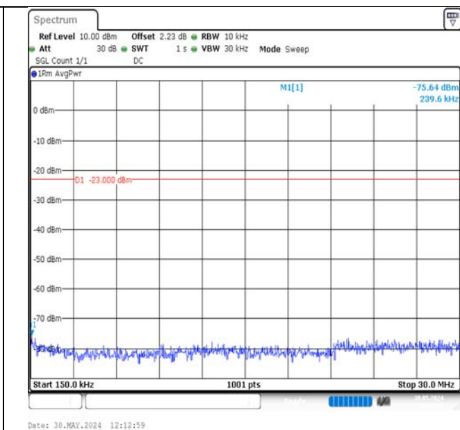
Band17-5MHz-QPSK-23755-1RB#0-0.15~30-PASS
