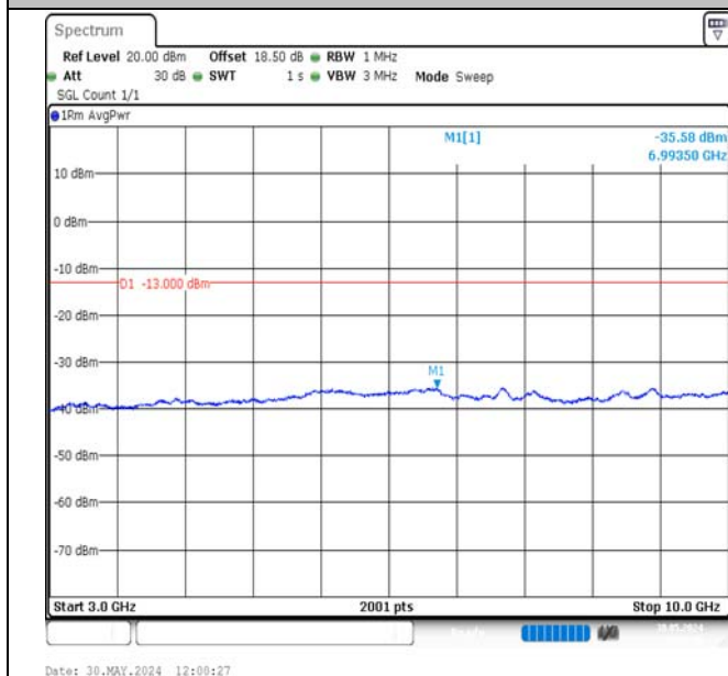
Band13-5MHz-QPSK-23205-1RB#24-3000~10000-PASS
