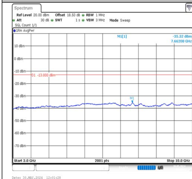
Band13-5MHz-16QAM-23205-25RB#0-3000~10000-PASS
