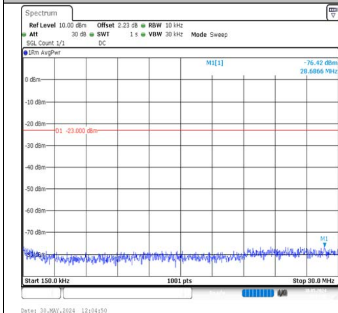
Band13-5MHz-16QAM-23255-1RB#24-0.15~30-PASS
