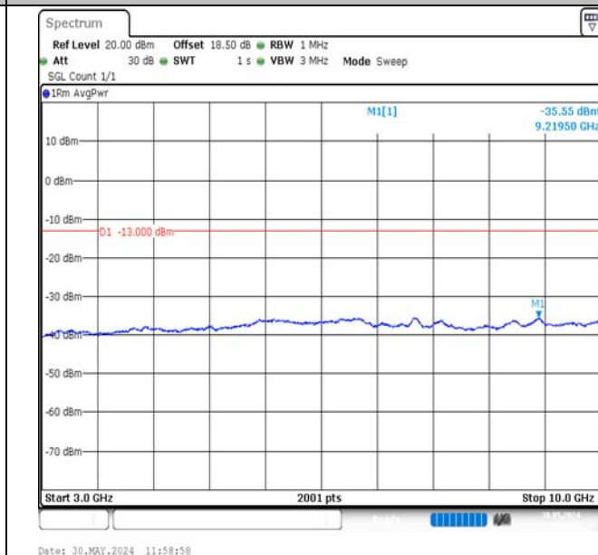
Band13-10MHz-QPSK-23230-50RB#0-3000~10000-PASS
