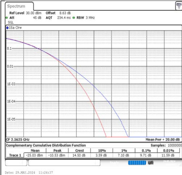
Band7-15MHz-QPSK-21375-1RB#0-PASS
