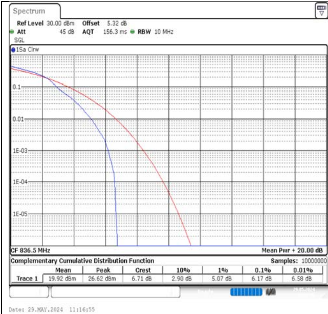
Band5-10MHz-16QAM-20525-1RB#0-PASS
