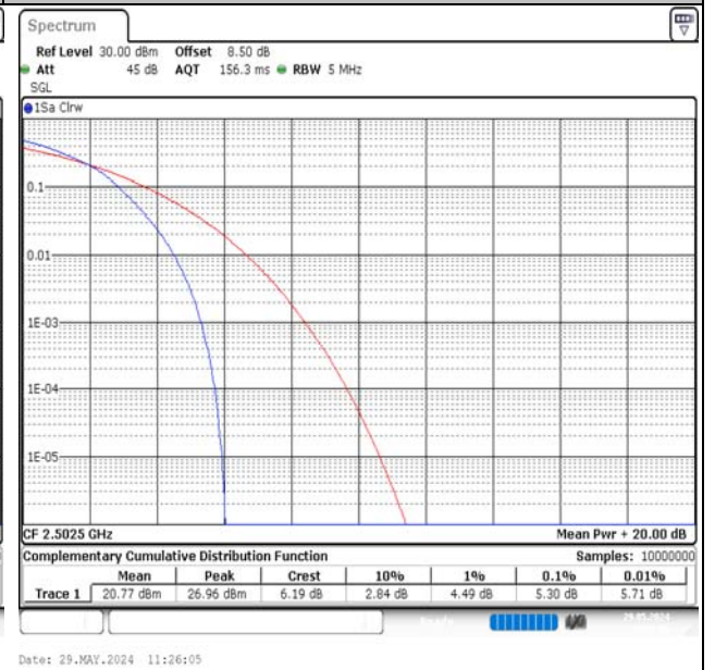
Band7-5MHz-16QAM-20775-25RB#0-PASS
