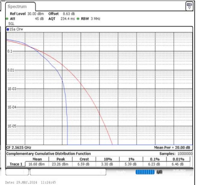
Band7-15MHz-QPSK-21375-75RB#0-PASS
