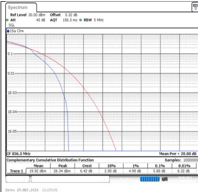
Band5-5MHz-16QAM-20525-1RB#0-PASS
