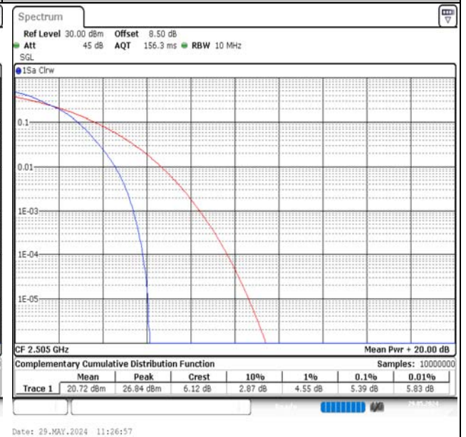
Band7-10MHz-16QAM-20800-50RB#0-PASS
