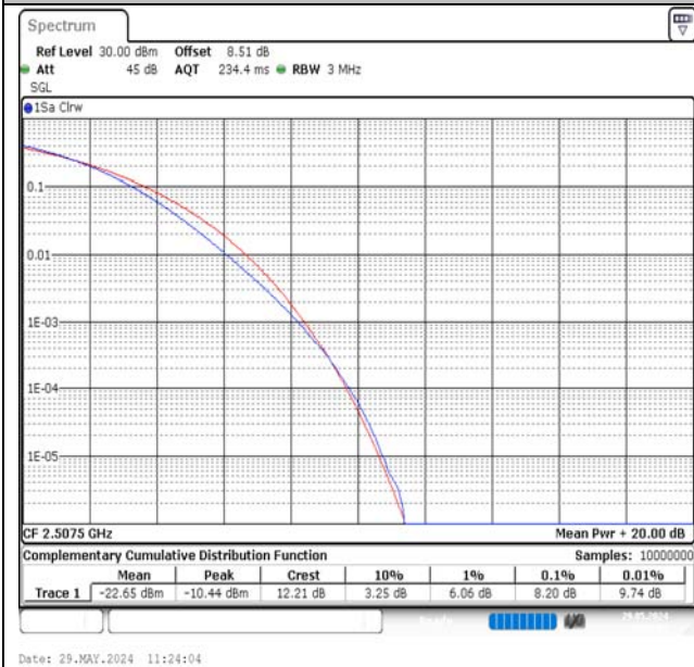
Band7-15MHz-16QAM-20825-1RB#0-PASS
