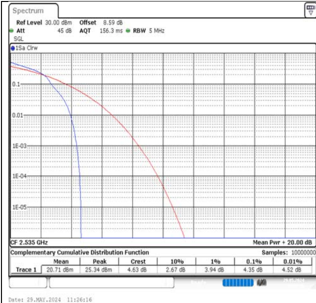
Band7-5MHz-16QAM-21100-1RB#0-PASS
