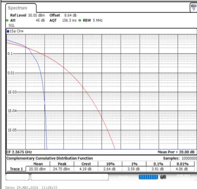
Band7-5MHz-16QAM-21425-1RB#0-PASS
