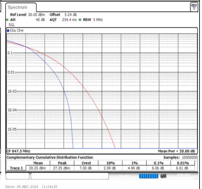
Band5-3MHz-16QAM-20635-15RB#0-PASS
