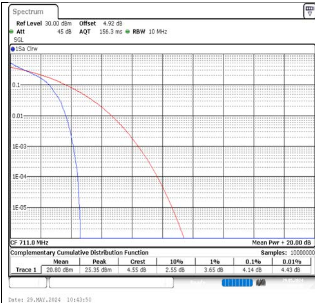
Band17-10MHz-QPSK-23800-1RB#0-PASS
