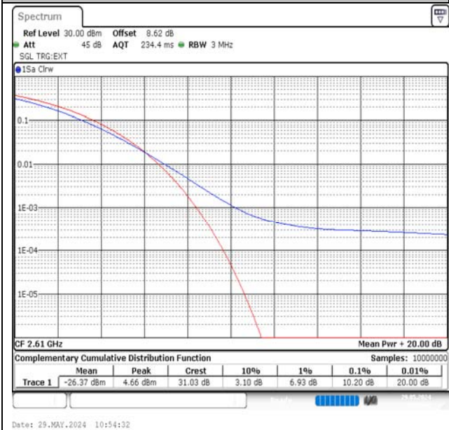
Band38-20MHz-16QAM-38150-1RB#0-PASS
