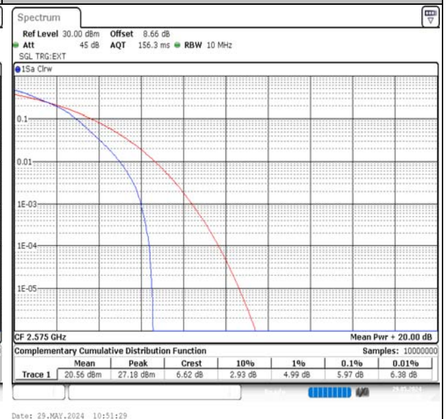
Band38-10MHz-16QAM-37800-50RB#0-PASS
