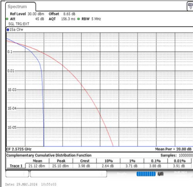
Band38-5MHz-QPSK-37775-1RB#0-PASS
