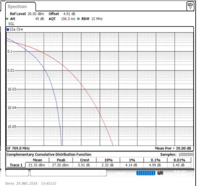
Band17-10MHz-QPSK-23780-50RB#0-PASS
