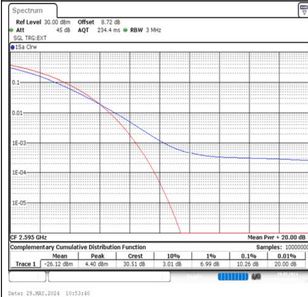
Band38-20MHz-QPSK-38000-1RB#0-PASS
