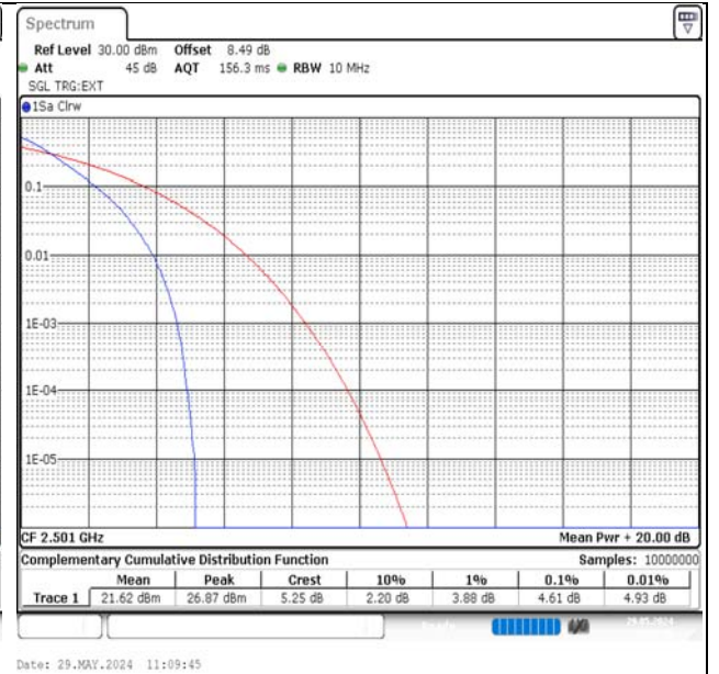
Band41-10MHz-QPSK-39700-50RB#0-PASS
