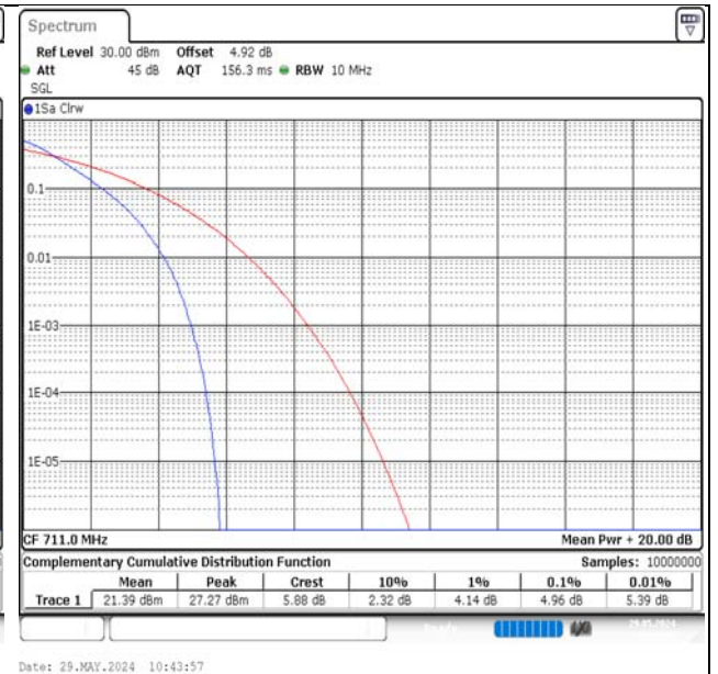
Band17-10MHz-QPSK-23800-50RB#0-PASS
