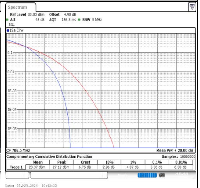
Band17-5MHz-16QAM-23755-25RB#0-PASS
