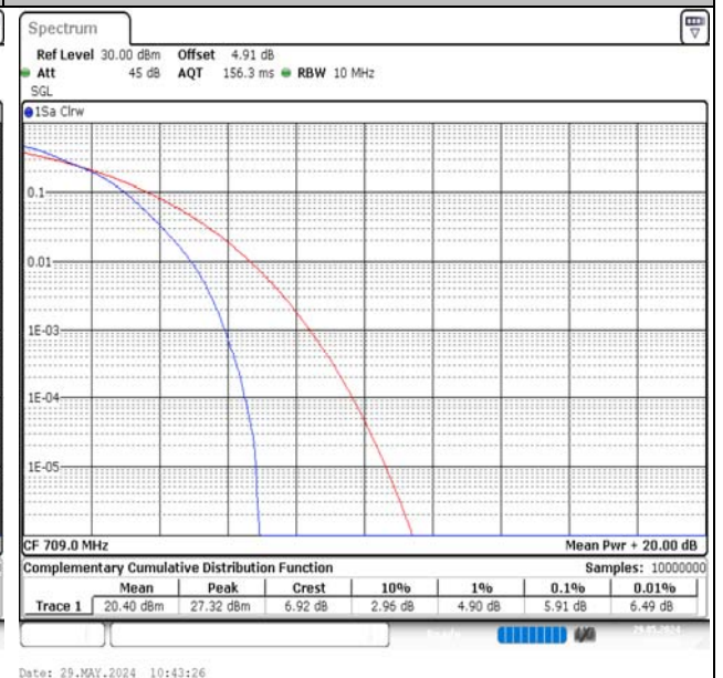
Band17-10MHz-16QAM-23780-50RB#0-PASS
