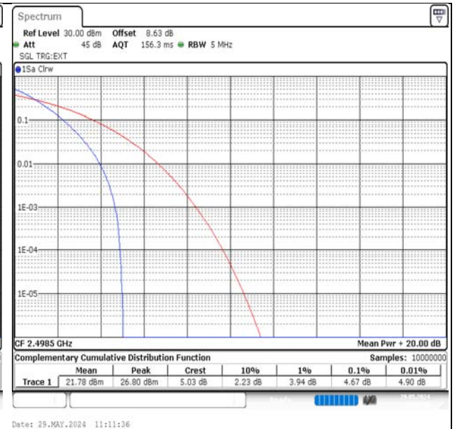
Band41-5MHz-QPSK-39675-25RB#0-PASS
