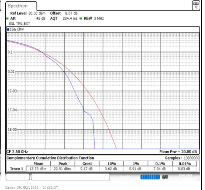
Band38-20MHz-16QAM-37850-100RB#0-PASS
