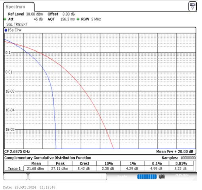
Band41-5MHz-QPSK-41565-25RB#0-PASS
