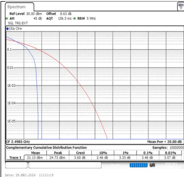
Band41-5MHz-QPSK-39675-1RB#0-PASS
