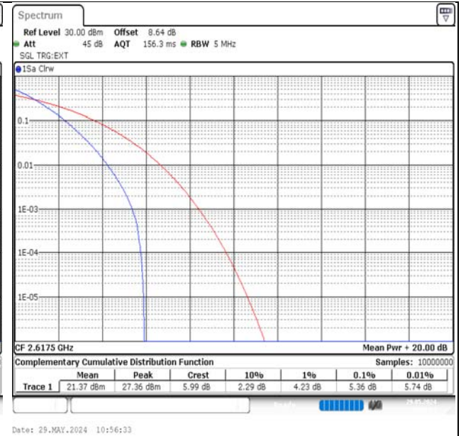
Band38-5MHz-QPSK-38225-25RB#0-PASS
