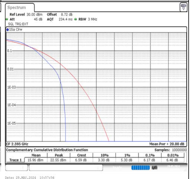
Band38-15MHz-QPSK-38000-75RB#0-PASS
