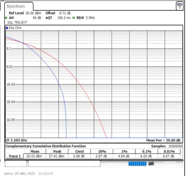
Band41-5MHz-16QAM-40620-25RB#0-PASS
