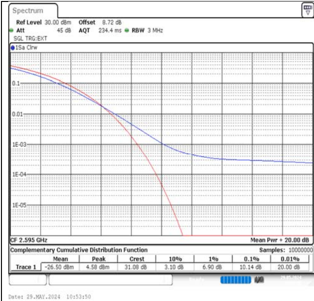
Band38-20MHz-16QAM-38000-1RB#0-PASS
