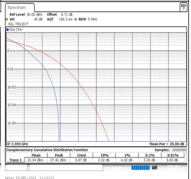
Band41-5MHz-QPSK-40620-25RB#0-PASS
