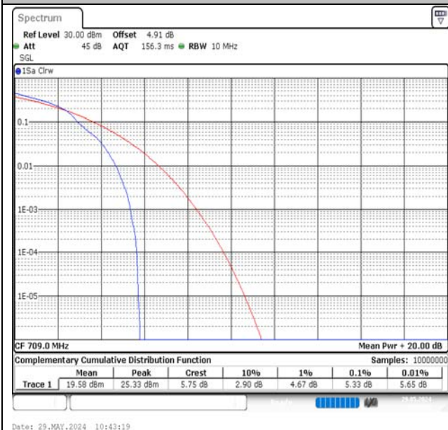
Band17-10MHz-16QAM-23780-1RB#0-PASS
