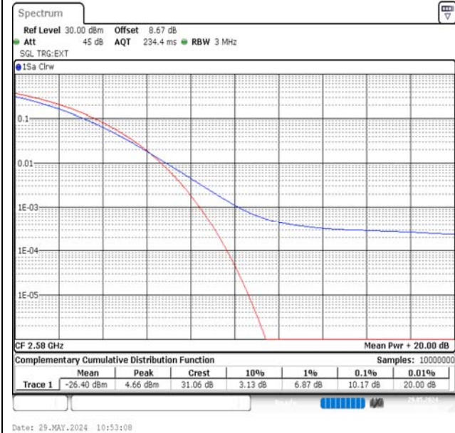
Band38-20MHz-16QAM-37850-1RB#0-PASS
