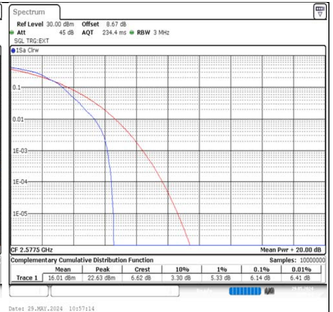
Band38-15MHz-QPSK-37825-75RB#0-PASS
