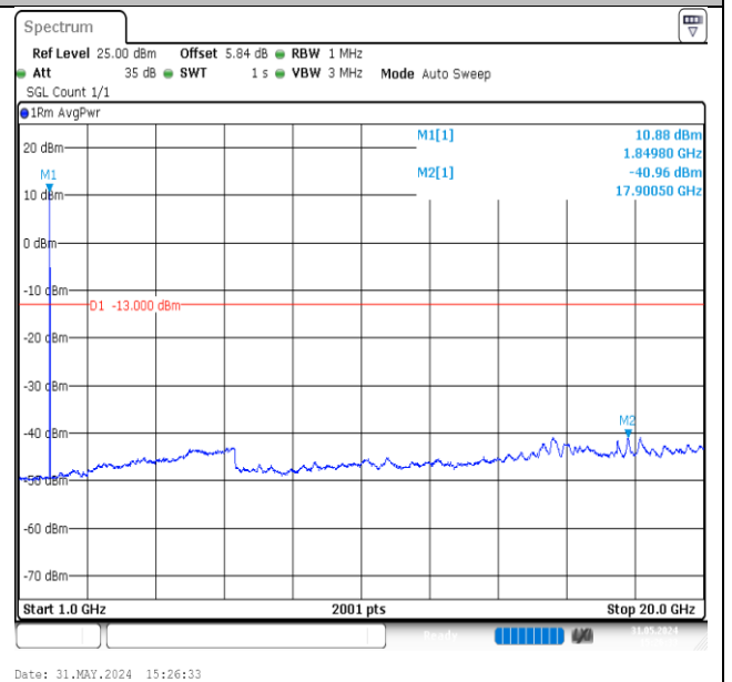
Band2-9262-1000~20000MHz-PASS
