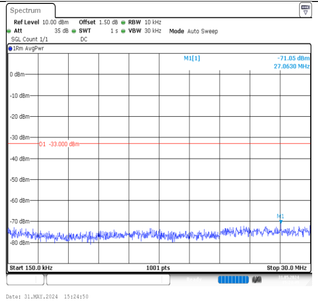
Band4-1312-0.15~30MHz-PASS
