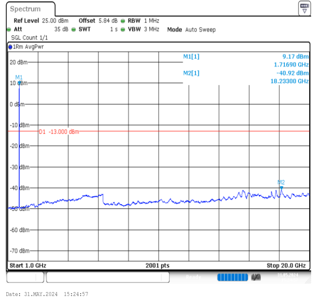
Band4-1312-1000~20000MHz-PASS
