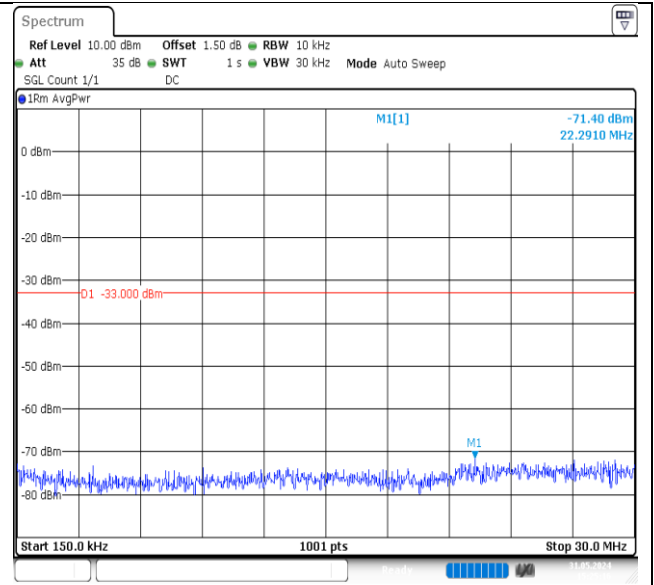
Band4-1413-0.15~30MHz-PASS
