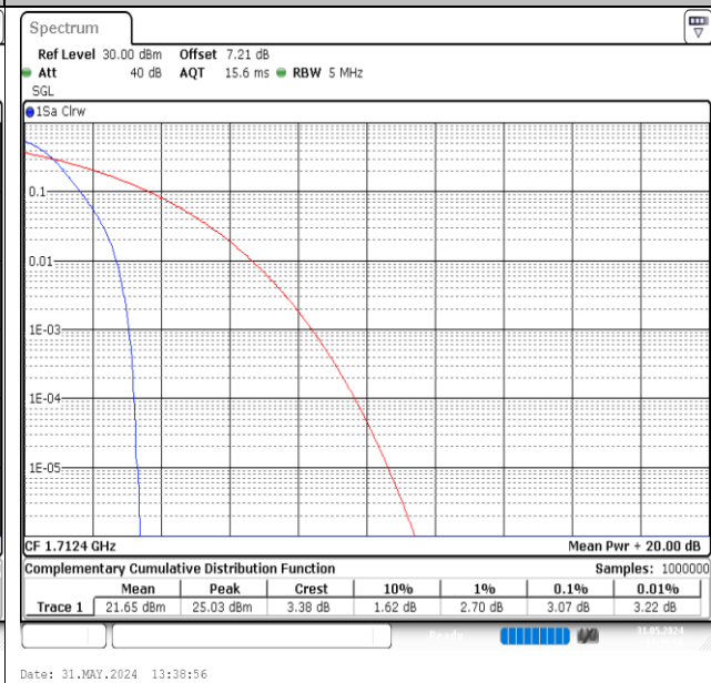
Band4-1312-PASS
