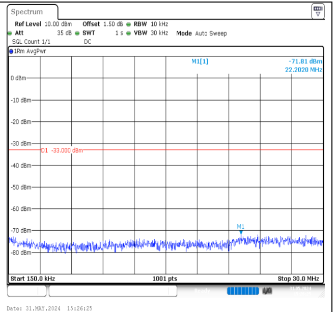
Band2-9262-0.15~30MHz-PASS
