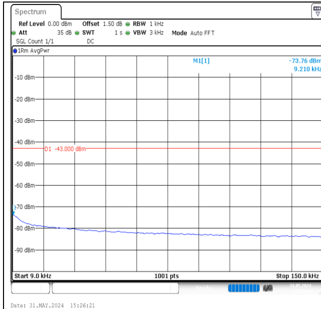
Band2-9262-0.009~0.15MHz-PASS
