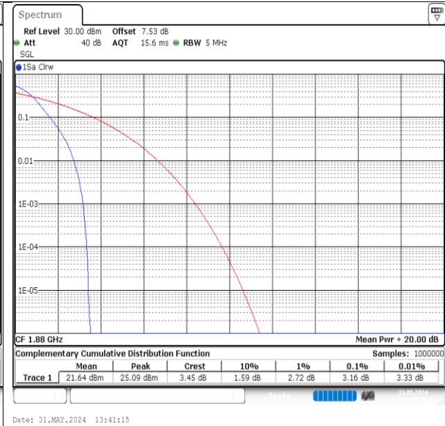
Band2-9400-PASS
