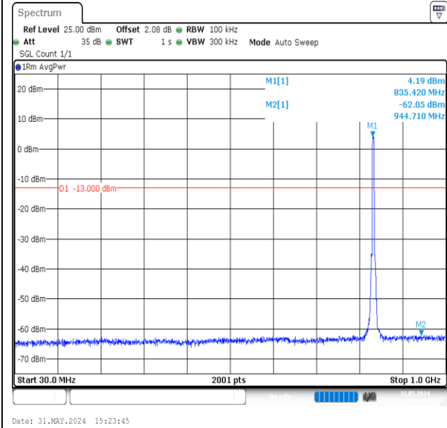
Band5-4182-30~1000MHz-PASS
