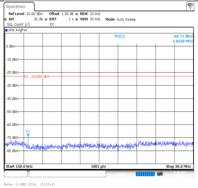
Band5-4182-0.15~30MHz-PASS
