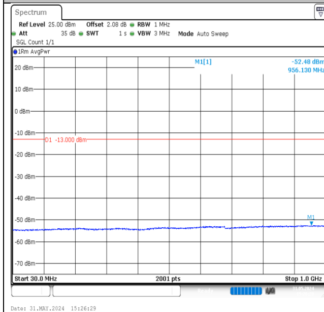
Band2-9262-30~1000MHz-PASS
