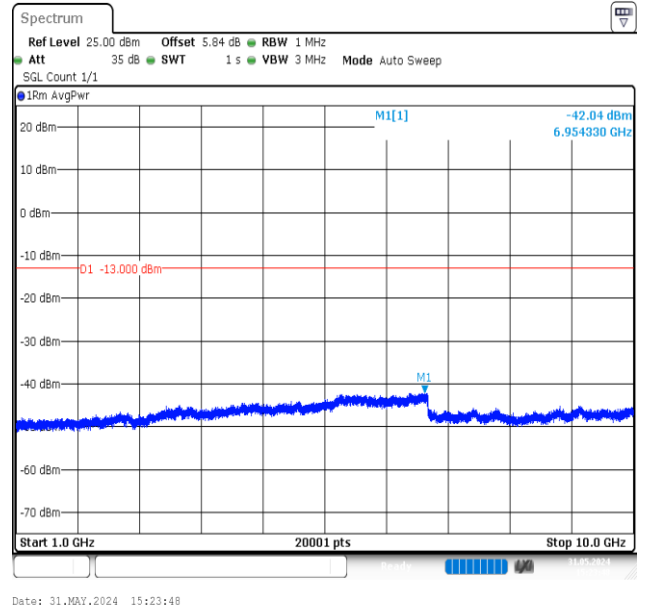
Band5-4182-1000~10000MHz-PASS
