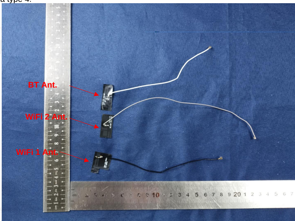
Antenna type 4:
