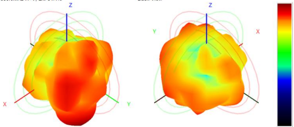
5850.0MHz H+V, Eff. 52.4%
