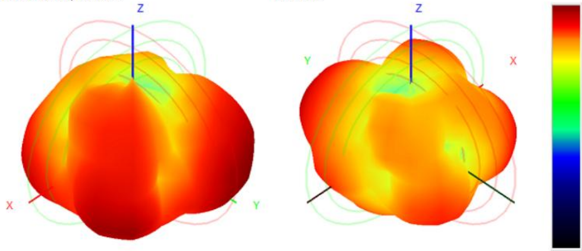
5350.0MHz H+V, Eff. 51.1%
