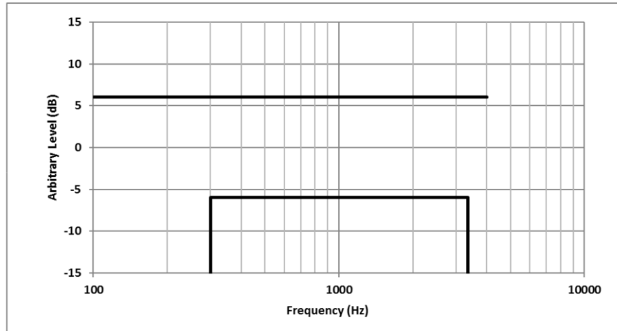
Figure 2 – Narrowband Receive Frequency Response Limits
