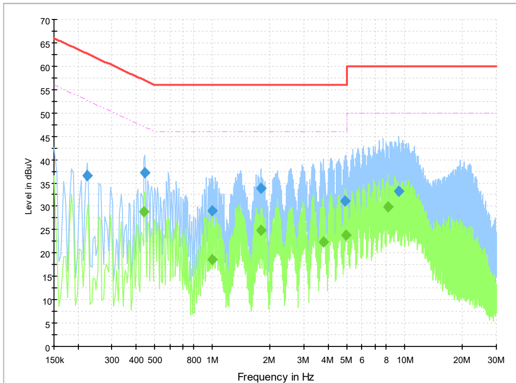
Fig.10 AC Powerline Conducted Emission-Idle
