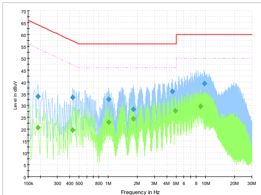
Fig.26. AC Powerline Conducted Emission- BLE
