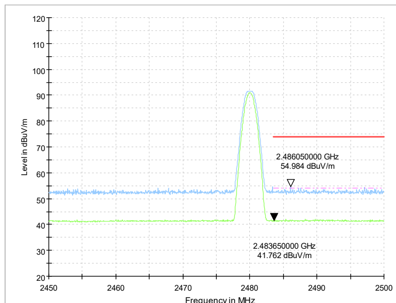
Fig.19. Frequency Band Edges: GFSK, 2480 MHz, Hopping Off, 2.45 GHz - 2.50GHz
