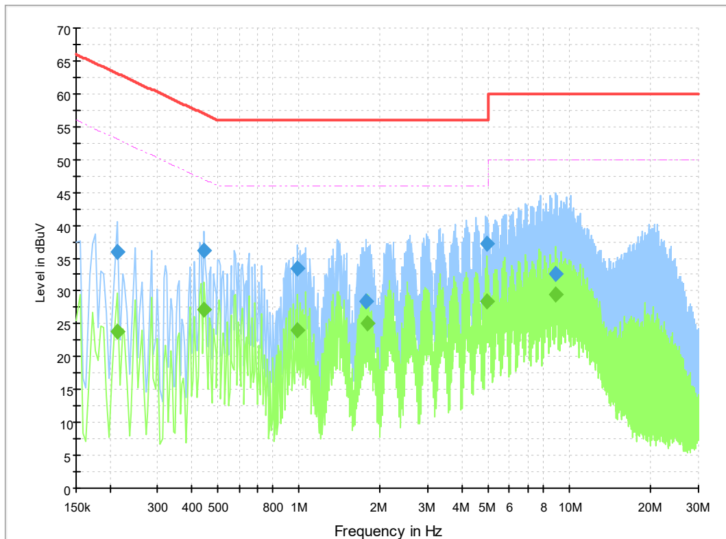
Fig.27. AC Powerline Conducted Emission-Idle
