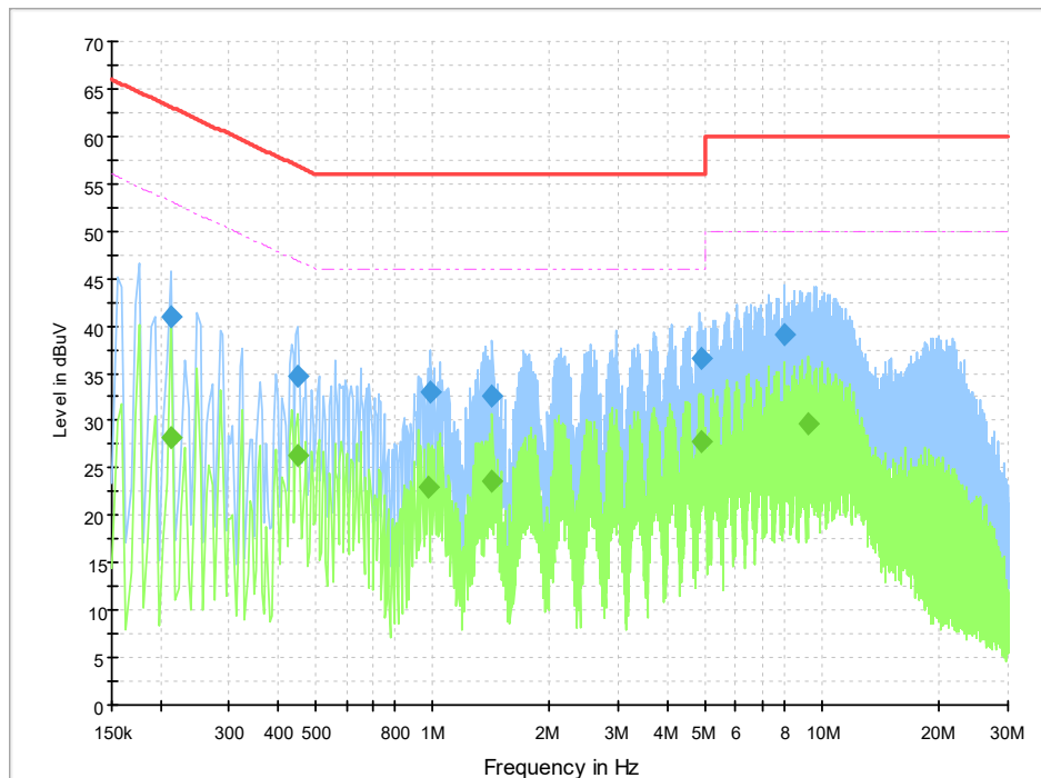
Fig.100. AC Powerline Conducted Emission- bluetooth
