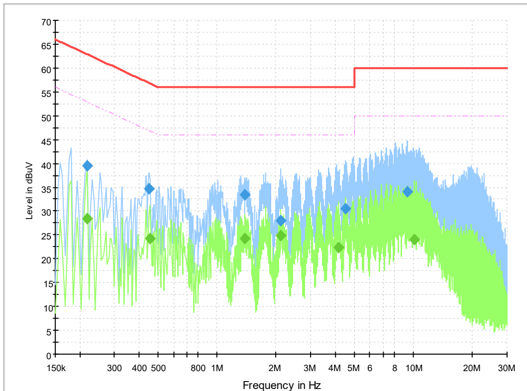
Fig.101. AC Powerline Conducted Emission-Idle
