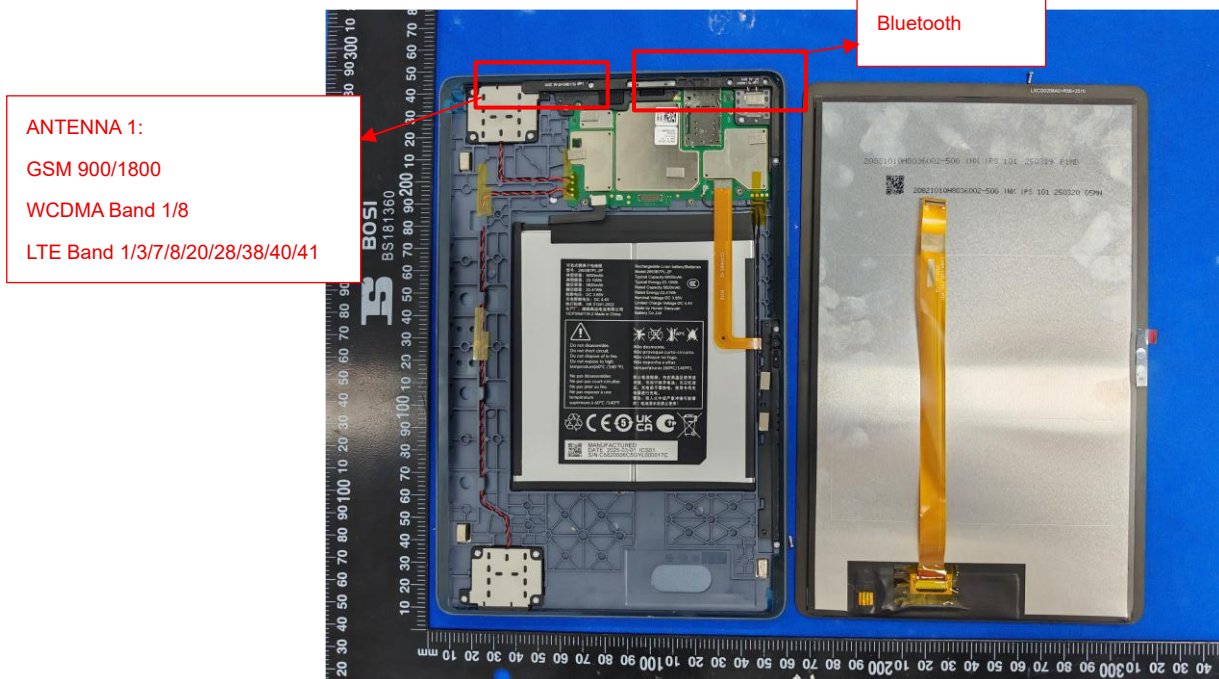
EUT UNCOVER VIEW 1
