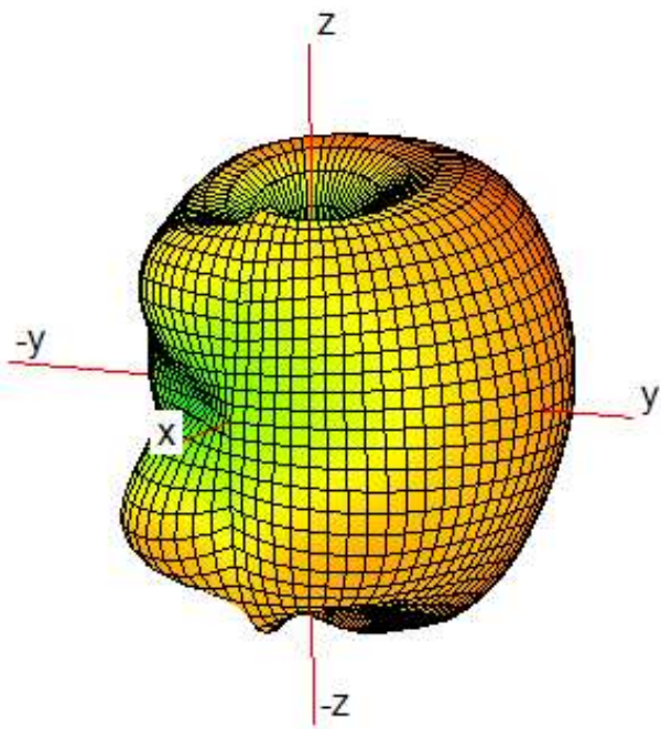
WIFI 2.4G
