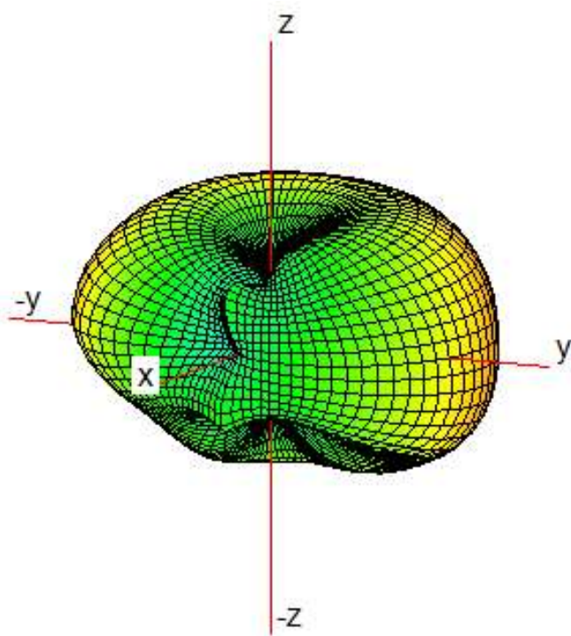
WIFI 5G
