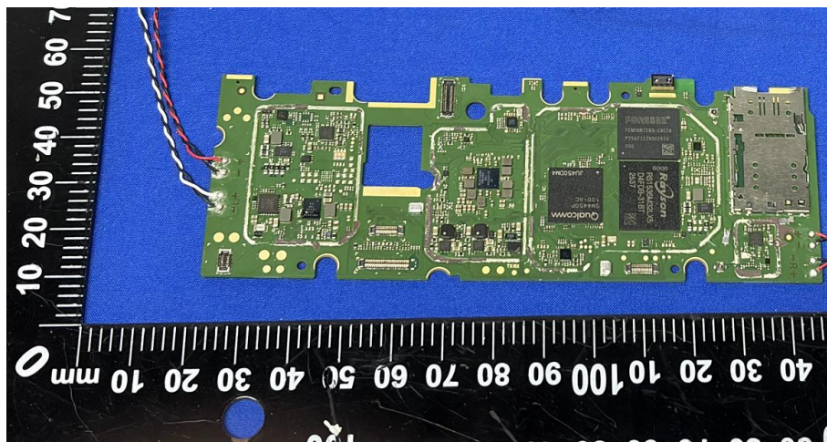
MAIN BOARD TOP VIEW (WITHOUT SHIELDING)
