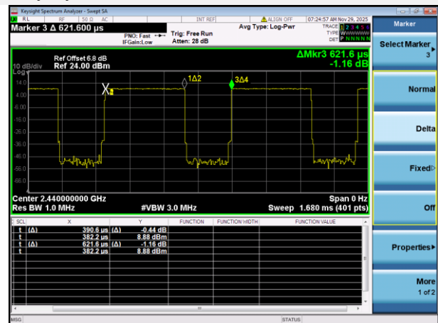
Duty Cycle
