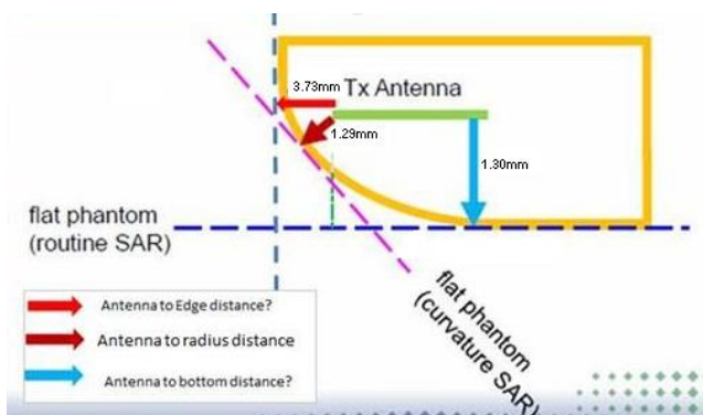
X=3.73mm, Y=1.30mm, Z=1.29mm Exterior Radius Dimension for WWAN
