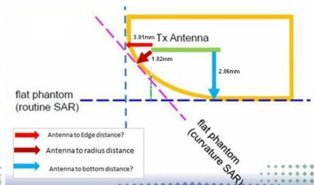
X=3.81mm, Y=2.86mm, Z=1.82mm Exterior Radius Dimension for WLAN
