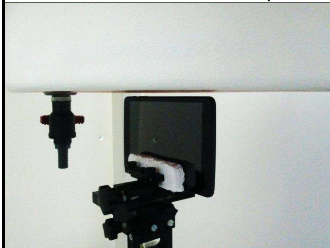
Right Side of EUT with 0.4 cm Gap
