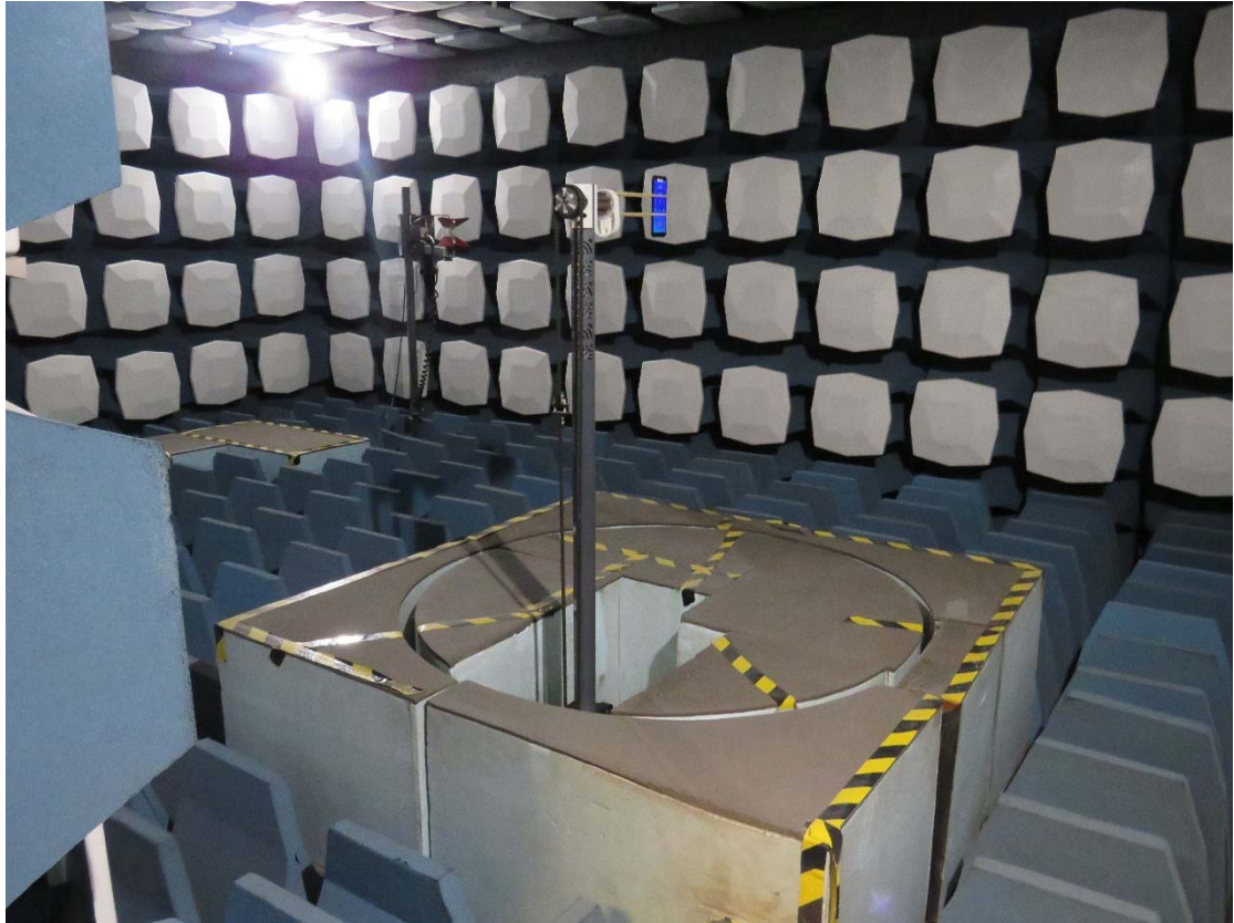
Part 22 24 Radiation Test
