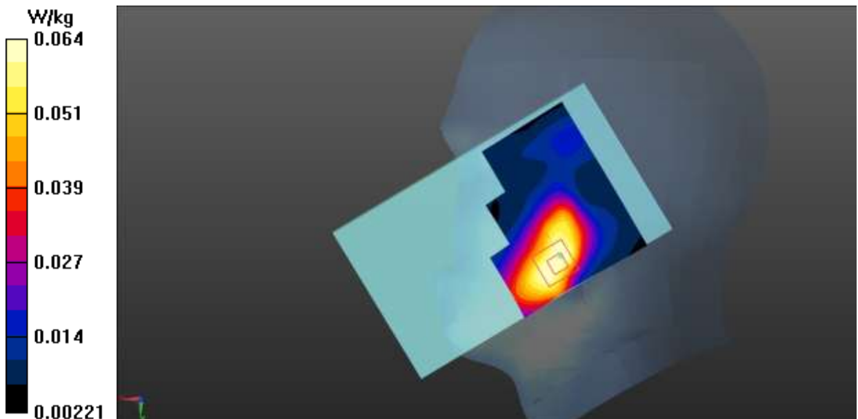
Fig.3 GSM 1900 Head
